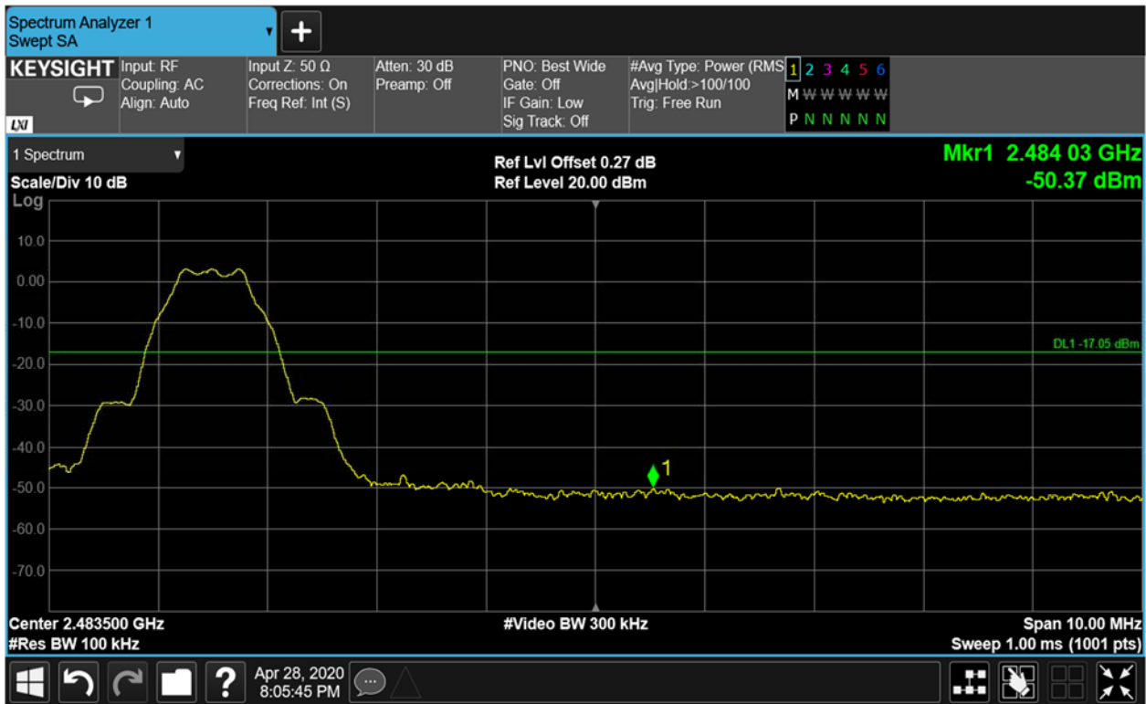
Figure 9-24 Conducted- High Band Edge (Ch. 39)
