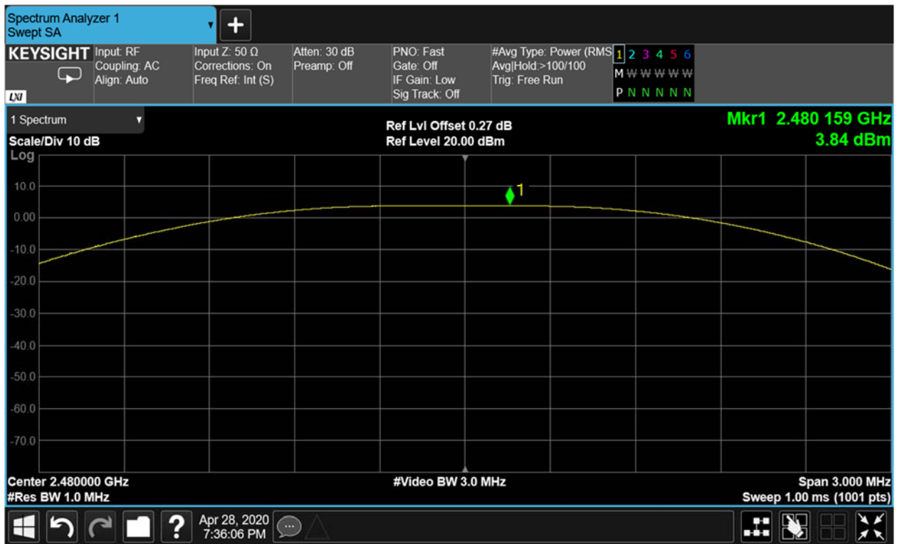
Figure 9-10 Peak Power (Ch. 39)
