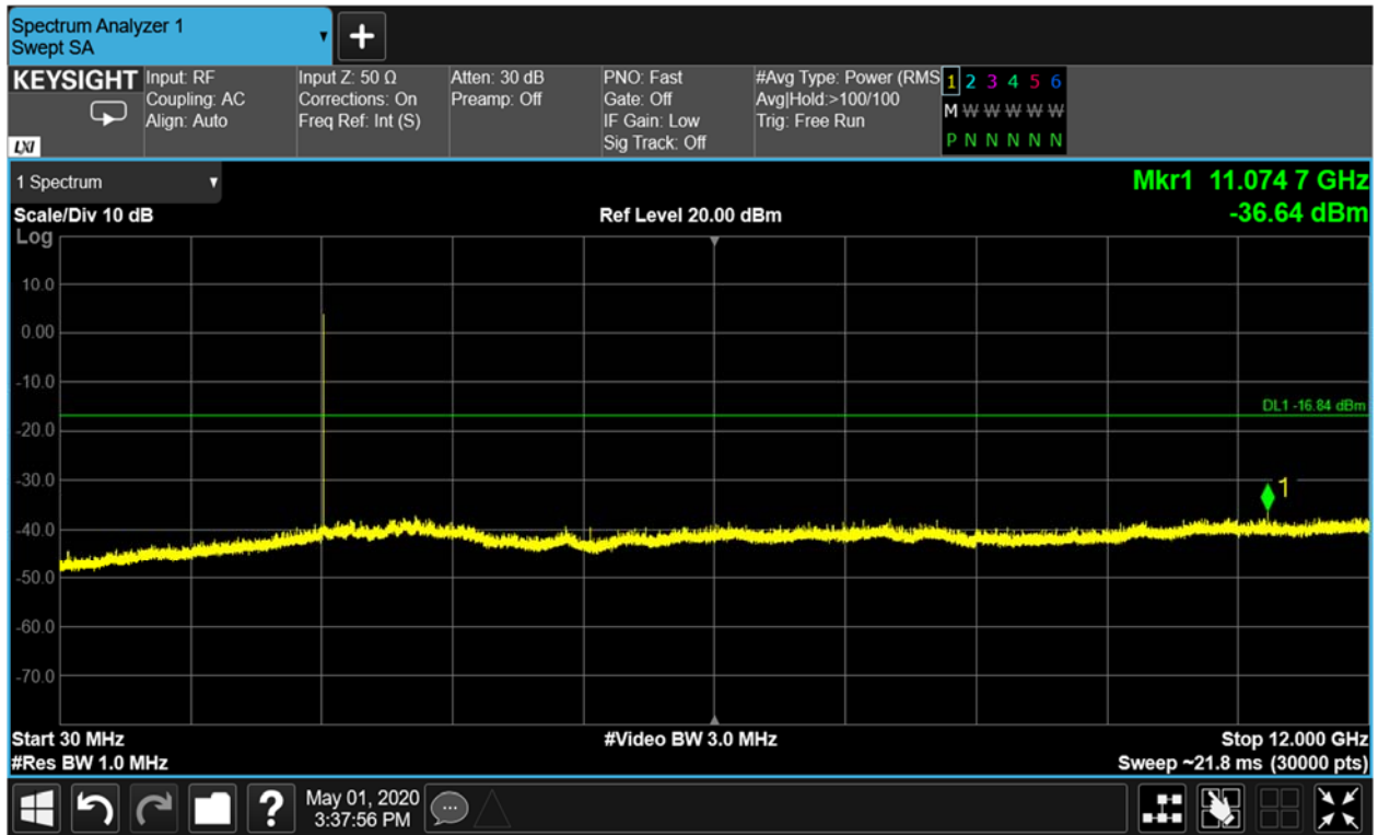
Figure 9-18 Conducted Spurious Emissions 30-12000 MHz (Ch. 19)
