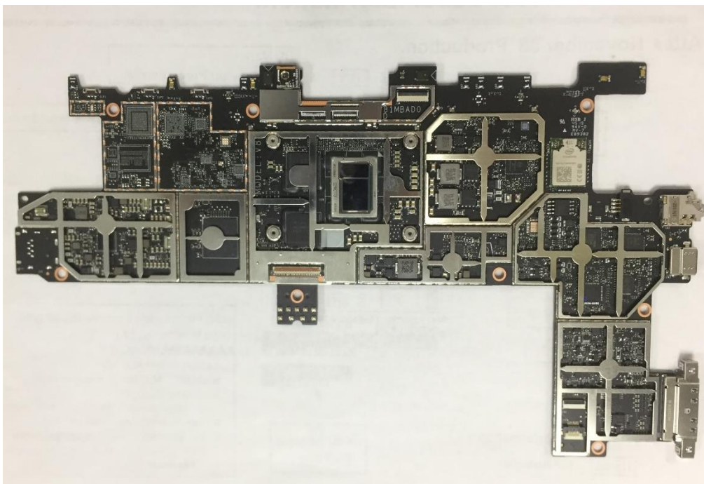
Figure 2 Main logic board-without shield cans-Top View
