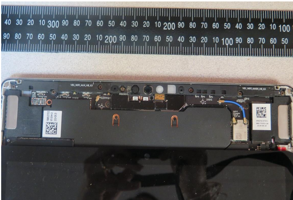
Figure 4 Close up Wi-Fi RF section
