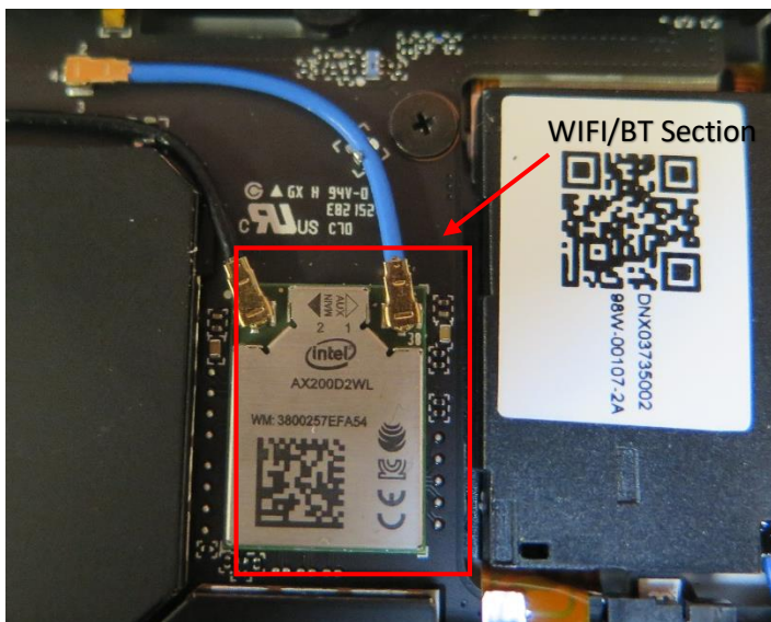
Figure 5 Close up Wi-Fi RF Module -Top View
