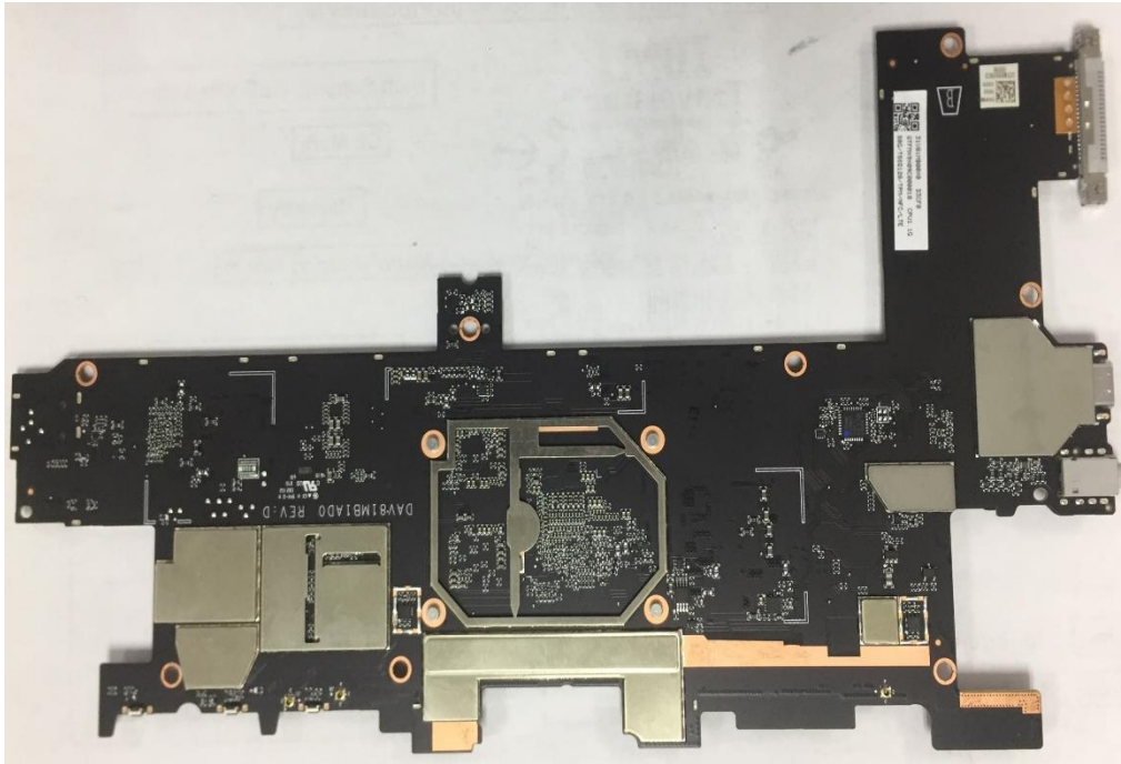
Figure 3 Main logic board-without shield cans-Back View
