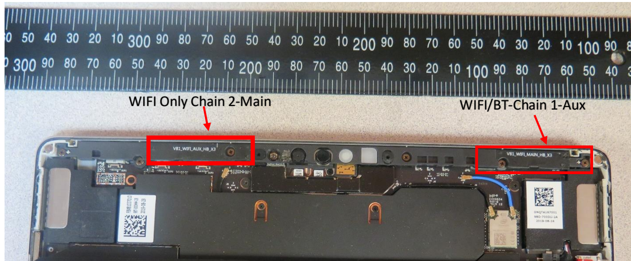
Figure 6 Wi-Fi Antenna- Close-up-Top View
