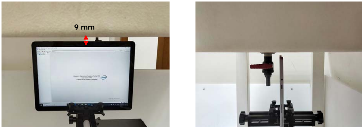
Fig.11 EUT Top side to flat phantom
