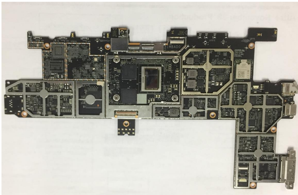
Figure 2 Main logic board-without shield cans-Top View
