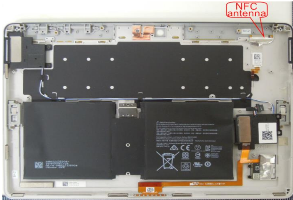
Figure 9 NFC Antenna- Close-up-Top View
