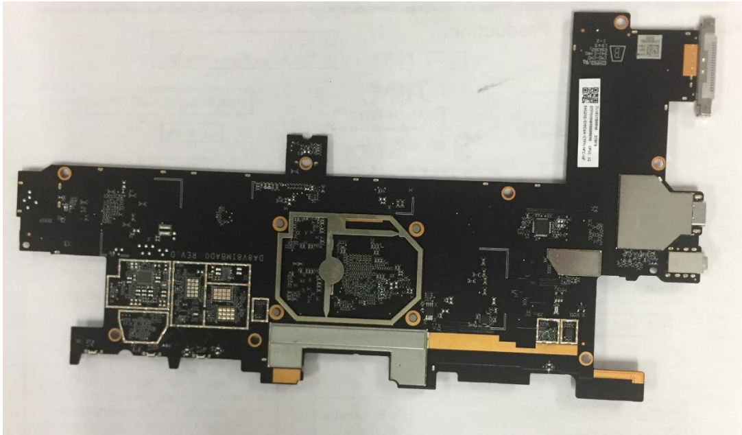
Figure 3 Main logic board-without shield cans-Back View
