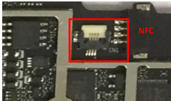
Figure 8 NFC Section- Close-up-Top View
