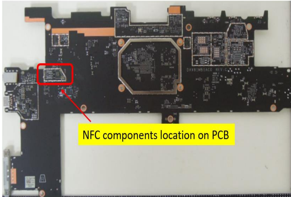
Figure 7 NFC Section- -Bottom View
