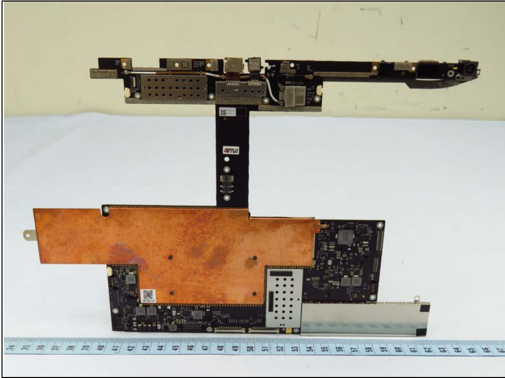
Motherboard with shield cans
