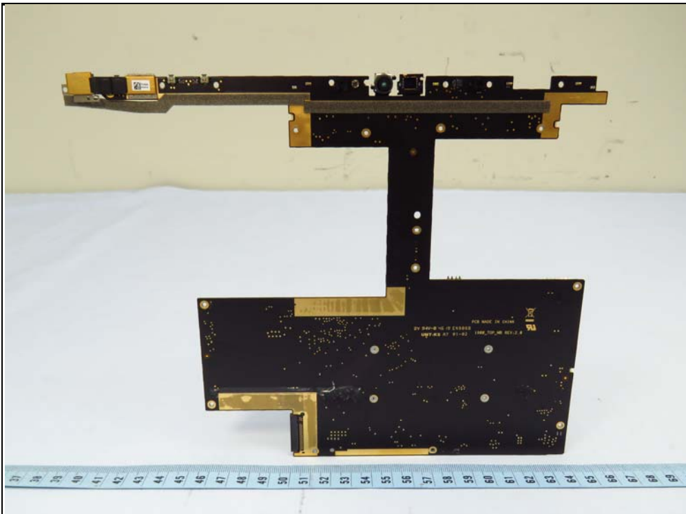
Motherboard bottom side with shield cans
