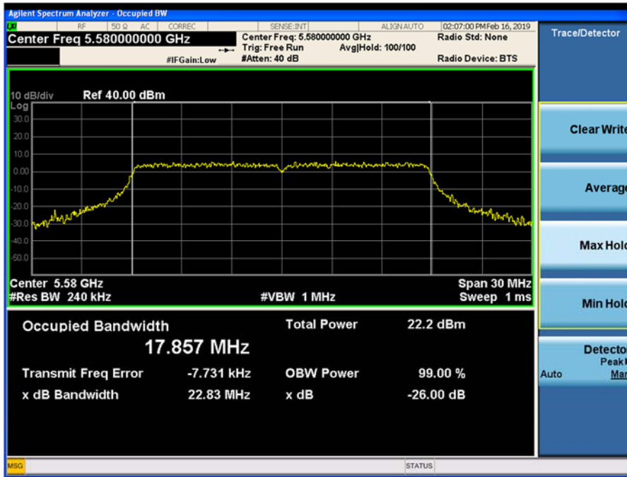
Plot 9-59. 26-dB Emission Bandwidth and 99% OBW Chain 1 802.11n HT20 (Ch. 116)
