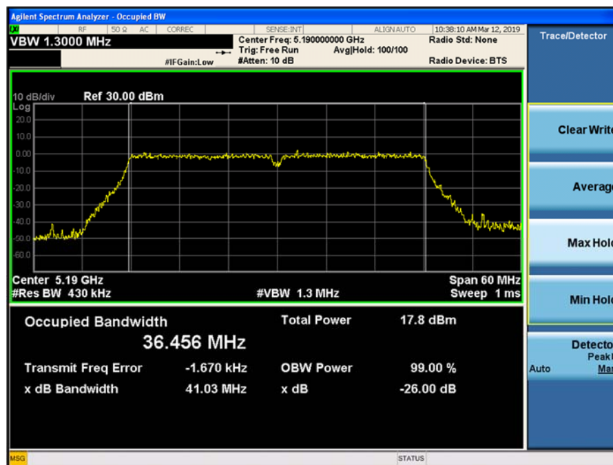
Plot 9-75. 26-dB Emission Bandwidth and 99% OBW Chain 1 802.11n HT40 (Ch. 38)
