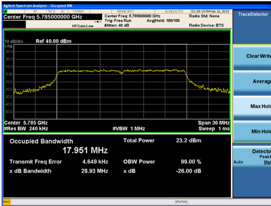
Plot 9-50. 26-dB Emission Bandwidth and 99% OBW Chain 0 802.11n HT20 (Ch. 157)
