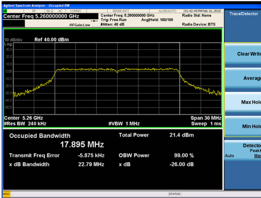
Plot 9-88. 26dB Emission Bandwidth and 99% OBW Chain 0 802.11ac VHT 20 (CH. 52)
