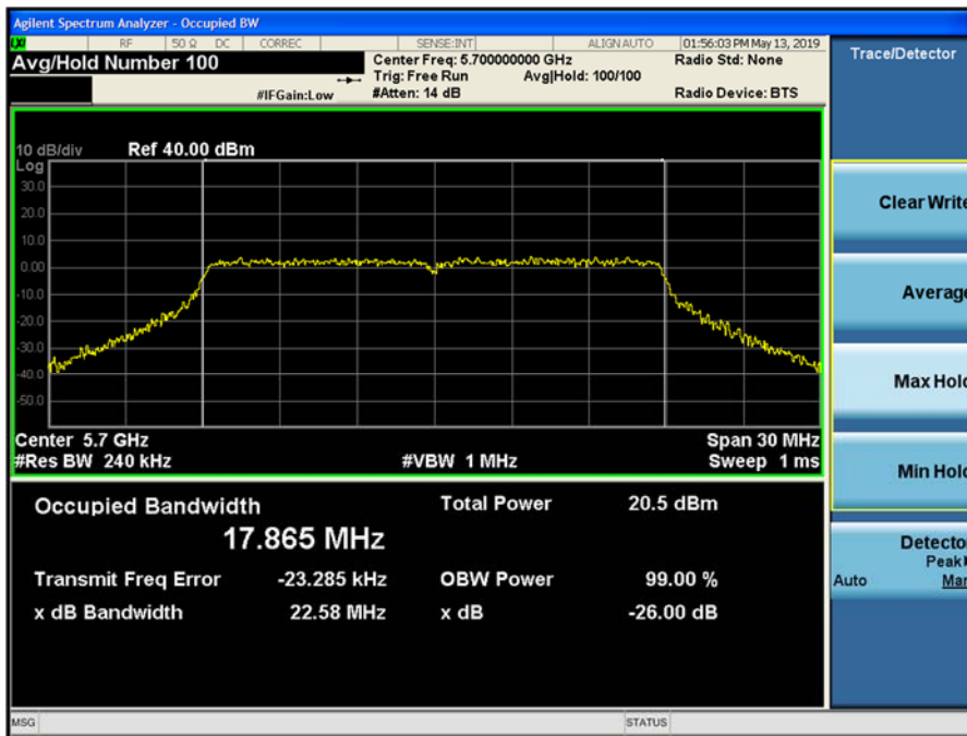
Plot 9-93. 26dB Emission Bandwidth and 99% OBW Chain 0 802.11ac VHT 20 (CH. 140)
