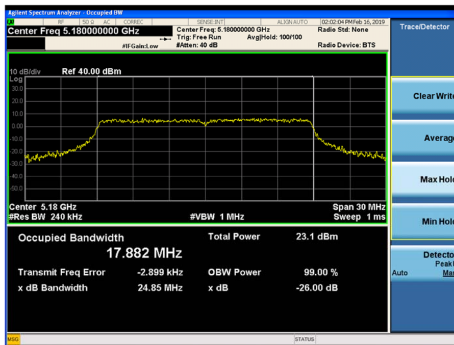
Plot 9-52. 26-dB Emission Bandwidth and 99% OBW Chain 1 802.11n HT20 (Ch. 36)
