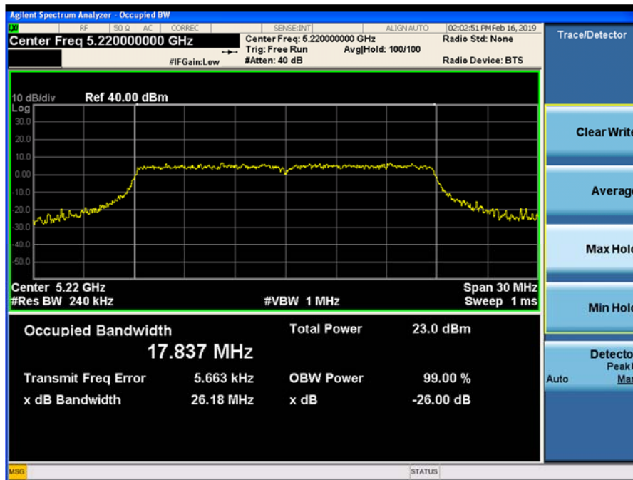
Plot 9-53. 26-dB Emission Bandwidth and 99% OBW Chain 1 802.11n HT20 (Ch. 44)
