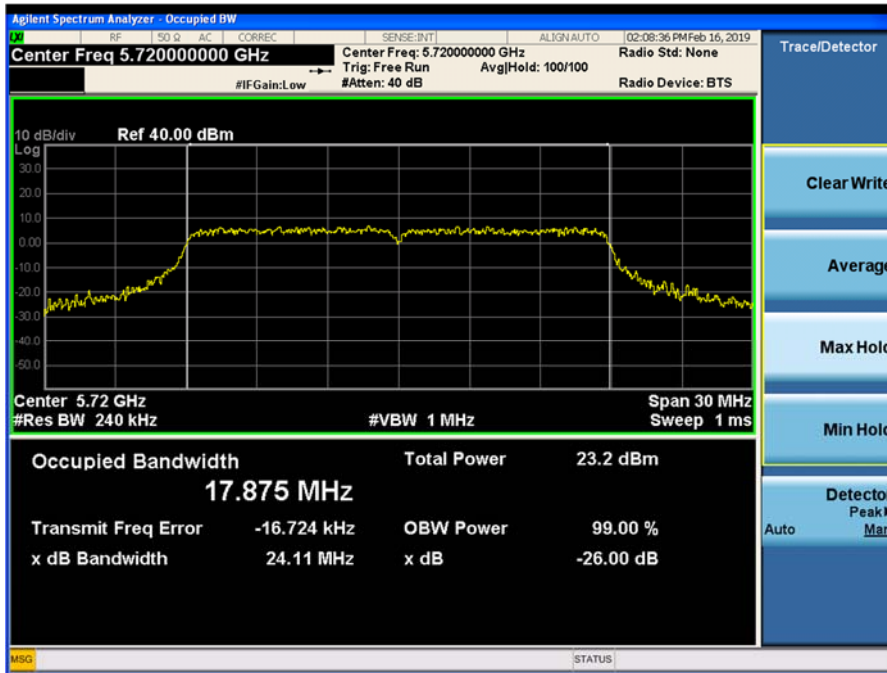
Plot 9-61. 26-dB Emission Bandwidth and 99% OBW Chain 1 802.11n HT20 (Ch. 144)
