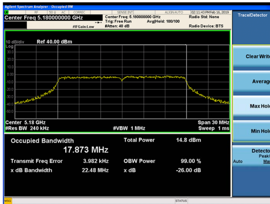
Plot 9-98. 26dB Emission Bandwidth and 99% OBW Chain 1 802.11ac VHT 20 (CH. 36)
