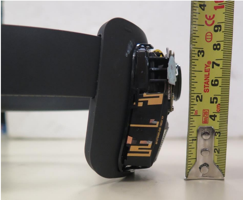
Figure 7 Wi-Fi Chain 0 & 1 Antenna View
