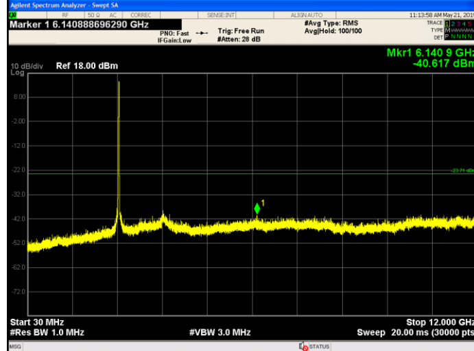
Figure 9-212 Chain 0 Conducted Spurious Emissions 30MHz-12GHz 802.11g - Ch.11
