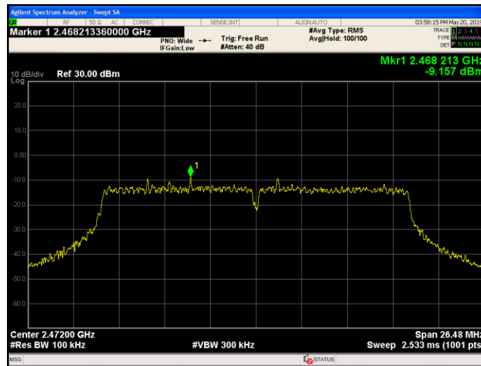
Figure 9-253 Chain 0 Reference Level 802.11gn20-Ch.13
