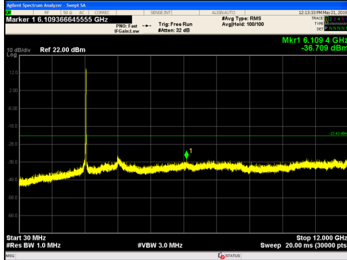
Figure 9-215 Chain 1 Conducted Spurious Emissions 30 MHz-12GHz 802.11g - Ch.11
