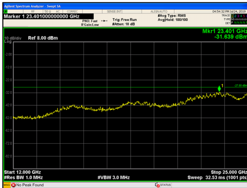
Figure 9-18 Conducted Spurious Emissions 12-25 GHz (Ch.0)
