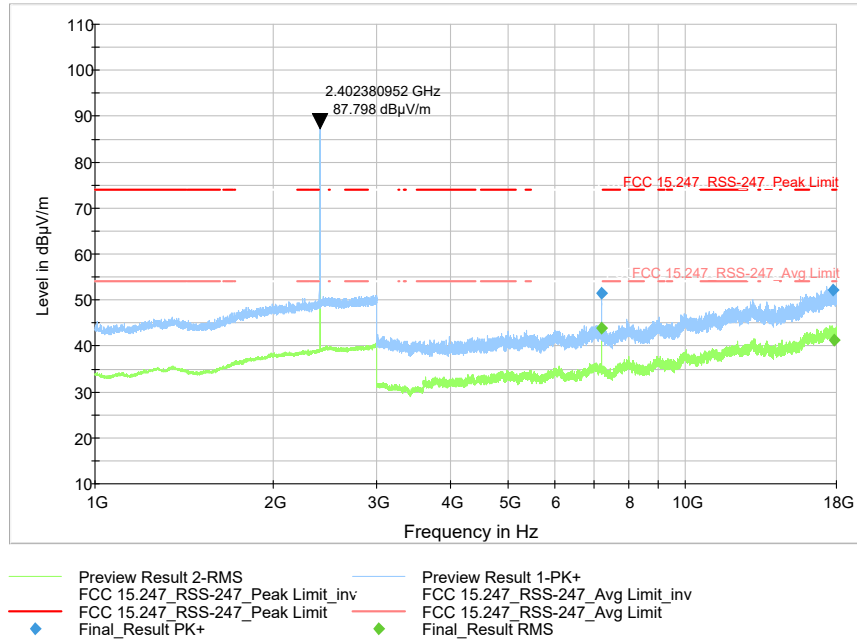
Figure 9-33 Radiated Spurious Emissions 1-18 GHz (Ch. 0)
