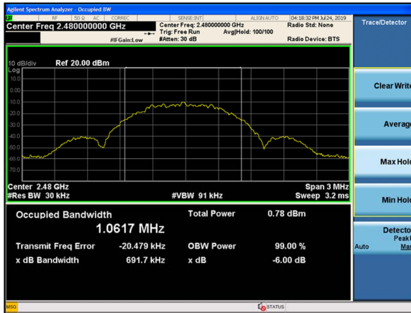
Figure 9-9 99% Bandwidth (Ch. 39)
