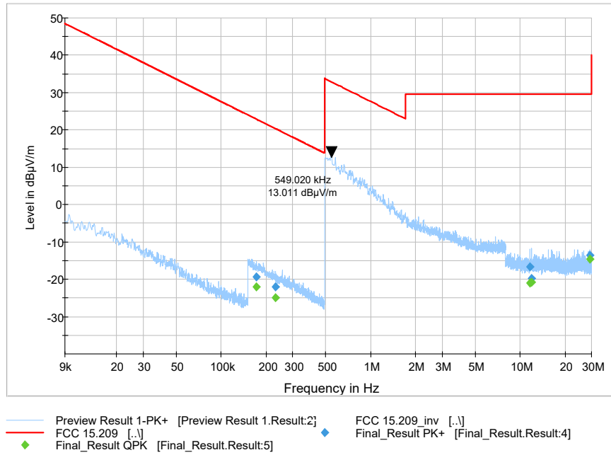
Figure 9-31 Radiated Spurious Emissions (Ch. 39) 2480 (9kHz – 30MHz)
