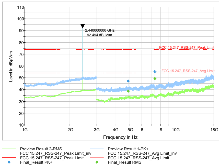
Figure 9-34 Radiated Spurious Emissions 1-18 GHz (Ch. 19)
