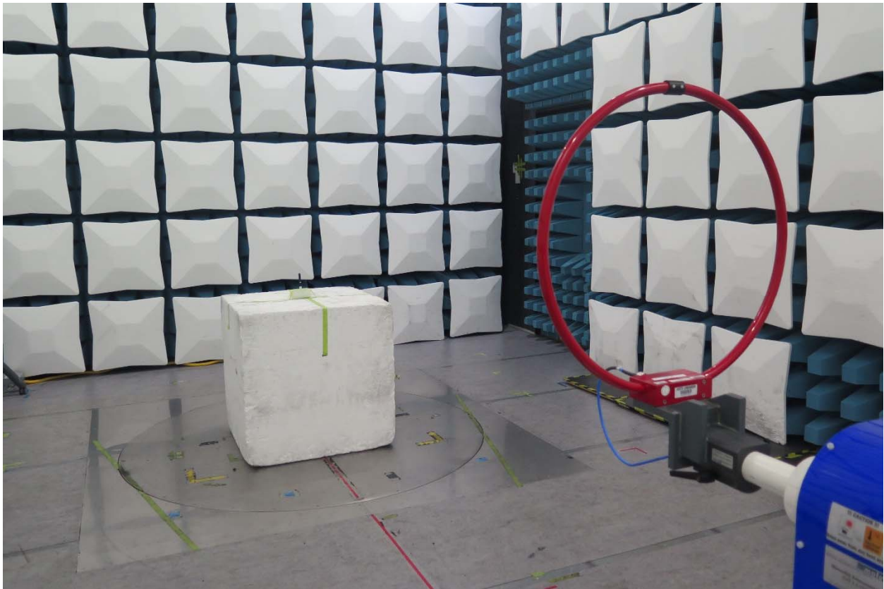
Figure 1 Radiated Spurious Emissions Test Setup (9KHz-30MHz)
