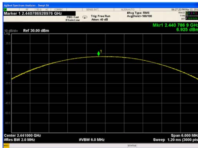
Figure 9-17 Peak Power (Ch. 39, 2-DH5)
