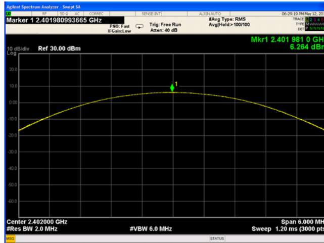
Figure 9-19 Peak Power (Ch. 0, 3-DH5)
