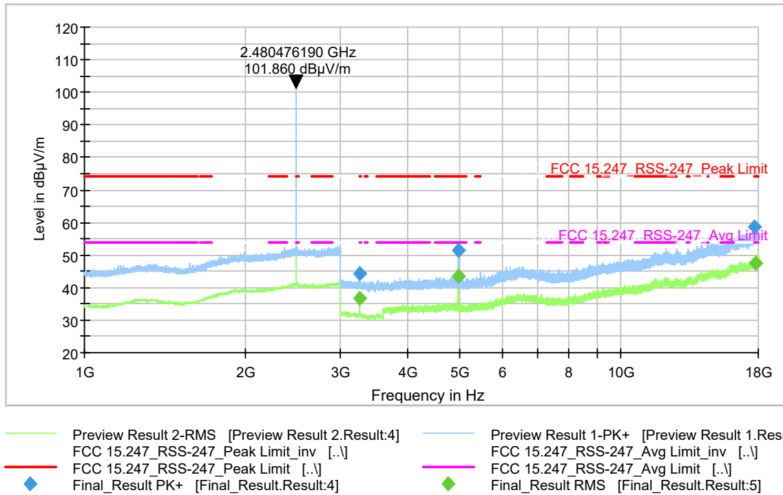
Figure 9-636 Radiated Spurious Emissions (Ch. 78) 1-DH5 (1-18 GHz)
