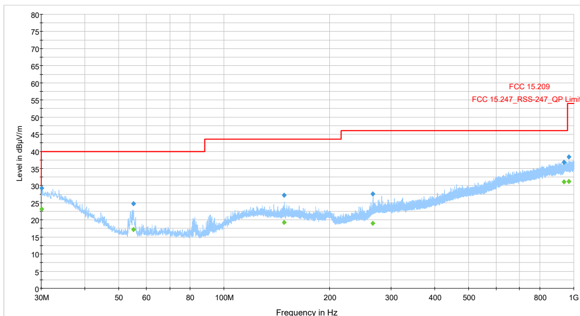
Preview Result 1-PK+ FCC 15.209 FCC 15.247_RSS-247_QP Limit Final_Result PK+ Final_Result QPK
