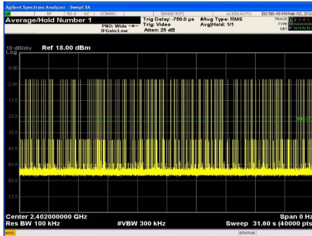
Figure 9-28 Time of Occupancy - DH3
