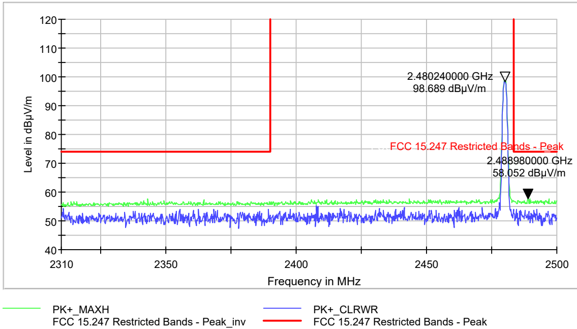
Figure 9-62 Restricted Band Edge 1-DH5 Mode– Ch. 78 (2483.5-2500MHz) – Peak
