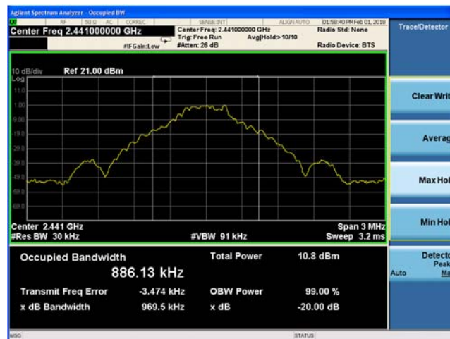
Figure 9-5 20dB Bandwidth (Ch. 39, 1-DH5)
