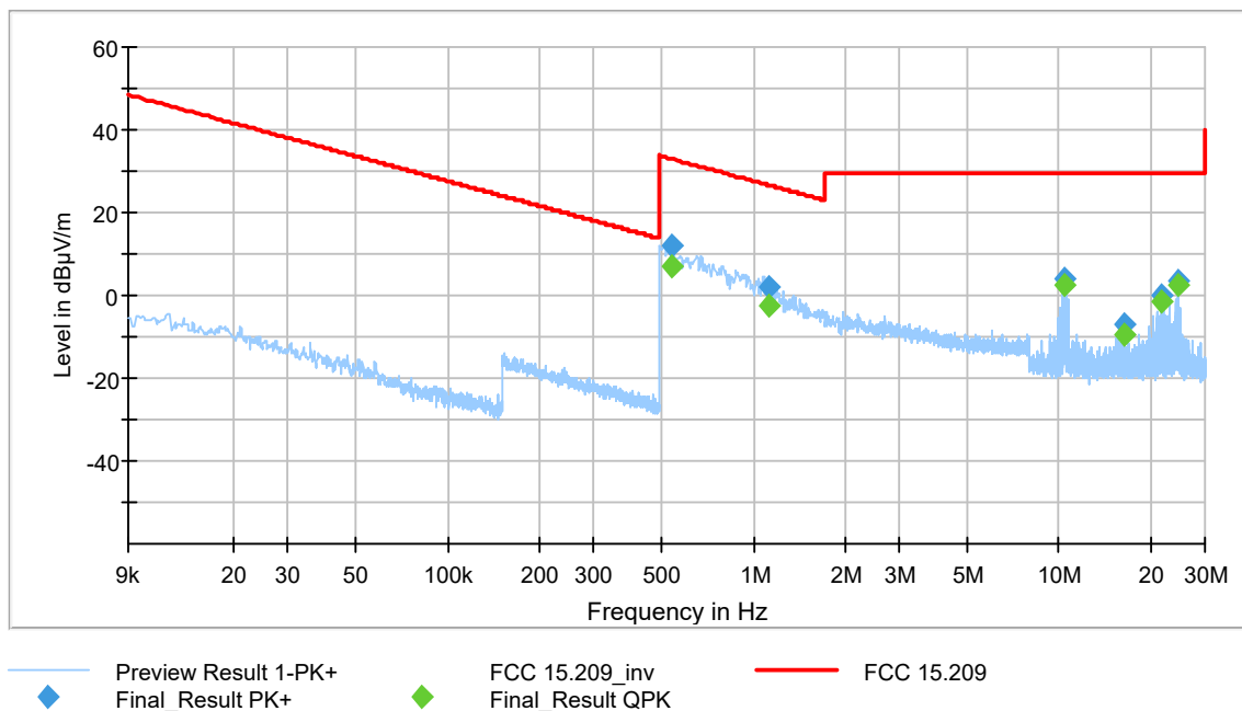
Plot 9-72. Radiated Spurious Emissions (Ch. 39) 1-DH5 (9kHz- 30MHz)
