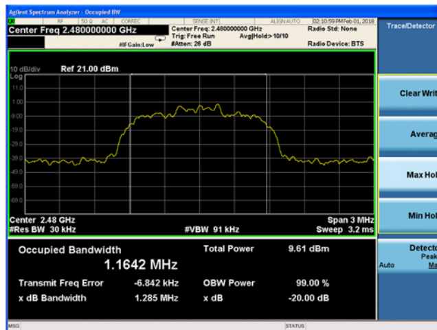
Figure 9-9 20dB Bandwidth (Ch. 78, 2-DH5)
