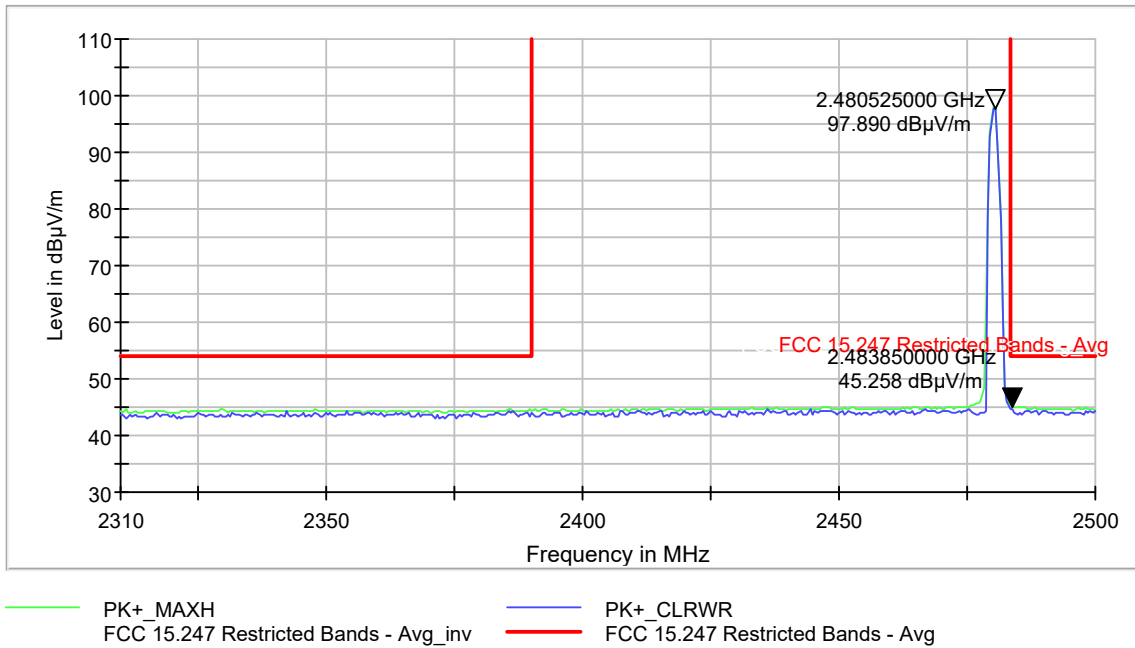
Figure 9-63 Restricted Band Edge 1-DH5 Mode– Ch. 78 (2483.5-2500MHz) – Average
