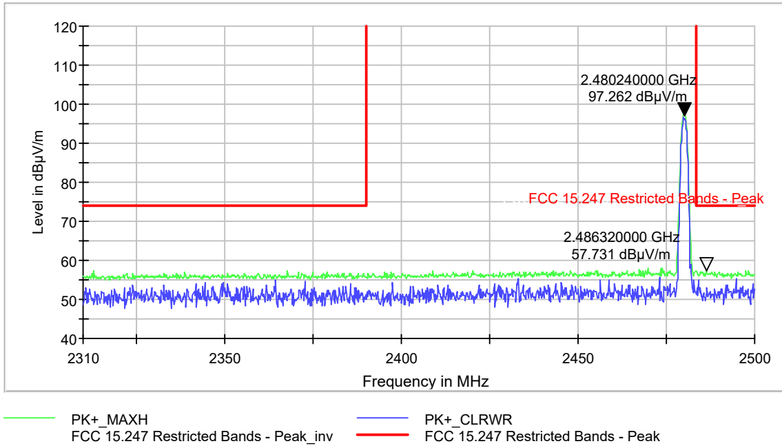
Figure 9-66 Restricted Band Edge 2-DH5 Mode– Ch. 78 (2483.5-2500MHz) – Peak
