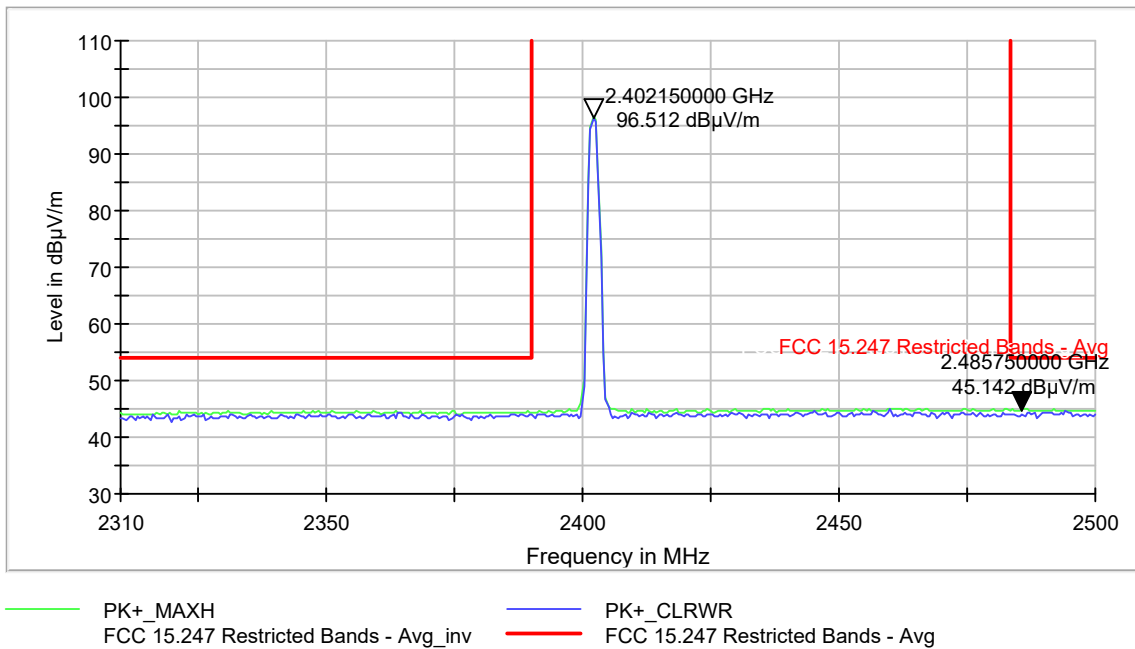
Figure 9-61 Restricted Band Edge 1-DH5 Mode- Ch. 0 (2310-2390MHz) – Average
