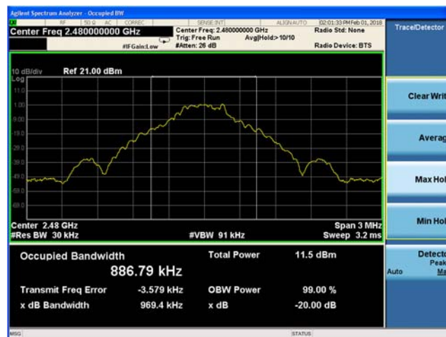
Figure 9-6 20dB Bandwidth (Ch. 78, 1-DH5)
