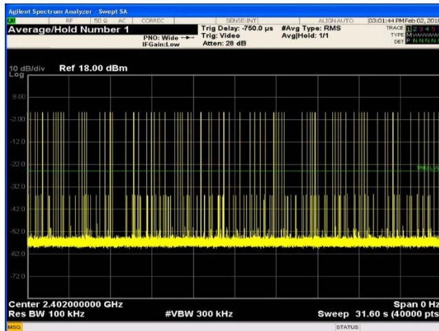
Figure 9-29 Time of Occupancy - DH5
