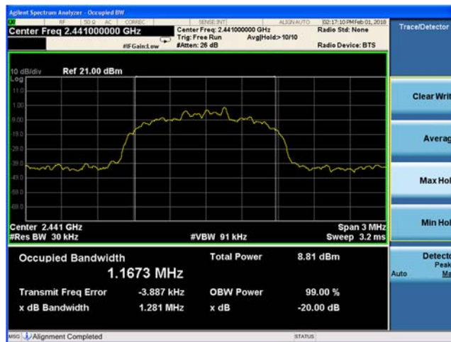
Figure 9-11 20dB Bandwidth (Ch. 39, 3-DH5)
