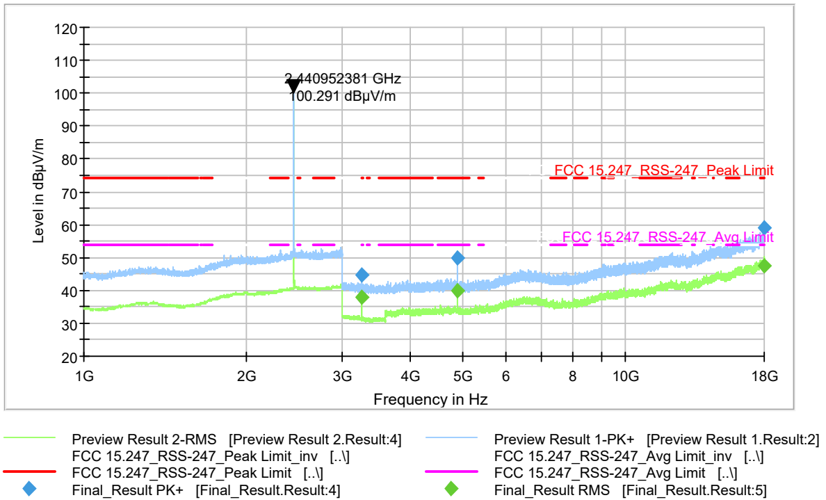
Figure 9-78 Radiated Spurious Emissions (Ch. 39) 2-DH5 (1-18 GHz)
