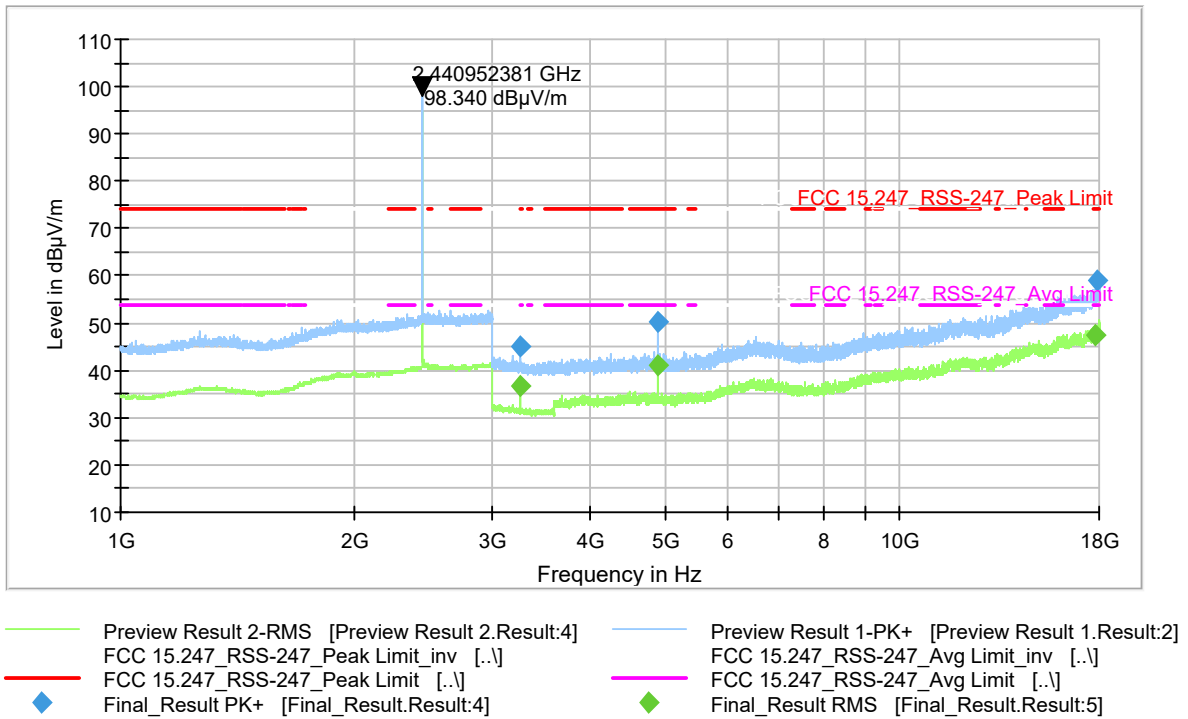
Figure 9-81 Radiated Spurious Emissions (Ch. 39) 3-DH5 (1-18 GHz)
