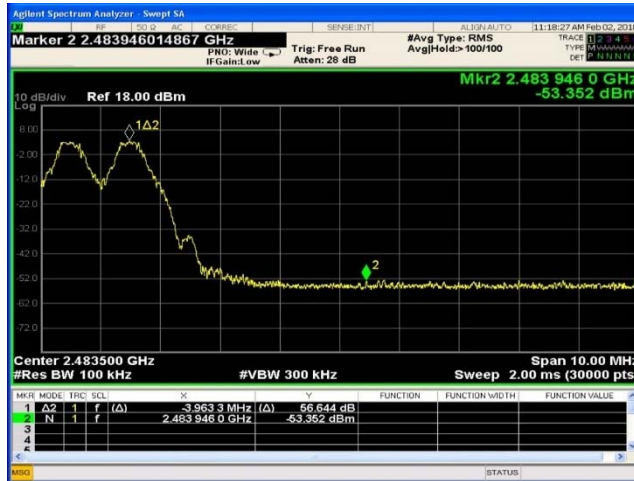
Figure 9-39 High Channel Band 1-DH5 Mode (Hopping enabled)
