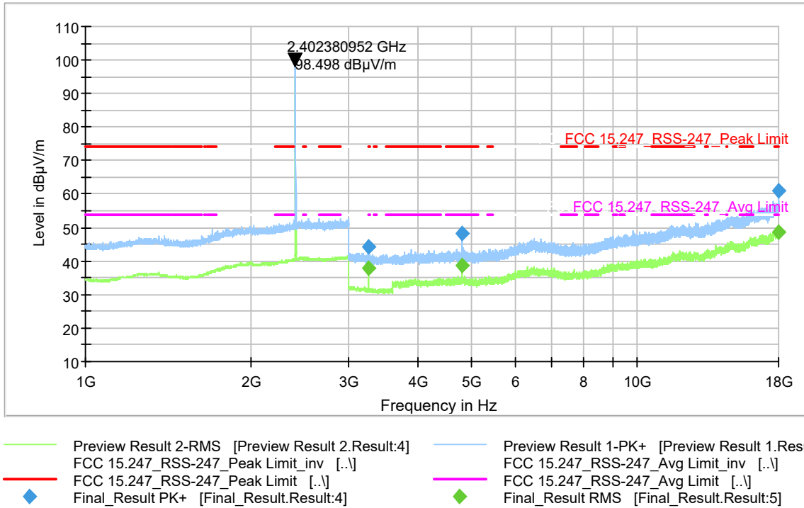
Figure 9-647 Radiated Spurious Emissions (Ch. 0) 2-DH5 (1-18 GHz)
