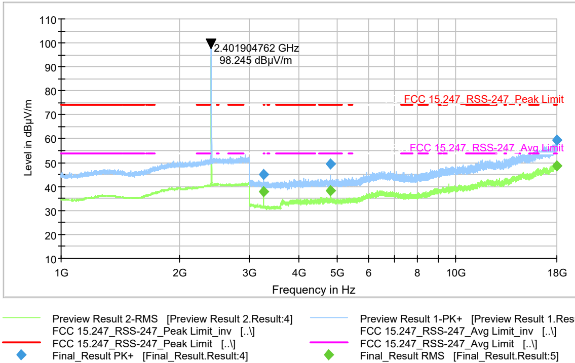
Figure 9-80 Radiated Spurious Emissions (Ch. 0) 3-DH5 (1-18 GHz)
