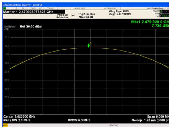
Figure 9-15 Peak Power (Ch. 78, 1-DH5)
