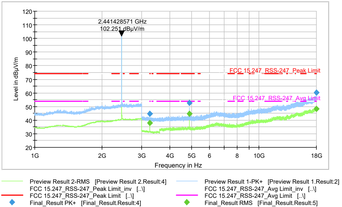
Figure 9-625 Radiated Spurious Emissions (Ch. 39) 1-DH5 (1-18 GHz)
