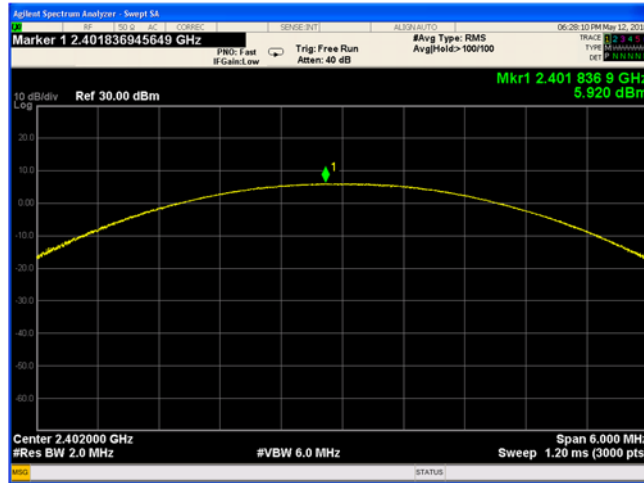
Figure 9-16 Peak Power (Ch. 0, 2-DH5)
