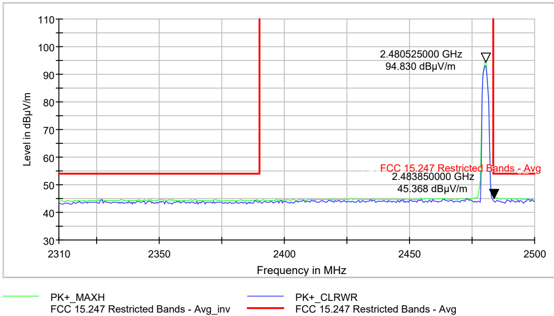
Figure 9-67 Restricted Band Edge 2-DH5 Mode– Ch. 78 (2483.5-2500MHz) – Average
