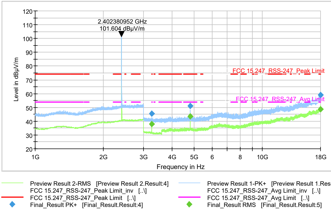
Figure 9-614 Radiated Spurious Emissions (Ch. 0) 1-DH5 (1-18 GHz)
