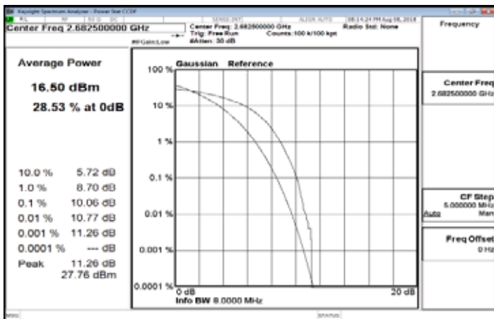
LTE_Band41_15MHz_16QAM_75_0_HighCH41515
