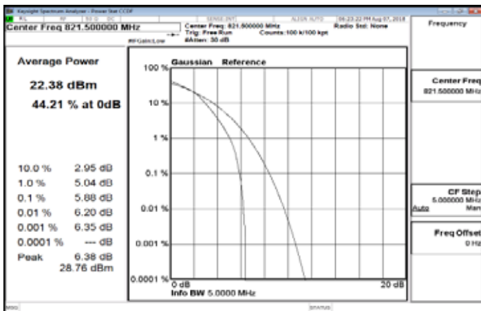
Part 90_LTE_Band26_5MHz_16QAM_25_0_HighCH26765
