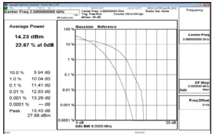
LTE_Band41_20MHz_16QAM_100_0_HighCH41490
