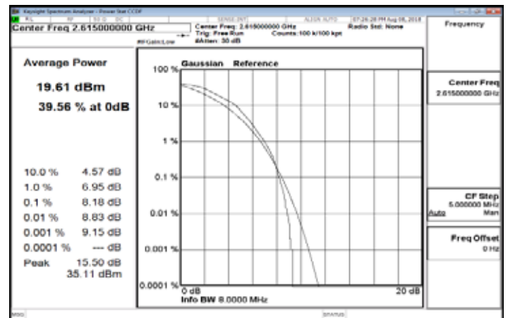
LTE_Band38_10MHz_16QAM_50_0_HighCH38200-2615
