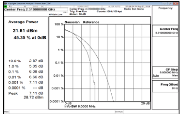
LTE_Band30_10MHz_16QAM_50_0_MidCH27710
