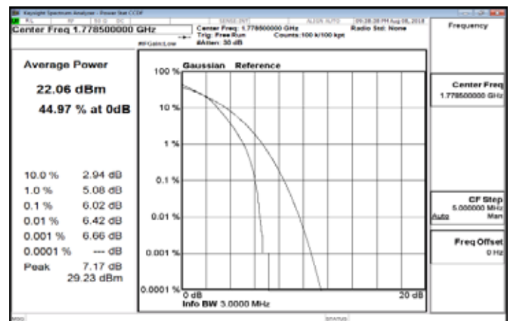
LTE_Band66_3MHz_16QAM_15_0_HighCH132657
