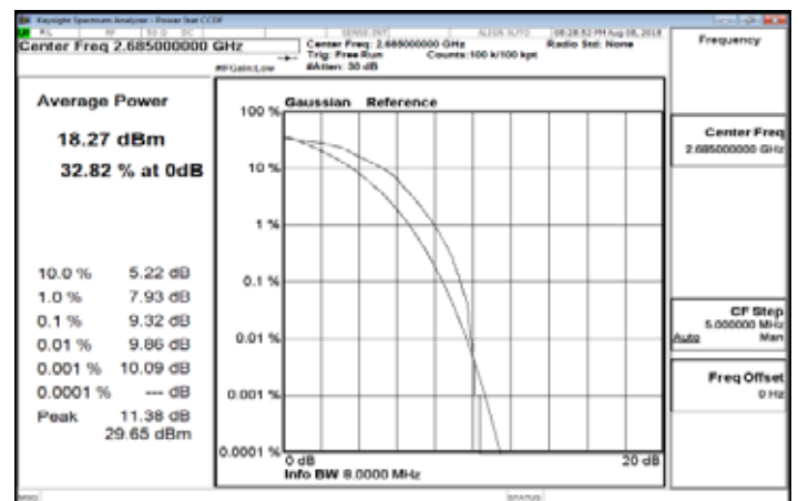
LTE_Band41_10MHz_16QAM_50_0_HighCH41540
