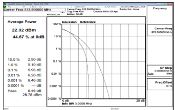
Part 90_LTE_Band26_3MHz_16QAM_15_0_HighCH26775
