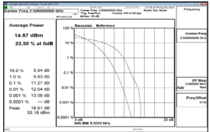
LTE_Band41_20MHz_16QAM_100_0_MidCH40620
