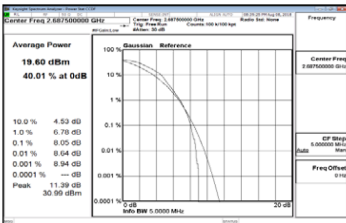
LTE_Band41_5MHz_16QAM_25_0_HighCH41565
