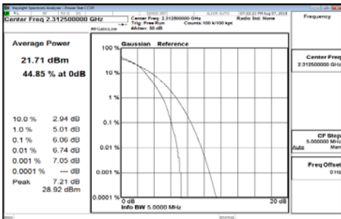
LTE_Band30_5MHz_16QAM_25_0_HighCH27735
