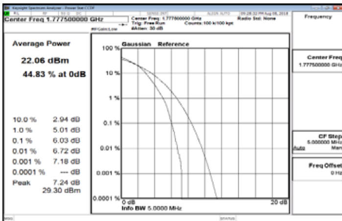
LTE_Band66_5MHz_16QAM_25_0_HighCH132647
