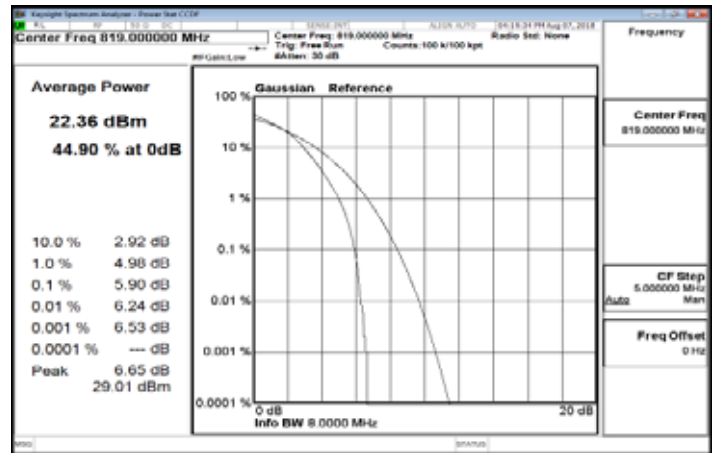
Part 90_LTE_Band26_10MHz_64QAM_50_0_MidCH26740
