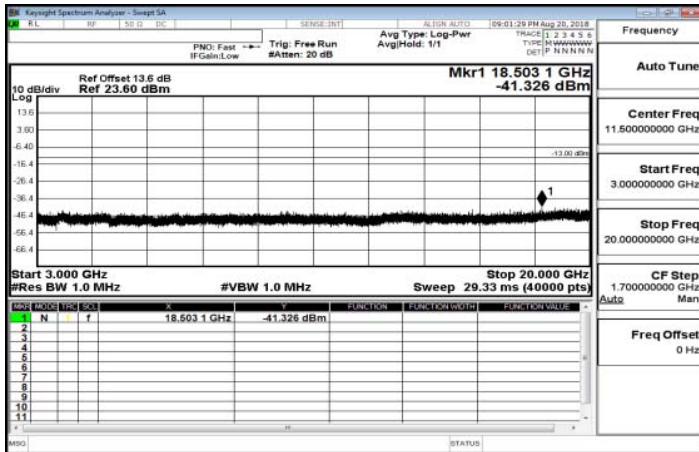
3GHz-20GHz_Band12_5MHz_QPSK_1_0_LowCH23035-701.5
