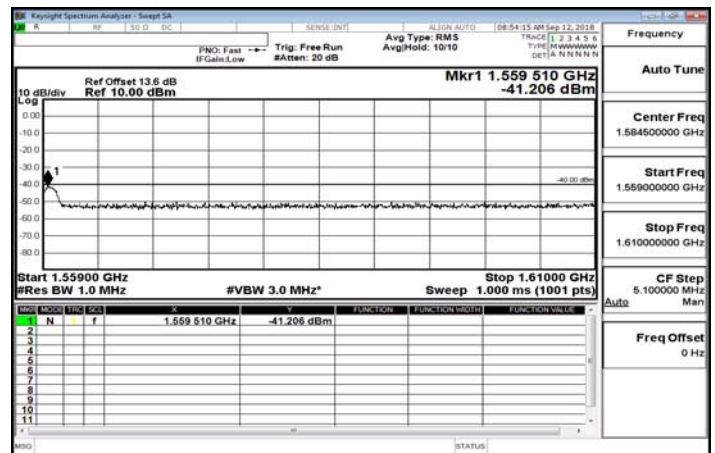
1559MHz-1610MHz_Band13_5MHz_QPSK_1_0_MidCH23230-782
