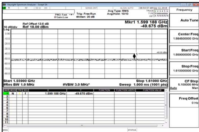
1559MHz~1610MHz_Band13_10MHz_QPSK_1_0_MidCH23230-782
