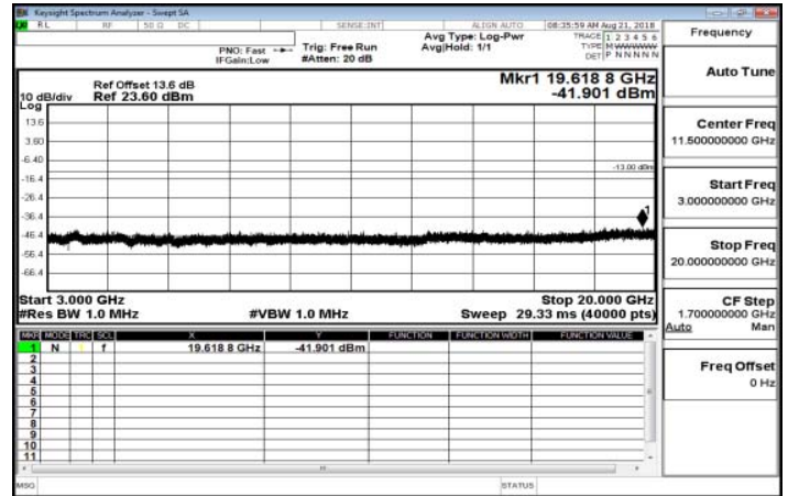
3GHz-20GHz_Band13_5MHz_QPSK_1_0_MidCH23230-782
