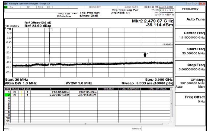
30MHz-3GHz_Band12_1_4MHz_QPSK_1_0_HighCH23173-715.3
