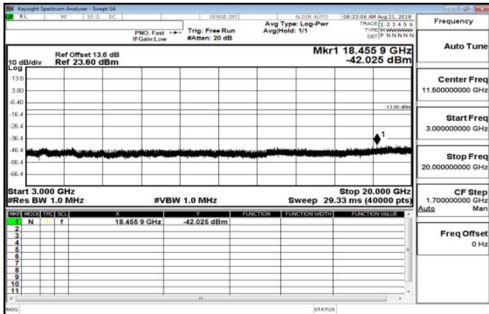
3GHz~20GHz_Band13_10MHz_QPSK_1_0_MidCH23230-782
