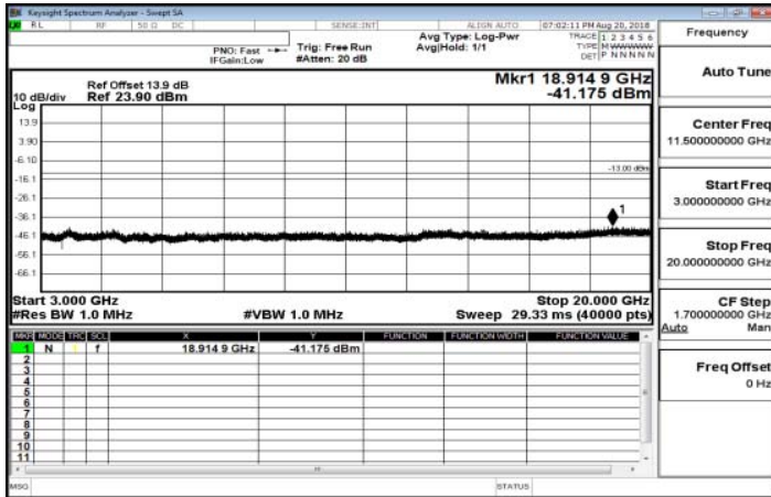
3GHz-20GHz_Band25_1_4MHz_OPSK_1_0_MidCH26365-1882.5
