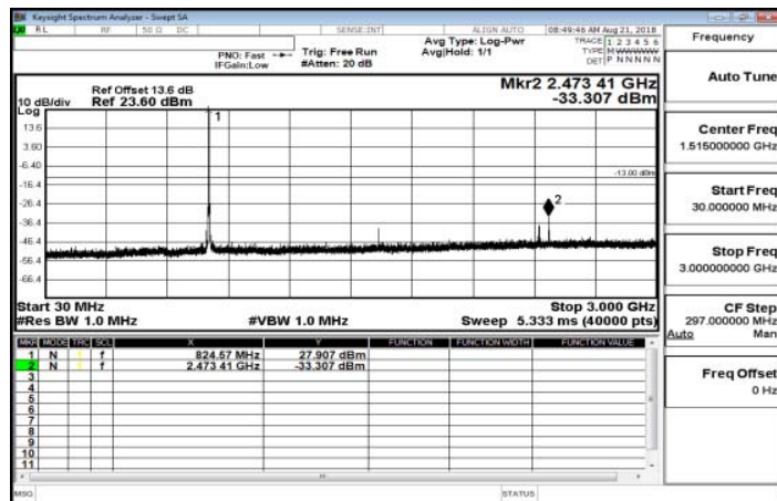
30MHz-3GHz_Band26_5MHz_QPSK_1_0_LowCH26815
