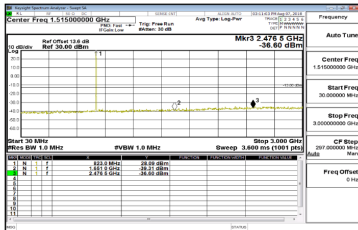
30MHz-3GHz_Band26_5MHz_QPSK_1_0_LowCH26805
