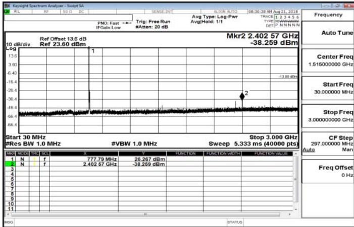
30MHz~3GHz_Band13_10MHz_QPSK_1_0_MidCH23230-782
