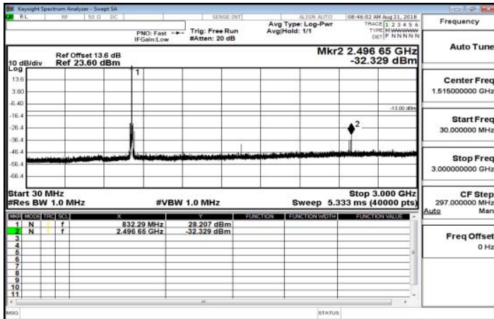
30MHz-3GHz_Band26_10MHz_QPSK_1_0_MidCH26915
