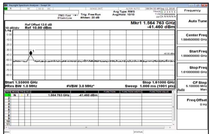
1559MHz-1610MHz_Band13_5MHz_QPSK_1_0_HighCH23255-784.5
