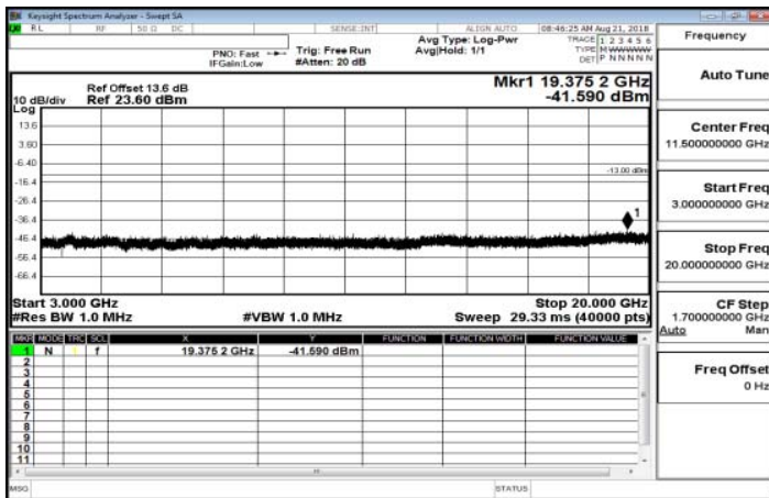
3GHz-20GHz_Band26_10MHz_QPSK_1_0_MidCH26915
