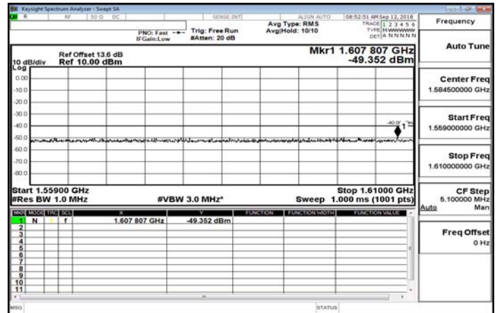
1559MHz-1610MHz_Band13_5MHz_QPSK_1_0_LowCH23205-779.5
