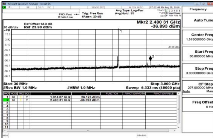
30MHz-3GHz_Band25_1_4MHz_OPSK_1_0_HighCH26683-1914.3
