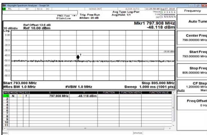
793MHz-806MHz_Band13_5MHz_QPSK_1_0_HighCH23255-784.5
