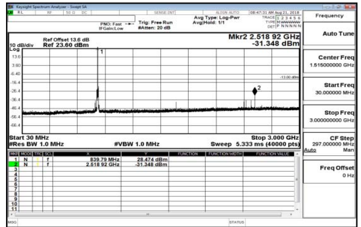
30MHz-3GHz_Band26_10MHz_QPSK_1_0_HighCH26990
