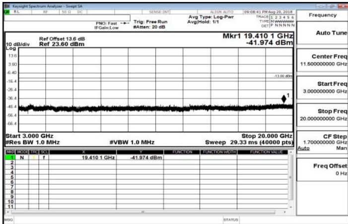
3GHz-20GHz_Band12_1_4MHz_QPSK_1_0_LowCH23017-699.7
