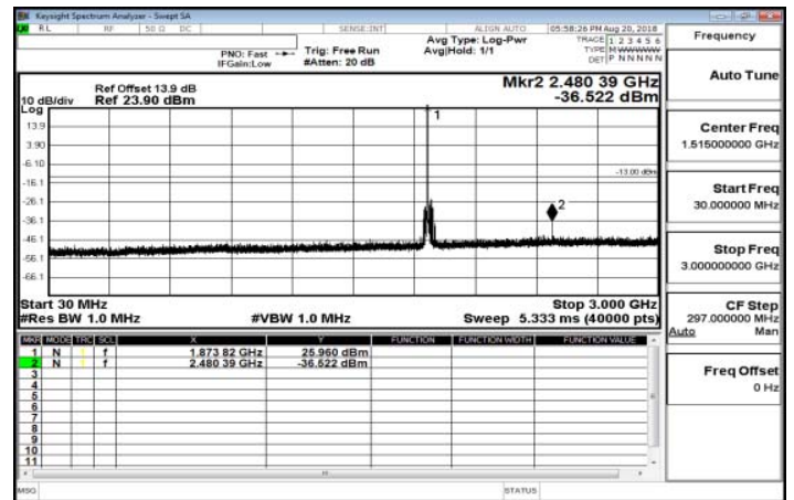
30MHz~3GHz_Band25_20MHz_QPSK_1_0_MidCH26365-1882.5
