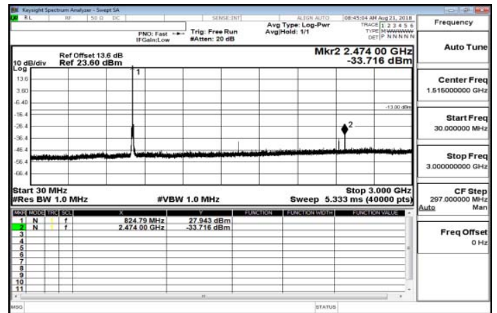
30MHz-3GHz_Band26_10MHz_QPSK_1_0_LowCH26840
