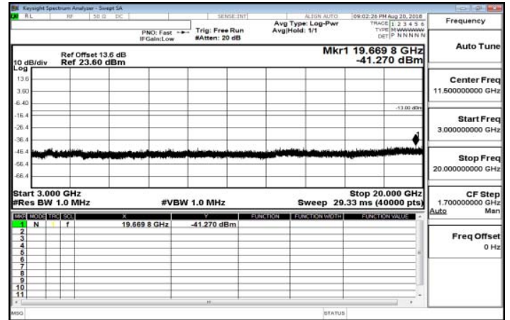
3GHz-20GHz_Band12_5MHz_QPSK_1_0_MidCH23095-707.5
