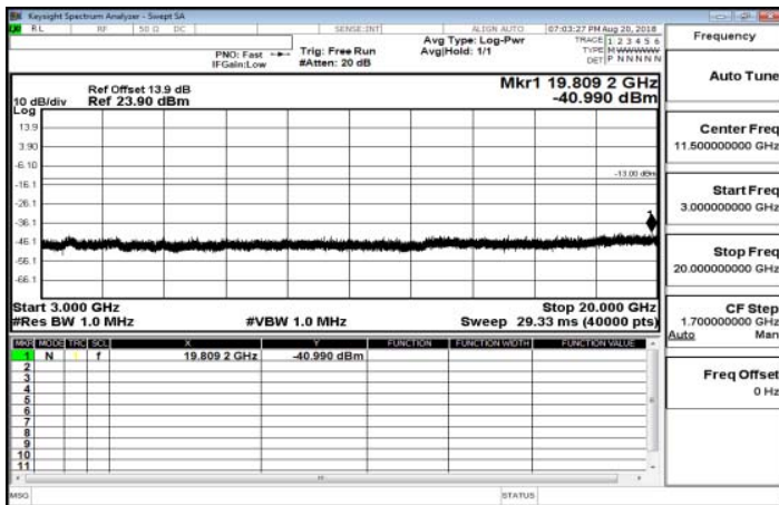
3GHz-20GHz_Band25_1_4MHz_OPSK_1_0_HighCH26683-1914.3
