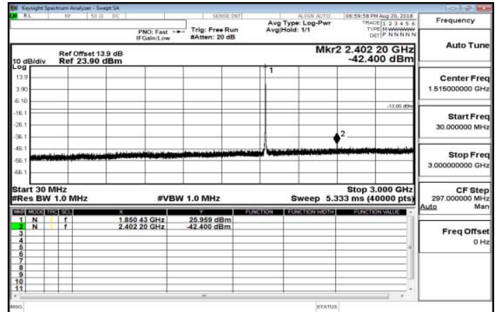
30MHz~3GHz_Band25_1_4MHz_QPSK_1_0_LowCH26047-1850.7
