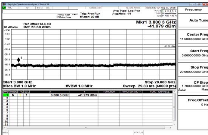
3GHz-20GHz_Band26_1_4MHz_QPSK_1_0_HighCH27033
