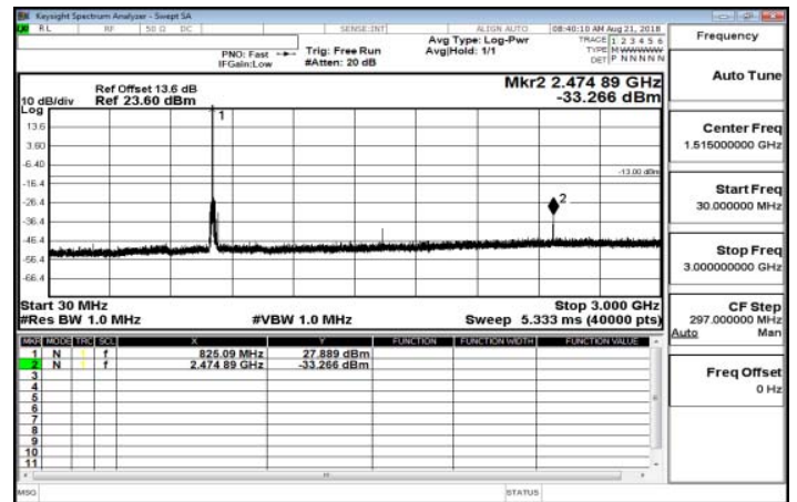
30MHz-3GHz_Band26_15MHz_QPSK_1_0_LowCH26865
