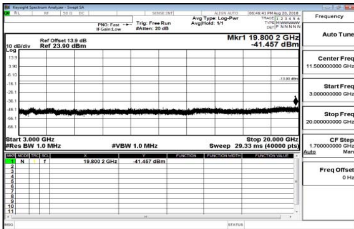
3GHz-20GHz_Band25_5MHz_QPSK_1_0_HighCH26665-1912.5
