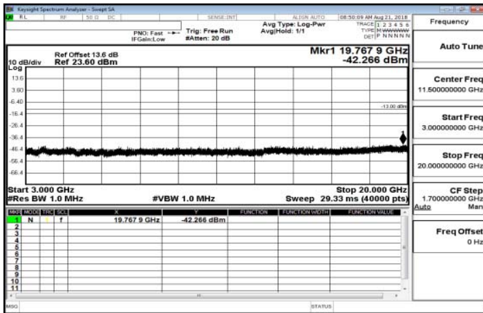
3GHz-20GHz_Band26_5MHz_QPSK_1_0_LowCH26815
