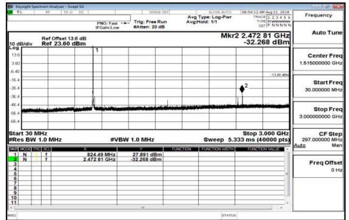
30MHz-3GHz_Band26_3MHz_QPSK_1_0_LowCH26805
