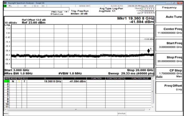
3GHz-20GHz_Band12_1_4MHz_QPSK_1_0_MidCH23095-707.5
