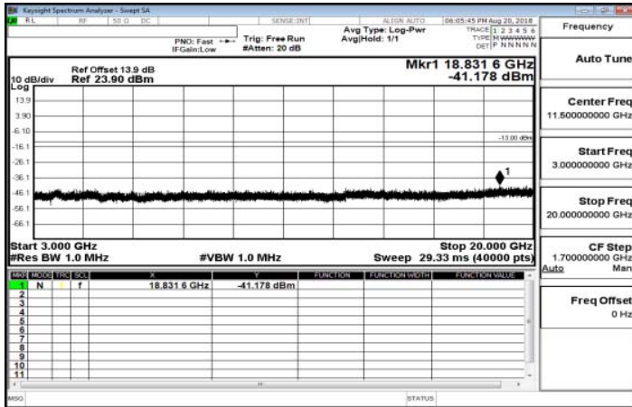
3GHz-20GHz_Band25_10MHz_QPSK_1_0_MidCH26365-1882.5
