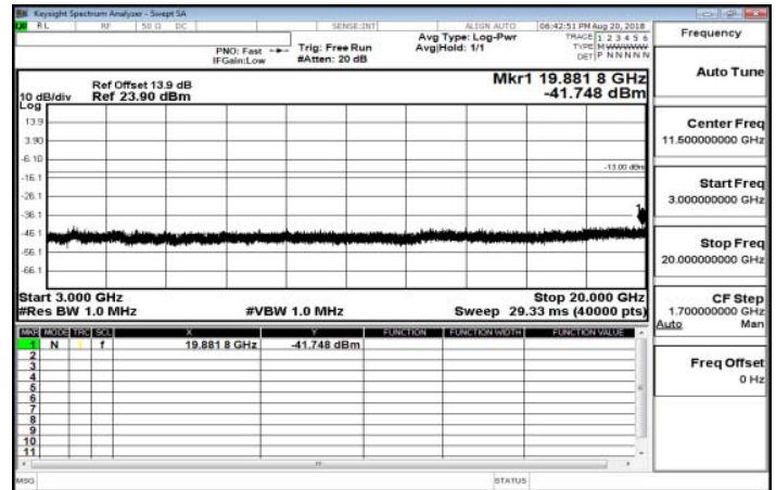
3GHz-20GHz_Band25_5MHz_QPSK_1_0_LowCH26065-1852.5
