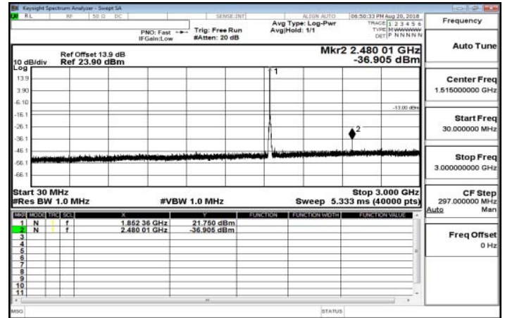
30MHz-3GHz_Band25_3MHz_OPSK_1_0_LowCH26055-1851.5
