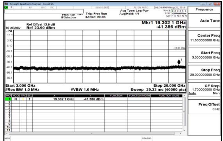
3GHz-20GHz_Band25_10MHz_QPSK_1_0_LowCH26090-1855
