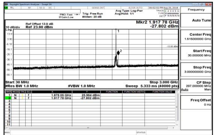
30MHz-3GHz_Band25_15MHz_QPSK_1_0_MidCH26365-1882.5
