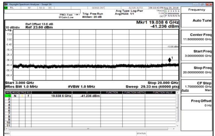
3GHz-20GHz_Band12_1_4MHz_QPSK_1_0_HighCH23173-715.3
