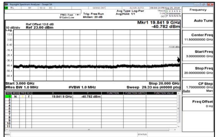
3GHz-20GHz_Band12_5MHz_QPSK_1_0_HighCH23155-713.5
