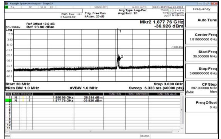
30MHz-3GHz_Band25_15MHz_QPSK_1_0_LowCH26115-1857.5
