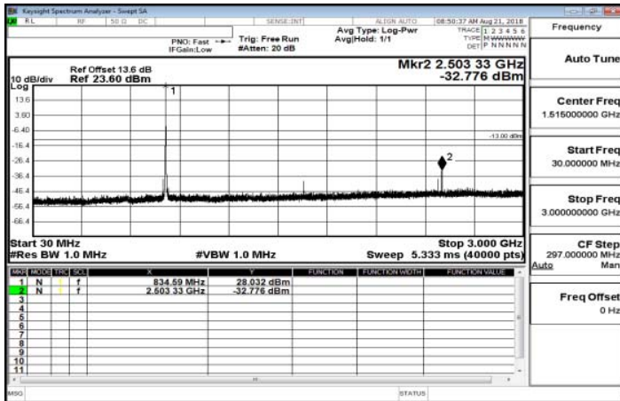
30MHz-3GHz_Band26_5MHz_QPSK_1_0_MidCH26915
