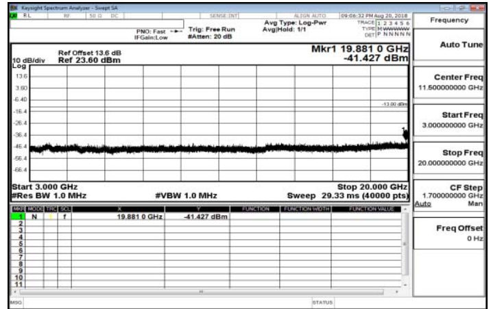
3GHz-20GHz_Band12_3MHz_QPSK_1_0_MidCH23095-707.5
