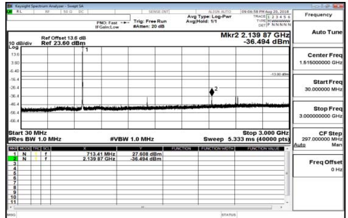
30MHz-3GHz_Band12_3MHz_QPSK_1_0_HighCH23165-714.5
