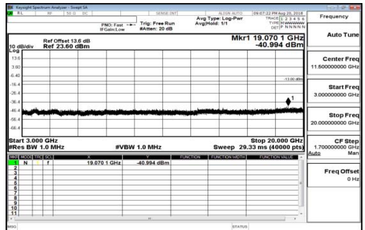
3GHz-20GHz_Band12_3MHz_QPSK_1_0_HighCH23165-714.5
