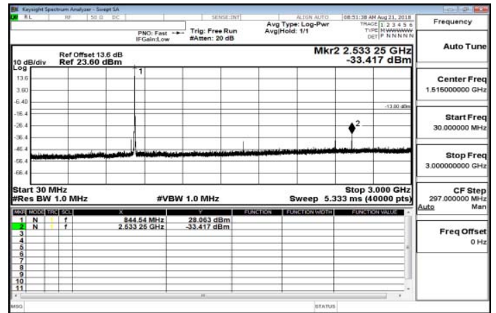
30MHz-3GHz_Band26_5MHz_QPSK_1_0_HighCH27015
