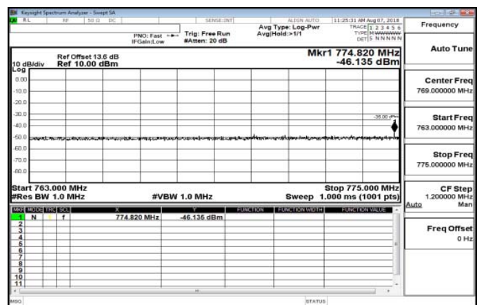
763.3MHz~775MHz_Band13_5MHz_QPSK_1_0_HighCH23255-784.5
