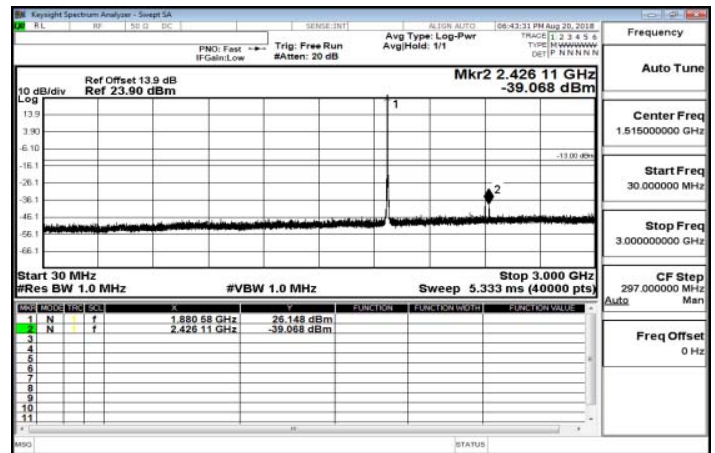
30MHz-3GHz_Band25_5MHz_QPSK_1_0_MidCH26365-1882.5
