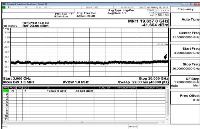
3GHz-20GHz_Band25_3MHz_QPSK_1_0_HighCH26675-1913.5
