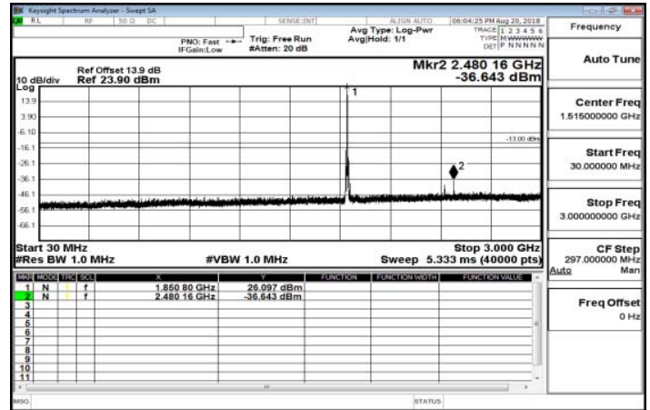
30MHz-3GHz_Band25_10MHz_QPSK_1_0_LowCH26090-1855
