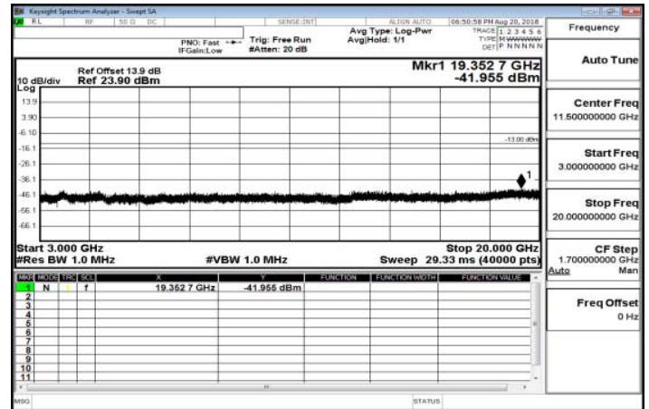
3GHz-20GHz_Band25_3MHz_OPSK_1_0_LowCH26055-1851.5
