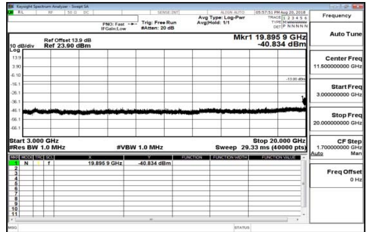
3GHz~20GHz_Band25_20MHz_QPSK_1_0_LowCH26140-1860
