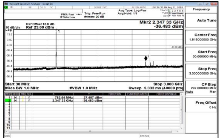
30MHz-3GHz_Band13_5MHz_QPSK_1_0_HighCH23255-784.5
