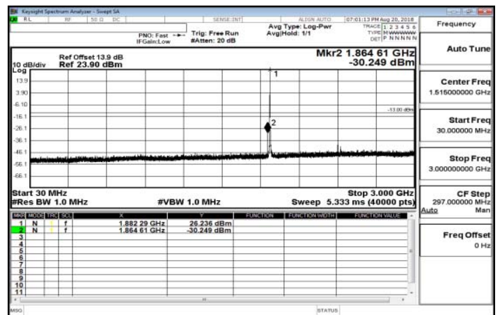
30MHz~3GHz_Band25_1_4MHz_QPSK_1_0_MidCH26365-1882.5
