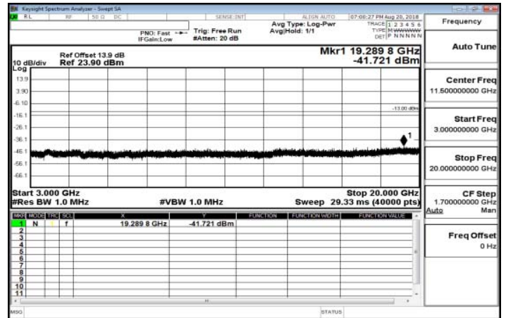
3GHz~20GHz_Band25_1_4MHz_QPSK_1_0_LowCH26047-1850.7
