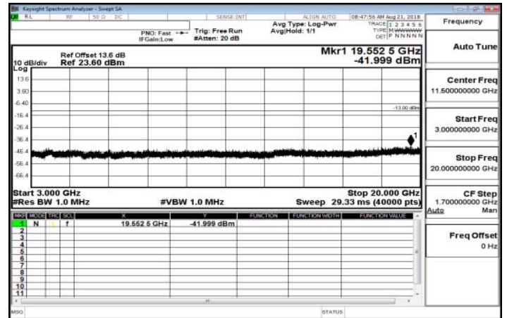
3GHz-20GHz_Band26_10MHz_QPSK_1_0_HighCH26990
