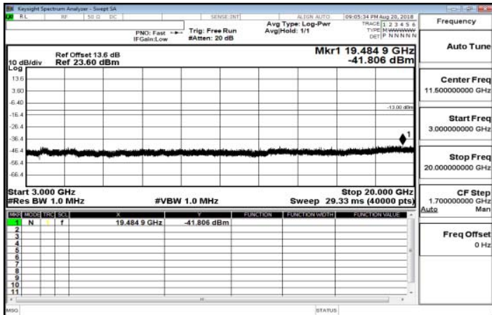
3GHz-20GHz_Band12_3MHz_QPSK_1_0_LowCH23025-700.5
