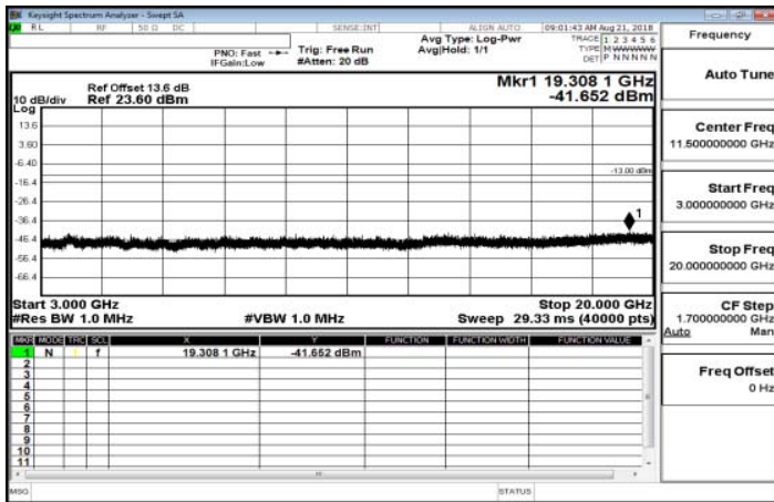
3GHz-20GHz_Band26_1_4MHz_QPSK_1_0_MidCH26915
