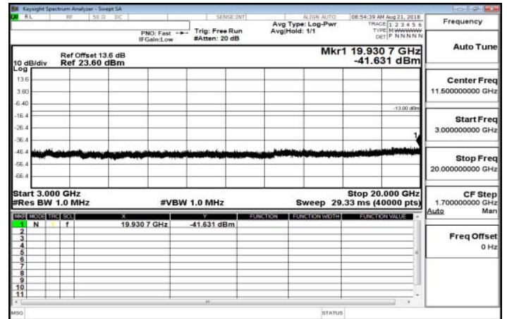
3GHz-20GHz_Band26_3MHz_QPSK_1_0_LowCH26805
