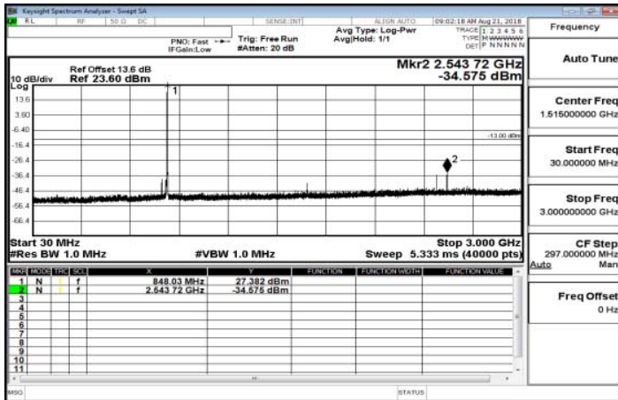
30MHz-3GHz_Band26_1_4MHz_QPSK_1_0_HighCH27033
