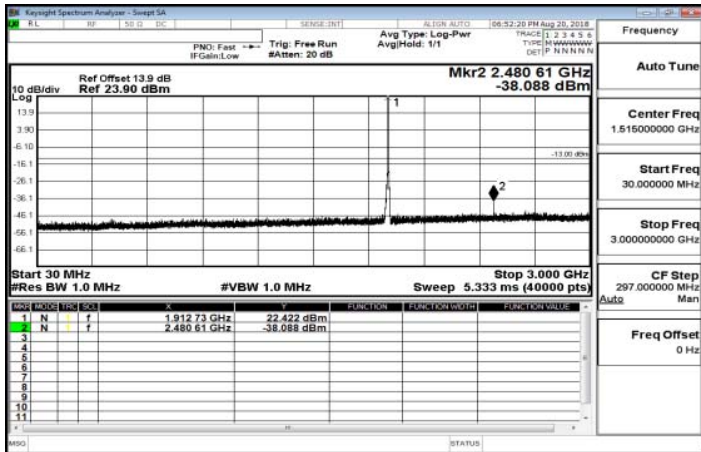
30MHz-3GHz_Band25_3MHz_QPSK_1_0_HighCH26675-1913.5
