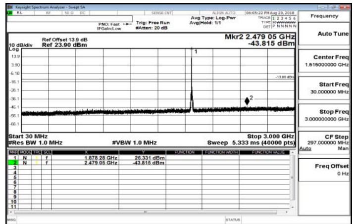
30MHz-3GHz_Band25_10MHz_QPSK_1_0_MidCH26365-1882.5
