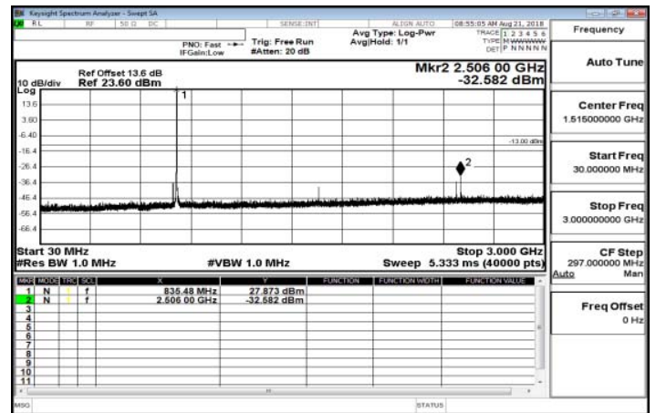
30MHz-3GHz_Band26_3MHz_QPSK_1_0_MidCH26915
