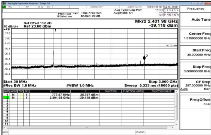
30MHz-3GHz_Band13_5MHz_QPSK_1_0_LowCH23205-779.5
