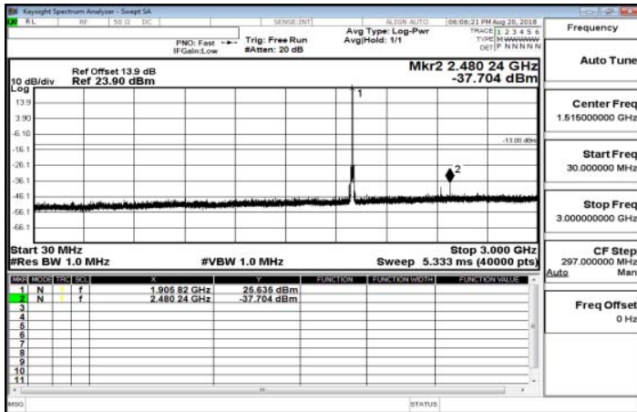
30MHz-3GHz_Band25_10MHz_QPSK_1_0_HighCH26640-1910
