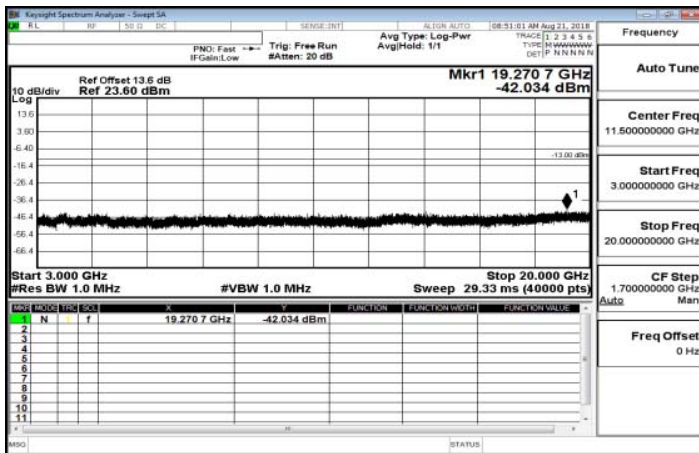
3GHz-20GHz_Band26_5MHz_QPSK_1_0_MidCH26915
