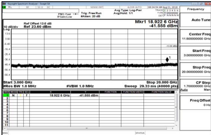
3GHz-20GHz_Band13_5MHz_QPSK_1_0_LowCH23205-779.5
