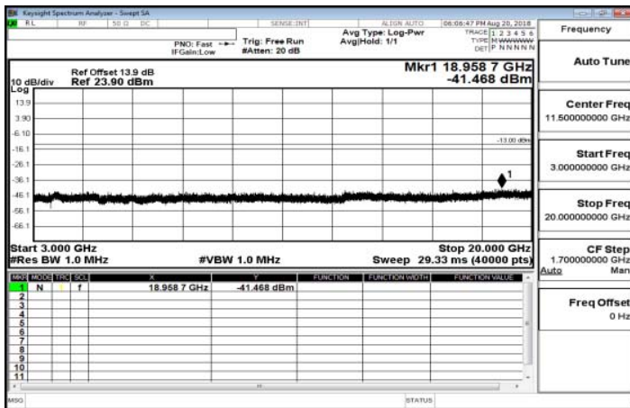
3GHz-20GHz_Band25_10MHz_QPSK_1_0_HighCH26640-1910
