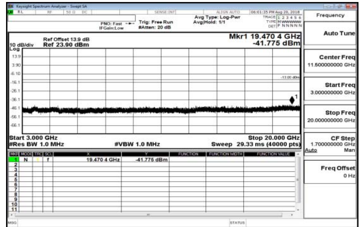
3GHz-20GHz_Band25_15MHz_QPSK_1_0_LowCH26115-1857.5
