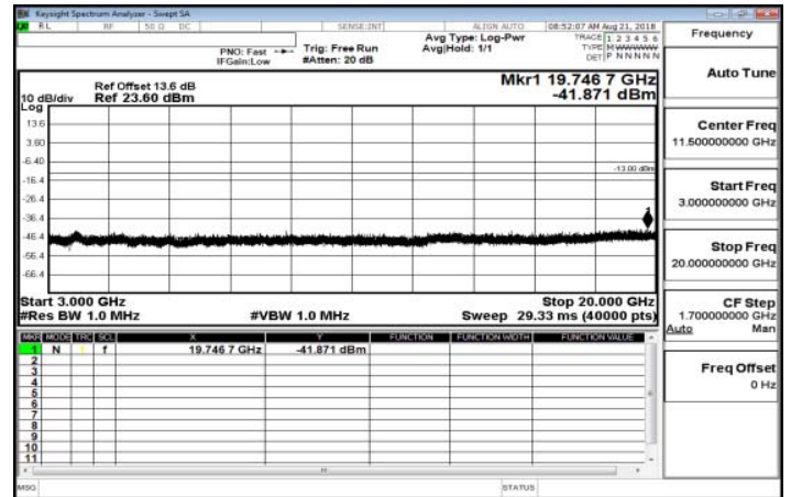
3GHz-20GHz_Band26_5MHz_QPSK_1_0_HighCH27015
