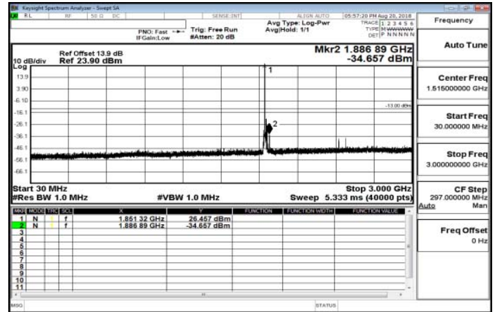
30MHz~3GHz_Band25_20MHz_QPSK_1_0_LowCH26140-1860
