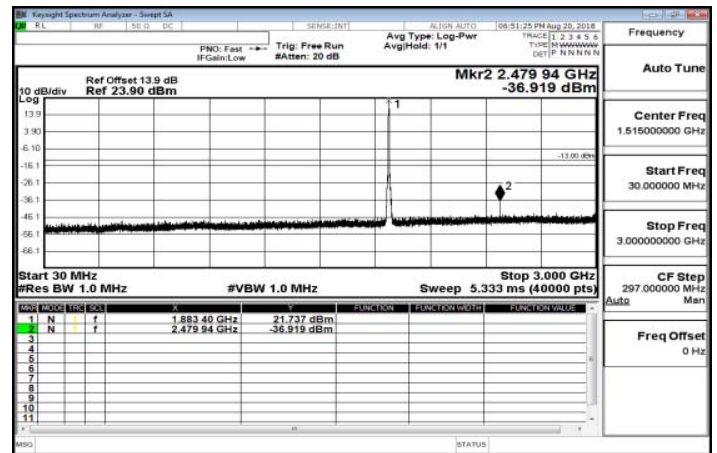
30MHz-3GHz_Band25_3MHz_OPSK_1_0_MidCH26365-1882.5
