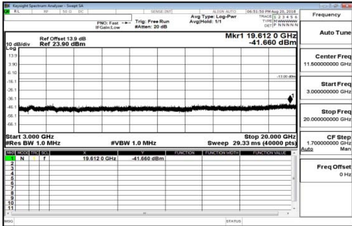
3GHz-20GHz_Band25_3MHz_QPSK_1_0_MidCH26365-1882.5
