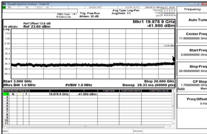
3GHz-20GHz_Band26_10MHz_QPSK_1_0_LowCH26840
