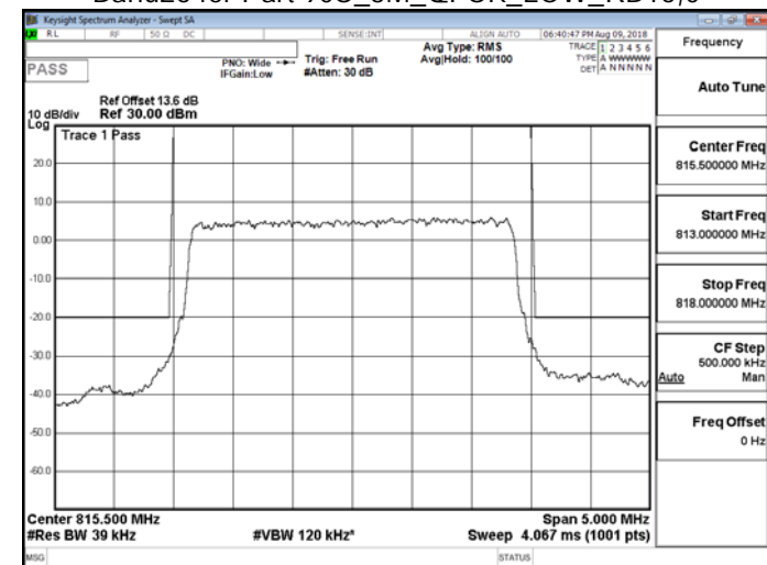
Band26 for Part 90S_3M_QPSK_LOW_RB15,0
