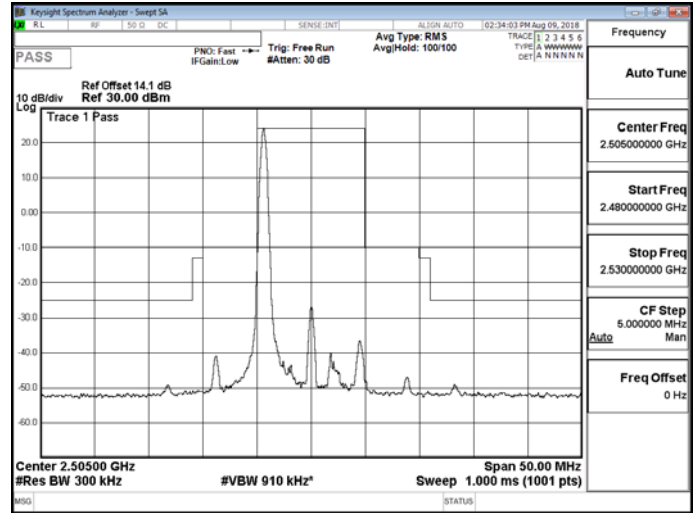
Band 7_10M_QPSK_LOW_RB1,49
