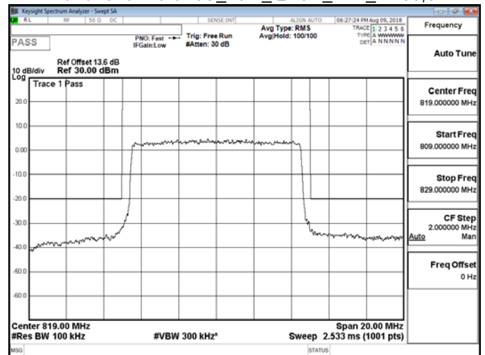
Band26 for Part 90S_10M_QPSK_MID_RB50,0
