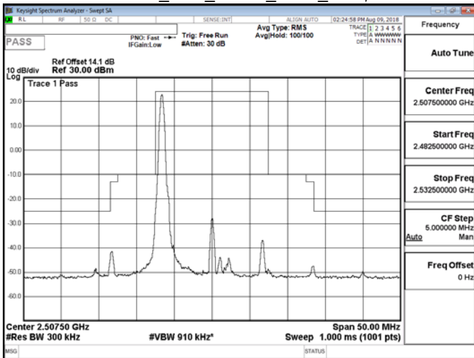
Band 7_15M_QPSK_LOW_RB1,74
