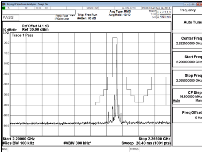
Band 30_5M_QPSK_LOW_RB25,0
