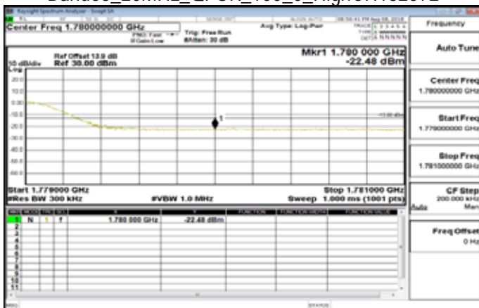
Band66_20MHz_QPSK_100_0_HighCH132572
