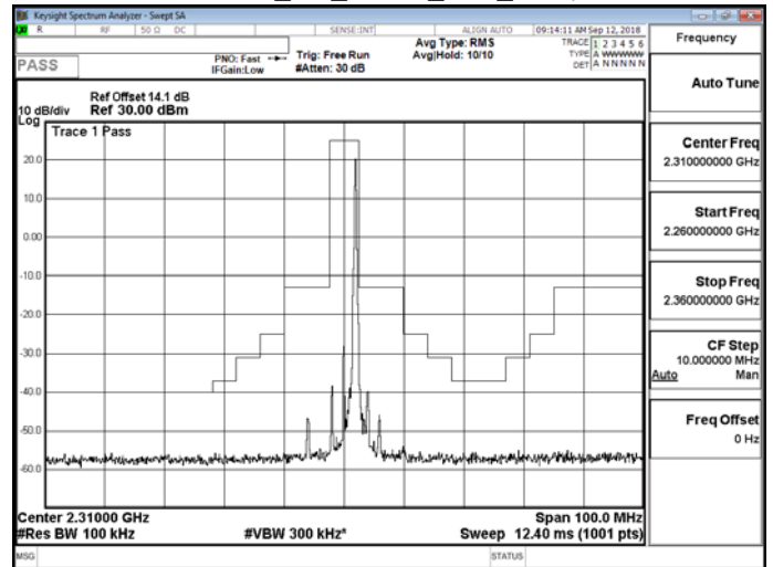
Band 30_5M_QPSK_MID_RB25,0
