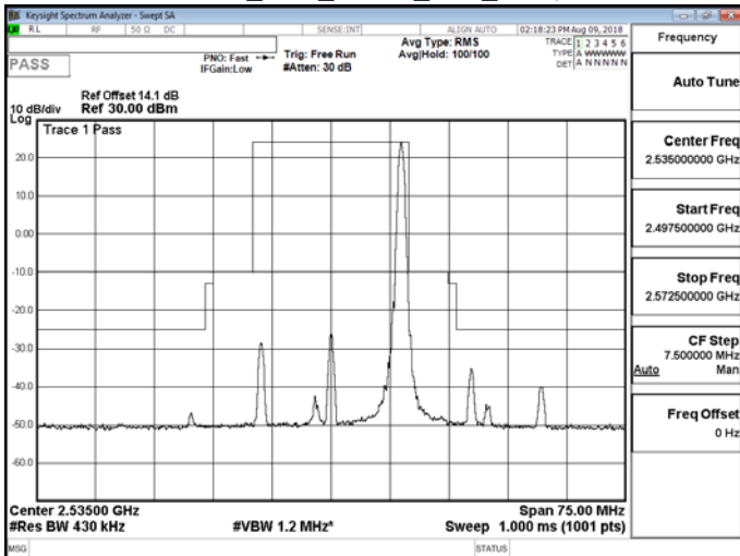
Band 7_20M_QPSK_MID_RB100,0
