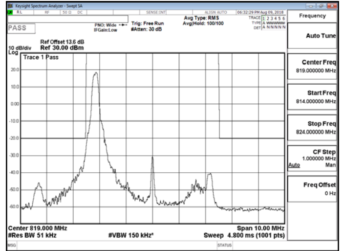
Band26 for Part 90S_5M_QPSK_MID_RB1,24
