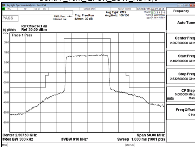
Band 7_15M_QPSK_LOW_RB75,0
