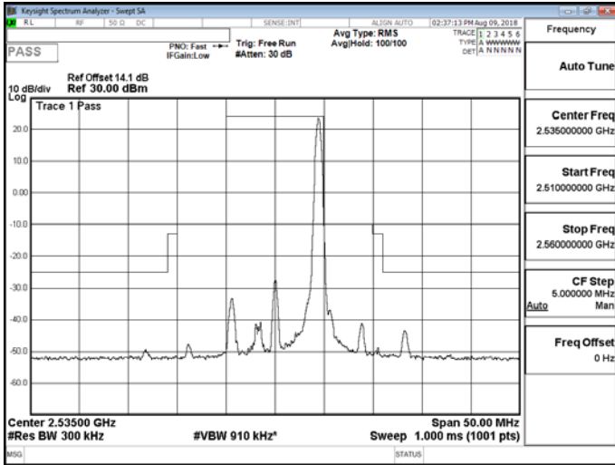
Band 7_10M_QPSK_MID_RB50,0
