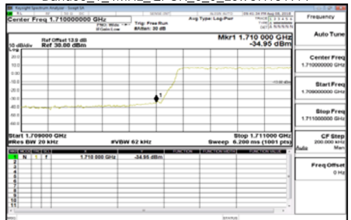
Band66_1_4MHz_QPSK_6_0_LowCH131979
