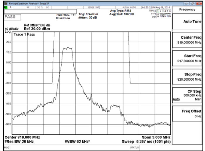
Band26 for Part 90S_1.4M_OPK_MID_RB1,5
