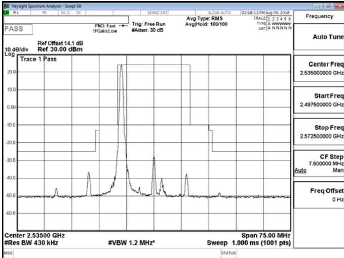
Band 7_20M_QPSK_MID_RB1,99
