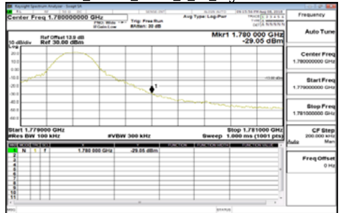
Band66_10MHz_QPSK_1_49_HighCH132622
