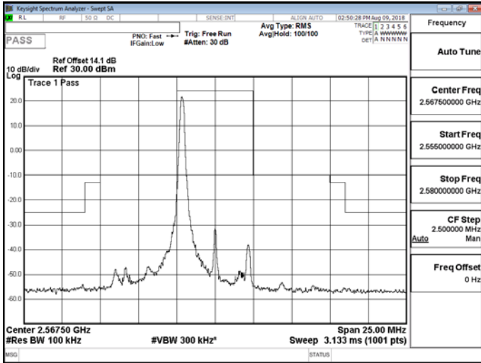
Band 7_5M_QPSK_HIGH_RB1,24
