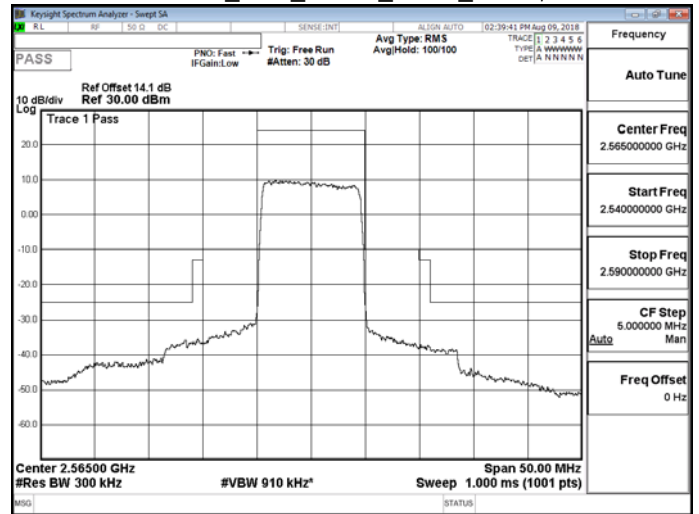
Band 7_10M_QPSK_HIGH_RB50,0
