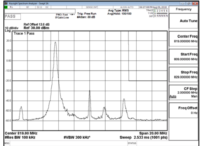
Band26 for Part 90S_10M_QPSK_MID_RB1,49
