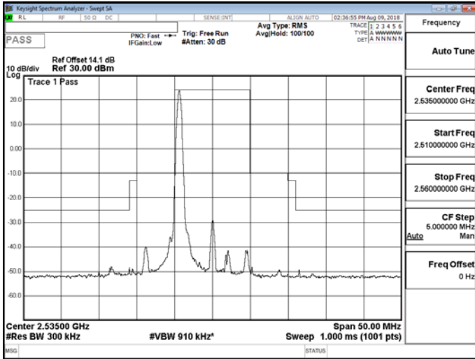
Band 7_10M_QPSK_MID_RB1,49
