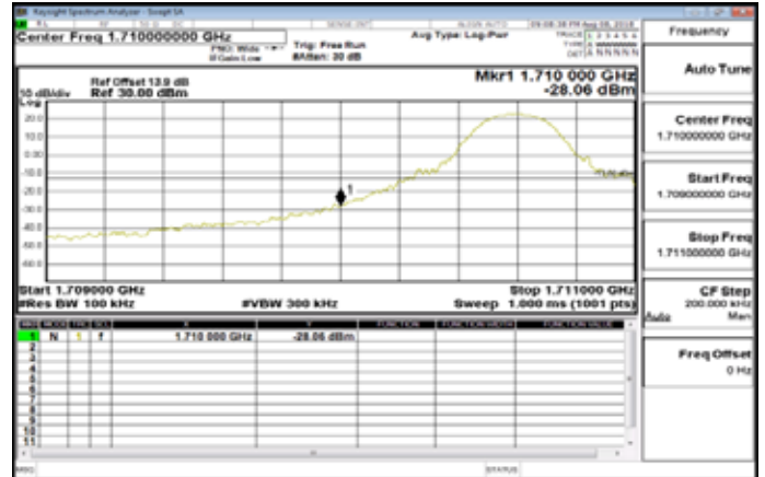
Band66_10MHz_QPSK_1_0_LowCH132022
