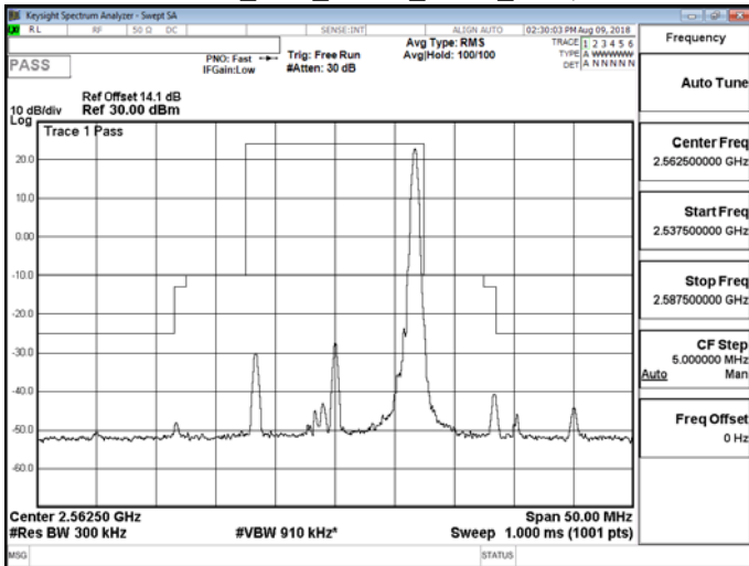
Band 7_15M_QPSK_HIGH_RB75,0
