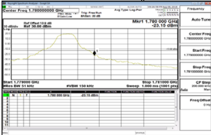
Band66_5MHz_QPSK_1_24_HighCH132647
