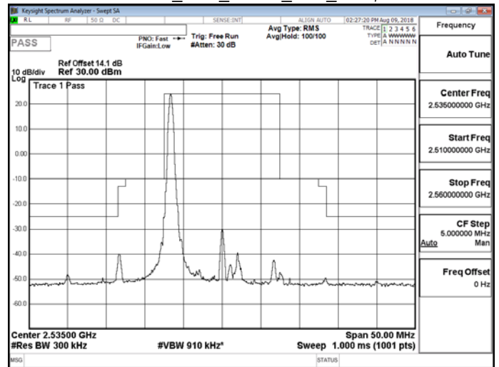
Band 7_15M_QPSK_MID_RB1,74
