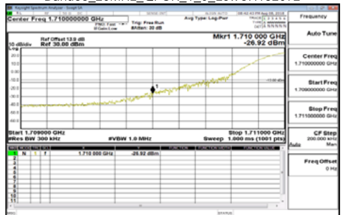
Band66_20MHz_QPSK_1_0_LowCH132072
