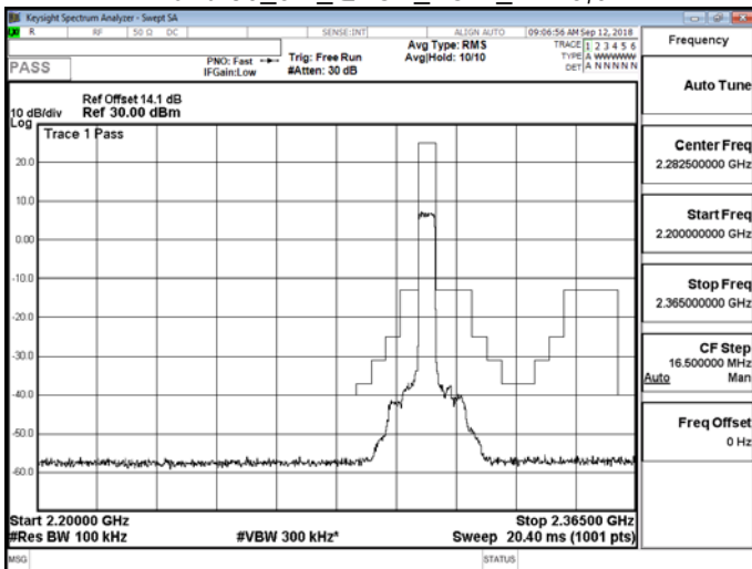
Band 30_5M_QPSK_LOW_RB25,0
