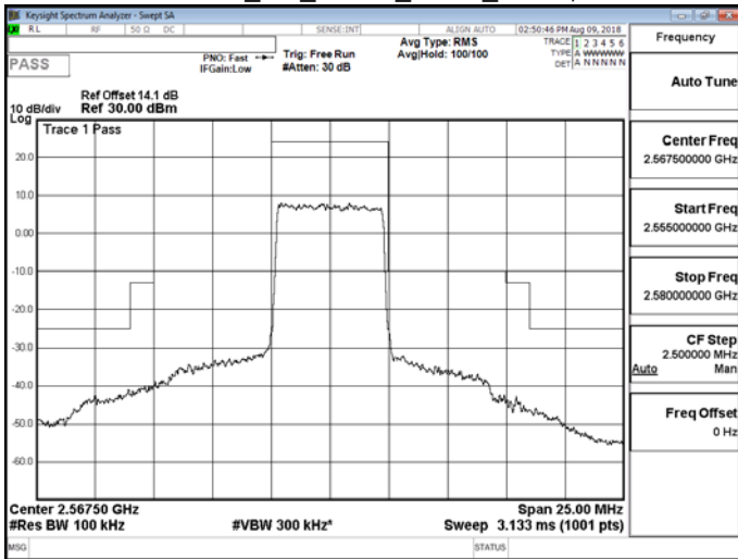
Band 7_5M_QPSK_HIGH_RB25,0
