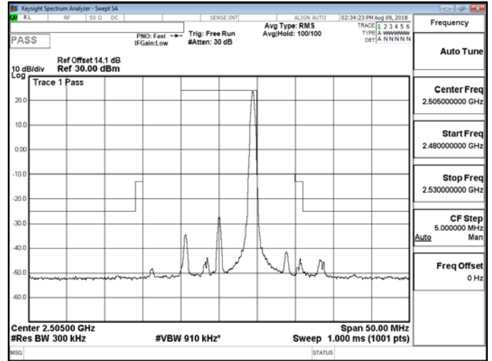
Band 7_10M_QPSK_LOW_RB50,0
