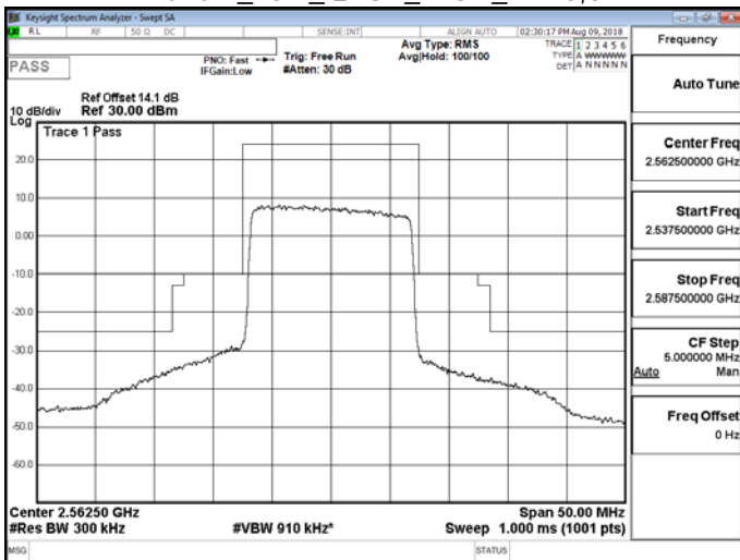
Band 7_15M_QPSK_HIGH_RB75,0
