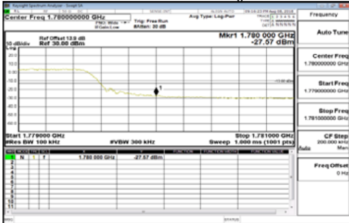
Band66_10MHz_QPSK_50_0_HighCH132622
