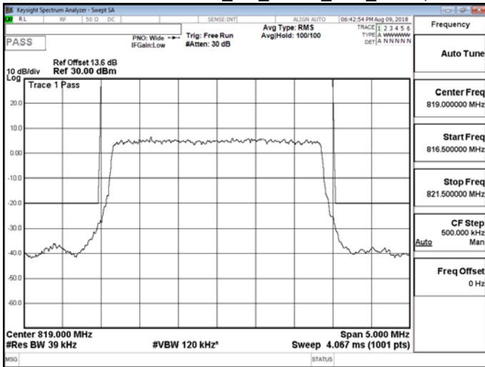
Band26 for Part 90S_3M_QPSK_MID_RB15,0
