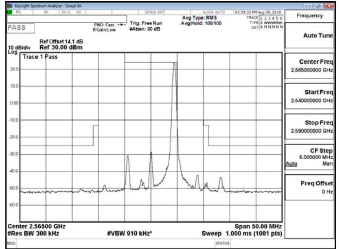
Band 7_10M_QPSK_HIGH_RB50,0
