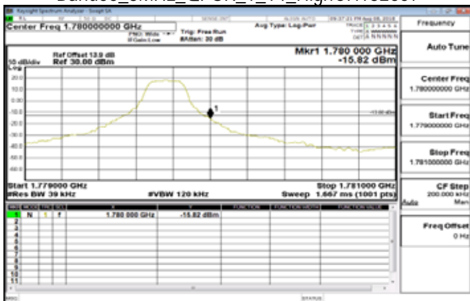
Band66_3MHz_QPSK_1_14_HighCH132657
