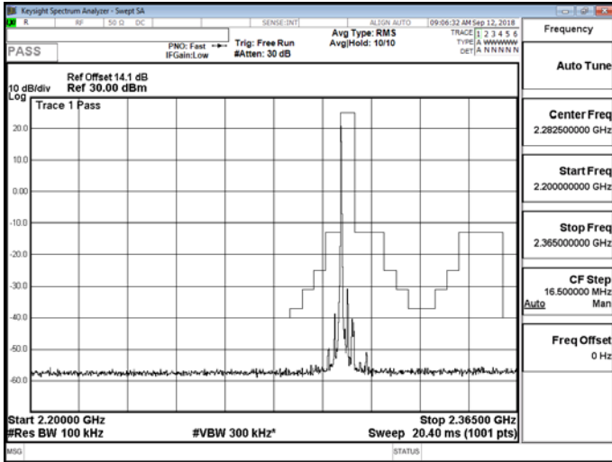
Band 30_5M_QPSK_LOW_RB1,24
