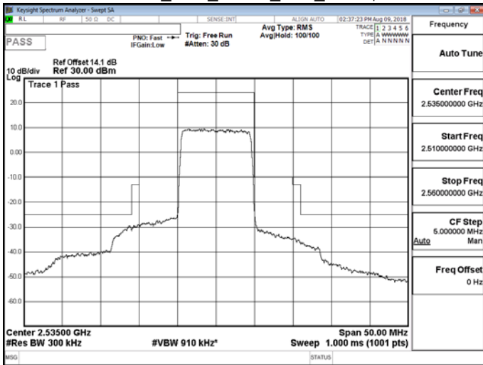
Band 7_10M_QPSK_MID_RB50,0
