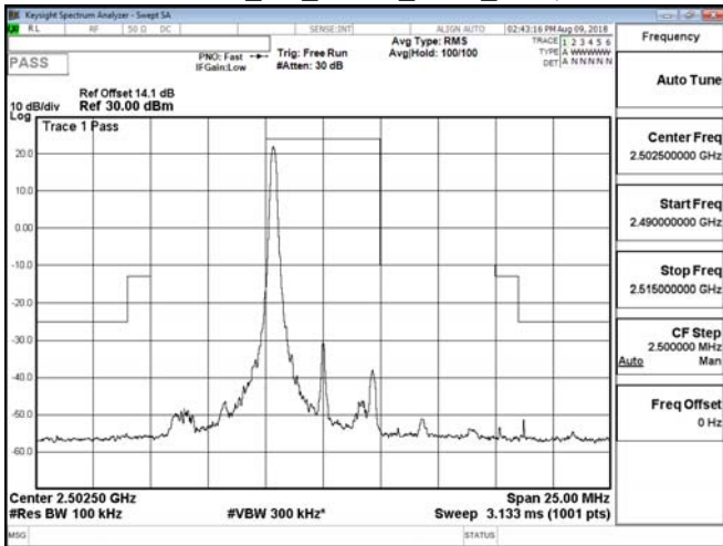
Band 7_5M_QPSK_LOW_RB1,24
