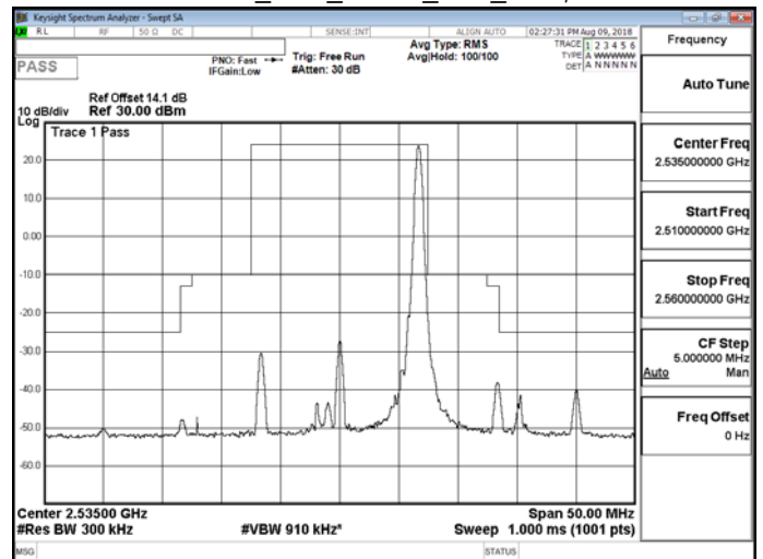
Band 7_15M_QPSK_MID_RB75,0
