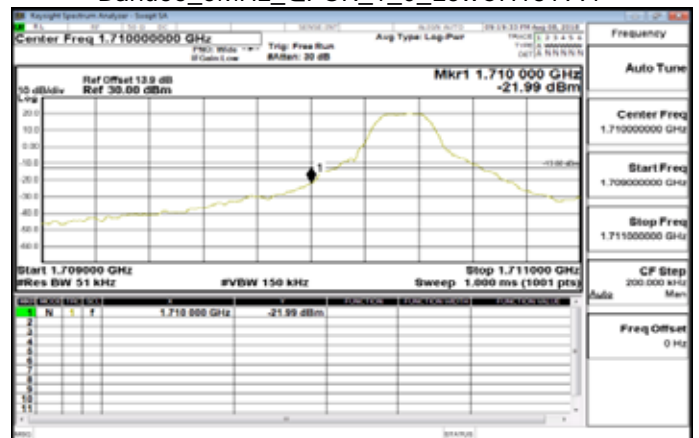
Band66_5MHz_QPSK_1_0_LowCH131997
