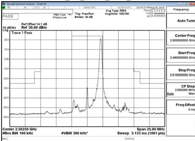
Band 7_5M_QPSK_LOW_RB25,0
