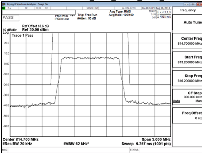
Band26 for Part 90S_1.4M_OPK_LOW_RB6.0
