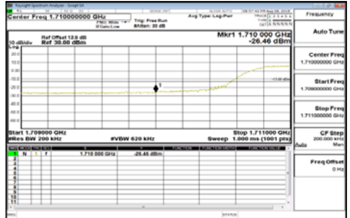
Band66_15MHz_QPSK_75_0_LowCH132047
