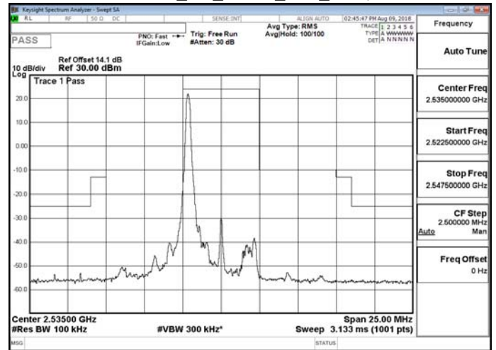
Band 7_5M_QPSK_MID_RB1,24
