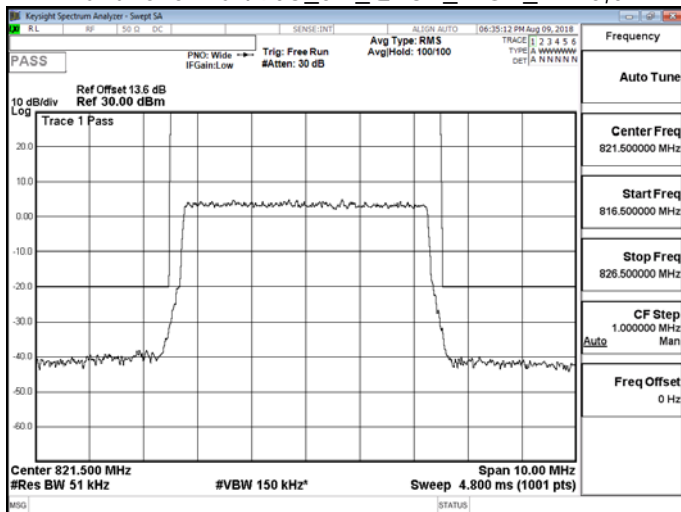
Band26 for Part 90S_5M_QPSK_HIGH_RB25,0
