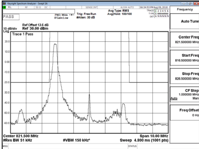
Band26 for Part 90S_5M_QPSK_HIGH_RB1,24
