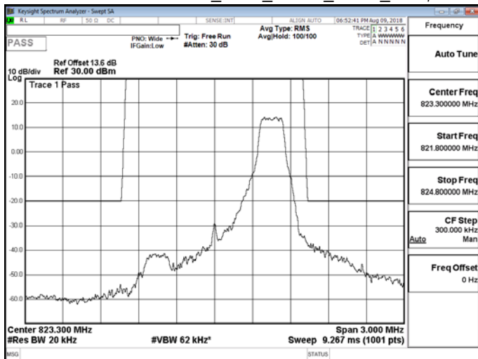
Band26 for Part 90S_1.4M_QPSK_HIGH_RB6,0
