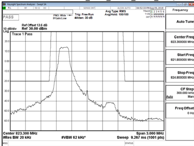
Band26 for Part 90S_1.4M_QPSK_HIGH_RB1,5
