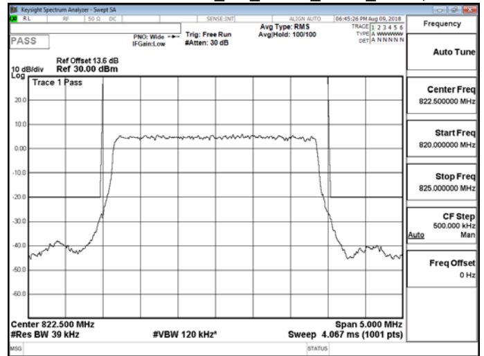
Band26 for Part 90S_3M_QPSK_HIGH_RB15,0
