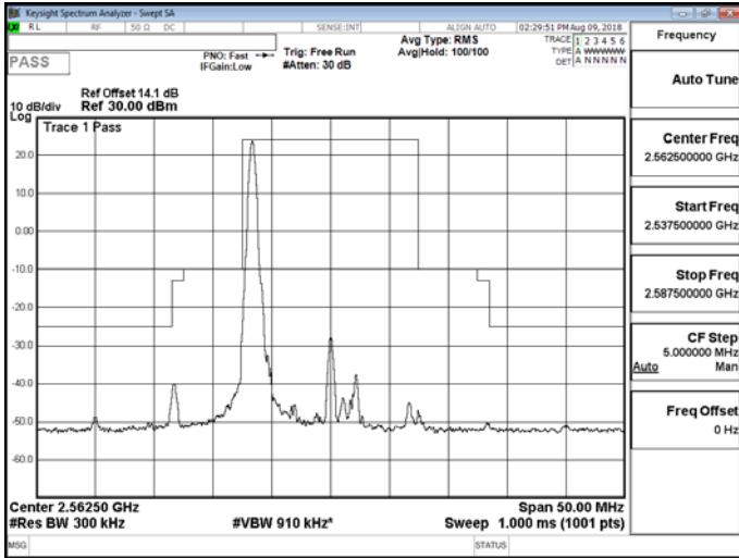
Band 7_15M_QPSK_HIGH_RB1,74
