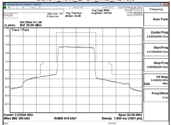
Band 7_15M_QPSK_MID_RB75,0
