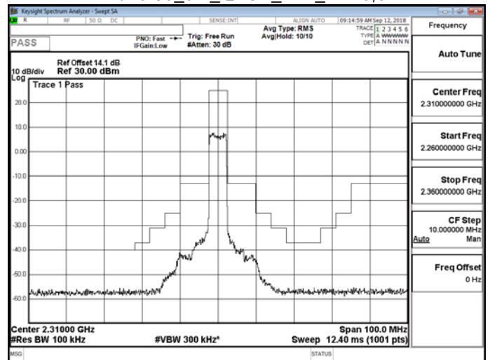
Band 30_5M_QPSK_MID_RB25,0
