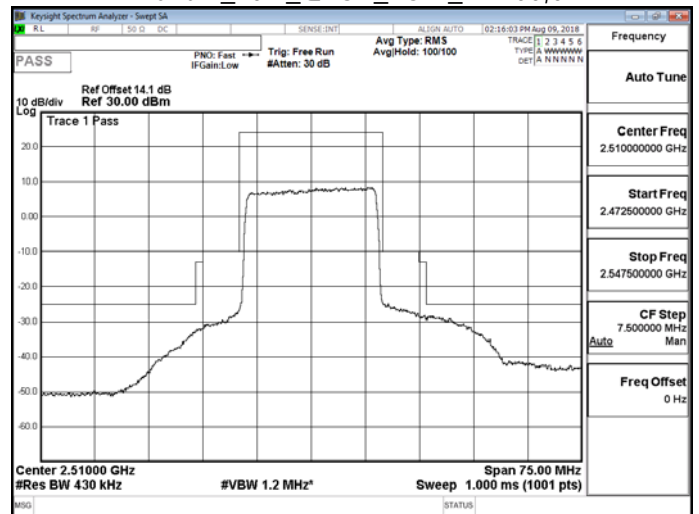
Band 7_20M_QPSK_LOW_RB100,0
