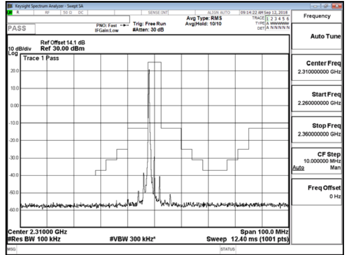
Band 30_5M_QPSK_MID_RB1,24
