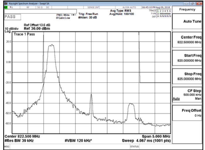
Band26 for Part 90S_3M_QPSK_HIGH_RB1,14
