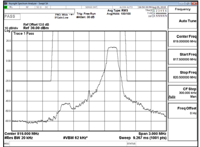
Band26 for Part 90S_1.4M_OPK_MID_RB6.0
