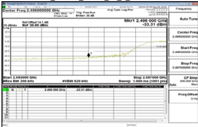
Band41_15MHz_QPSK_75_0_LowCH39725
