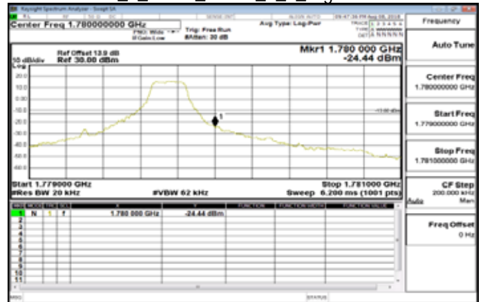
Band66_1_4MHz_QPSK_1_5_HighCH132665
