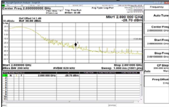
Band41_15MHz_QPSK_1_74_HighCH41515
