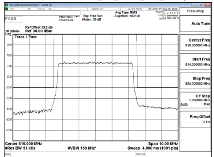
Band26 for Part 90S_5M_QPSK_MID_RB25,0
