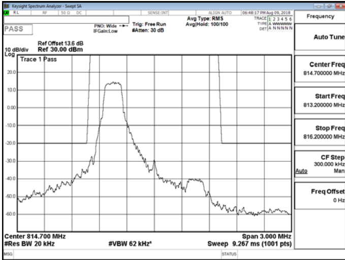
Band26 for Part 90S_1.4M_OPK_LOW_RB1,5
