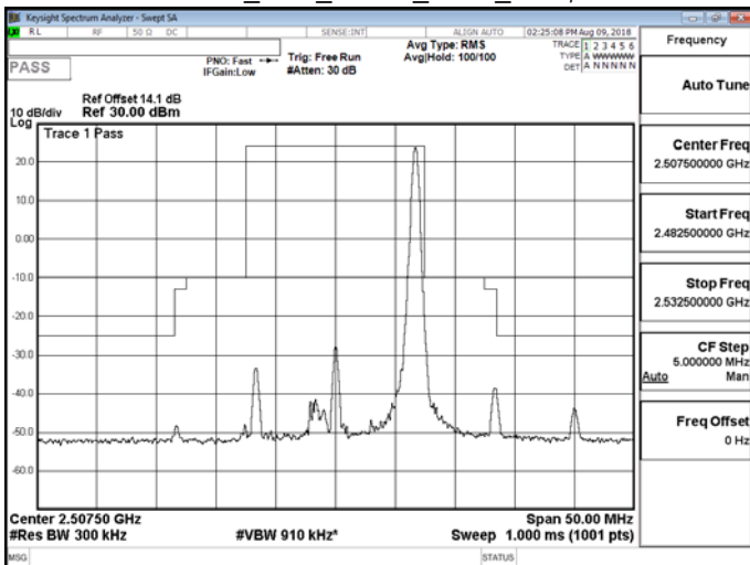
Band 7_15M_QPSK_LOW_RB75,0
