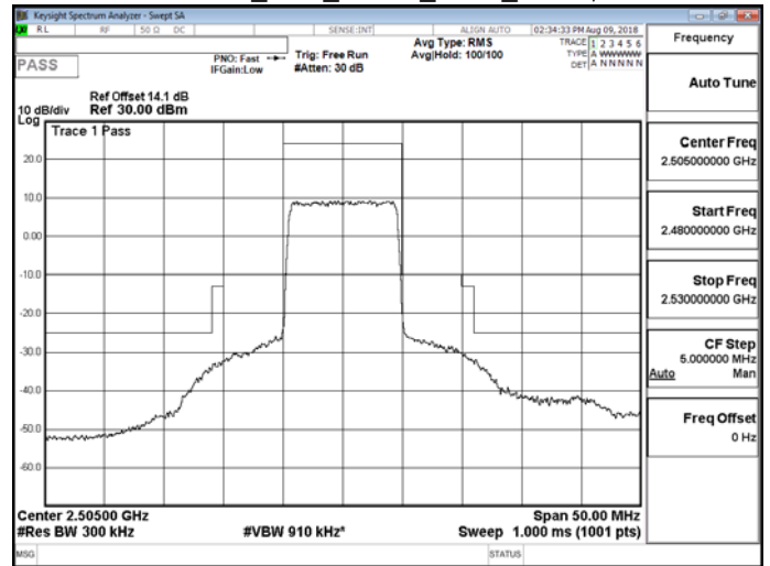
Band 7_10M_QPSK_LOW_RB50,0
