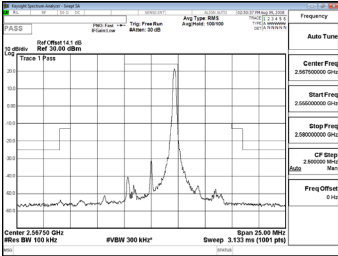
Band 7_5M_QPSK_HIGH_RB25,0
