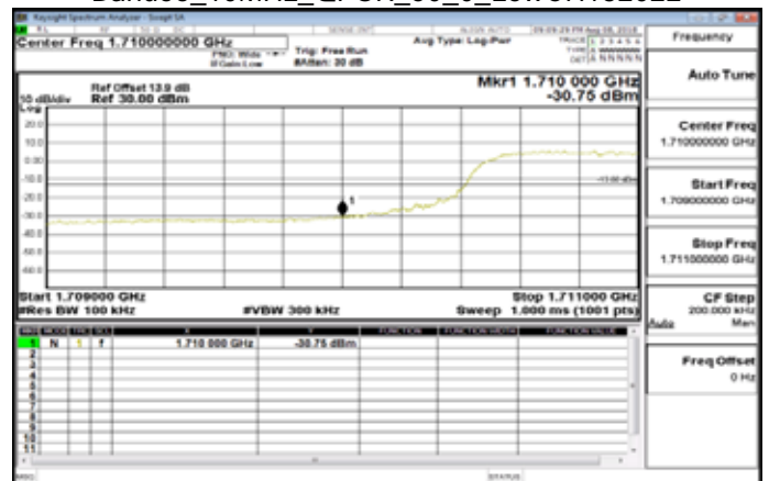
Band66_10MHz_QPSK_50_0_LowCH132022
