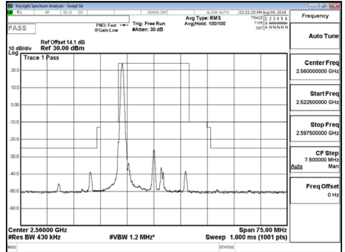
Band 7_20M_QPSK_HIGH_RB1,99
