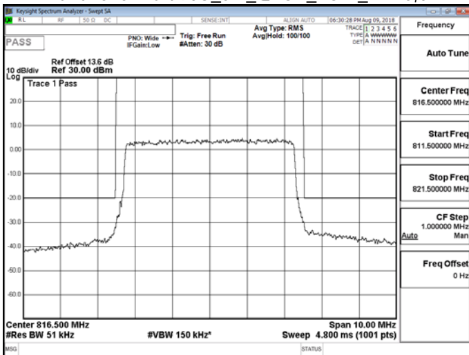
Band26 for Part 90S_5M_QPSK_LOW_RB25,0
