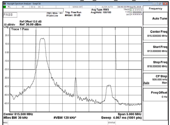
Band26 for Part 90S_3M_QPSK_LOW_RB1,14
