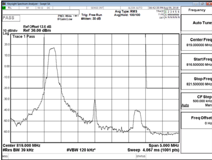
Band26 for Part 90S_3M_QPSK_MID_RB1,14
