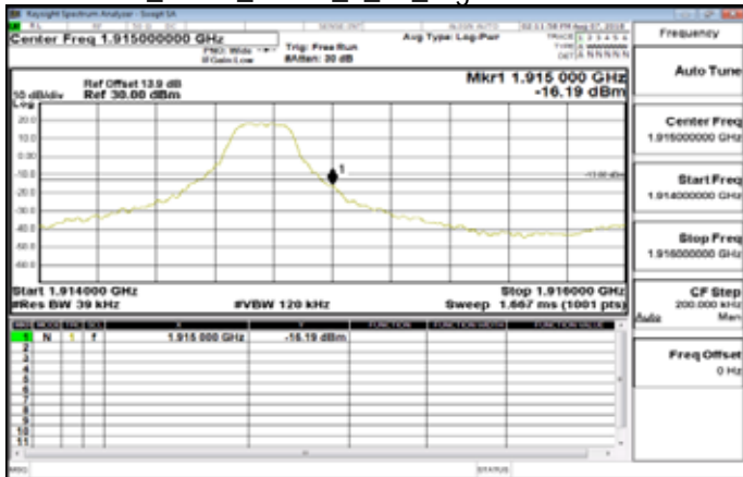
Band25_3MHz_QPSK_1_14_HighCH26675-1913.5
