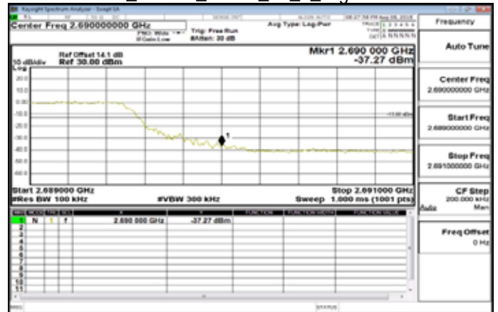
Band41_10MHz_QPSK_50_0_HighCH41540
