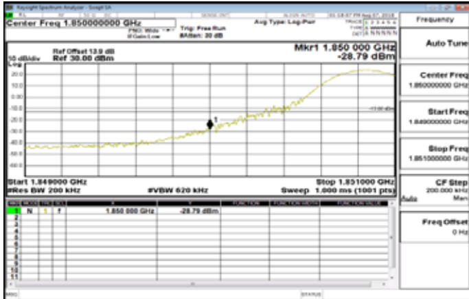
Band25_15MHz_QPSK_1_0_LowCH26115-1857.5
