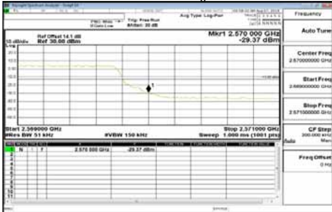
Band7_5MHz_QPSK_25_0_HighCH21425-2567.5
