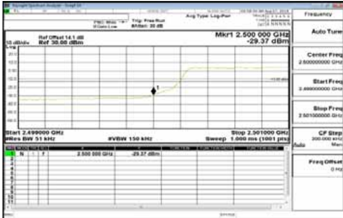
Band7_5MHz_QPSK_25_0_LowCH20775-2502.5
