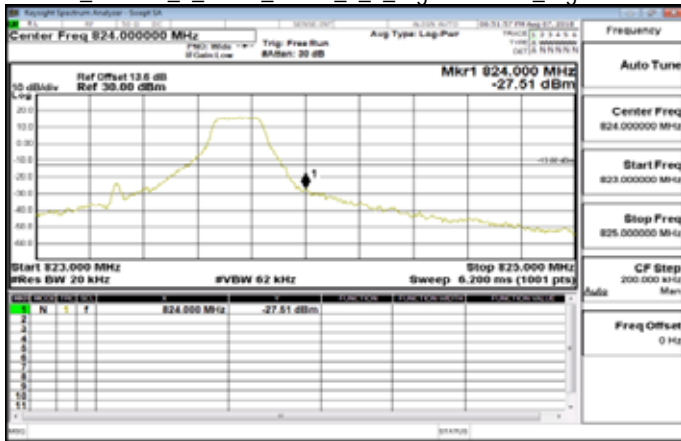
Part 90_Band26_1_4MHz_QPSK_1_5_HighCH26783_HighCH26783
