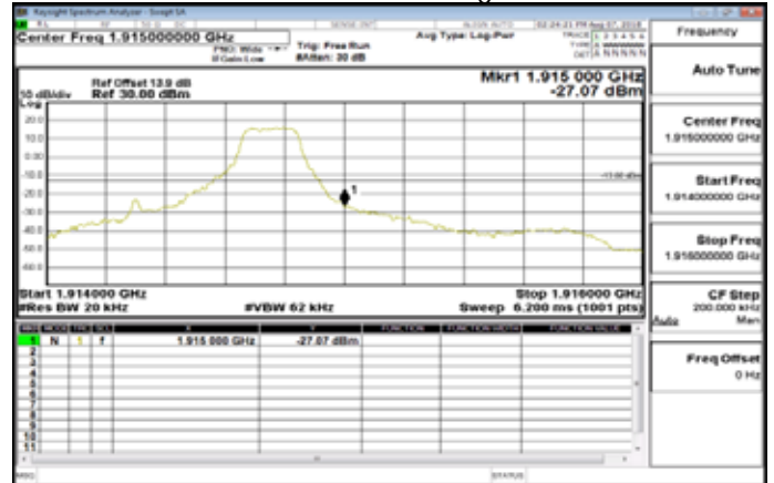
Band25_1_4MHz_QPSK_1_5_HighCH26683-1914.3
