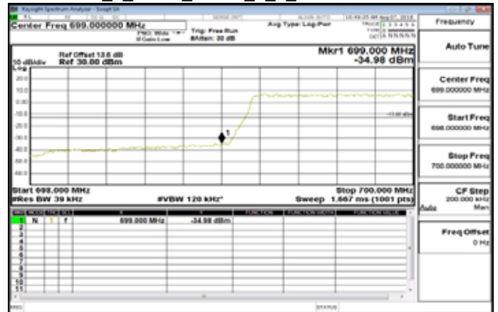
Band12_1_4MHz_QPSK_6_0_LowCH23017-699.7
