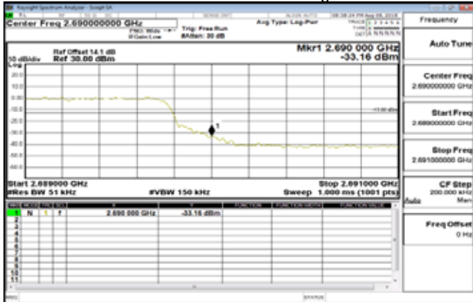
Band41_5MHz_QPSK_25_0_HighCH41565
