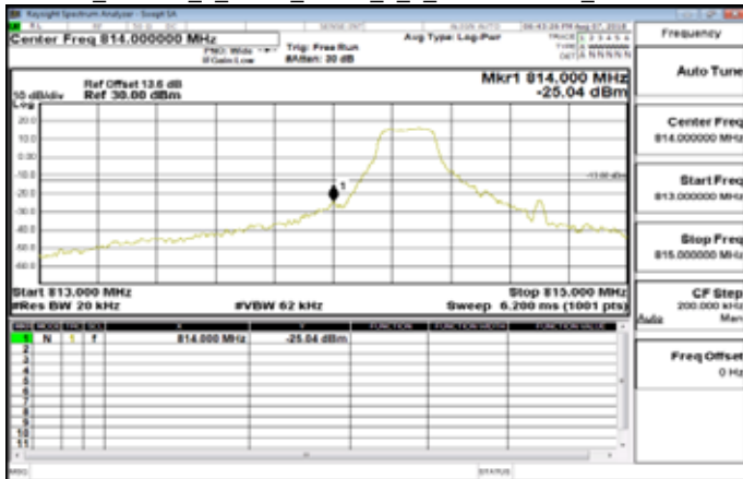
Part 90_Band26_1_4MHz_QPSK_1_0_LowCH26697_LowCH26697
