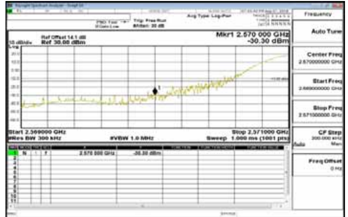
Band38_20MHz_QPSK_1_0_LowCH37850
