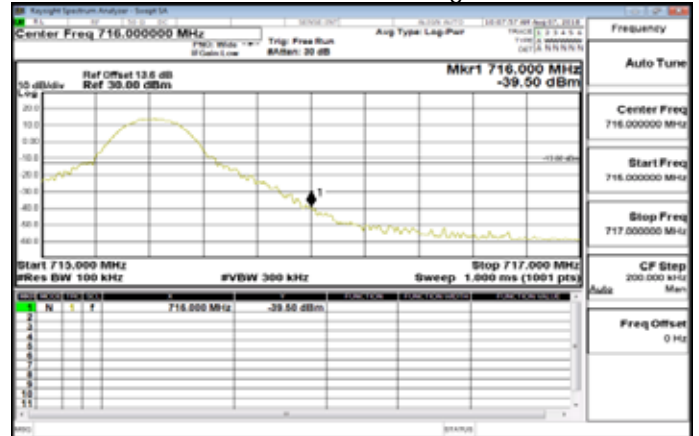
Band12_10MHz_QPSK_1_49_HighCH23130-711
