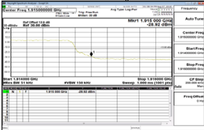
Band25_5MHz_QPSK_25_0_HighCH26665-1912.5
