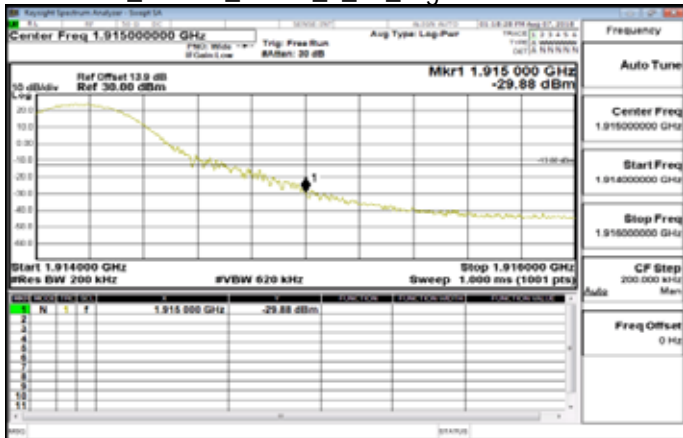
Band25_15MHz_QPSK_1_74_HighCH26615-1907.5
