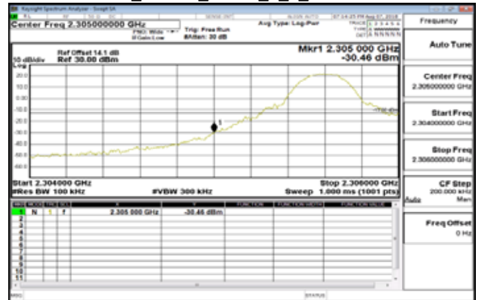
Band30_10MHz_QPSK_1_0_MidCH27710
