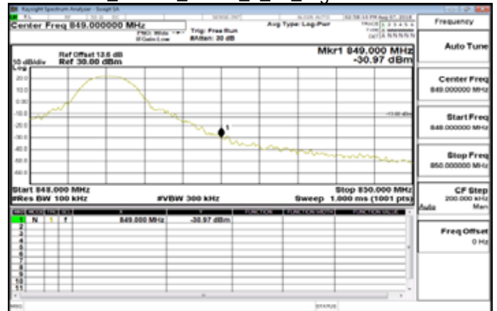
Band26_10MHz_QPSK_1_49_HighCH26990-844
