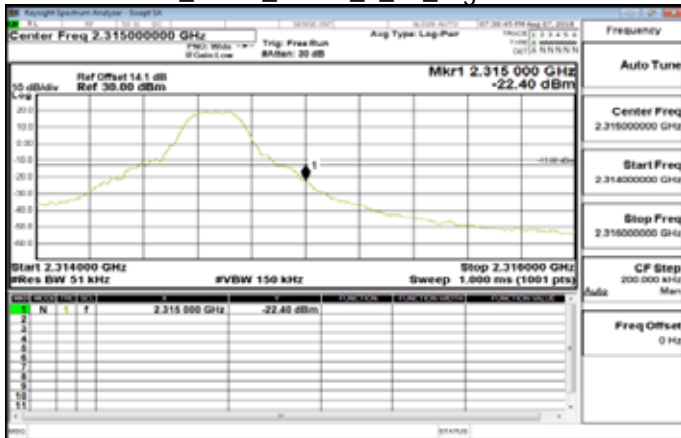
Band30_5MHz_QPSK_1_24_HighCH27735
