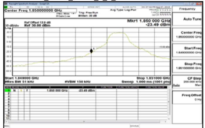
Band25_5MHz_QPSK_1_0_LowCH26065-1852.5
