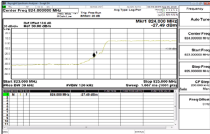
Band5_3MHz_QPSK_15_0_LowCH20415-825.5
