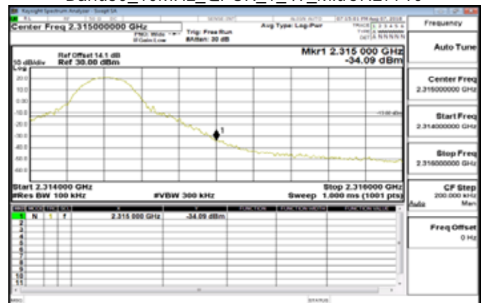
Band30_10MHz_QPSK_1_49_MidCH27710
