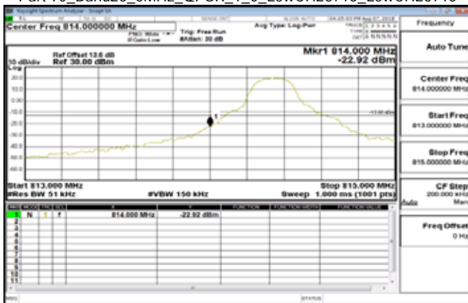
Part 90_Band26_5MHz_QPSK_1_0_LowCH26715_LowCH26715
