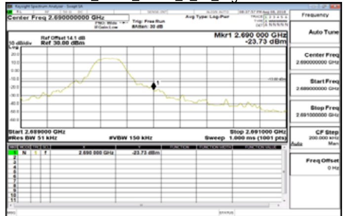
Band41_5MHz_QPSK_1_24_HighCH41565
