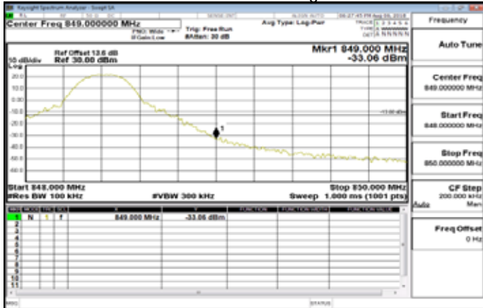
Band5_10MHz_QPSK_1_49_HighCH20600-844
