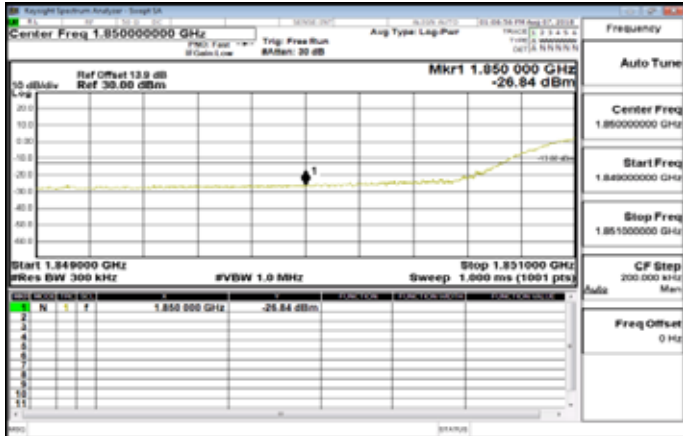
Band25_20MHz_QPSK_100_0_LowCH26140-1860
