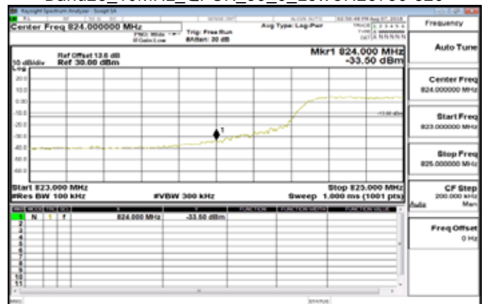
Band26_10MHz_QPSK_50_0_LowCH26750-820
