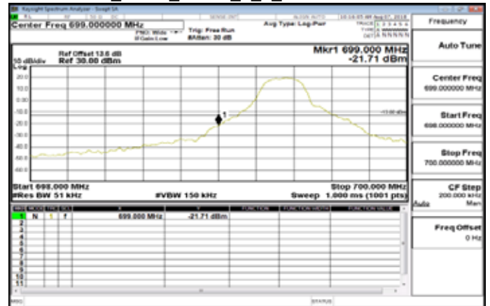
Band12_5MHz_QPSK_1_0_LowCH23035-701.5
