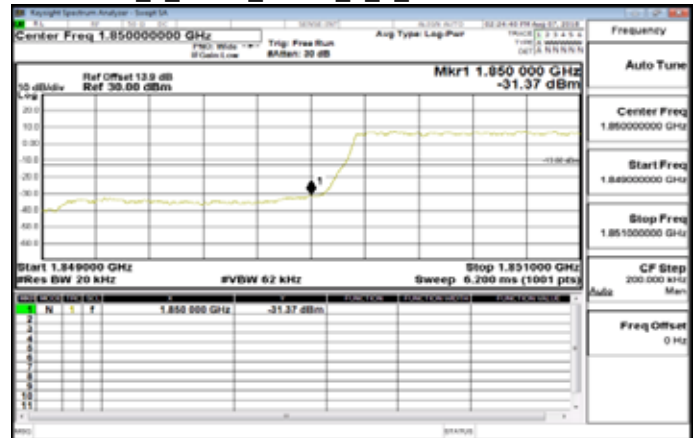
Band25_1_4MHz_QPSK_6_0_LowCH26047-1850.7
