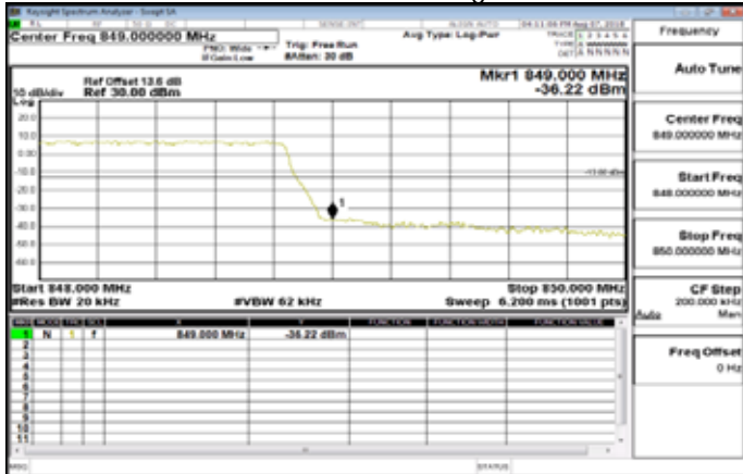
Band26_1_4MHz_QPSK_6_0_HighCH27033-848.3
