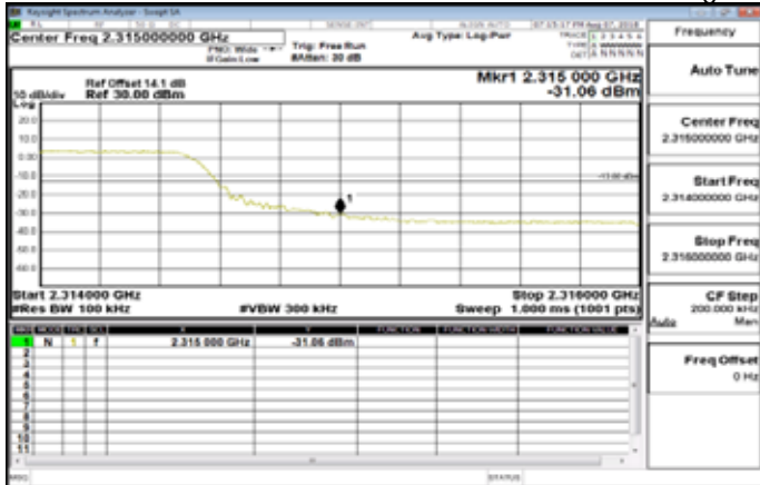
Band30_10MHz_QPSK_50_0_MidCH27710-2310 right
