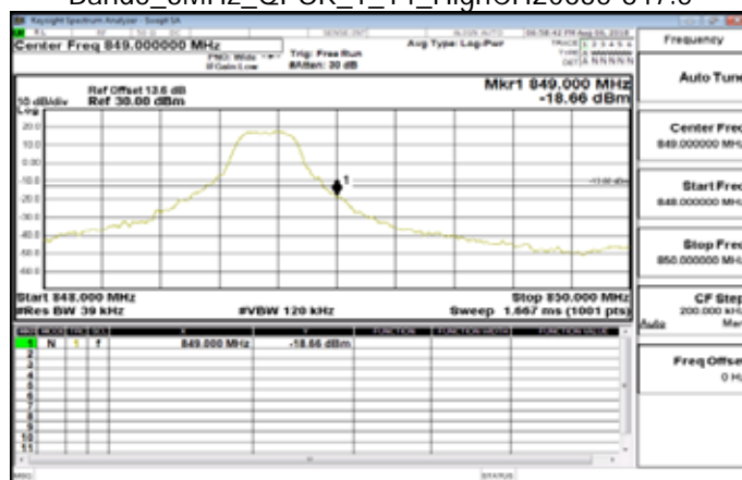
Band5_3MHz_QPSK_1_14_HighCH20635-847.5
