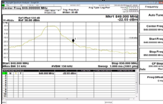
Band26_5MHz_QPSK_1_24_HighCH27015-846.5
