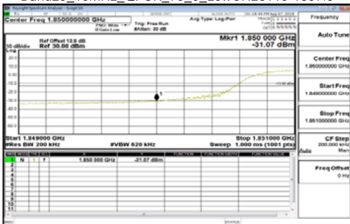
Band25_15MHz_QPSK_75_0_LowCH26115-1857.5
