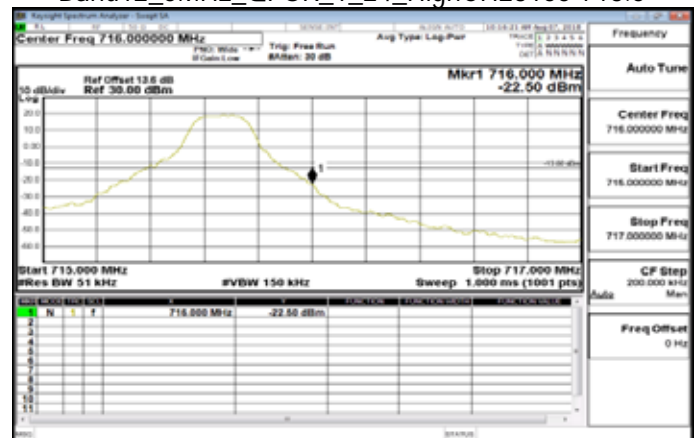
Band12_5MHz_QPSK_1_24_HighCH23155-713.5
