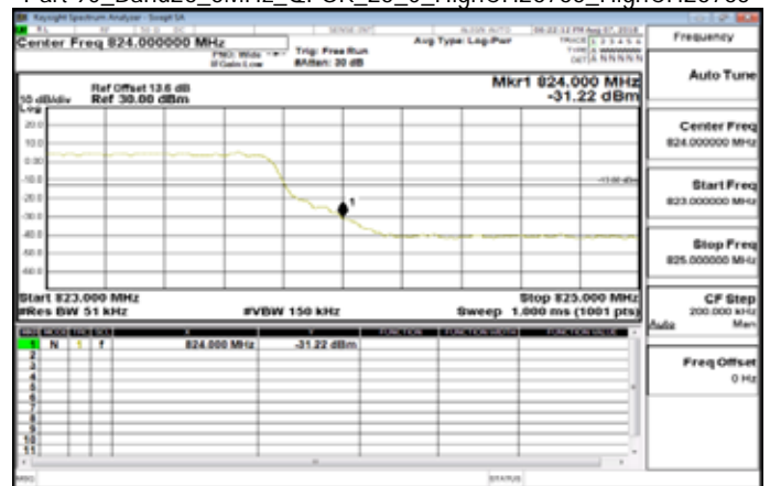
Part 90_Band26_5MHz_QPSK_25_0_HighCH26765_HighCH26765
