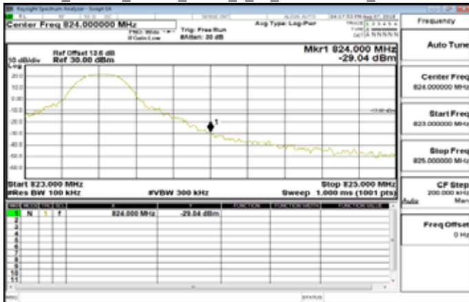
Part 90_Band26_10MHz_QPSK_1_49_MidCH26740_MidCH26740
