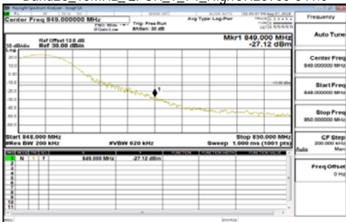
Band26_15MHz_QPSK_1_74_HighCH26965-841.5
