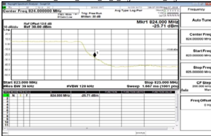
Part 90_Band26_3MHz_QPSK_15_0_HighCH26775_HighCH26775
