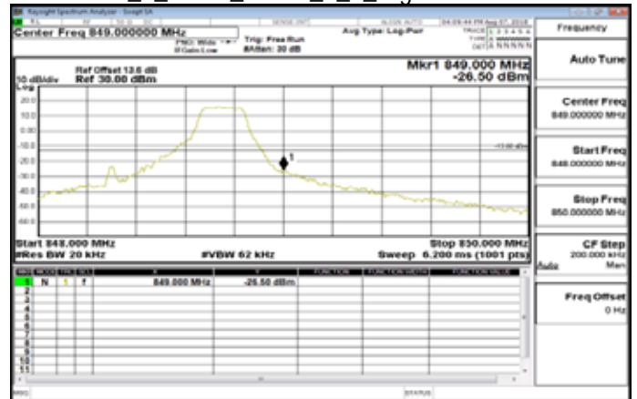
Band26_1_4MHz_QPSK_1_5_HighCH27033-848.3
