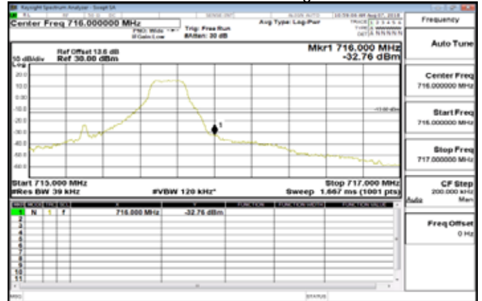
Band12_1_4MHz_QPSK_1_5_HighCH23173-715.3
