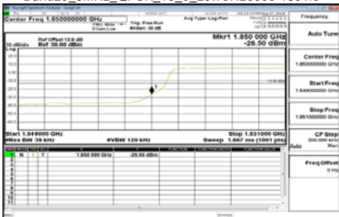
Band25_3MHz_QPSK_15_0_LowCH26055-1851.5
