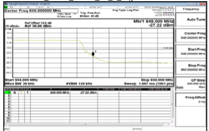
Band26_3MHz_QPSK_15_0_HighCH27025-847.5
