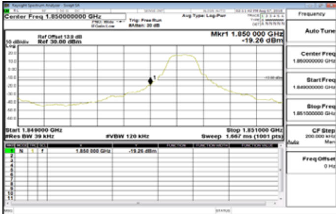
Band25_3MHz_QPSK_1_0_LowCH26055-1851.5
