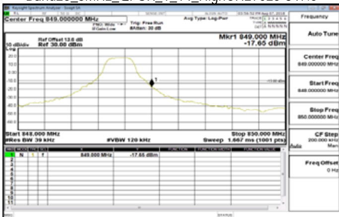
Band26_3MHz_QPSK_1_14_HighCH27025-847.5
