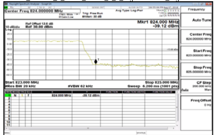
Part 90_Band26_1_4MHz_QPSK_6_0_HighCH26783_HighCH26783
