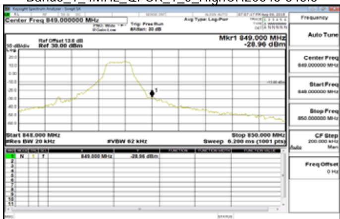
Band5_1_4MHz_QPSK_1_5_HighCH20643-848.3
