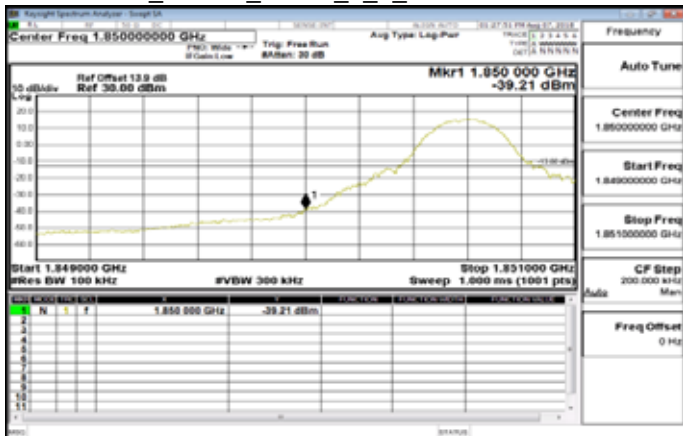
Band25_10MHz_QPSK_1_0_LowCH26090-1855
