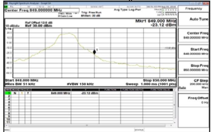
Band5_5MHz_QPSK_1_24_HighCH20625-846.5
