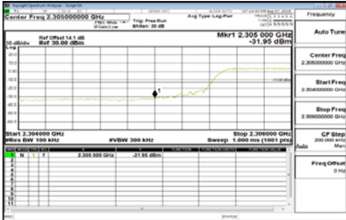
Band30_10MHz_QPSK_50_0_MidCH27710-2310 left
