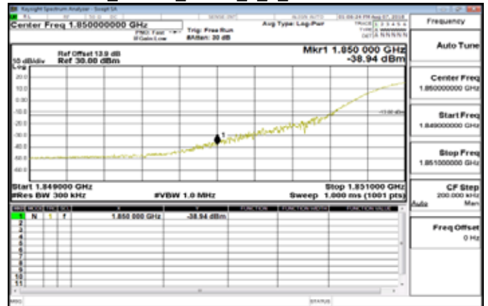
Band25_20MHz_QPSK_1_0_LowCH26140-1860
