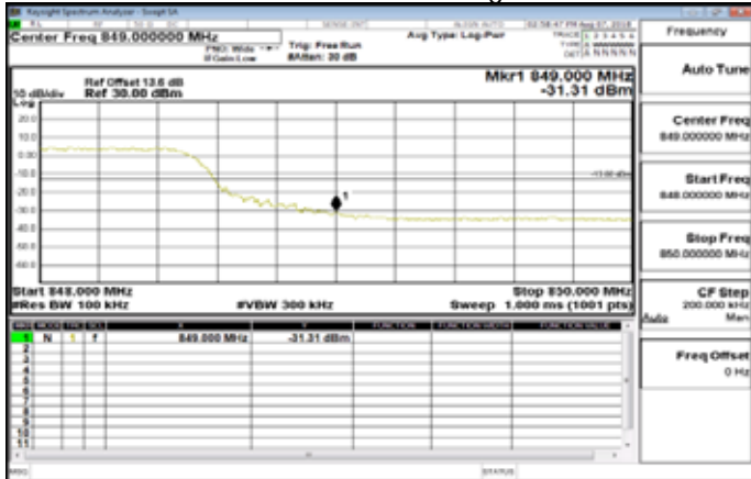
Band26_10MHz_QPSK_50_0_HighCH26990-844
