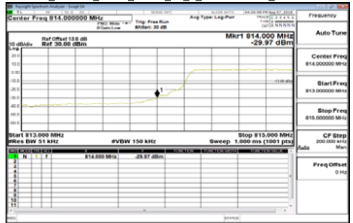
Part 90_Band26_5MHz_QPSK_25_0_LowCH26715_LowCH26715
