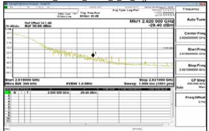
Band38_20MHz_QPSK_1_99_HighCH38150
