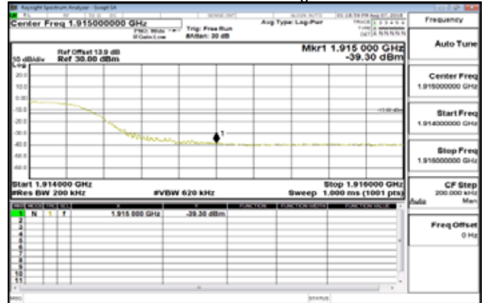
Band25_15MHz_QPSK_75_0_HighCH26615-1907.5
