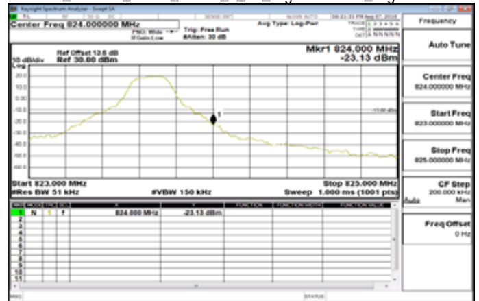
Part 90_Band26_5MHz_QPSK_1_24_HighCH26765_HighCH26765
