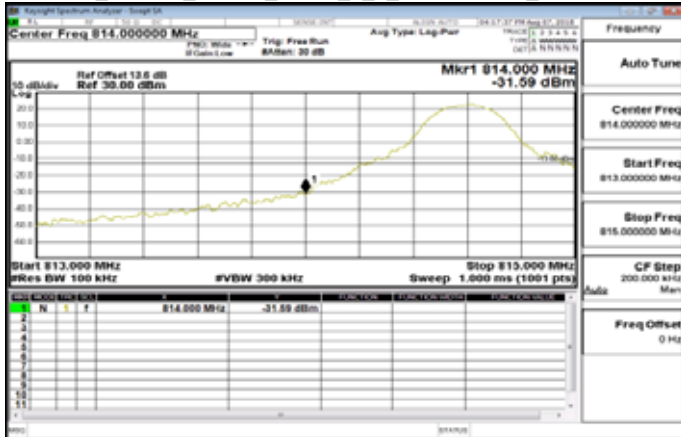
Part 90_Band26_10MHz_QPSK_1_0_MidCH26740_MidCH26740
