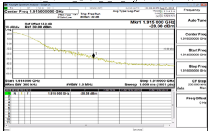
Band25_20MHz_QPSK_1_99_HighCH26590-1905
