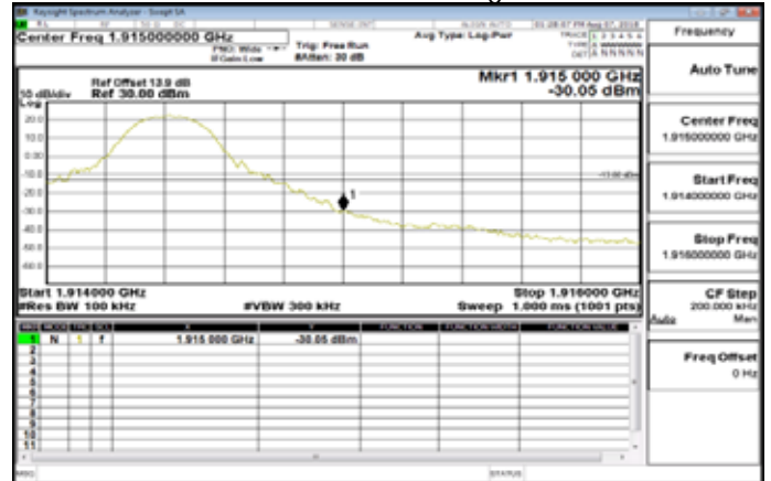
Band25_10MHz_QPSK_1_49_HighCH26640-1910
