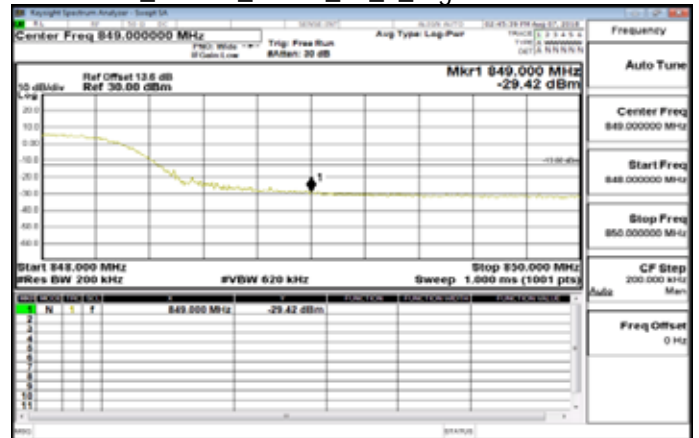
Band26_15MHz_QPSK_75_0_HighCH26965-841.5
