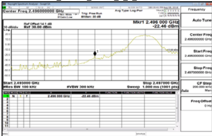
Band41_10MHz_QPSK_1_0_LowCH39700
