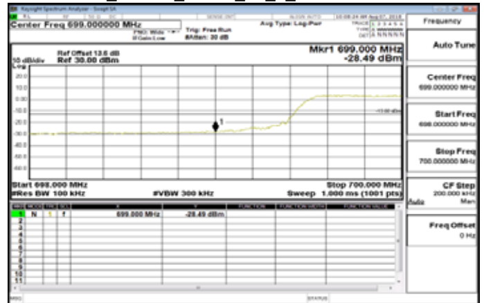
Band12_10MHz_QPSK_50_0_LowCH23060-704
