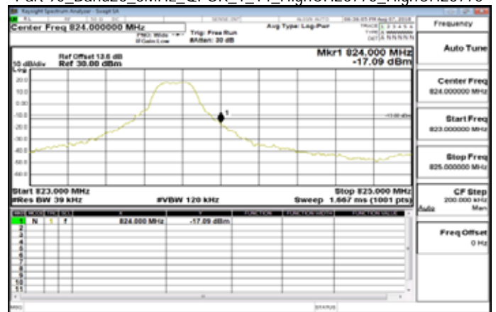
Part 90_Band26_3MHz_QPSK_1_14_HighCH26775_HighCH26775
