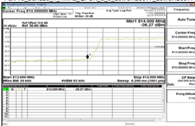
Part 90_Band26_1_4MHz_QPSK_6_0_LowCH26697_LowCH26697
