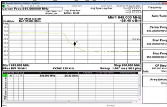
Band5_3MHz_QPSK_15_0_HighCH20635-847.5
