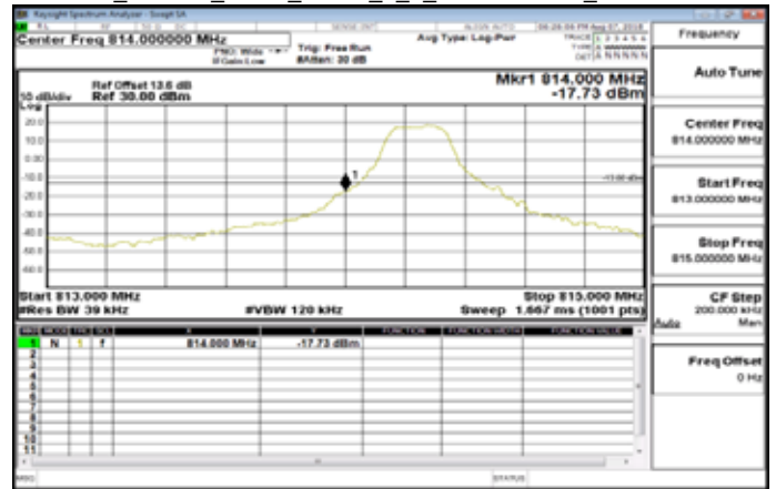
Part 90_Band26_3MHz_QPSK_1_0_LowCH26705_LowCH26705
