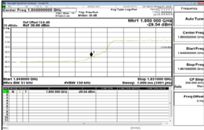
Band25_5MHz_QPSK_25_0_LowCH26065-1852.5
