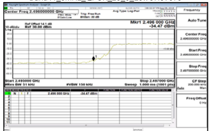
Band41_5MHz_QPSK_25_0_LowCH39675
