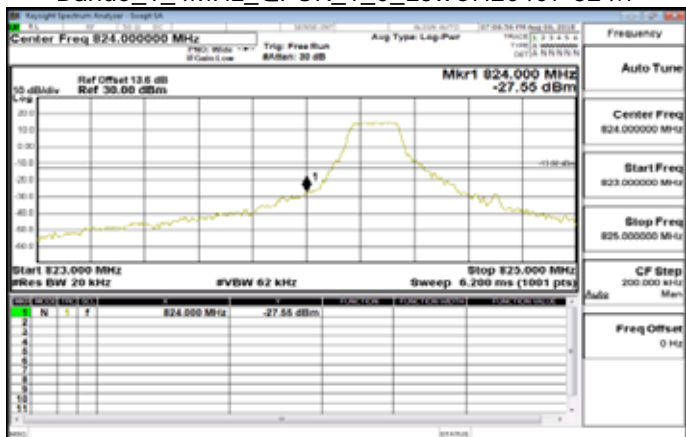
Band5_1_4MHz_QPSK_1_0_LowCH20407-824.7
