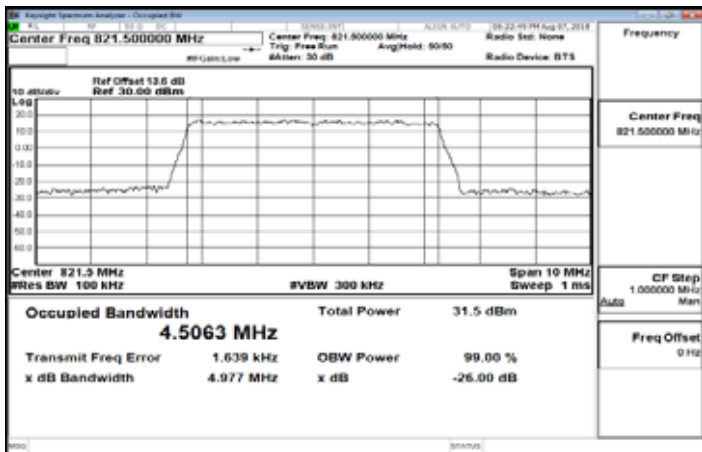
Part 90_Band26_5MHz_16QAM_25_0_HighCH26765
