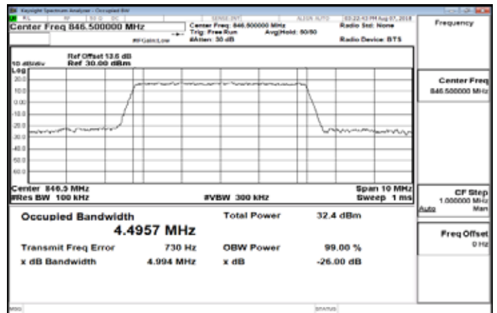
Band26_5MHz_QPSK_25_0_HighCH27015
