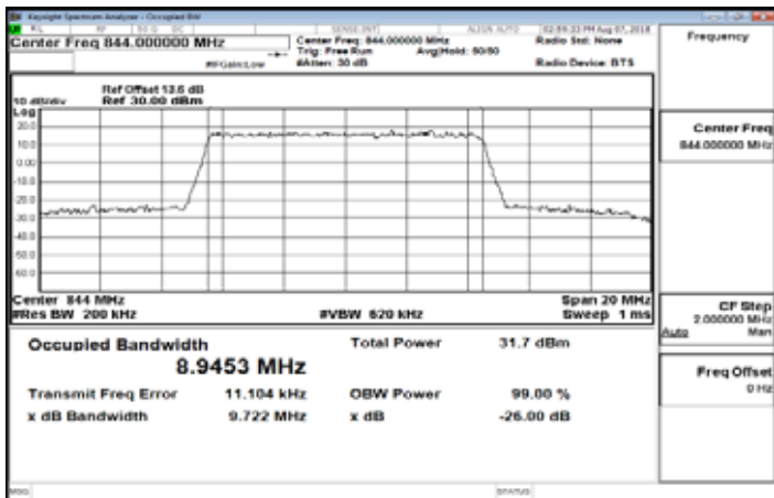
Band26_10MHz_16QAM_50_0_HighCH26990
