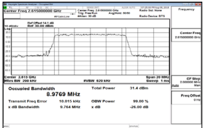
Band38_10MHz_QPSK_50_0_HighCH38200-2615
