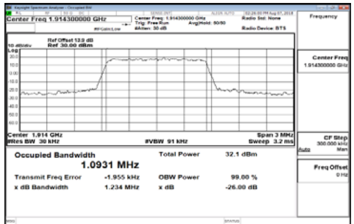
Band25_1_4MHz_QPSK_6_0_HighCH26683-1914.3
