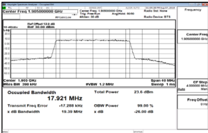
Band25_20MHz_16QAM_100_0_HighCH26590-1905
