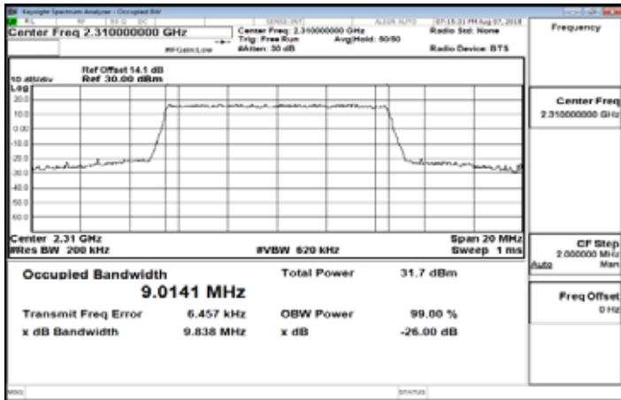
Band30_10MHz_16QAM_50_0_MidCH27710
