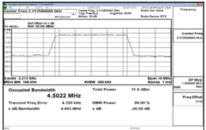
Band30_5MHz_16QAM_25_0_HighCH27735
