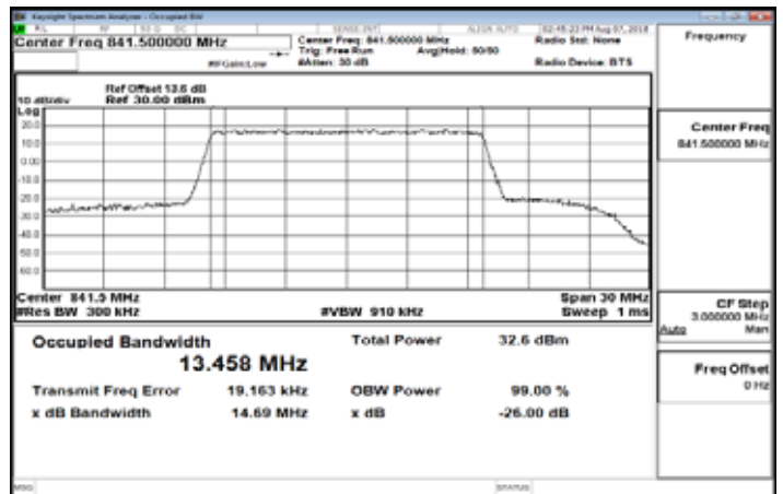
Band26_15MHz_QPSK_75_0_HighCH26965
