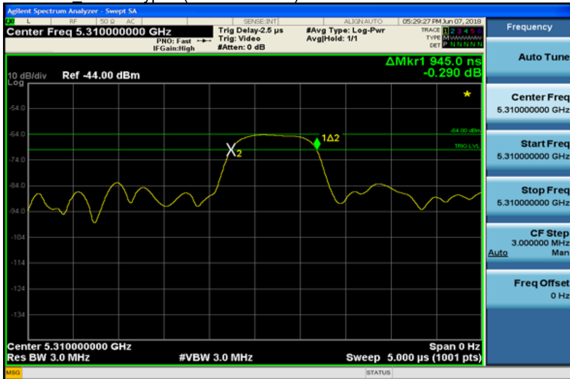
Radar Pulse width Radar Type 0(5310MHz-40M)
