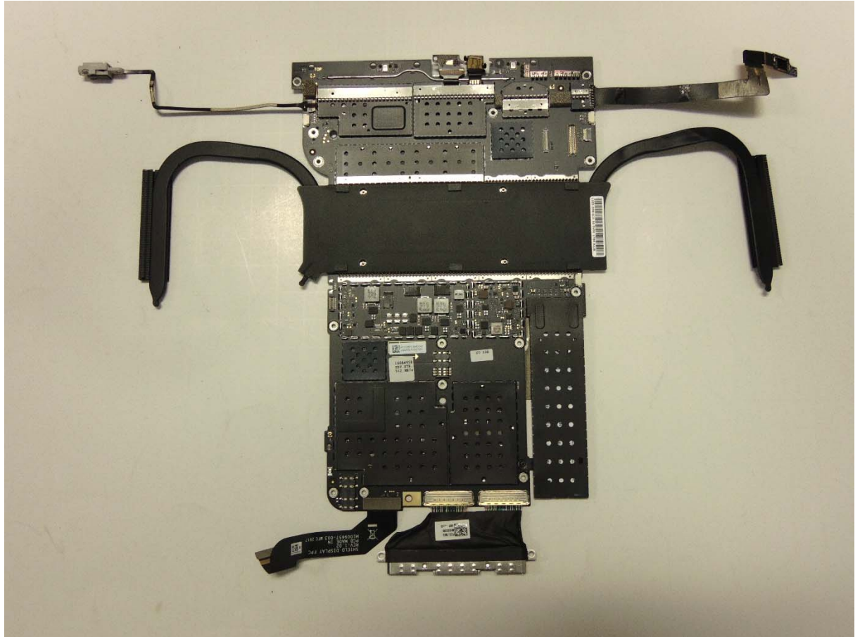
Motherboard top side with shield cans
