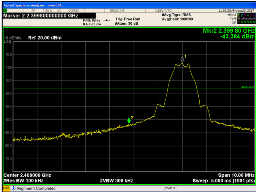
Figure 9-23 Conducted-Low Band Edge (Ch. 0)
