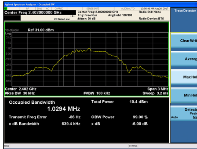
Figure 9-5 99% Bandwidth (Ch. 0)
