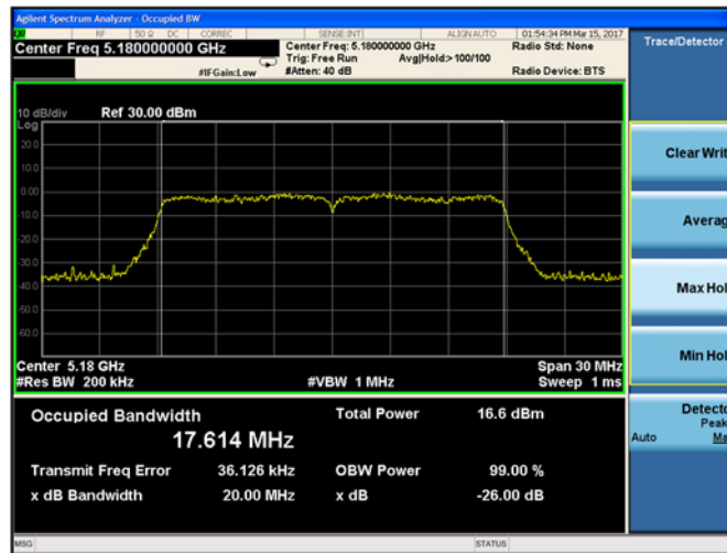
Plot 9-37. 26-dB Emission Bandwidth and 99% OBW Chain B 802.11n HT20 (Ch. 36)
