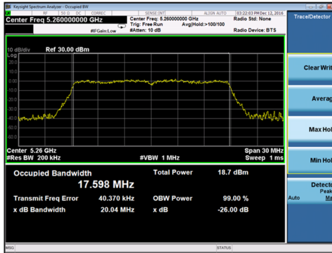
Plot 9-28. 26-dB Emission Bandwidth and 99% OBW Chain A 802.11n HT20 (Ch. 52)
