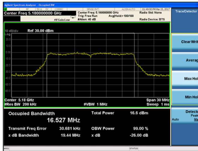
Plot 9-13. 26-dB Emission Bandwidth and 99% OBW Chain B 802.11a (Ch. 36)
