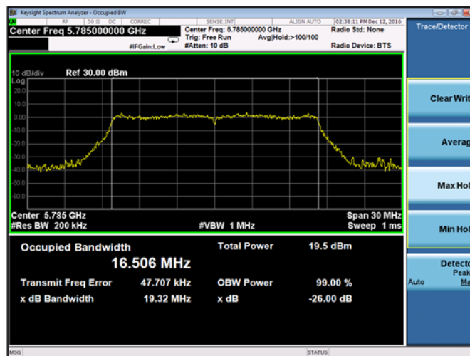
Plot 9-23. 26-dB Emission Bandwidth and 99% OBW Chain B 802.11a (Ch. 157)
