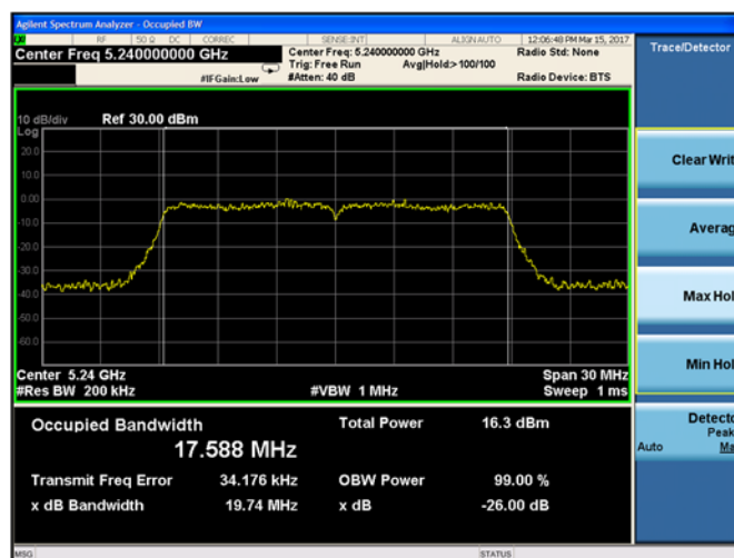
Plot 9-27. 26-dB Emission Bandwidth and 99% OBW Chain A 802.11n HT20 (Ch. 48)
