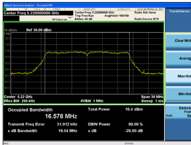
Plot 9-2. 26-dB Emission Bandwidth and 99% OBW Chain A 802.11a (Ch. 44)
