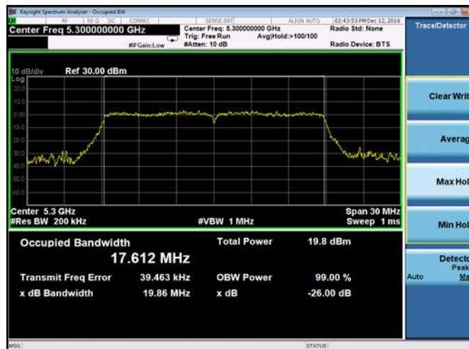
Plot 9-41. 26-dB Emission Bandwidth and 99% OBW Chain B 802.11n HT20 (Ch. 60)
