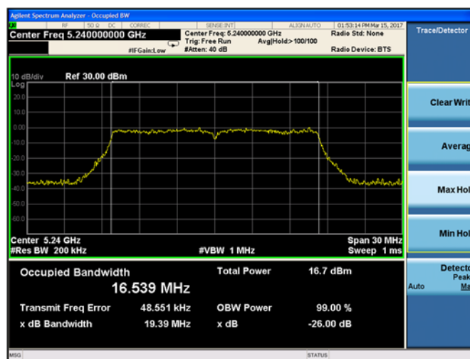
Plot 9-15. 26-dB Emission Bandwidth and 99% OBW Chain B 802.11a (Ch. 48)
