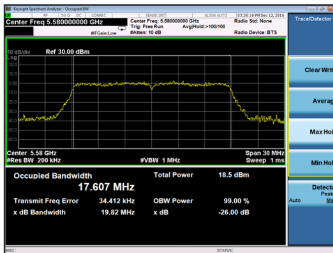
Plot 9-32. 26-dB Emission Bandwidth and 99% OBW Chain A 802.11n HT20 (Ch. 116)
