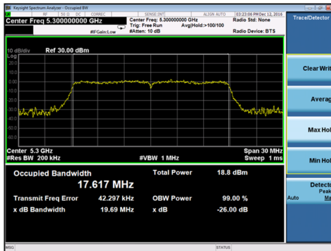
Plot 9-29. 26-dB Emission Bandwidth and 99% OBW Chain A 802.11n HT20 (Ch. 60)
