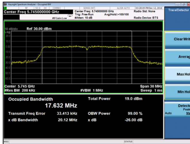
Plot 9-34. 26-dB Emission Bandwidth and 99% OBW Chain A 802.11n HT20 (Ch. 149)
