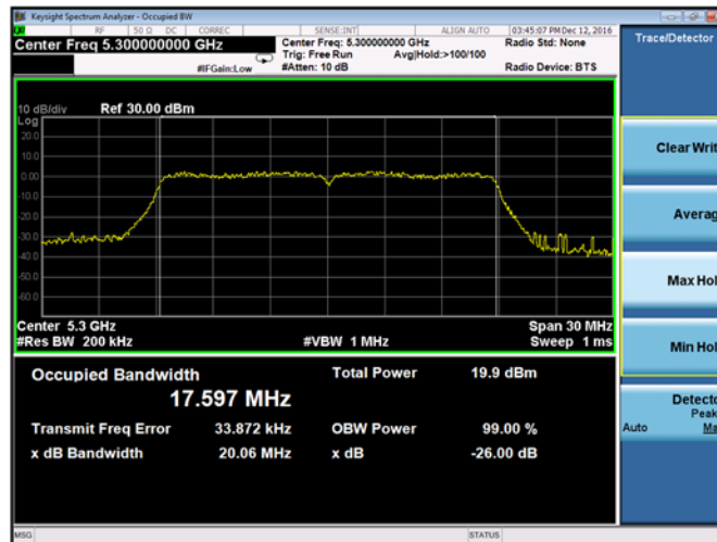
Plot 9-71. 26dB Emission Bandwidth and 99% OBW Chain A 802.11ac VHT 20 (CH. 60)
