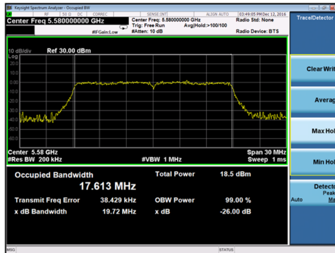
Plot 9-74. 26dB Emission Bandwidth and 99% OBW Chain A 802.11ac VHT 20 (CH. 116)
