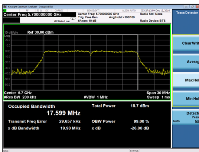
Plot 9-33. 26-dB Emission Bandwidth and 99% OBW Chain A 802.11n HT20 (Ch. 140)
