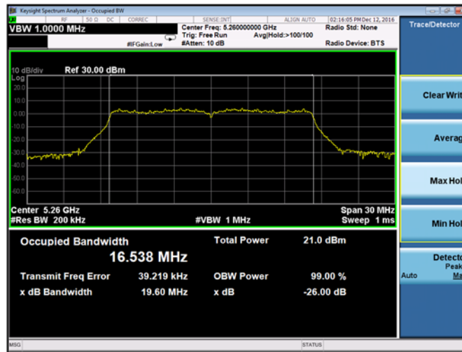
Plot 9-16. 26-dB Emission Bandwidth and 99% OBW Chain B 802.11a (Ch. 52)
