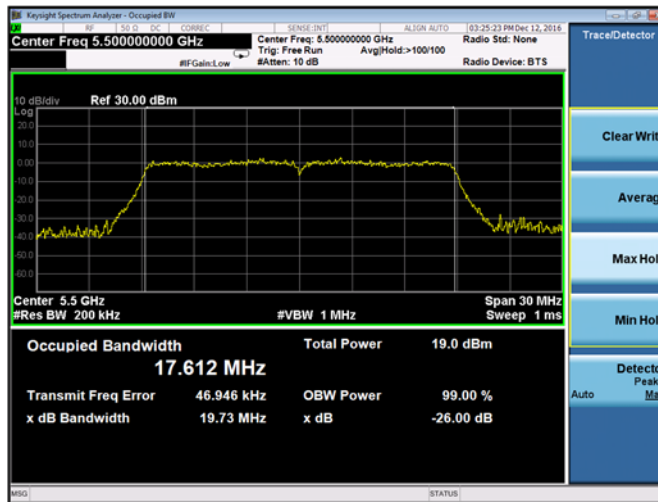
Plot 9-31. 26-dB Emission Bandwidth and 99% OBW Chain A 802.11n HT20 (Ch. 100)
