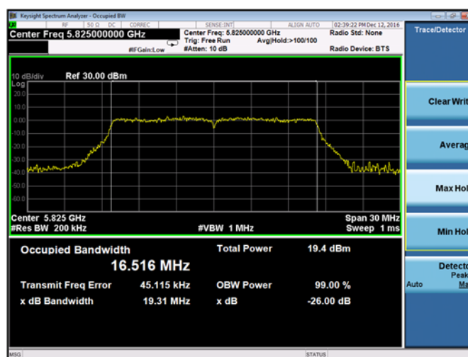
Plot 9-24. 26-dB Emission Bandwidth and 99% OBW Chain B 802.11a (Ch. 165)
