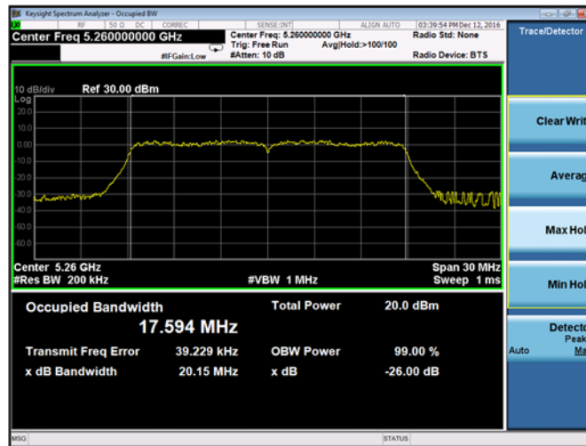
Plot 9-70. 26dB Emission Bandwidth and 99% OBW Chain A 802.11ac VHT 20 (CH. 52)
