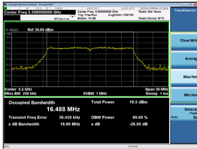
Plot 9-19. 26-dB Emission Bandwidth Chain and 99% OBW B 802.11a (Ch. 100)
