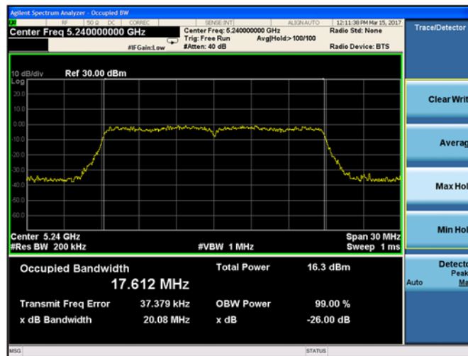
Plot 9-69. 26dB Emission Bandwidth and 99% OBW Chain A 802.11ac VHT 20 (CH. 48)
