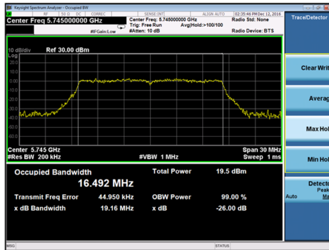
Plot 9-22. 26-dB Emission Bandwidth and 99% OBW Chain B 802.11a (Ch. 149)
