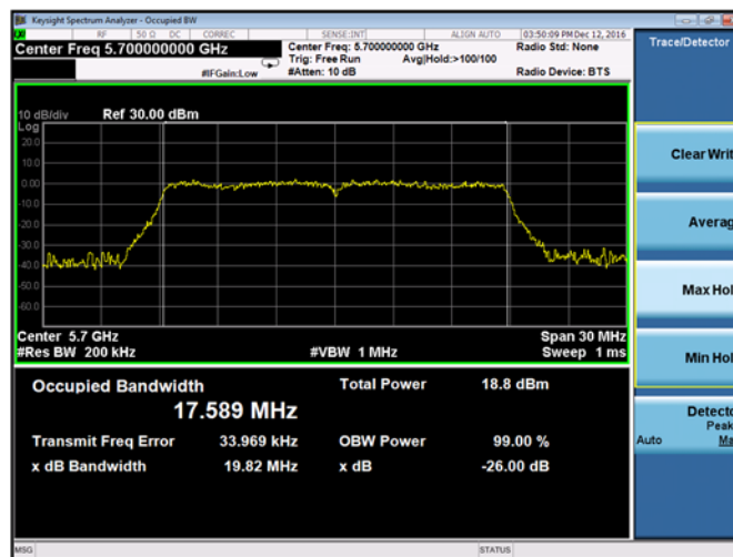
Plot 9-75. 26dB Emission Bandwidth and 99% OBW Chain A 802.11ac VHT 20 (CH. 140)
