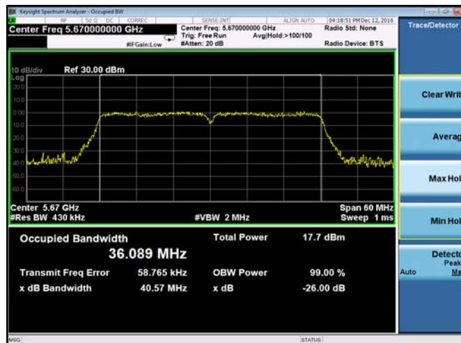
Plot 9-55. 26-dB Emission Bandwidth and 99% OBW Chain A 802.11n HT40 (Ch. 134)
