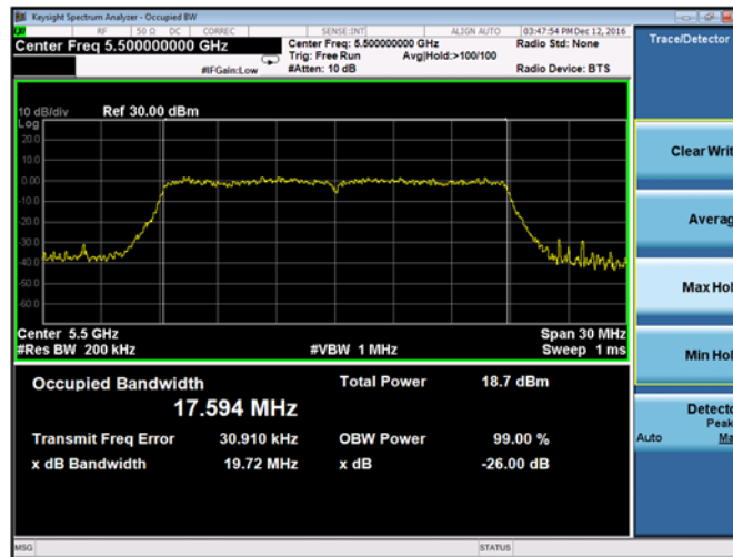
Plot 9-73. 26dB Emission Bandwidth and 99% OBW Chain A 802.11ac VHT 20 (CH. 100)
