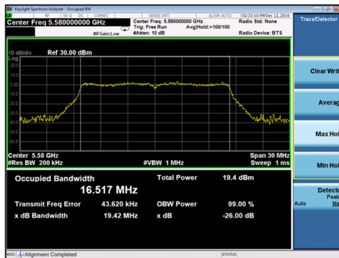
Plot 9-20. 26-dB Emission Bandwidth and 99% OBW Chain B 802.11a (Ch. 116)
