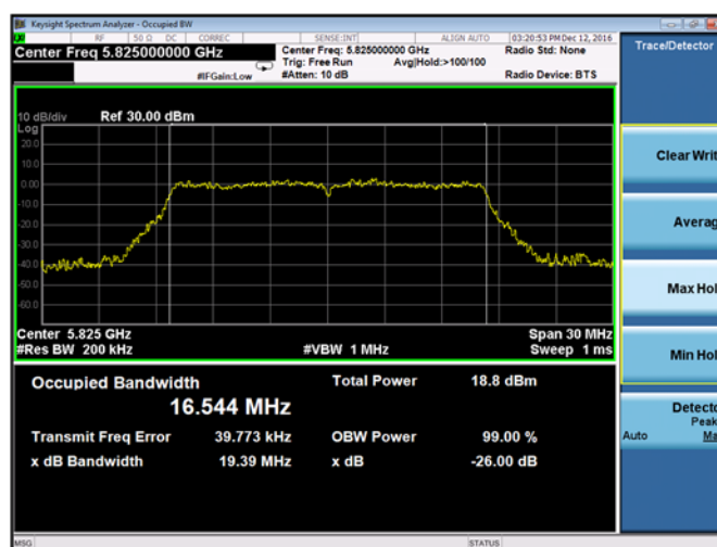
Plot 9-12. 26-dB Emission Bandwidth and 99% OBW Chain A 802.11a (Ch. 165)
