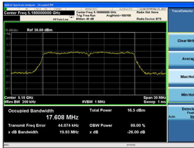
Plot 9-67. 26dB Emission Bandwidth and 99% OBW Chain A 802.11ac VHT 20 (CH. 36)
