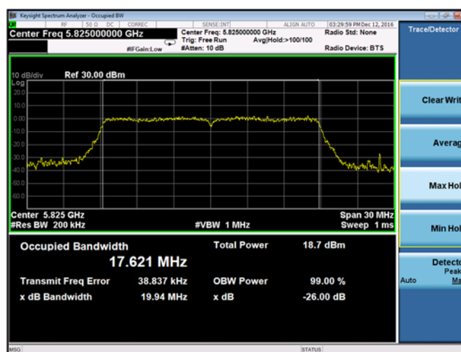
Plot 9-36. 26-dB Emission Bandwidth and 99% OBW Chain A 802.11n HT20 (Ch. 165)
