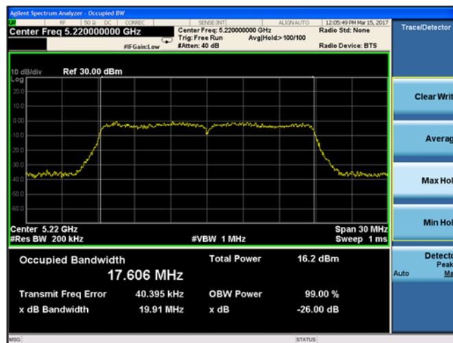
Plot 9-26. 26-dB Emission Bandwidth and 99% OBW Chain A 802.11n HT20 (Ch. 44)
