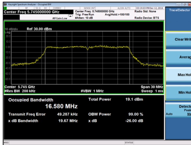
Plot 9-10. 26-dB Emission Bandwidth and 99% OBW Chain A 802.11a (Ch. 149)
