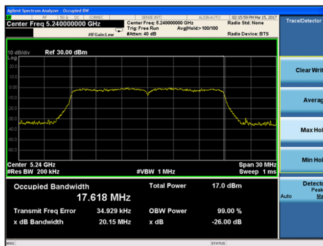
Plot 9-39. 26-dB Emission Bandwidth and 99% OBW Chain B 802.11n HT20 (Ch. 48)
