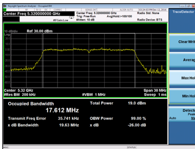
Plot 9-30. 26-dB Emission Bandwidth and 99% OBW Chain A 802.11n HT20 (Ch. 64)
