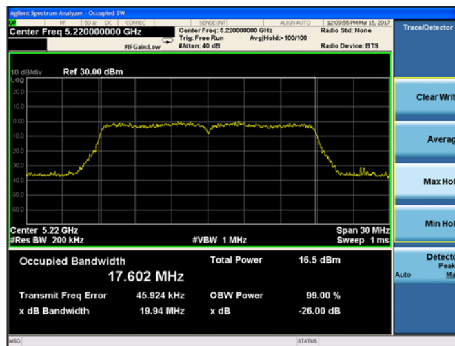
Plot 9-68. 26dB Emission Bandwidth and 99% OBW Chain A 802.11ac VHT 20 (CH. 44)
