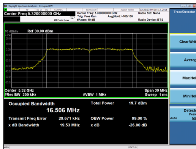
Plot 9-18. 26-dB Emission Bandwidth and 99% OBW Chain B 802.11a (Ch. 64)
