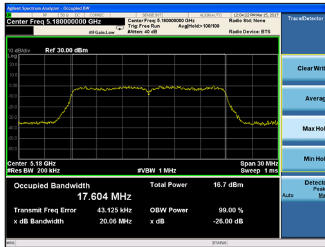
Plot 9-25. 26-dB Emission Bandwidth and 99% OBW Chain A 802.11n HT20 (Ch. 36)
