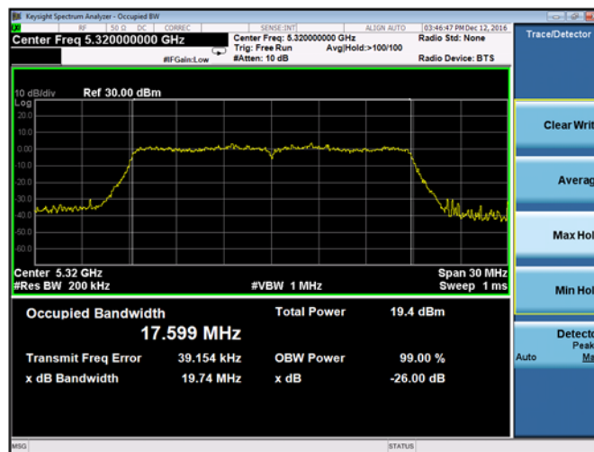
Plot 9-72. 26dB Emission Bandwidth and 99% OBW Chain A 802.11ac VHT 20 (CH. 64)
