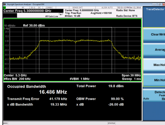
Plot 9-17. 26-dB Emission Bandwidth and 99% OBW Chain B 802.11a (Ch. 60)
