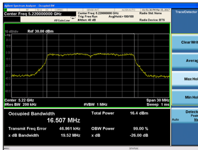
Plot 9-14. 26-dB Emission Bandwidth and 99% OBW Chain B 802.11a (Ch. 44)
