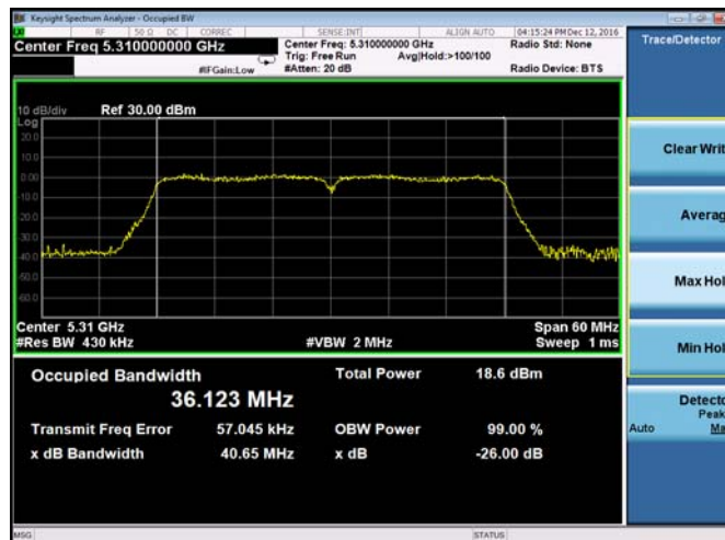
Plot 9-52. 26-dB Emission Bandwidth and 99% OBW Chain A 802.11n HT40 (Ch. 62)
