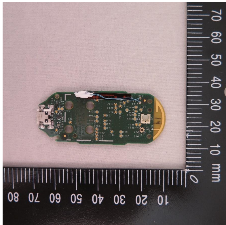
Figure 4. Back side of PCB with BT antenna with battery removed
