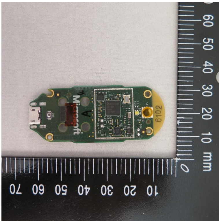
Figure 6. Top side of PCB with shield can removed
