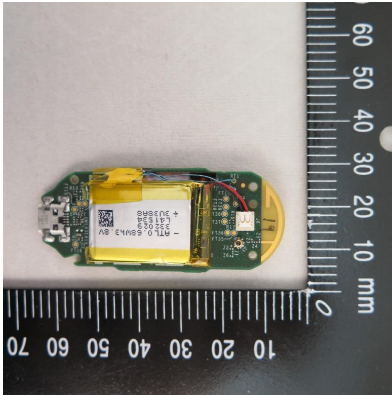
Figure 1. Back side of PCB with BT antenna
