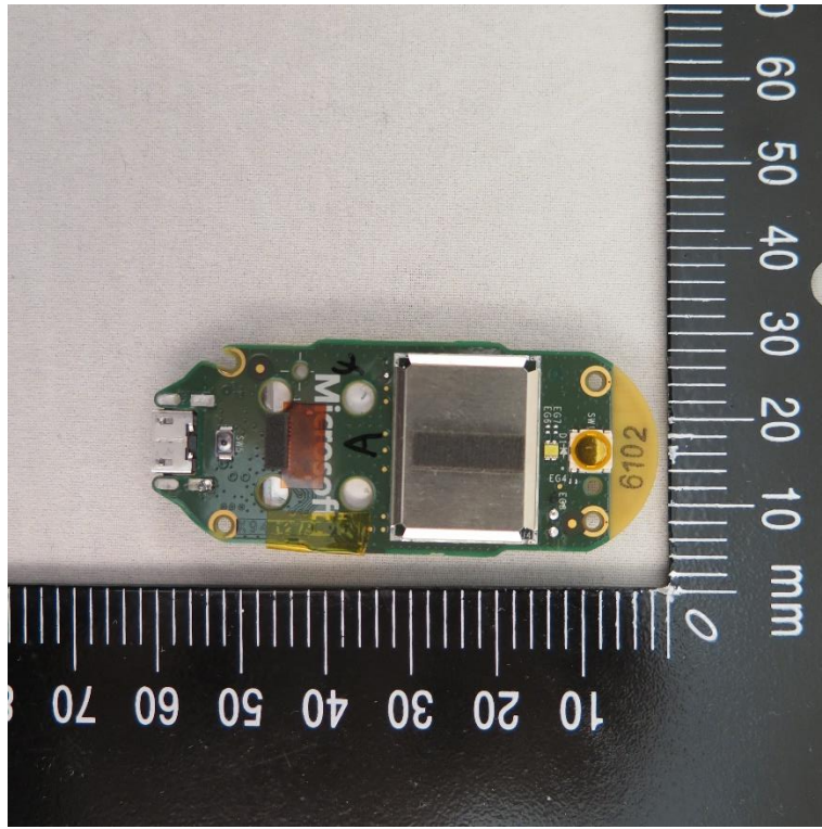
Figure 5. Top side of PCB with shield can
