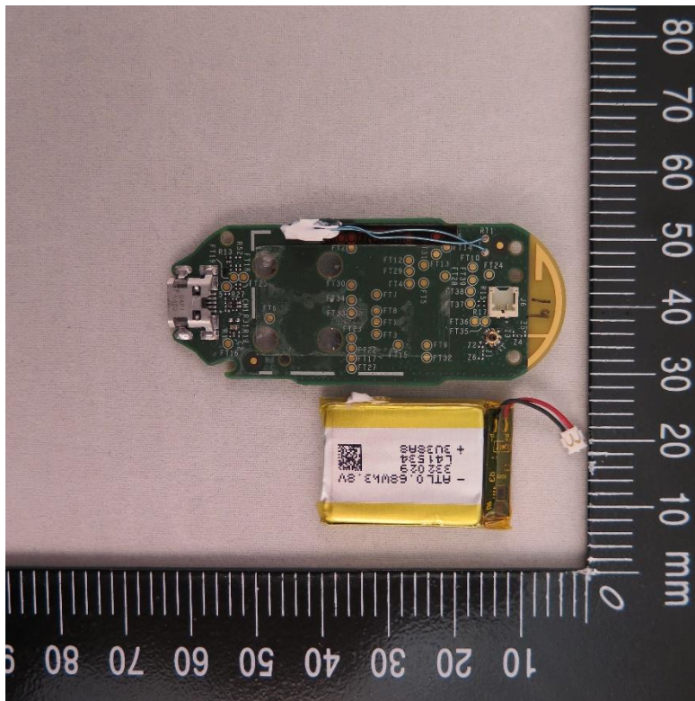
Figure 2. Back side of PCB with BT antenna and Battery removed
