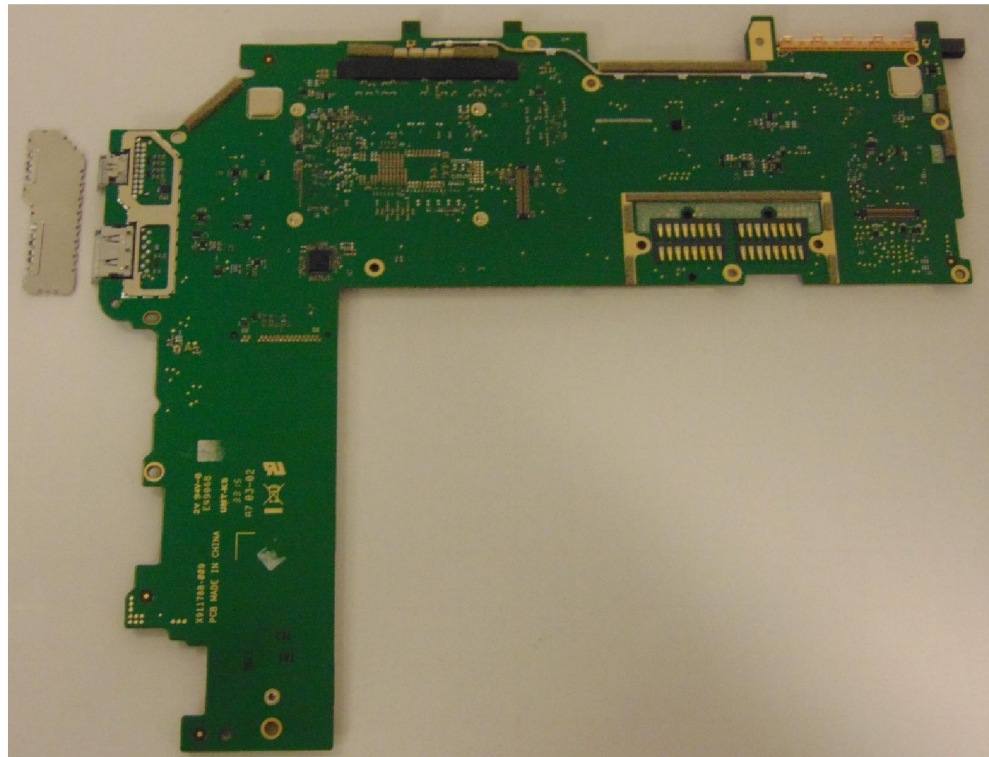
Motherboard bottom side with shield can removed
