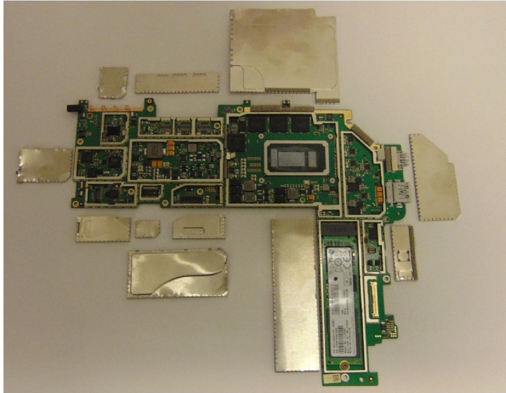
Motherboard top side with shield cans removed
