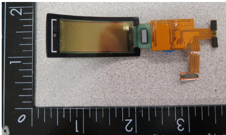
Board unfolded from display, showing back of Flex Board
