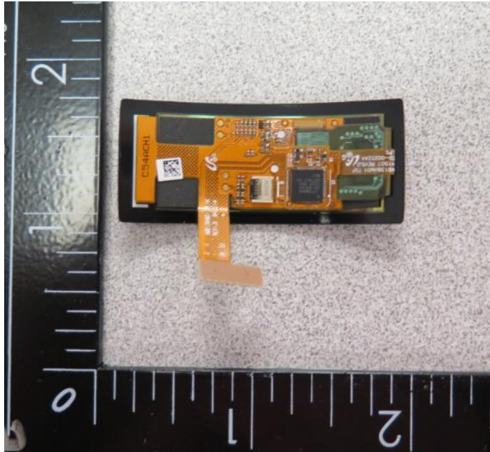
Board unfolded from display, showing back of Flex Board
