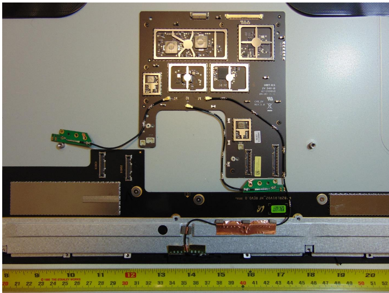
Figure 8. Connectivity Board with BT/WLAN (Close-up)
