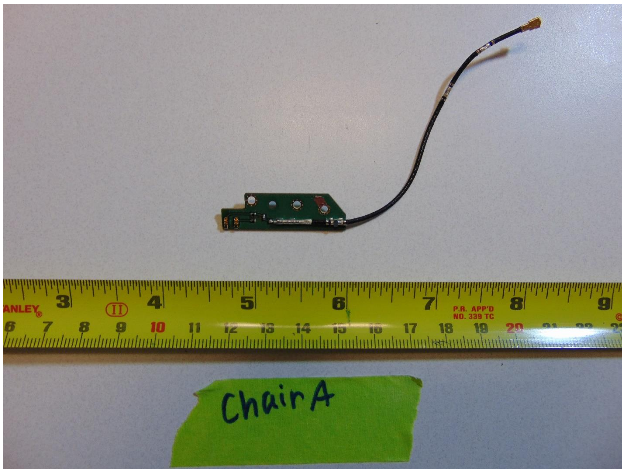
Figure 10. Chain A (WLAN MIMO)
