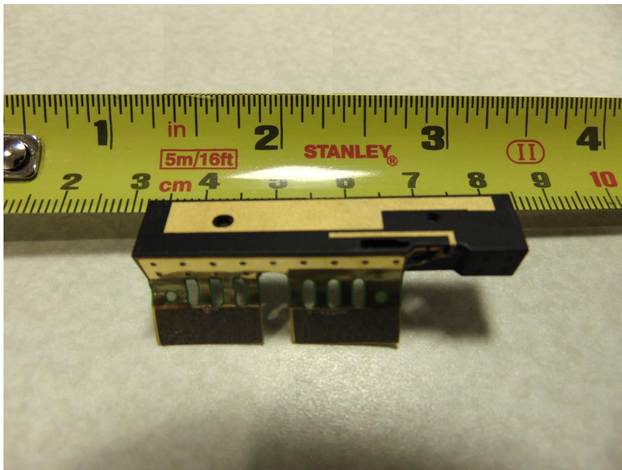
Figure 14. BT/Accessory Radio Antenna
