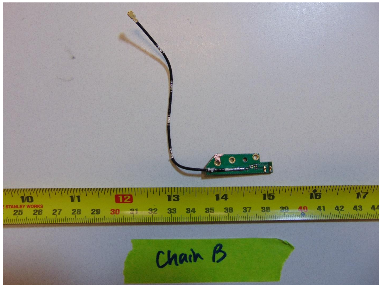
Figure 11. Chain B (WLAN Main)
