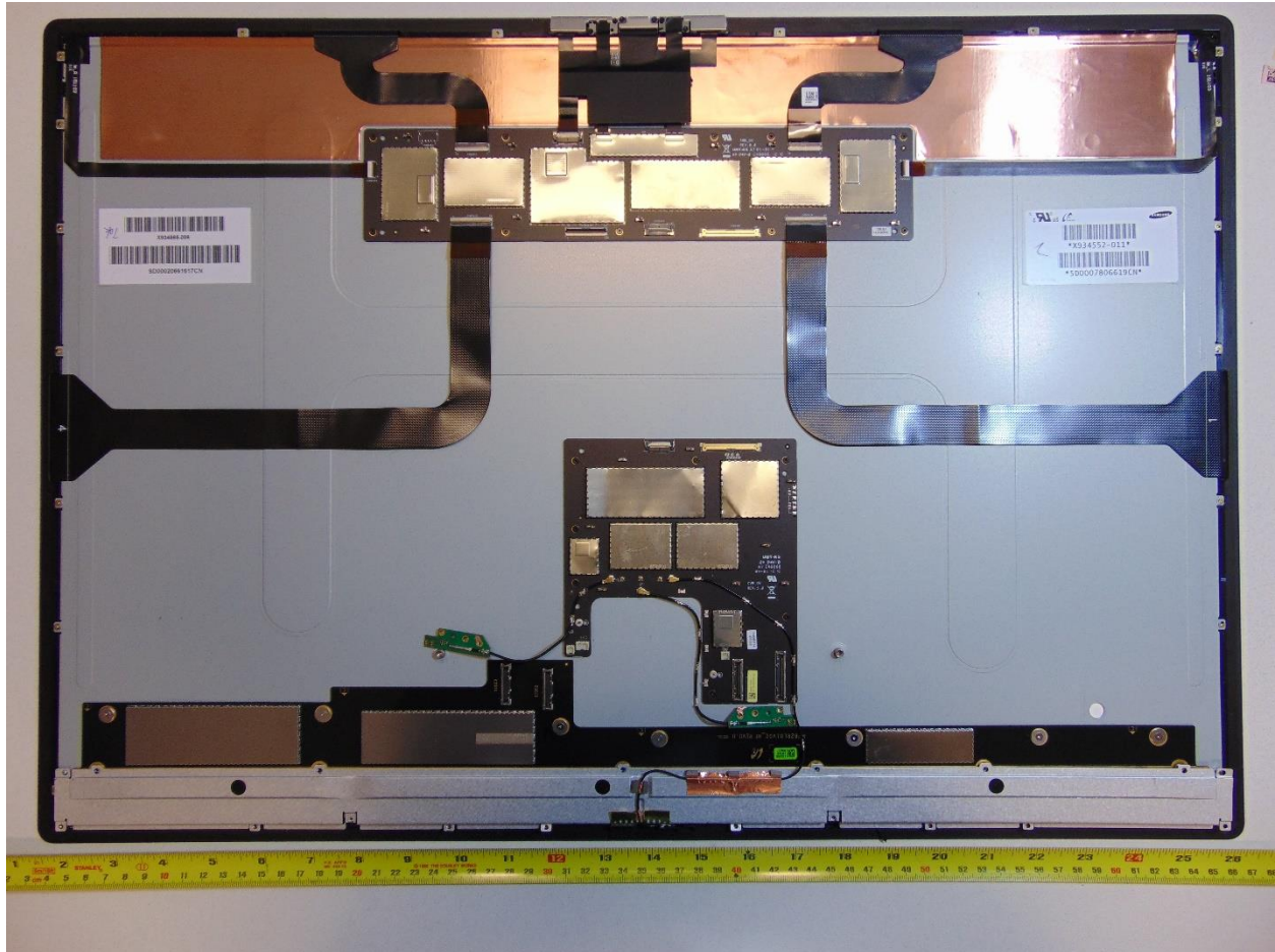
Figure 4. Rear cover of Monitor removed
