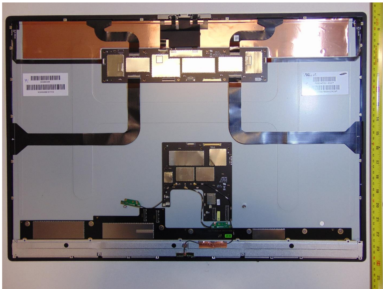
Figure 5. Rear cover of Monitor removed
