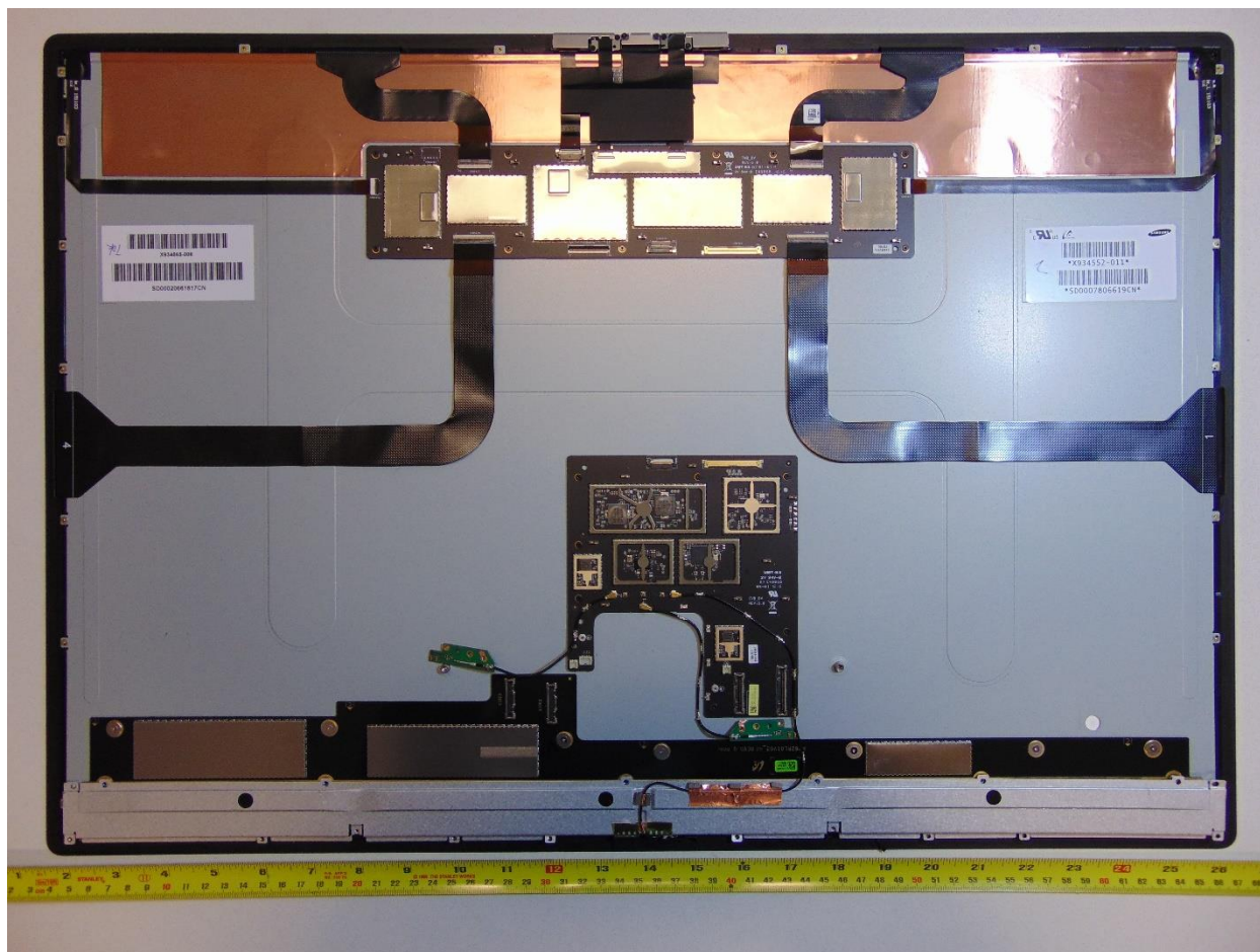
Figure 6. Shield cans removed from BT/WLAN connectivity board
