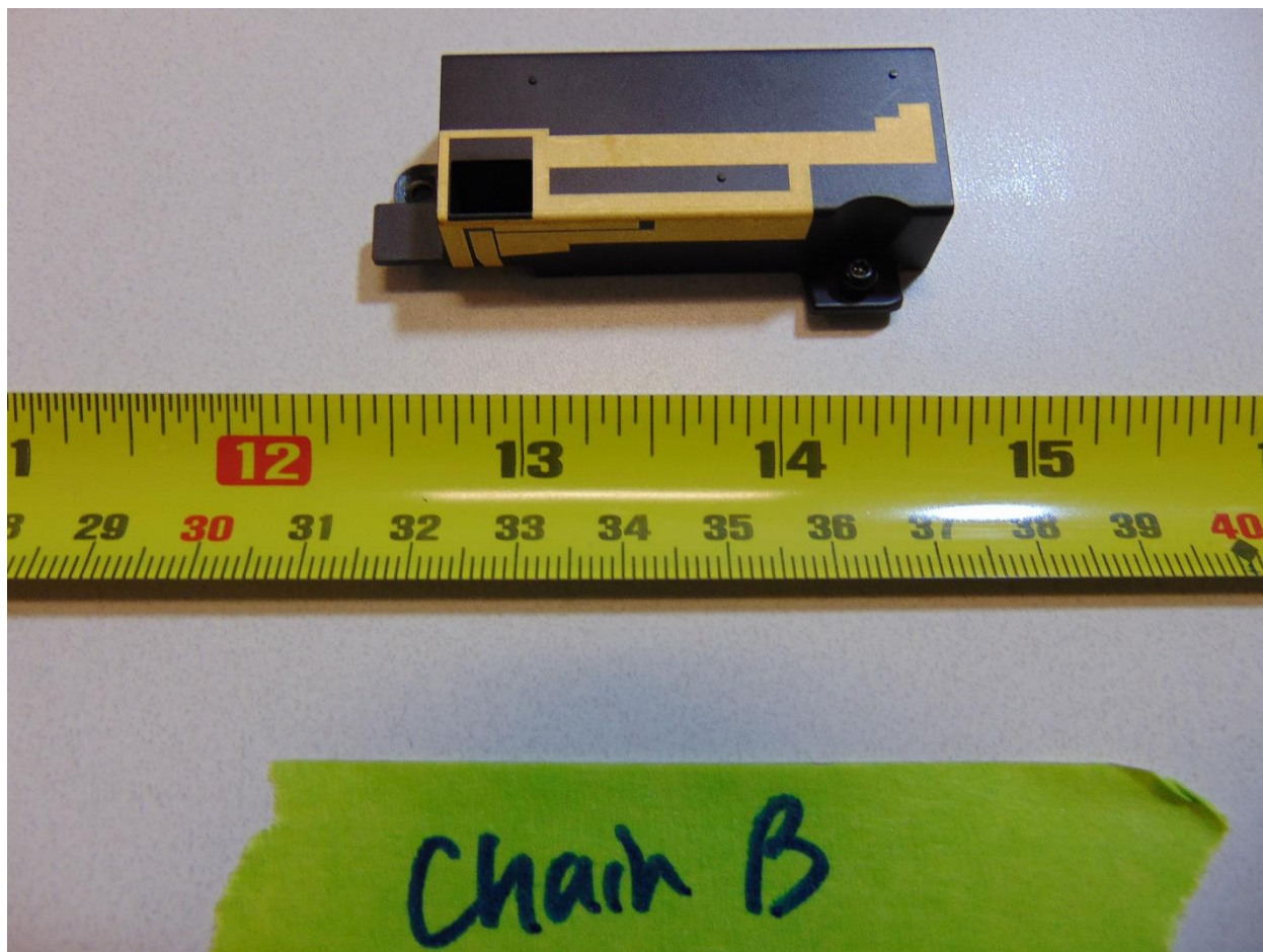
Figure 13. WLAN Main Antenna (Chain B)
