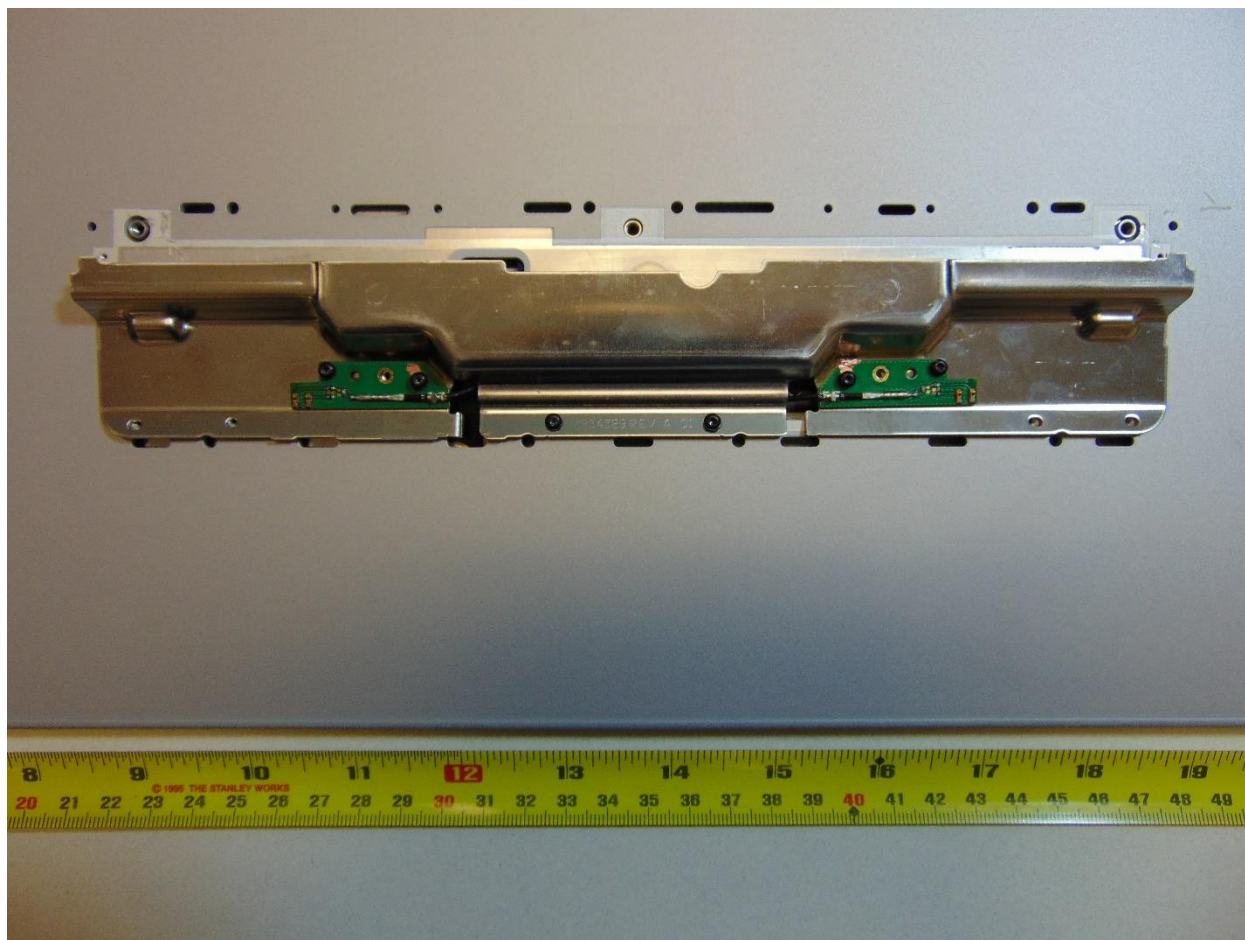
Figure 3. Hinge Cover, antennas removed
