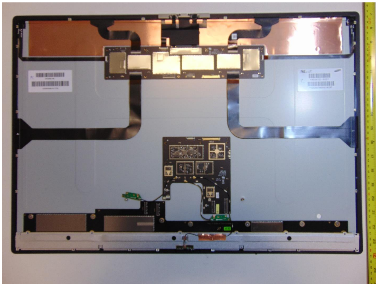
Figure 7. Shield cans removed for BT/WLAN connectivity board
