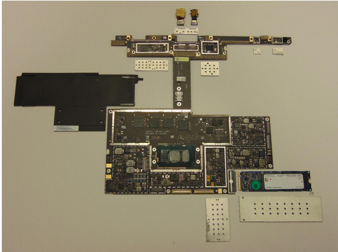
Motherboard top side with shield cans removed
