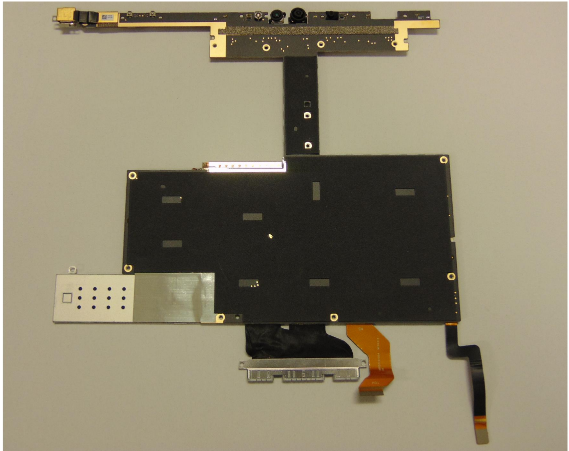
Motherboard bottom side with shield cans
