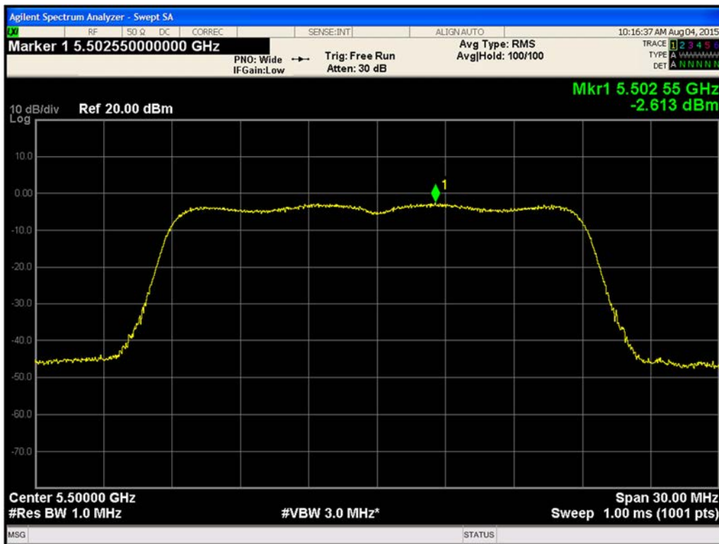
Figure 462. Maximum Power Spectral Density Chain A 802.11n HT20 (Ch. 100)
