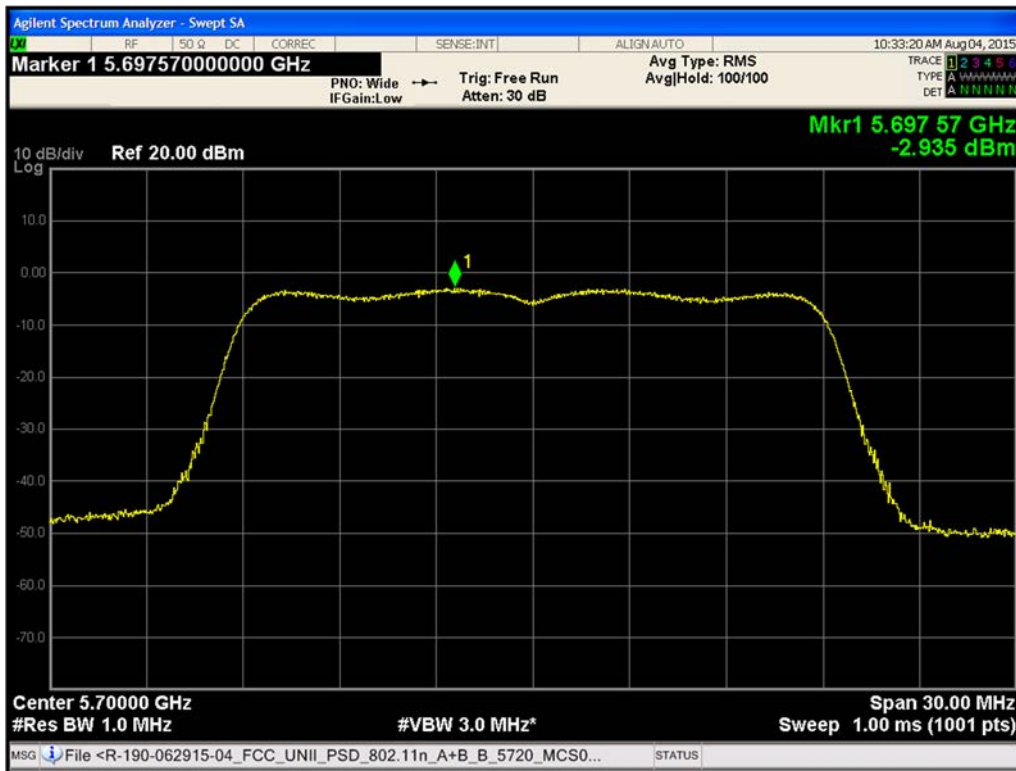
Figure 476. Maximum Power Spectral Density Chain B 802.11n HT20 (Ch. 140)
