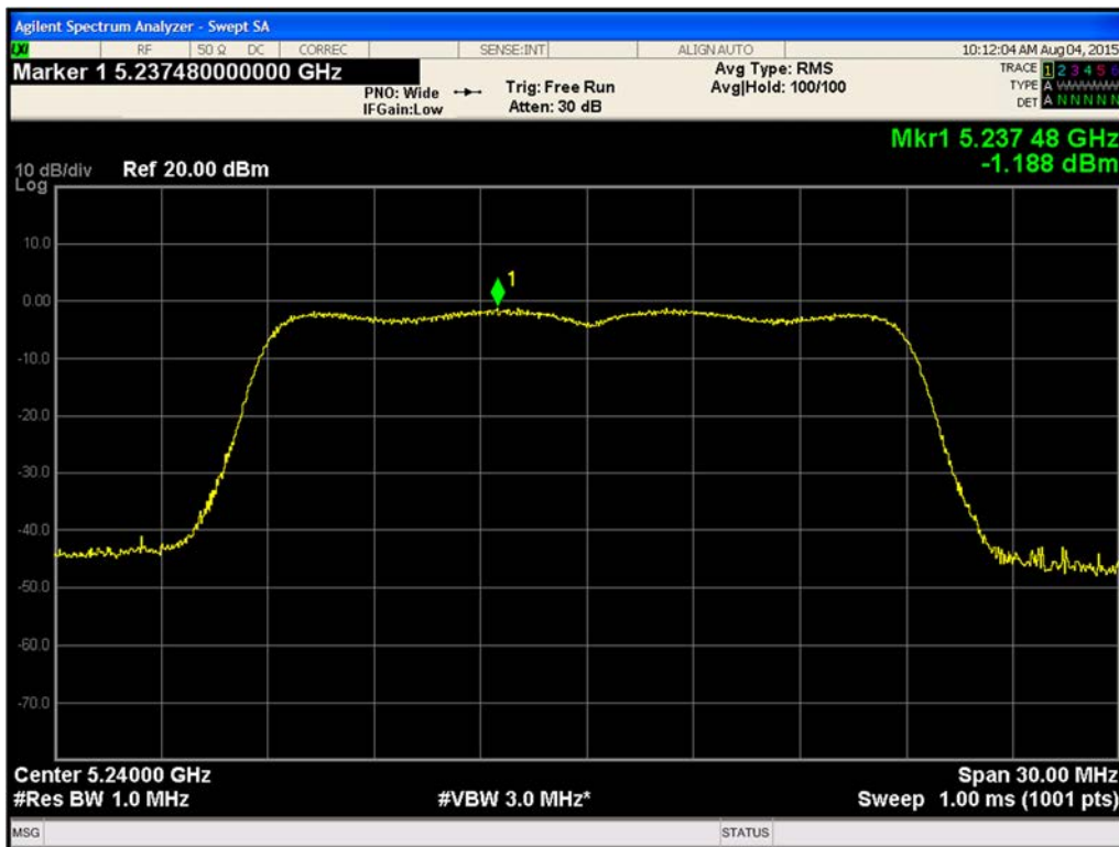
Figure 458. Maximum Power Spectral Density Chain A 802.11n HT20 (Ch. 48)
