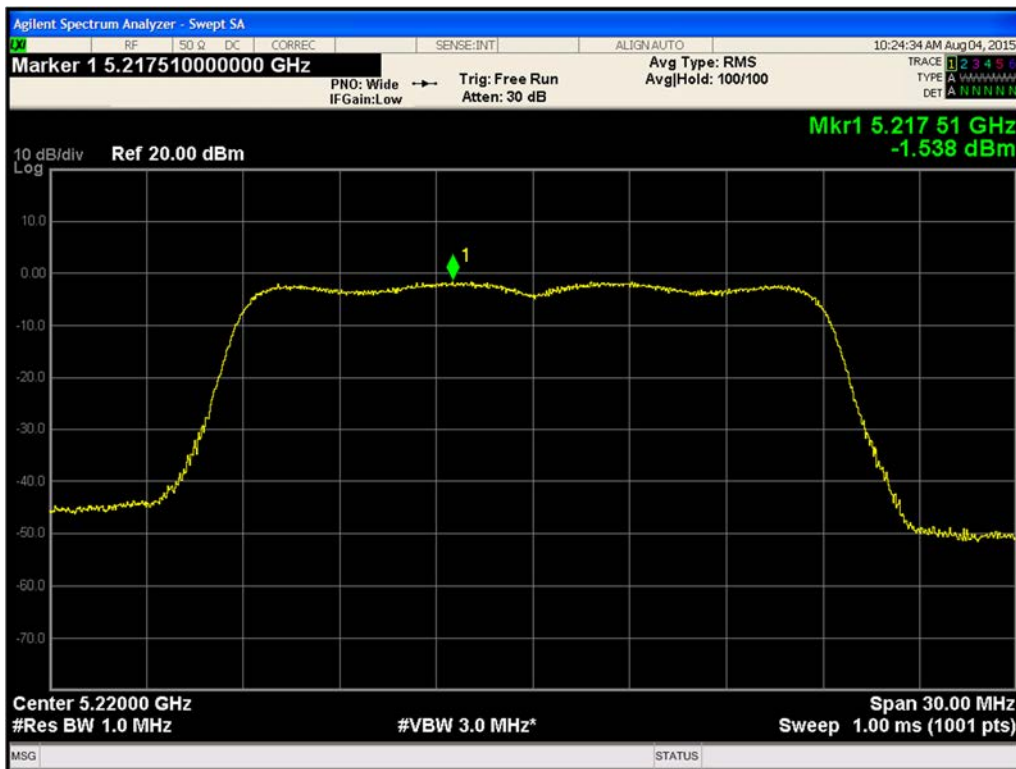
Figure 469. Maximum Power Spectral Density Chain B 802.11n HT20 (Ch. 44)
