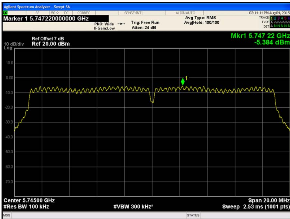
Figure 477. Maximum Power Spectral Density Chain B 802.11n HT20 (Ch. 149)
