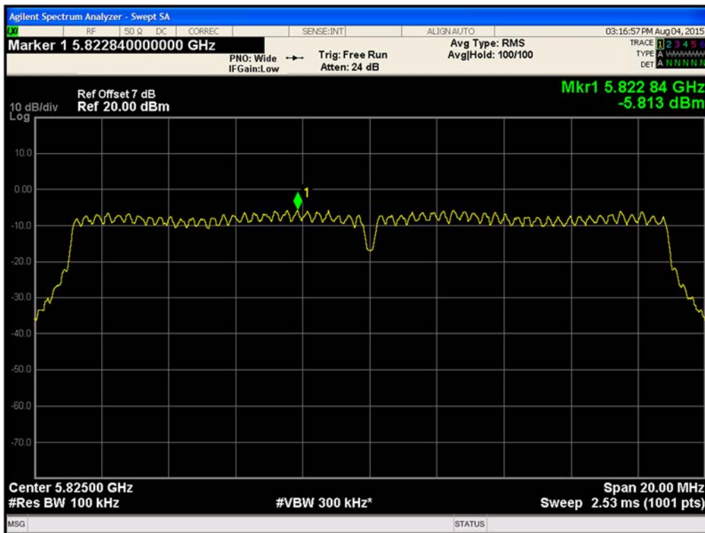
Figure 479. Maximum Power Spectral Density Chain B 802.11n HT20 (Ch. 165)
