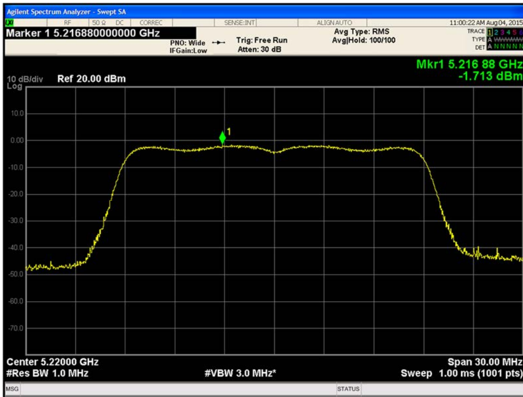
Figure 481. Maximum Power Spectral Density Chain A 802.11ac VHT20 (Ch. 44)
