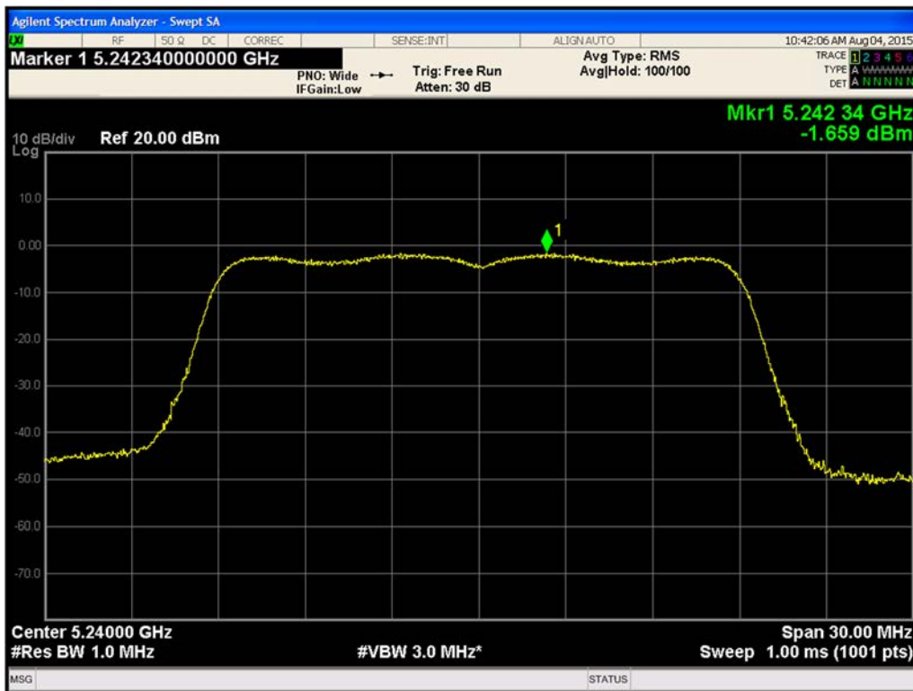
Figure 494. Maximum Power Spectral Density Chain B 802.11ac VHT20 (Ch. 48)
