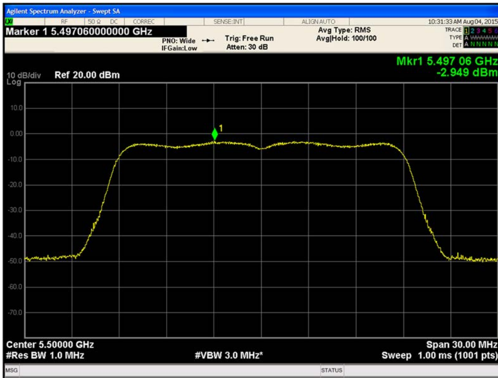
Figure 474. Maximum Power Spectral Density Chain B 802.11n HT20 (Ch. 100)
