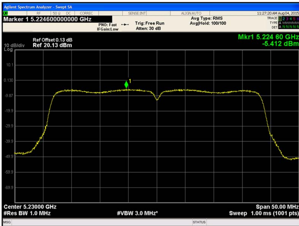
Figure 514. Maximum Power Spectral Density Chain B 802.11n HT40 (Ch. 46)
