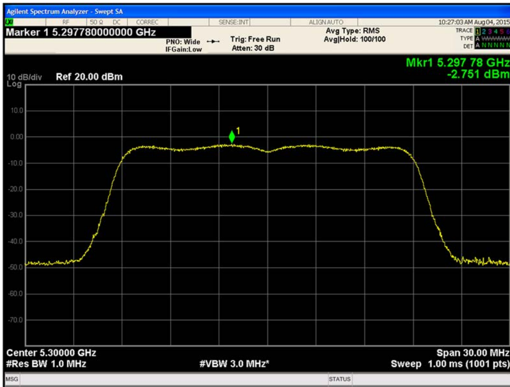
Figure 472. Maximum Power Spectral Density Chain B 802.11n HT20 (Ch. 60)
