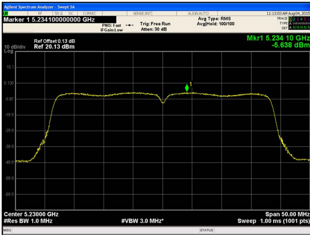
Figure 505. Maximum Power Spectral Density Chain A 802.11n HT40 (Ch. 46)
