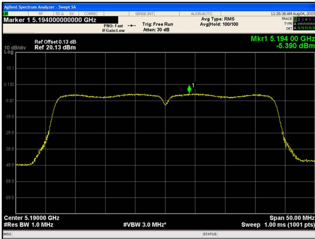
Figure 513. Maximum Power Spectral Density Chain B 802.11n HT40 (Ch. 38)
