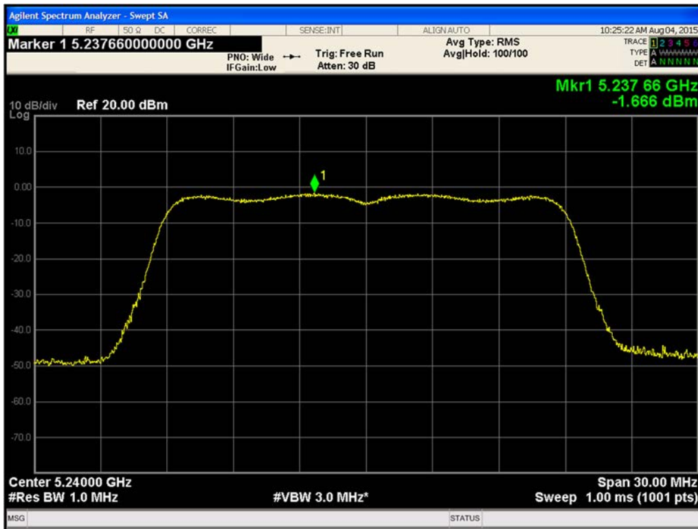
Figure 470. Maximum Power Spectral Density Chain B 802.11n HT20 (Ch. 48)
