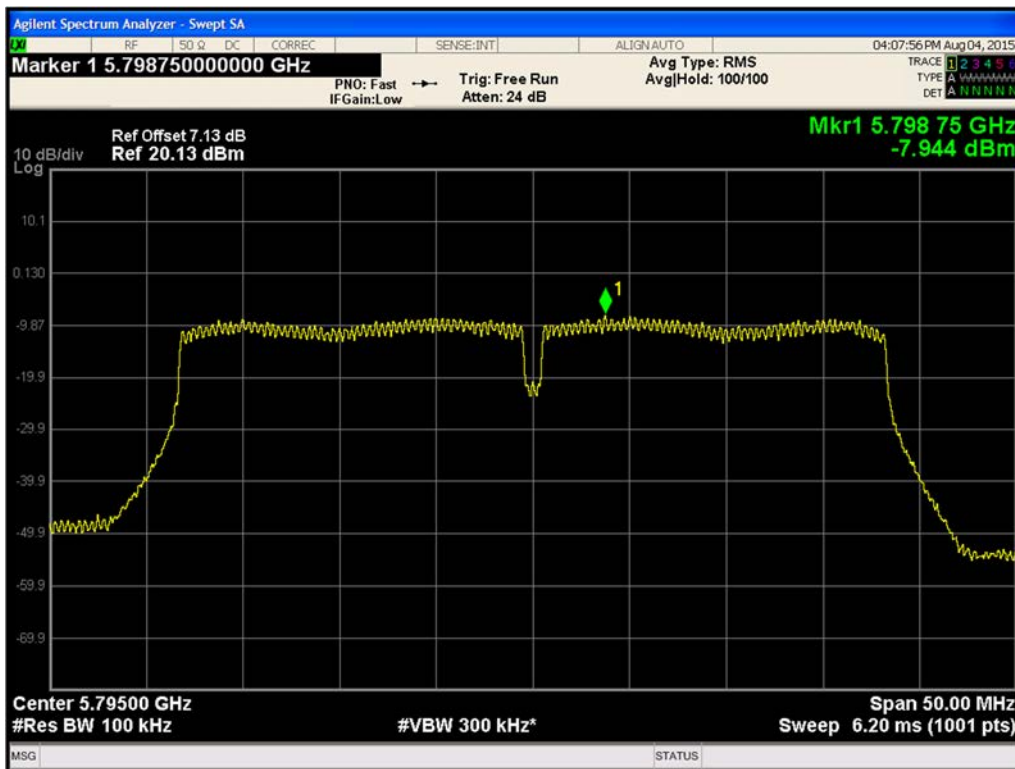
Figure 512. Maximum Power Spectral Density Chain A 802.11n HT40 (Ch. 159)
