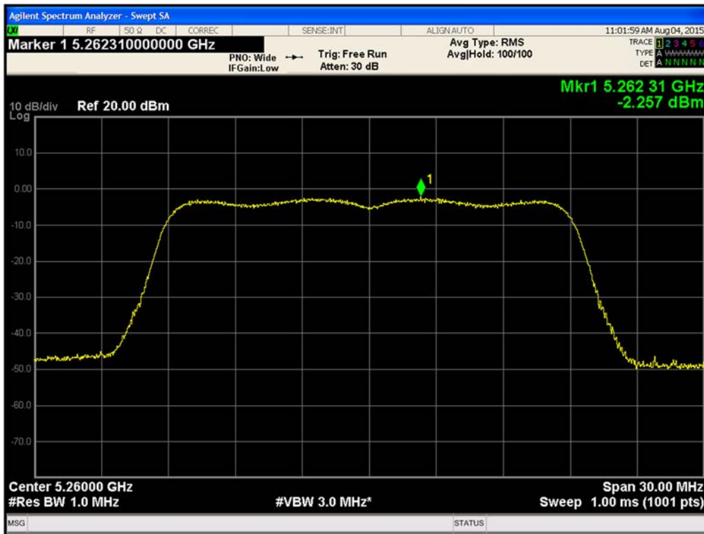
Figure 483. Maximum Power Spectral Density Chain A 802.11ac VHT20 (Ch. 52)
