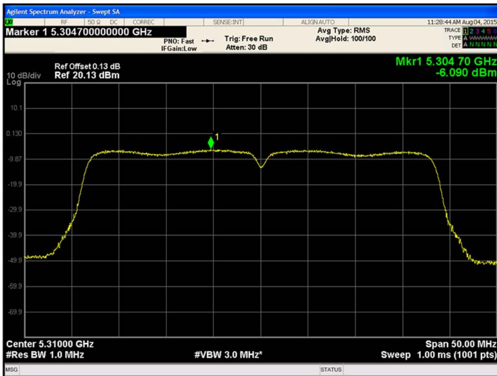
Figure 516. Maximum Power Spectral Density Chain B 802.11n HT40 (Ch. 62)
