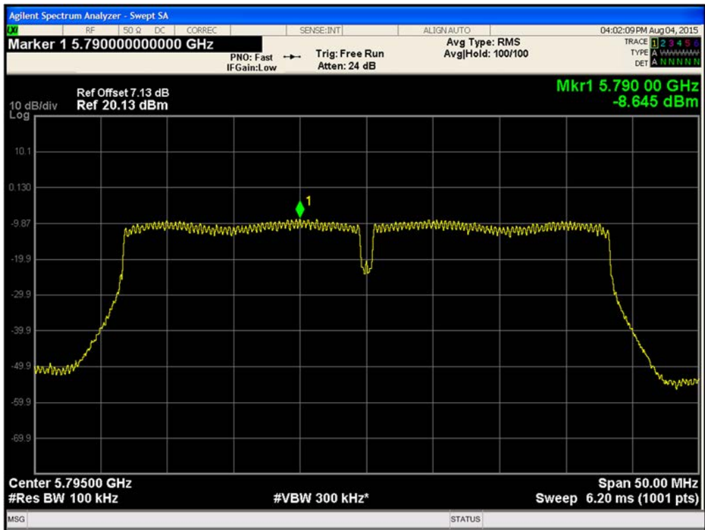
Figure 521. Maximum Power Spectral Density Chain B 802.11n HT40 (Ch. 159)
