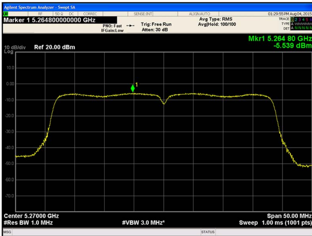
Figure 524. Maximum Power Spectral Density Chain A 802.11ac VHT40 (Ch. 54)
