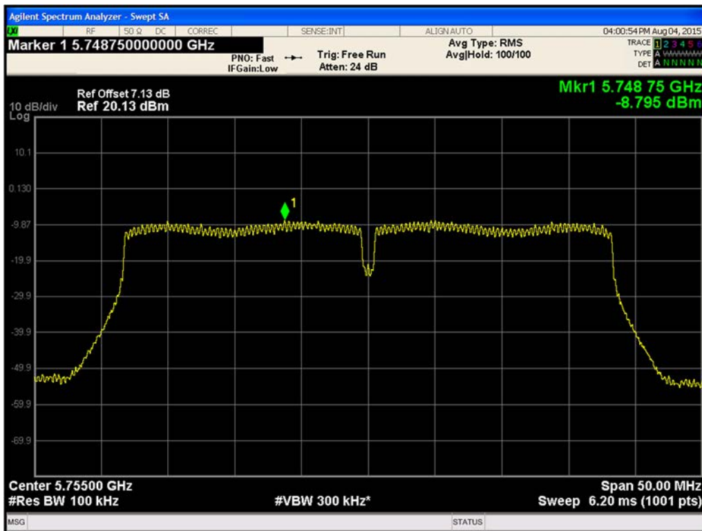
Figure 520. Maximum Power Spectral Density Chain B 802.11n HT40 (Ch. 151)
