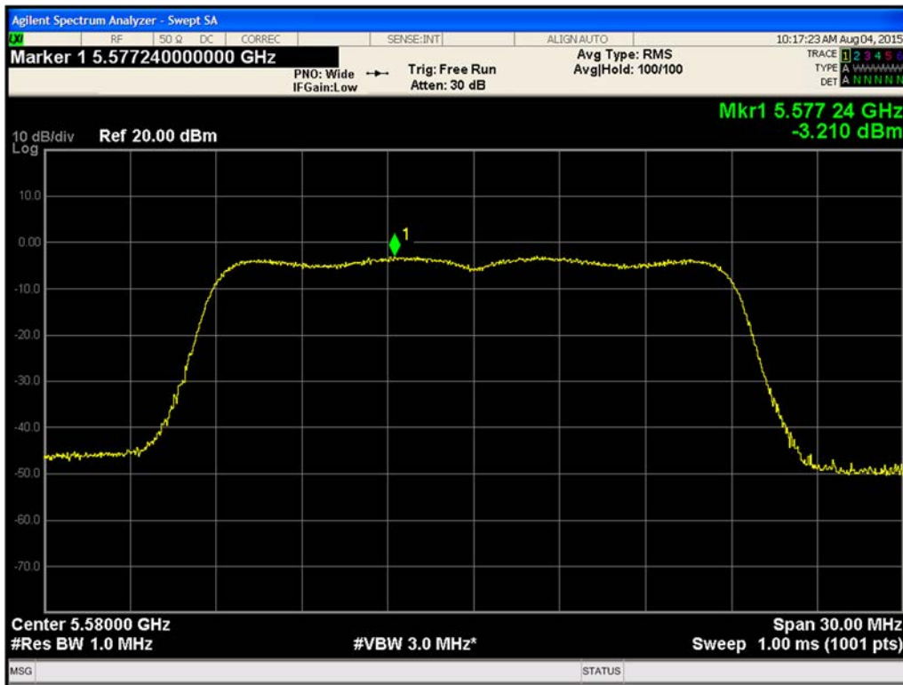
Figure 463. Maximum Power Spectral Density Chain A 802.11n HT20 (Ch. 116)
