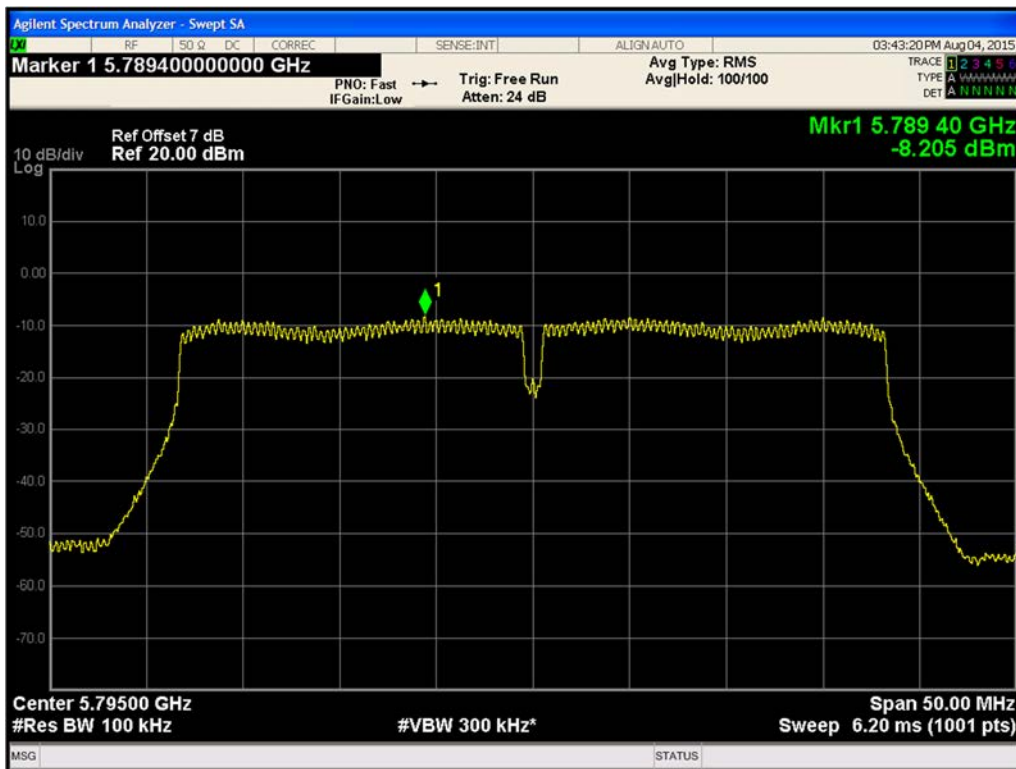
Figure 530. Maximum Power Spectral Density Chain A 802.11ac VHT40 (Ch. 159)
