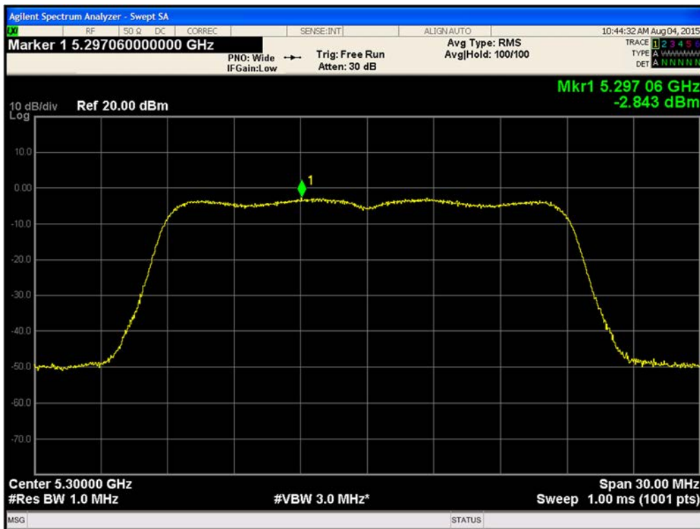
Figure 496. Maximum Power Spectral Density Chain B 802.11ac VHT20 (Ch. 60)
