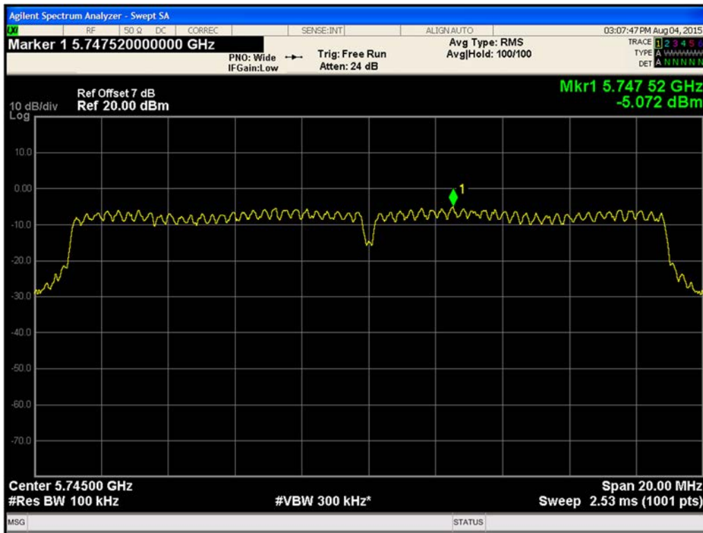
Figure 465. Maximum Power Spectral Density Chain A 802.1n HT20 (Ch. 149)
