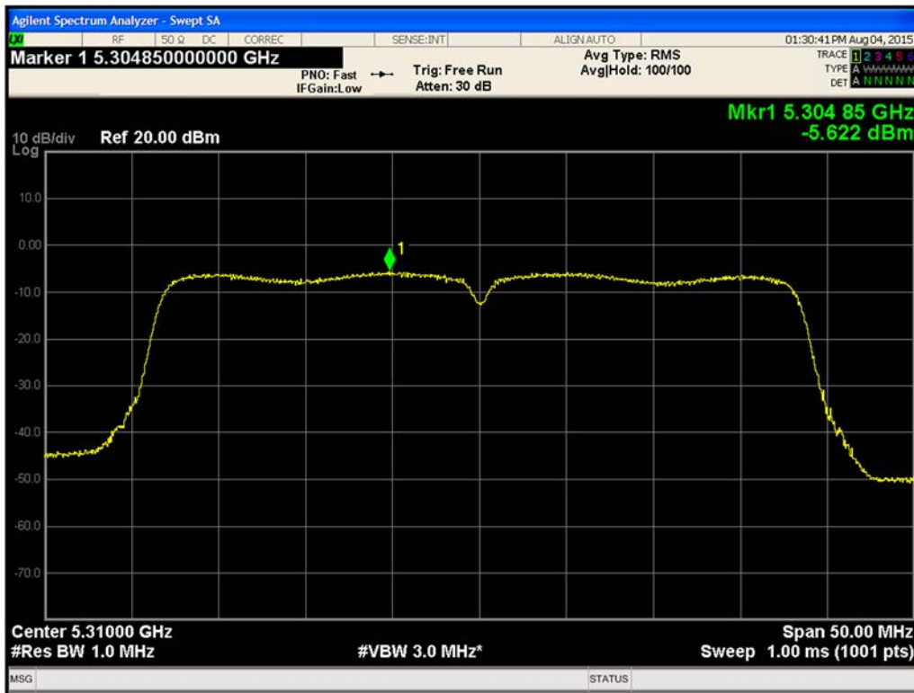
Figure 525. Maximum Power Spectral Density Chain A 802.11ac VHT40 (Ch.62)
