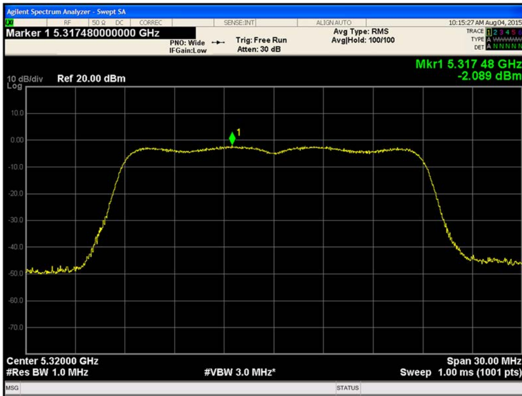
Figure 461. Maximum Power Spectral Density Chain A 802.11n HT20 (Ch. 64)
