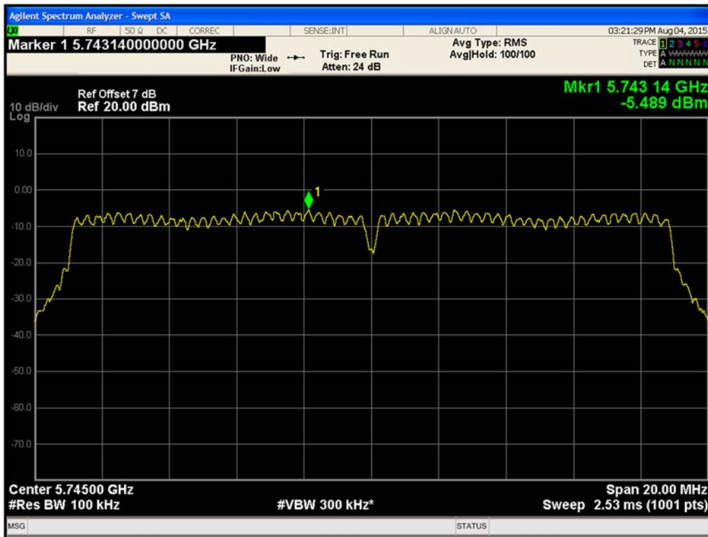
Figure 501. Maximum Power Spectral Density Chain B 802.11ac VHT20 (Ch. 149)
