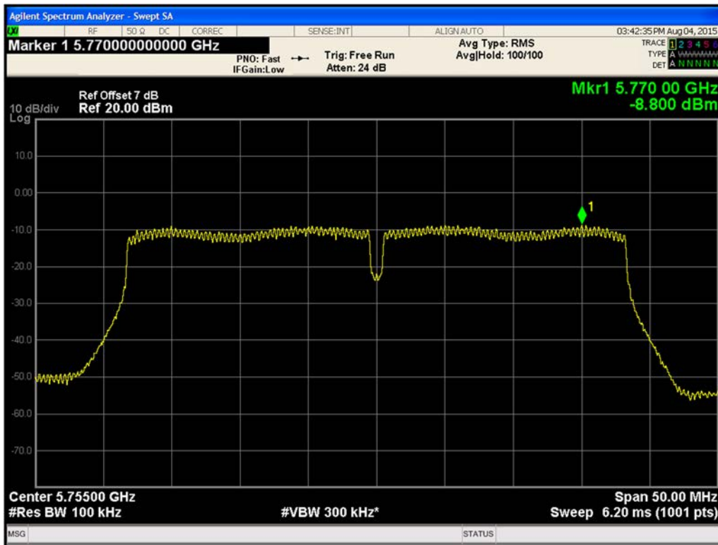
Figure 529. Maximum Power Spectral Density Chain A 802.11ac VHT40 (Ch. 151)
