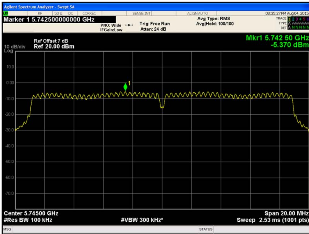
Figure 489. Maximum Power Spectral Density Chain A 802.11ac VHT20 (Ch. 149)
