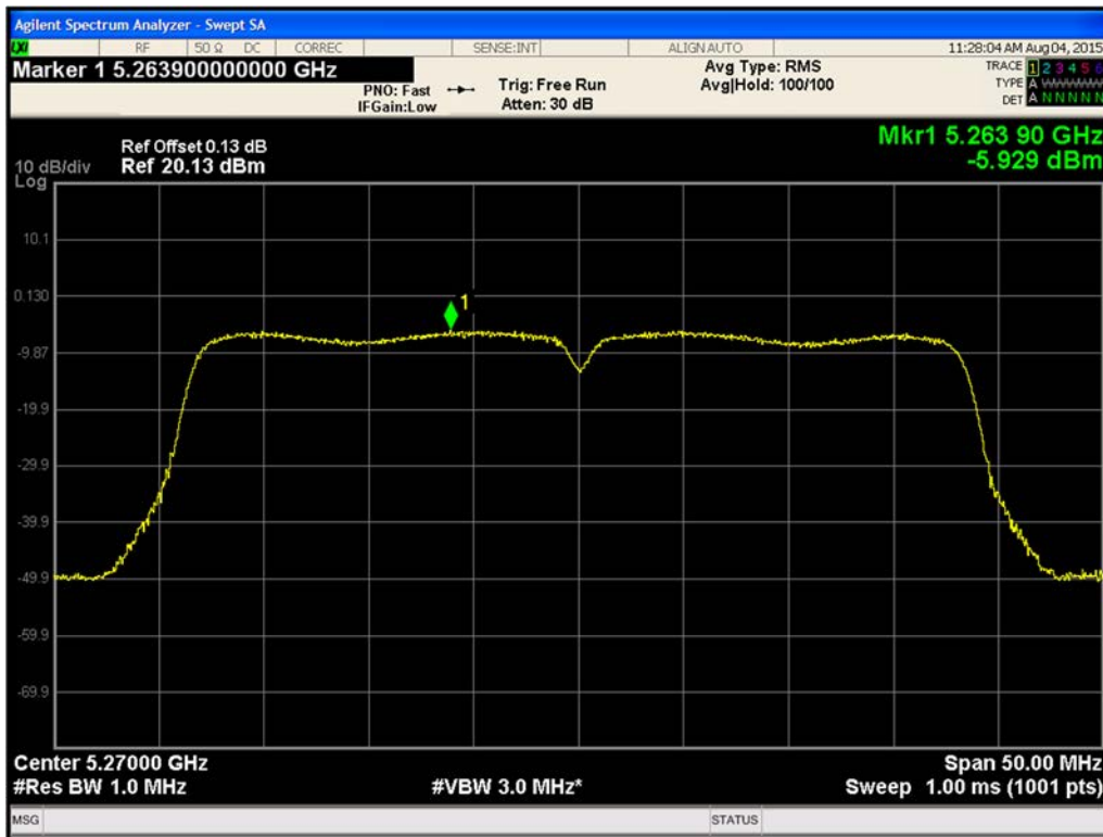
Figure 515. Maximum Power Spectral Density Chain B 802.11n HT40 (Ch. 54)
