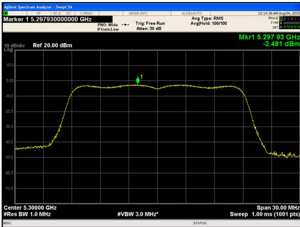
Figure 460. Maximum Power Spectral Density Chain A 802.11n HT20 (Ch. 60)
