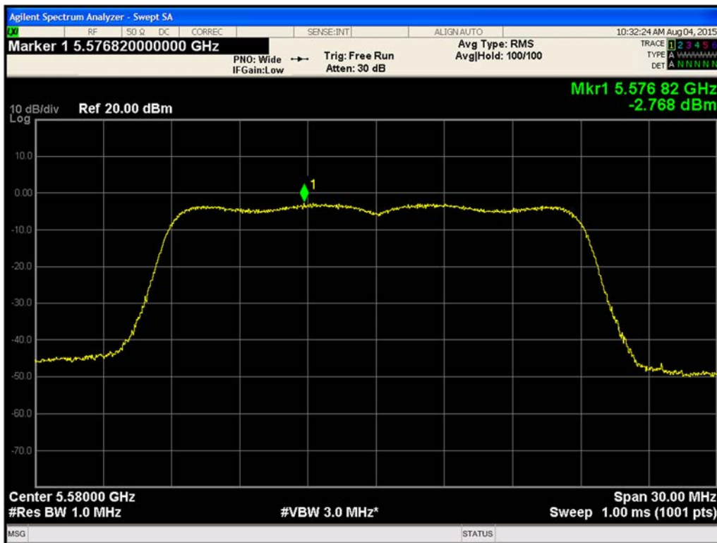
Figure 475. Maximum Power Spectral Density Chain B 802.11n HT20 (Ch. 116)
