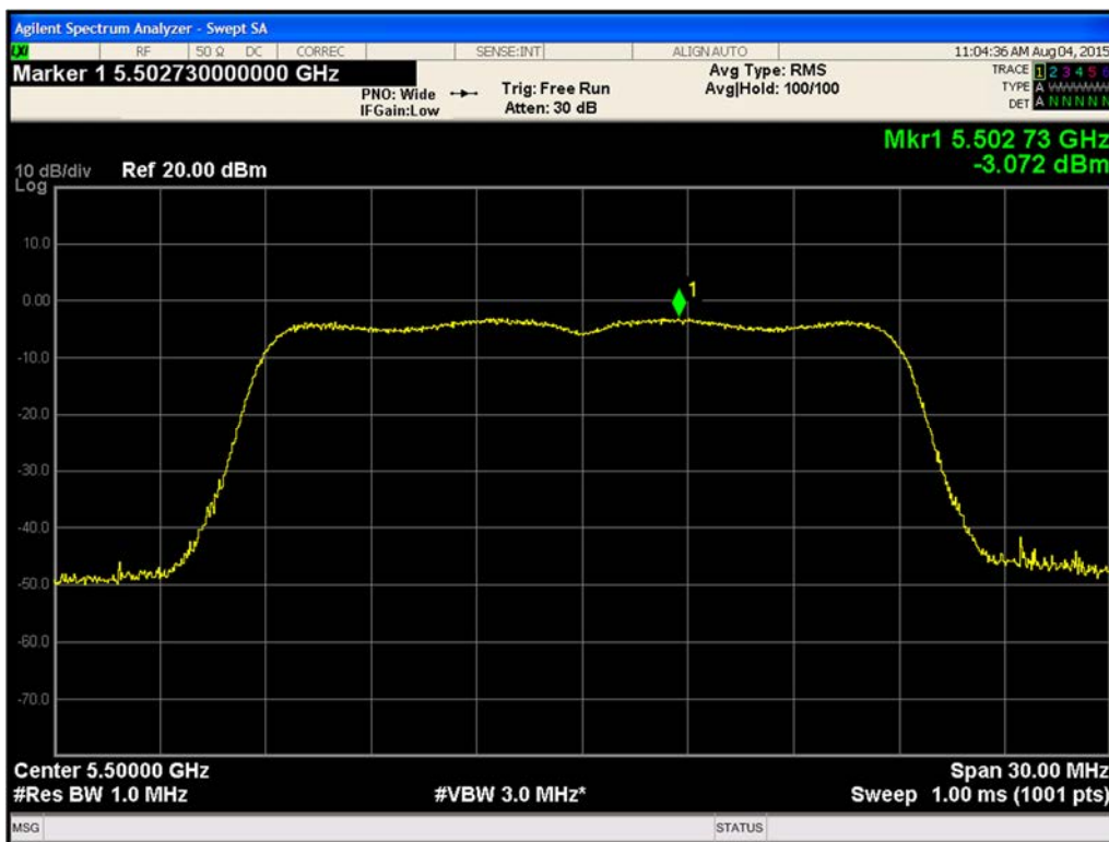
Figure 486. Maximum Power Spectral Density Chain A 802.11ac VHT20 (Ch. 100)
