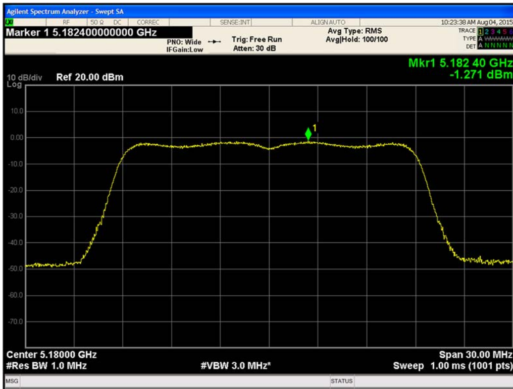
Figure 468. Maximum Power Spectral Density Chain B 802.11n HT20 (Ch. 36)
