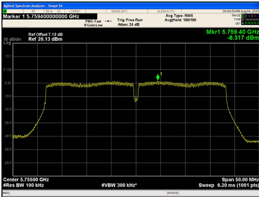
Figure 511. Maximum Power Spectral Density Chain A 802.11n HT40 (Ch. 151)
