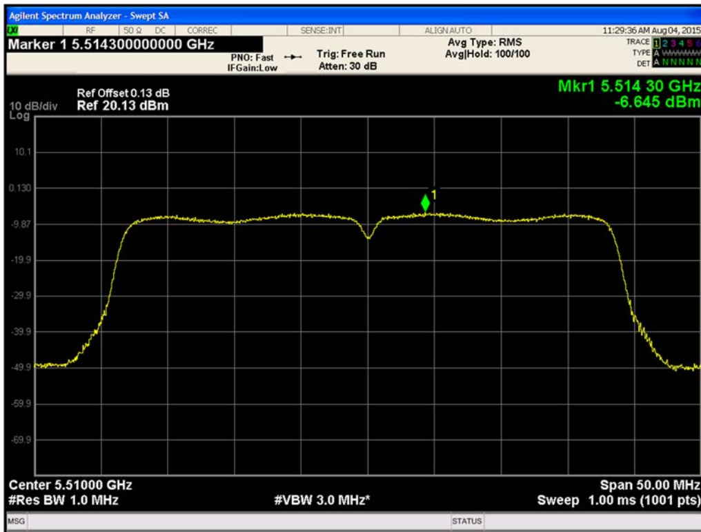
Figure 517. Maximum Power Spectral Density Chain B 802.11n HT40 (Ch. 102)
