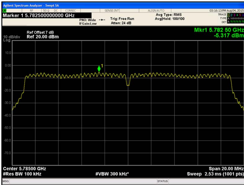
Figure 478. Maximum Power Spectral Density Chain B 802.11n HT20 (Ch. 157)
