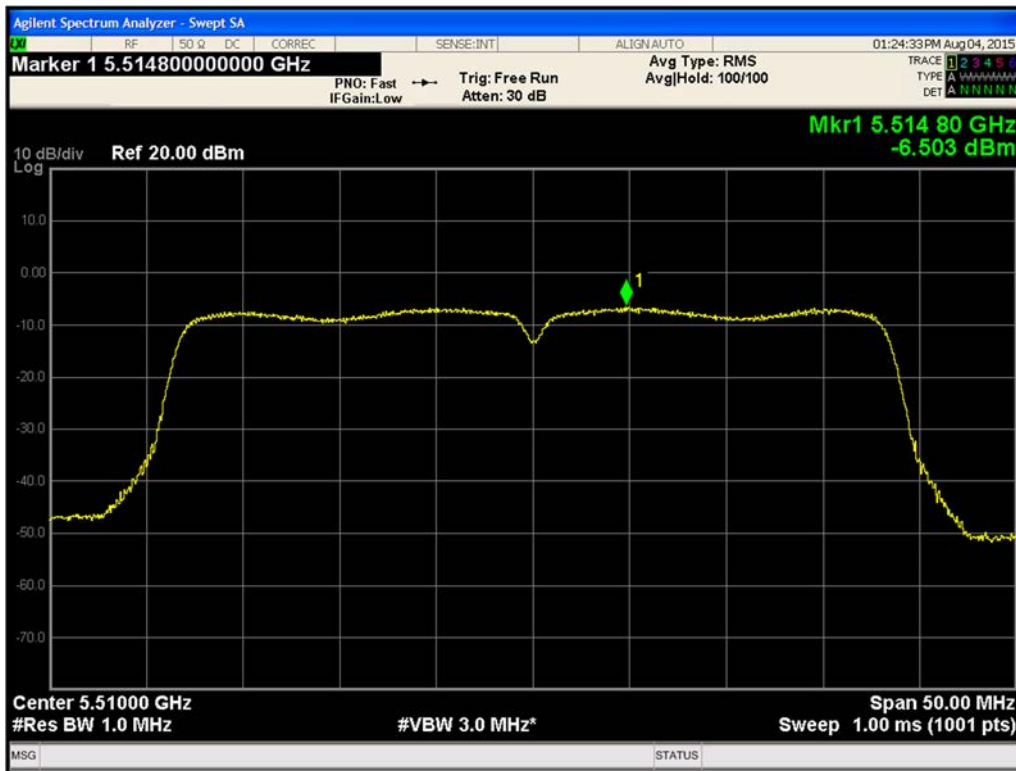
Figure 535. Maximum Power Spectral Density Chain B 802.11ac VHT40 (Ch. 102)
