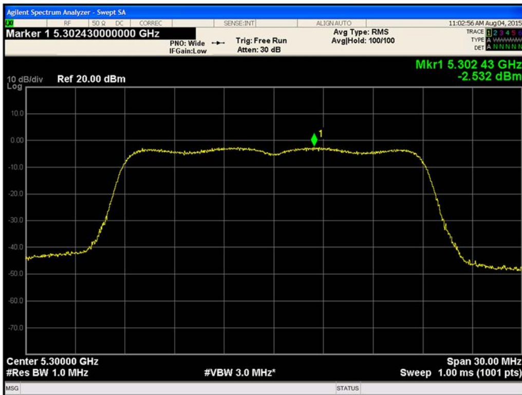
Figure 484. Maximum Power Spectral Density Chain A 802.11ac VHT20 (Ch. 60)
