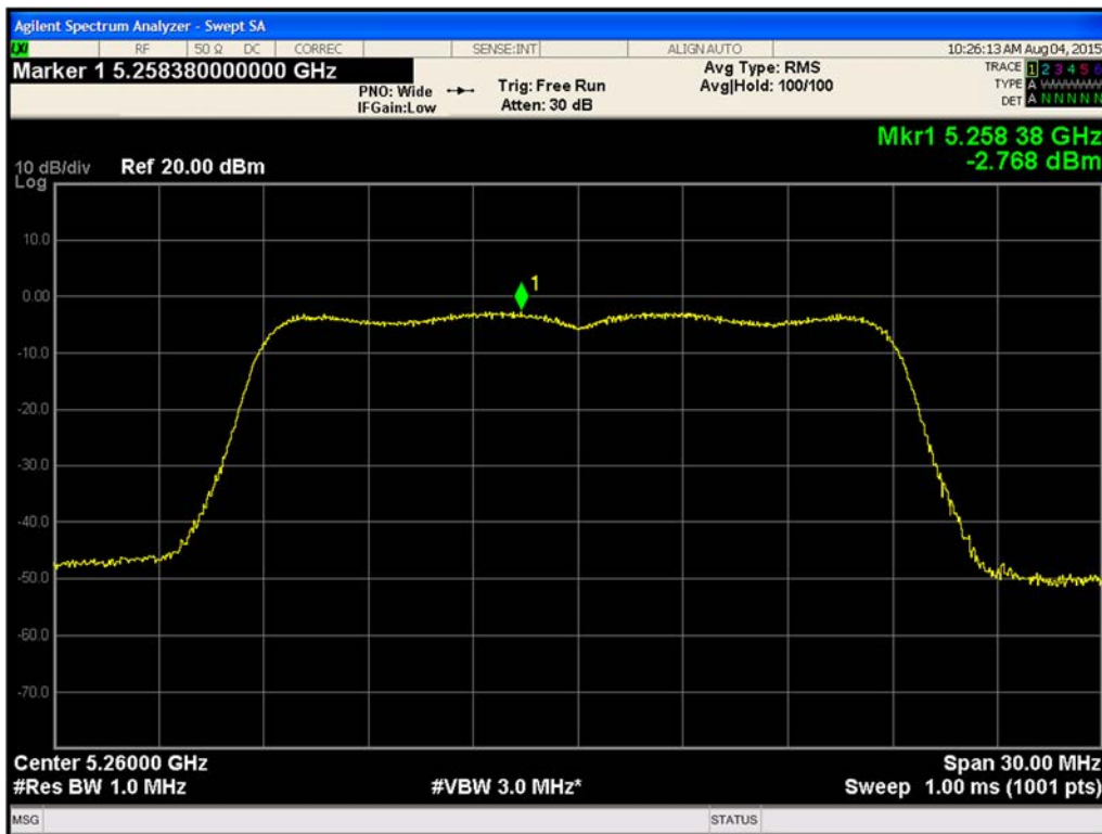
Figure 471. Maximum Power Spectral Density Chain B 802.11n HT20 (Ch. 52)
