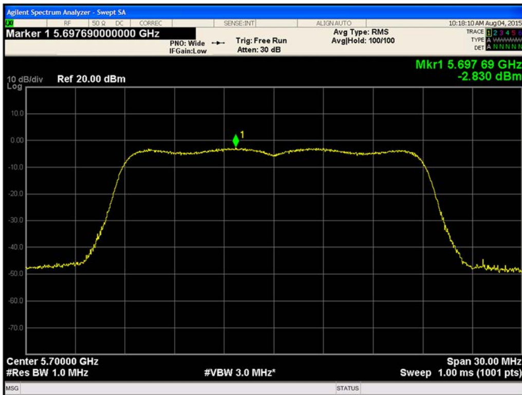
Figure 464. Maximum Power Spectral Density Chain A 802.11n HT20 (Ch. 140)
