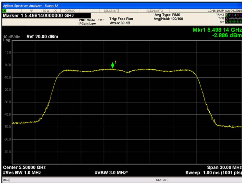
Figure 498. Maximum Power Spectral Density Chain B 802.11ac VHT20 (Ch. 100)
