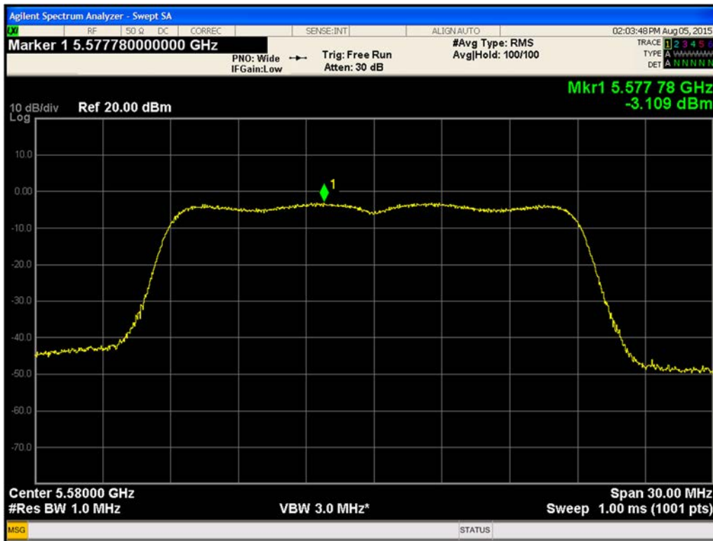
Figure 487. Maximum Power Spectral Density Chain A 802.11ac VHT20 (Ch. 116)
