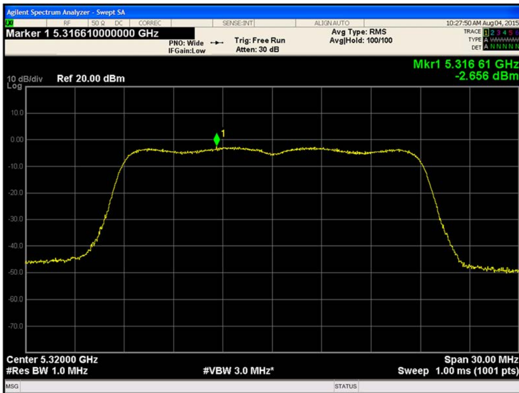
Figure 473. Maximum Power Spectral Density Chain B 802.11n HT20 (Ch. 64)
