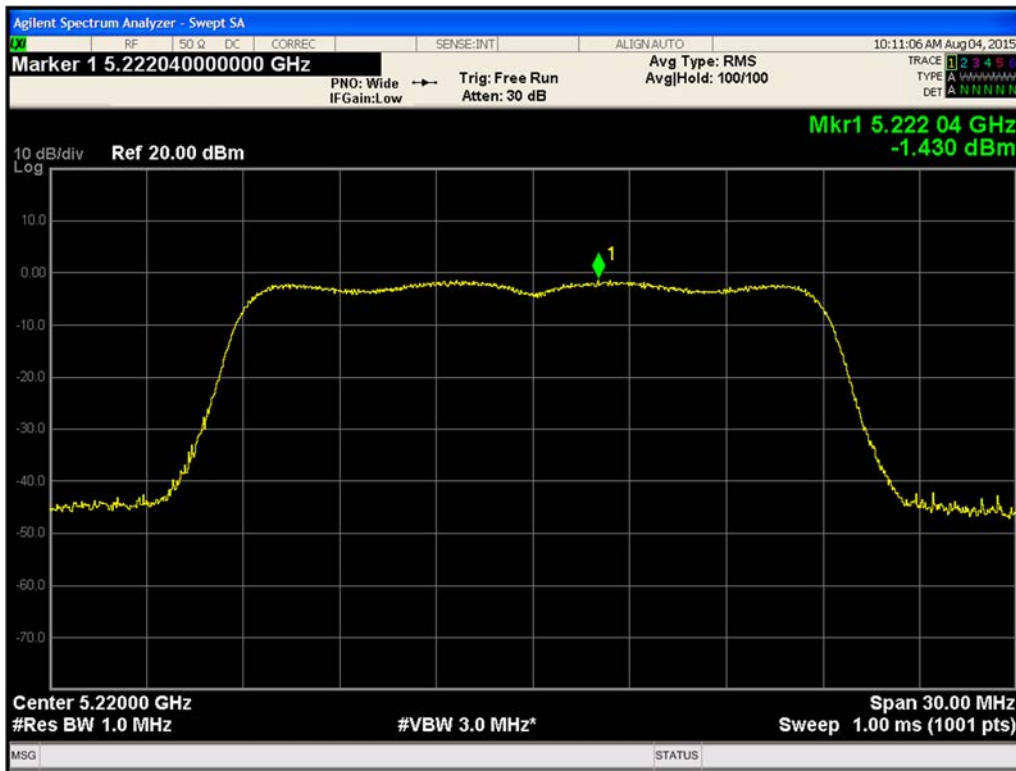
Figure 457. Maximum Power Spectral Density Chain A 802.11n HT20 (Ch. 44)
