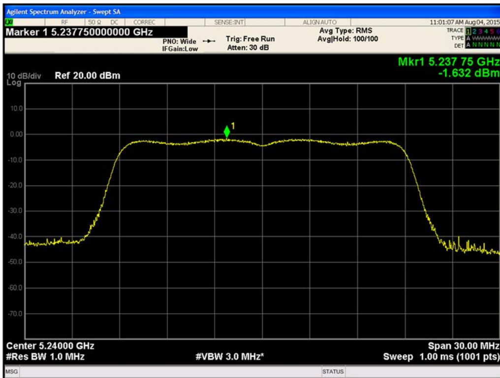
Figure 482. Maximum Power Spectral Density Chain A 802.11ac VHT20 (Ch. 48)
