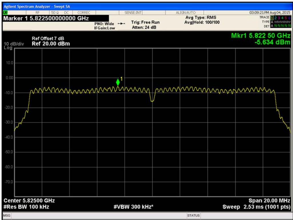
Figure 467. Maximum Power Spectral Density Chain A 802.11n HT20 (Ch. 165)
