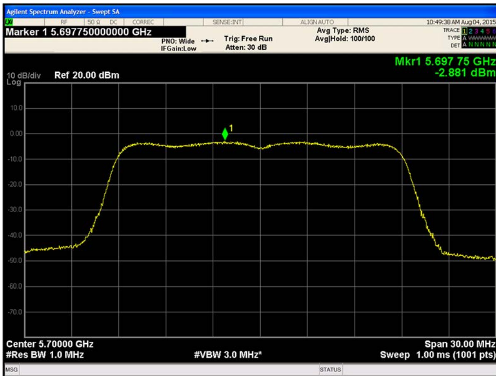
Figure 500. Maximum Power Spectral Density Chain B 802.11ac VHT20 (Ch. 140)
