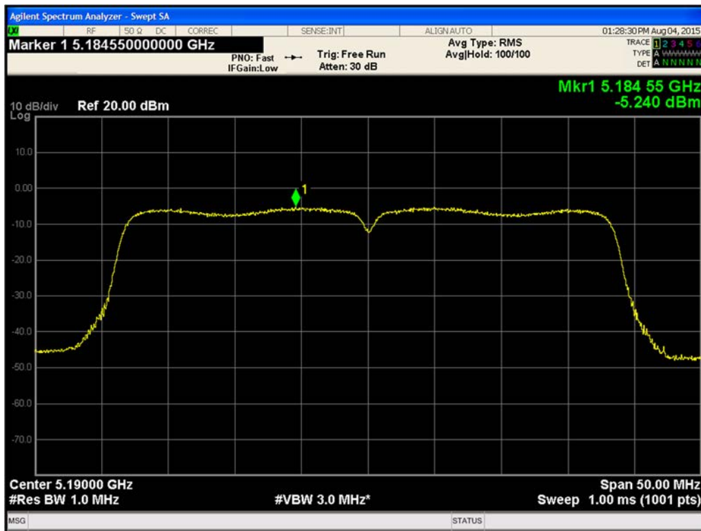
Figure 522. Maximum Power Spectral Density Chain A 802.11ac VHT40 (Ch. 38)
