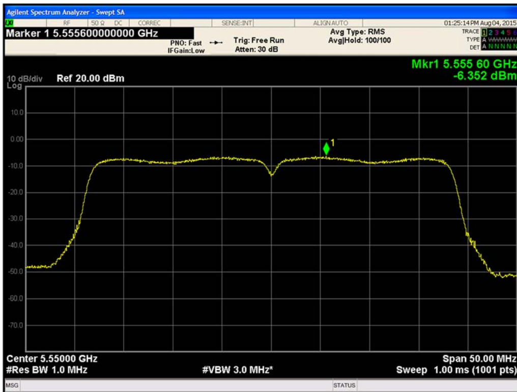
Figure 536. Maximum Power Spectral Density Chain B 802.11ac VHT40 (Ch. 110)
