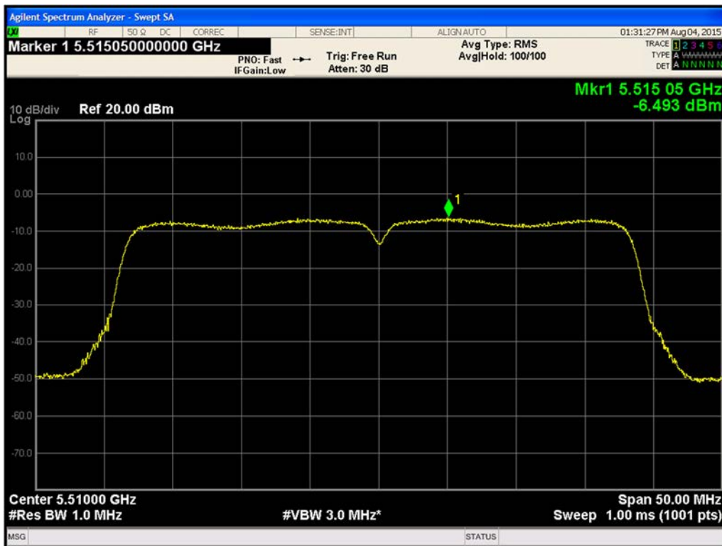
Figure 526. Maximum Power Spectral Density Chain A 802.11ac VHT40 (Ch. 102)
