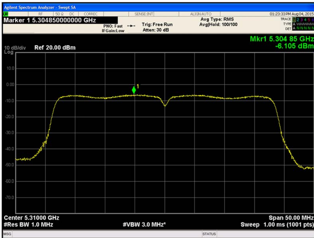
Figure 534. Maximum Power Spectral Density Chain B 802.11ac VHT40 (Ch. 62)
