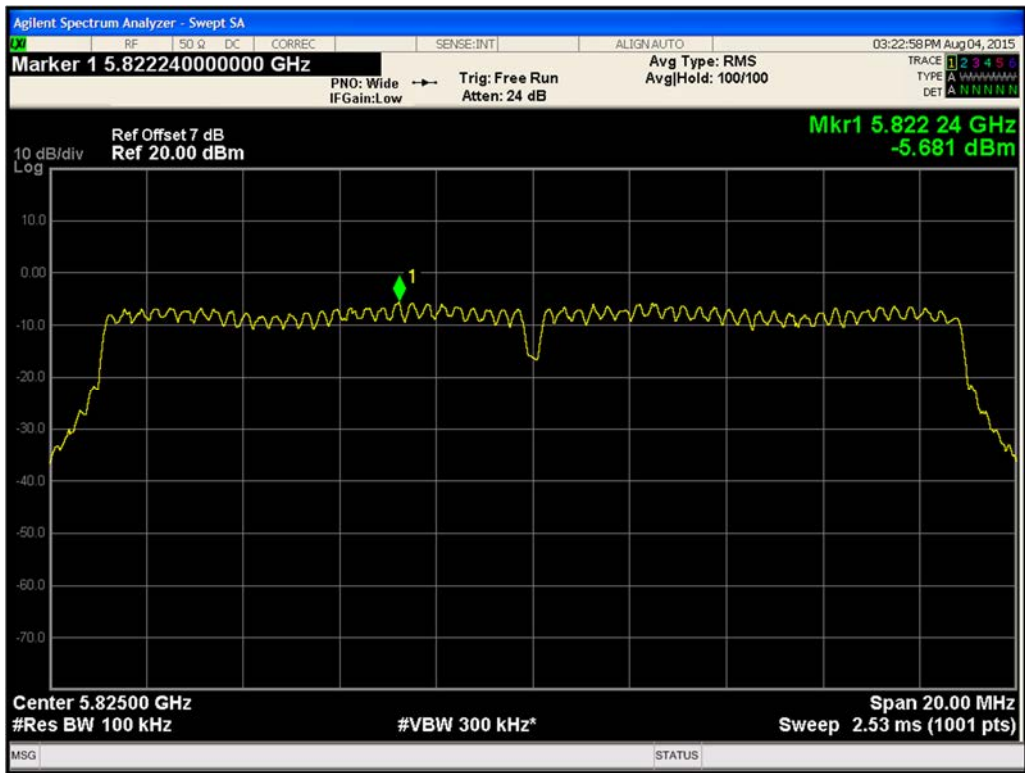
Figure 503. Maximum Power Spectral Density Chain B 802.11ac VHT20 (Ch. 165)
