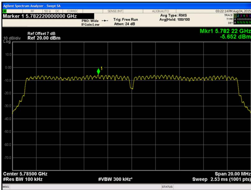
Figure 502. Maximum Power Spectral Density Chain B 802.11ac VHT20 (Ch. 157)
