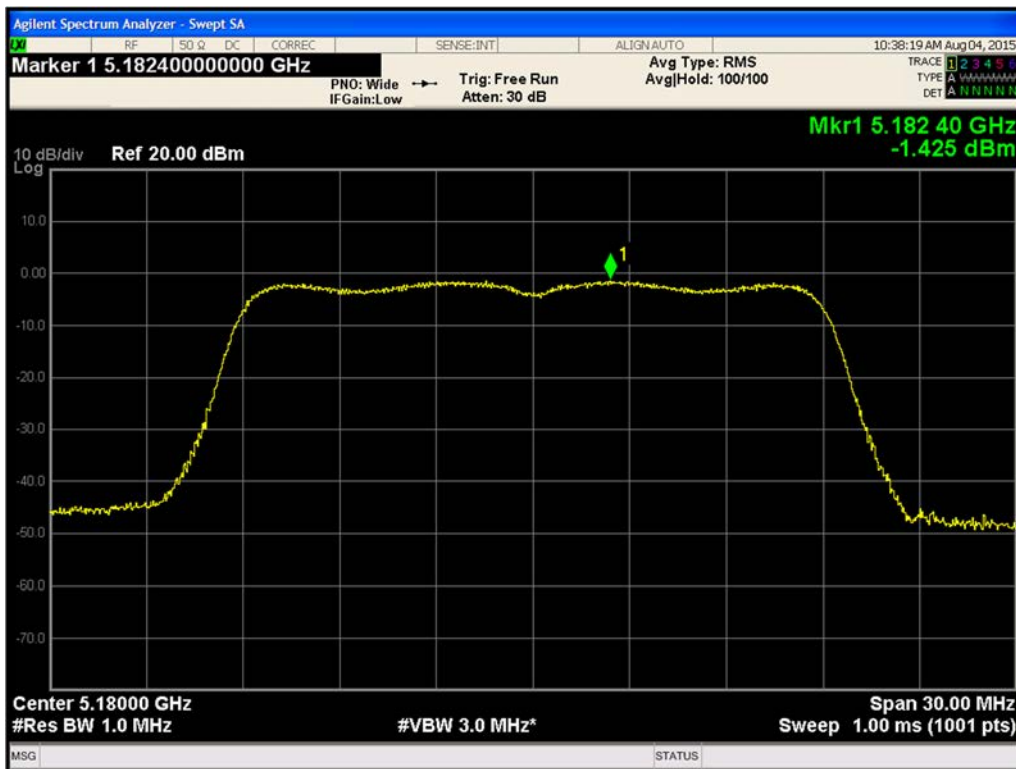
Figure 492. Maximum Power Spectral Density Chain B 802.11ac VHT20 (Ch. 36)
