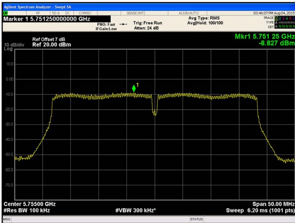
Figure 538. Maximum Power Spectral Density Chain B 802.11ac VHT40 (Ch. 151)
