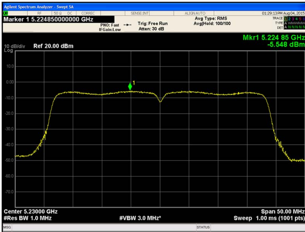
Figure 523. Maximum Power Spectral Density Chain A 802.11ac VHT40 (Ch. 46)
