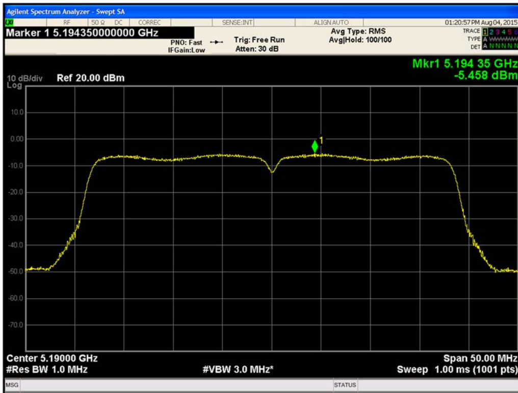
Figure 531. Maximum Power Spectral Density Chain B 802.11ac VHT40 (Ch. 38)
