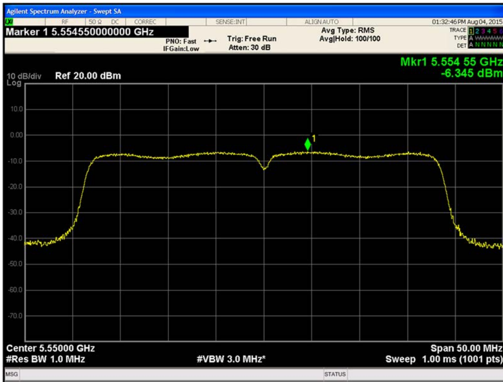
Figure 527. Maximum Power Spectral Density Chain A 802.11ac VHT40 (Ch. 110)
