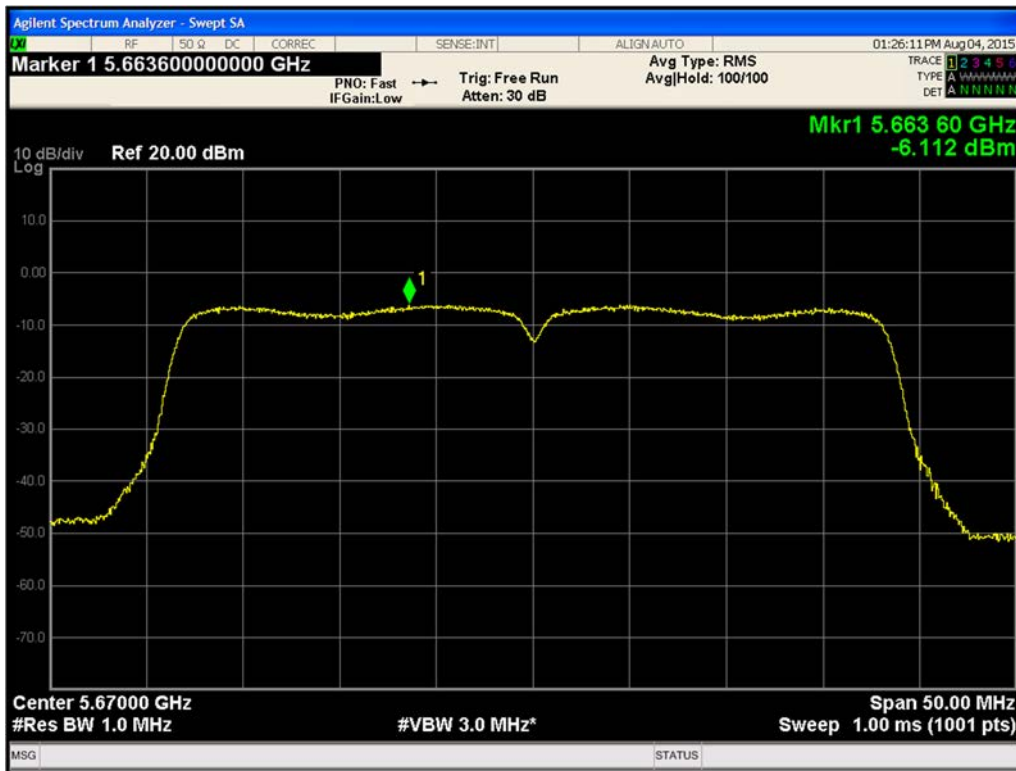
Figure 537. Maximum Power Spectral Density Chain B 802.11ac VHT40 (Ch. 134)
