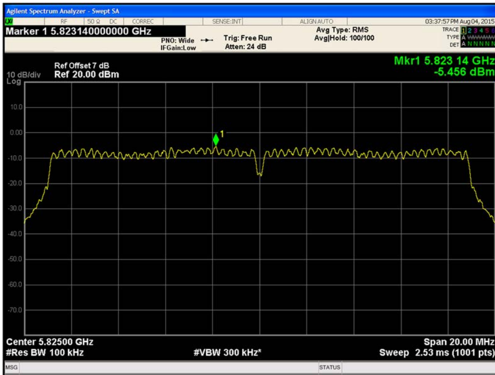
Figure 491. Maximum Power Spectral Density Chain A 802.11ac VHT20 (Ch. 165)
