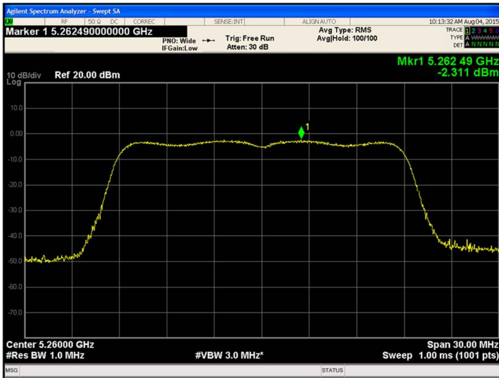
Figure 459. Maximum Power Spectral Density Chain A 802.11n HT20 (Ch. 52)
