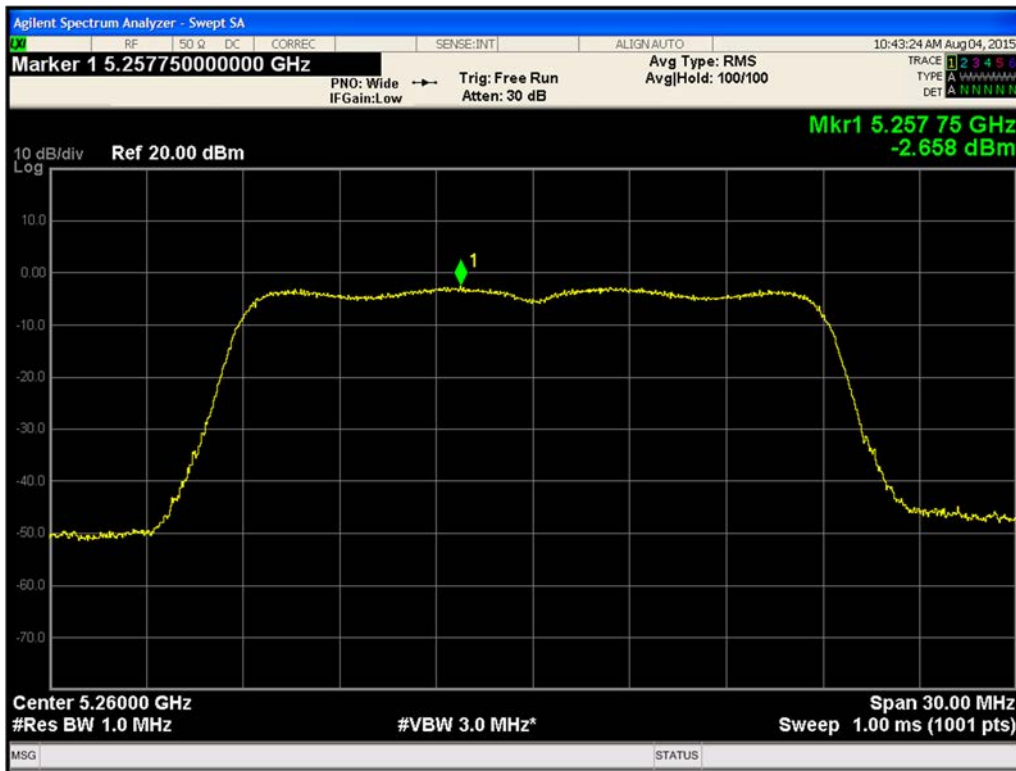
Figure 495. Maximum Power Spectral Density Chain B 802.11ac VHT20 (Ch. 52)
