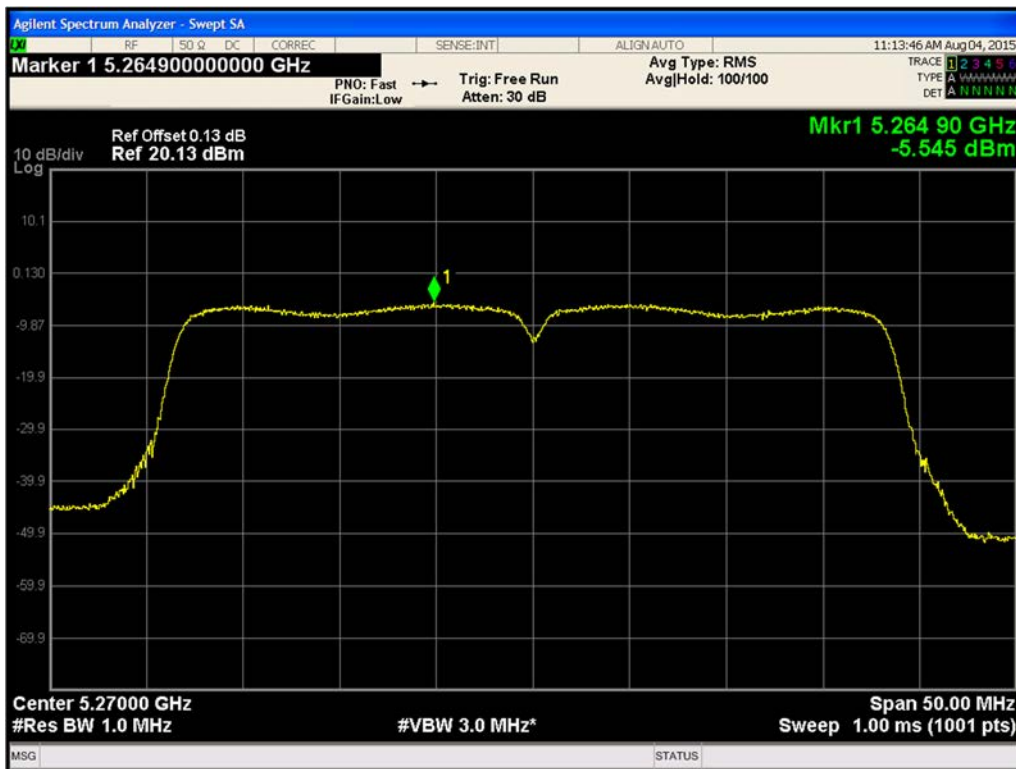
Figure 506. Maximum Power Spectral Density Chain A 802.11n HT40 (Ch. 54)
