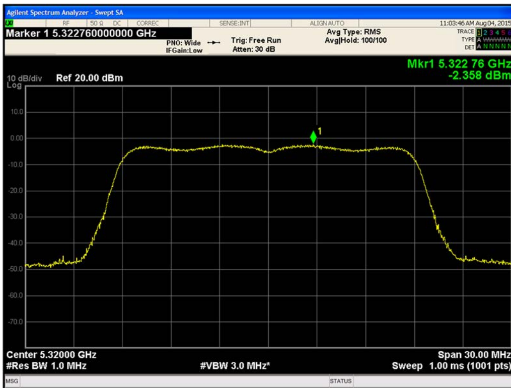
Figure 485. Maximum Power Spectral Density Chain A 802.11ac VHT20 (Ch. 64)
