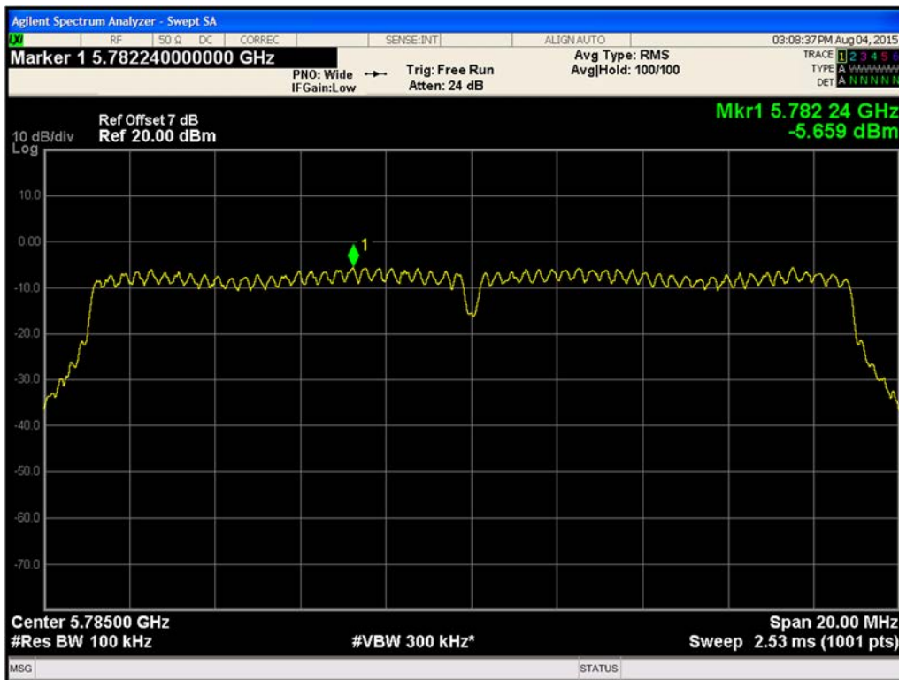
Figure 466. Maximum Power Spectral Density Chain A 802.11n HT20 (Ch. 157)
