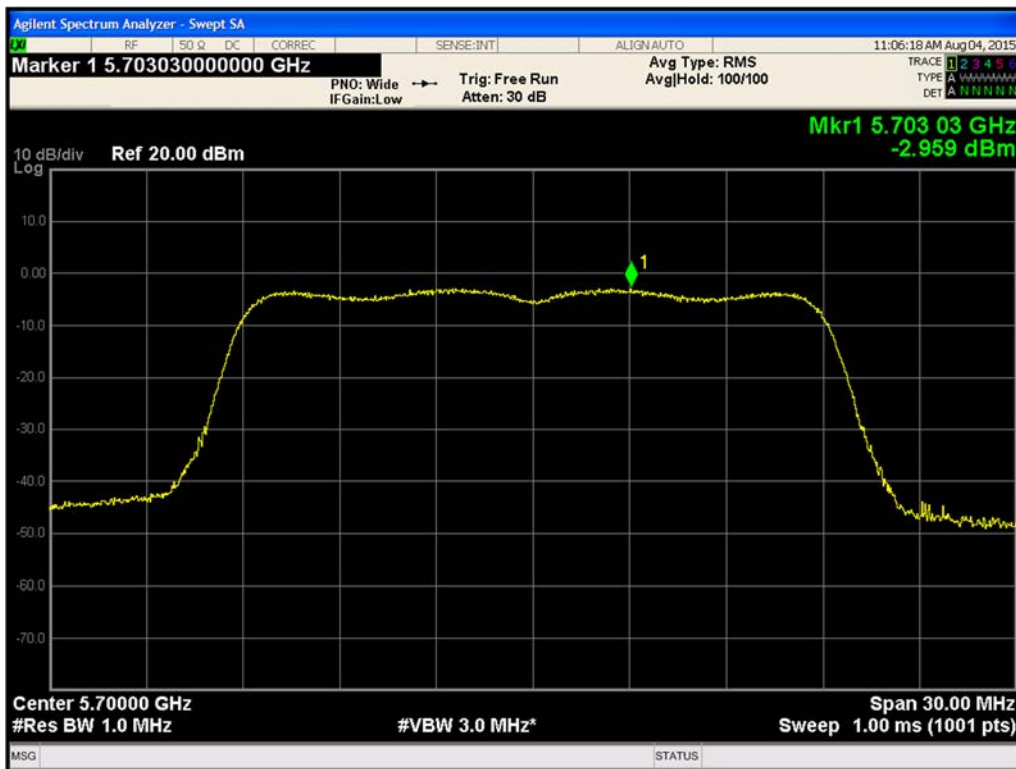
Figure 488. Maximum Power Spectral Density Chain A 802.11ac VHT20 (Ch. 140)
