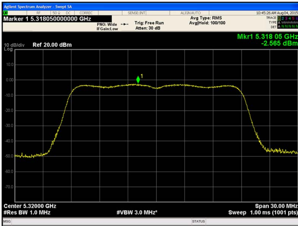
Figure 497. Maximum Power Spectral Density Chain B 802.11ac VHT20 (Ch. 64)
