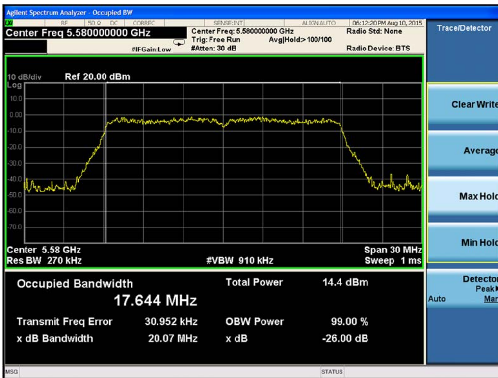
Figure 9-177. 99% Occupied Bandwidth Chain B 802.11n HT20 (Ch. 116)
