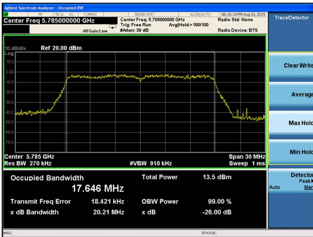
Figure 9-181. 99% Occupied Bandwidth Chain B 802.11n HT20 (Ch. 157)
