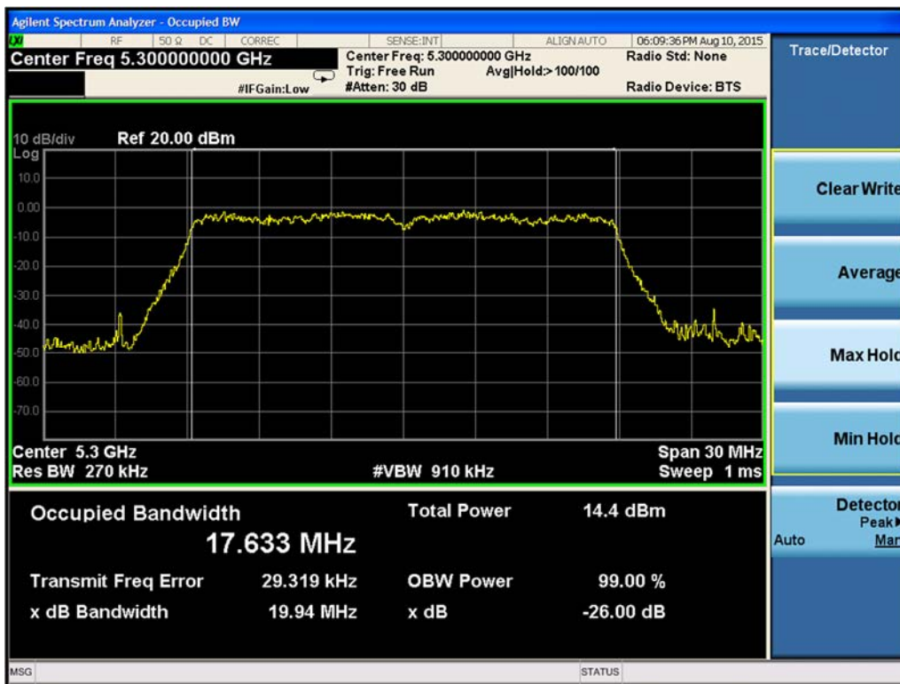
Figure 9-174. 99% Occupied Bandwidth Chain B 802.11n HT20 (Ch. 60)
