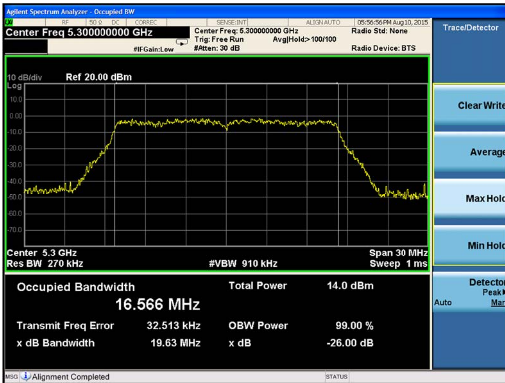
Figure 9-148. 99% Occupied Bandwidth Chain B 802.11a (Ch. 60)
