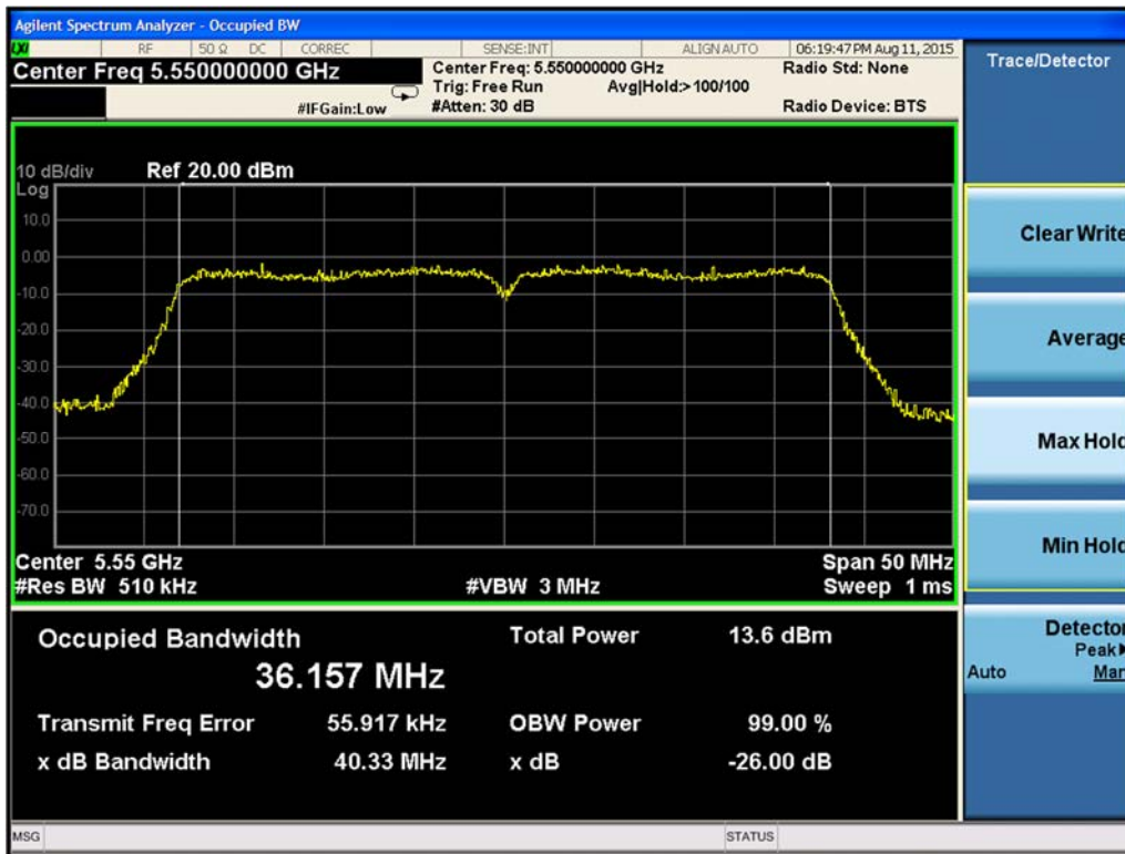
Figure 9-214. 99% Occupied Bandwidth Chain A 802.11n HT40 (Ch. 110)
