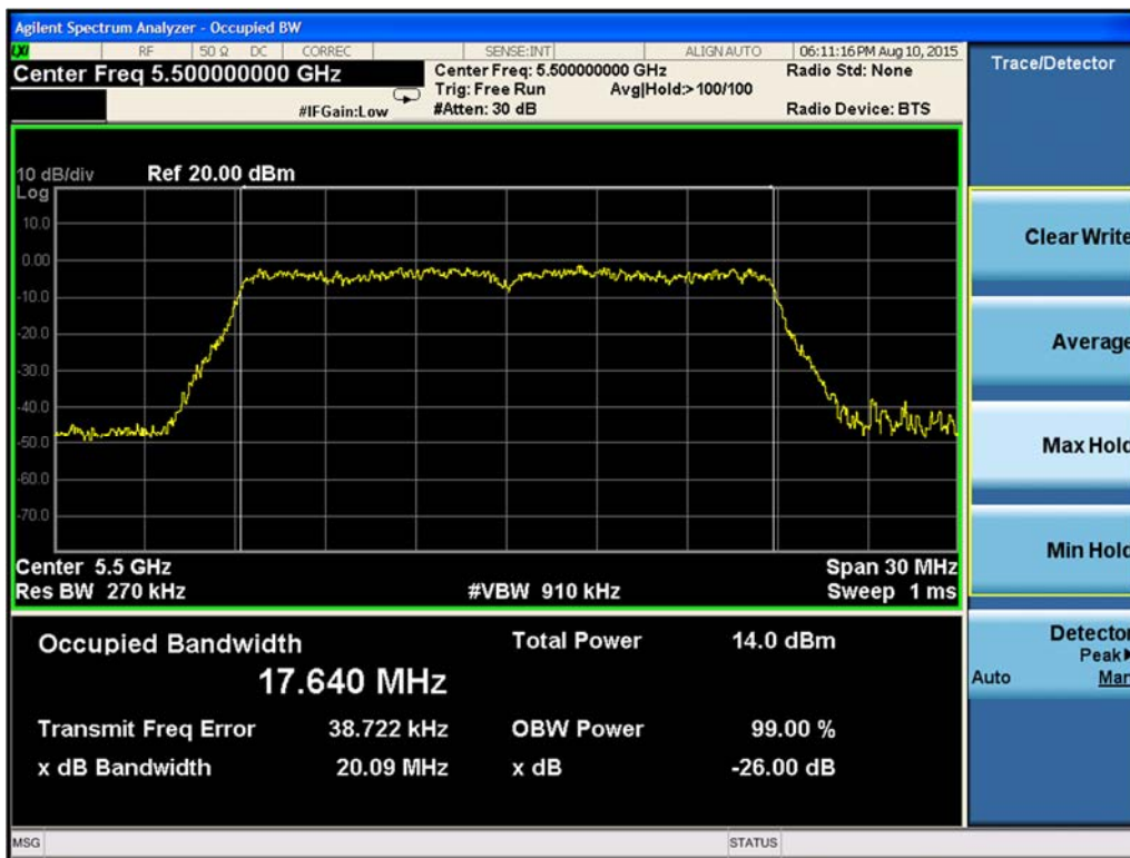
Figure 9-176. 99% Occupied Bandwidth Chain B 802.11n HT20 (Ch. 100)
