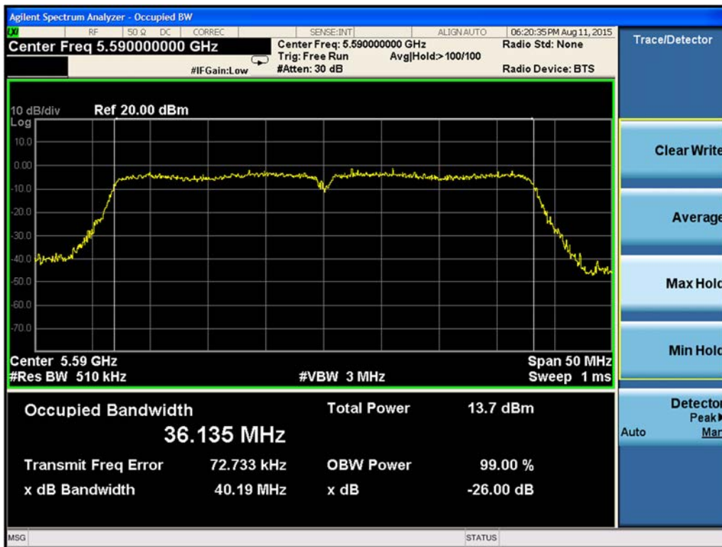
Figure 9-215. 99% Occupied Bandwidth Chain A 802.11n HT40 (Ch. 118)
