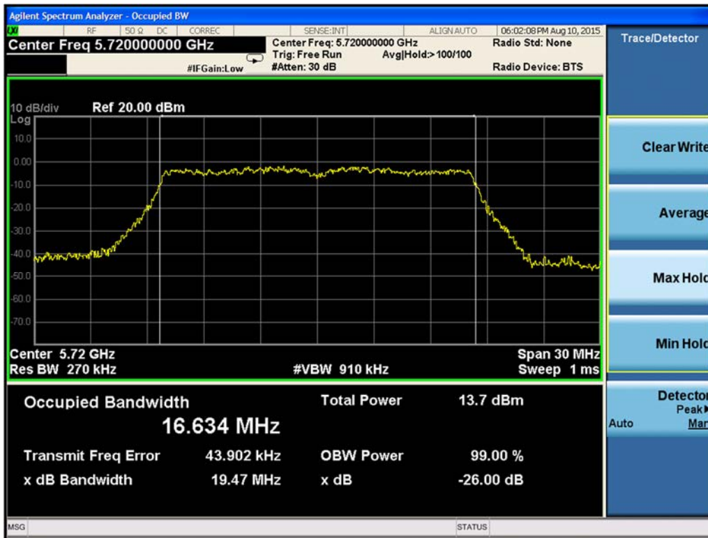
Figure 9-153. 99% Occupied Bandwidth Chain B 802.11a (Ch. 144)
