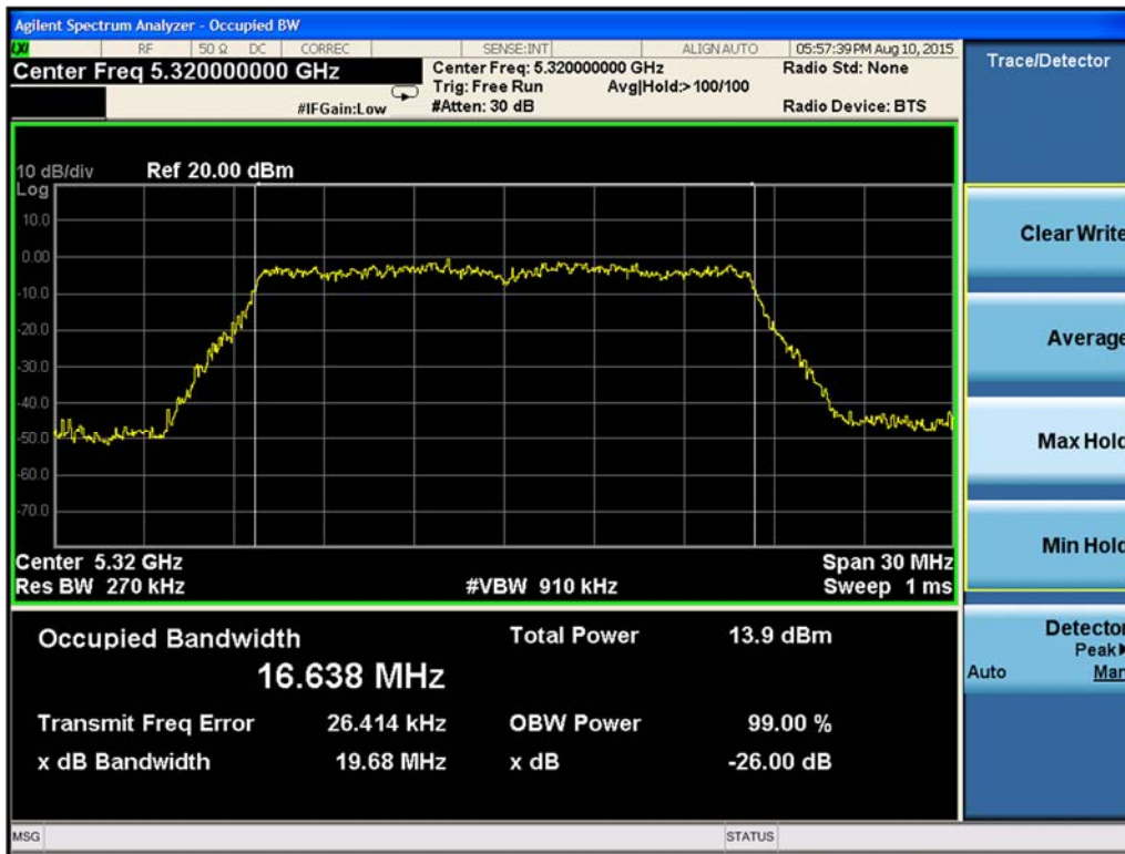
Figure 9-149. 99% Occupied Bandwidth Chain B 802.11a (Ch. 64)
