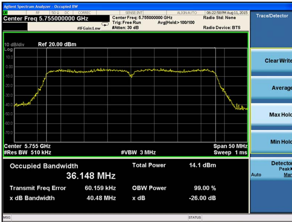
Figure 9-218. 99% Occupied Bandwidth Chain A 802.11n HT40 (Ch. 151)
