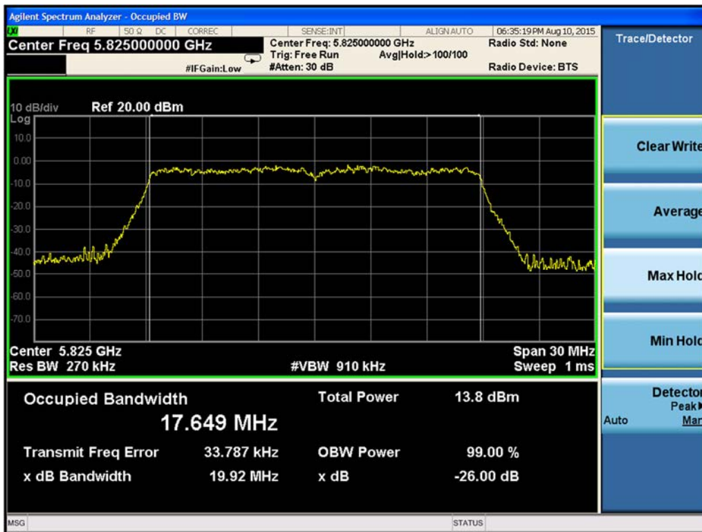
Figure 9-208. 99% Occupied Bandwidth Chain B 802.11ac VHT20 (Ch. 165)
