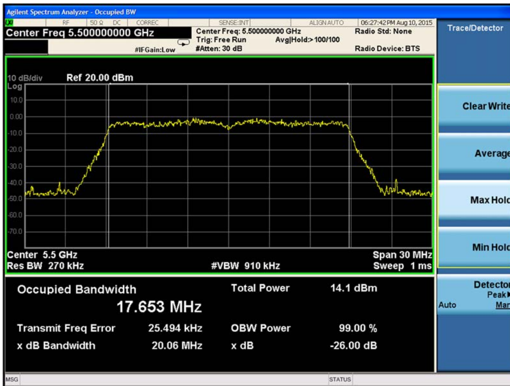
Figure 9-202. 99% Occupied Bandwidth Chain B 802.11ac VHT20 (Ch. 100)
