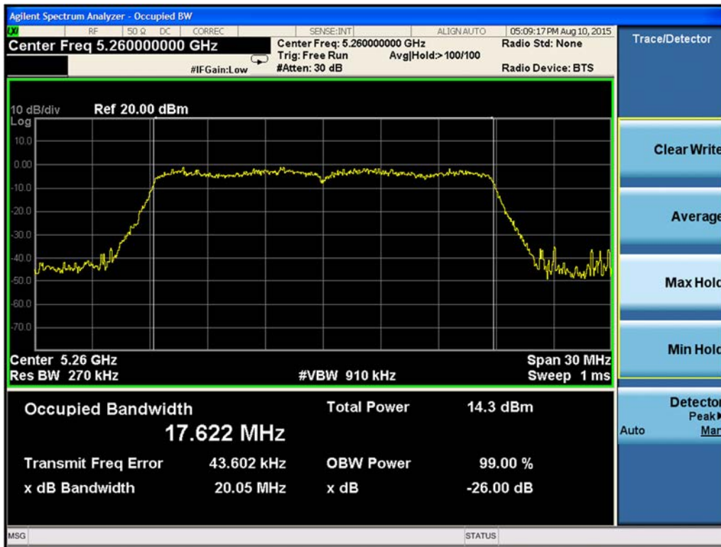
Figure 9-186. 99% Occupied Bandwidth Chain A 802.11ac VHT20 (Ch. 52)
