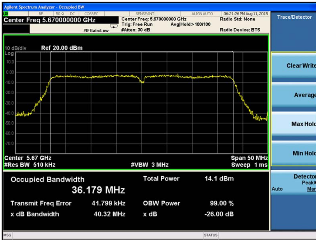
Figure 9-216. 99% Occupied Bandwidth Chain A 802.11n HT40 (Ch. 134)
