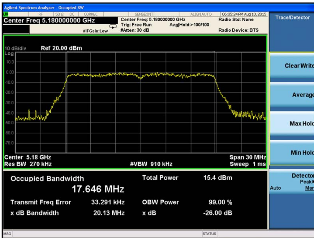
Figure 9-170. 99% Occupied Bandwidth Chain B 802.11n HT20 (Ch. 36)
