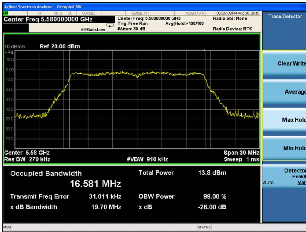
Figure 9-151. 99% Occupied Bandwidth Chain B 802.11a (Ch. 116)
