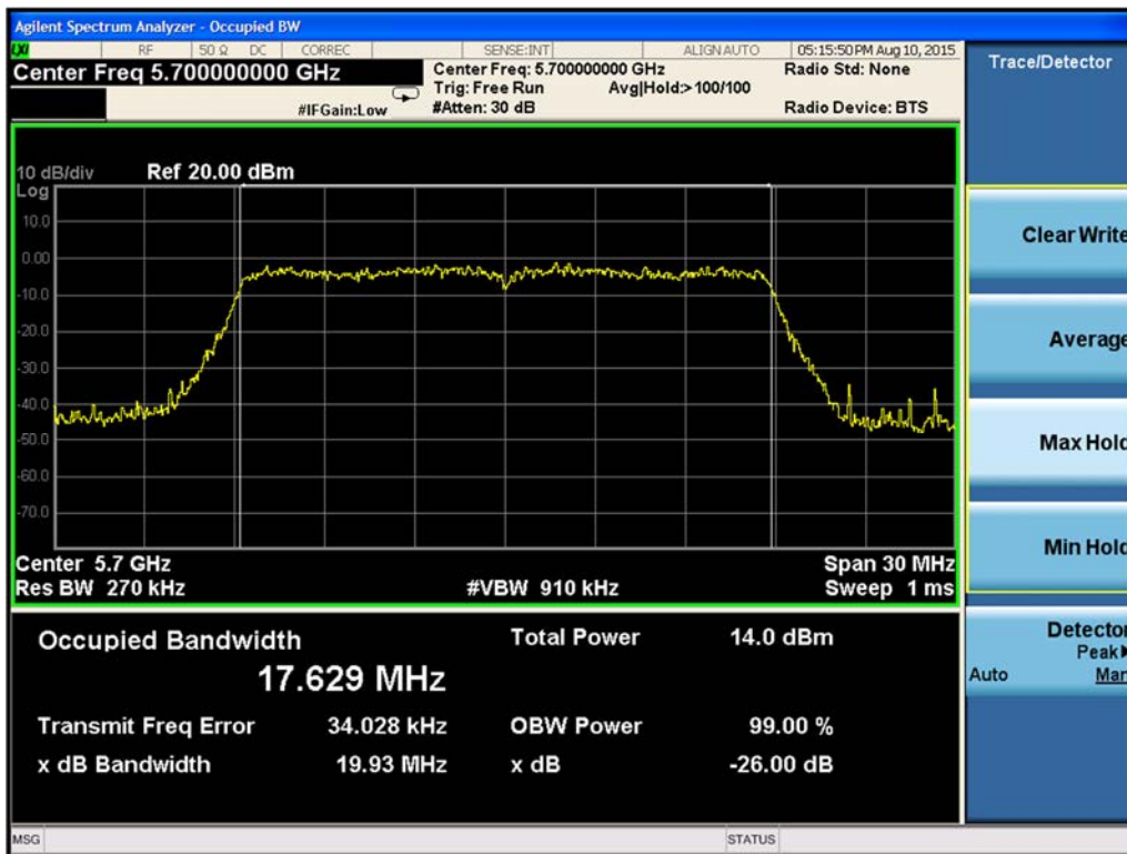
Figure 9-191. 99% Occupied Bandwidth Chain A 802.11ac VHT20 (Ch. 140)
