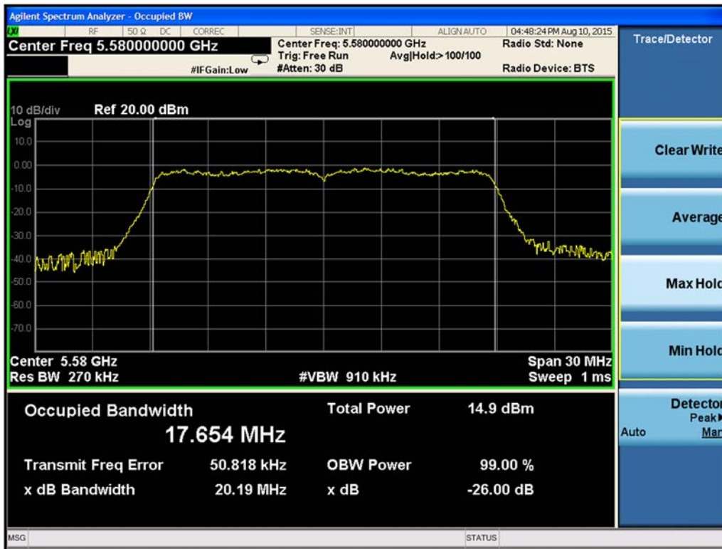
Figure 9-164. 99% Occupied Bandwidth Chain A 802.11n HT20 (Ch. 116)
