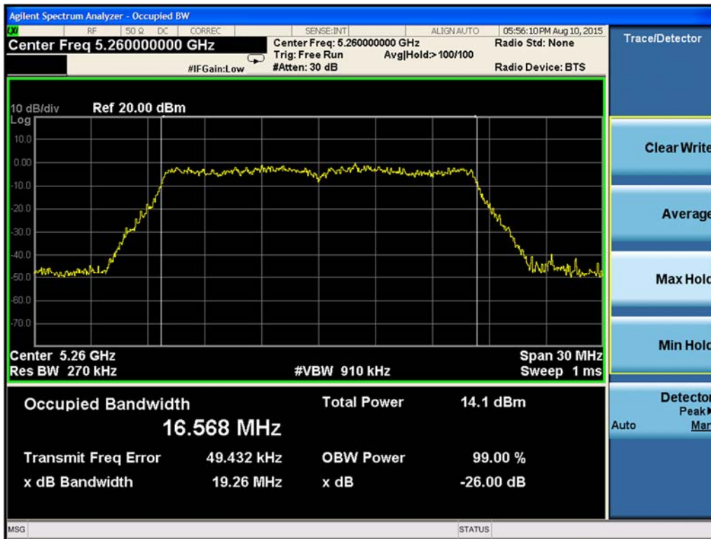
Figure 9-147. 99% Occupied Bandwidth Chain B 802.11a (Ch. 52)
