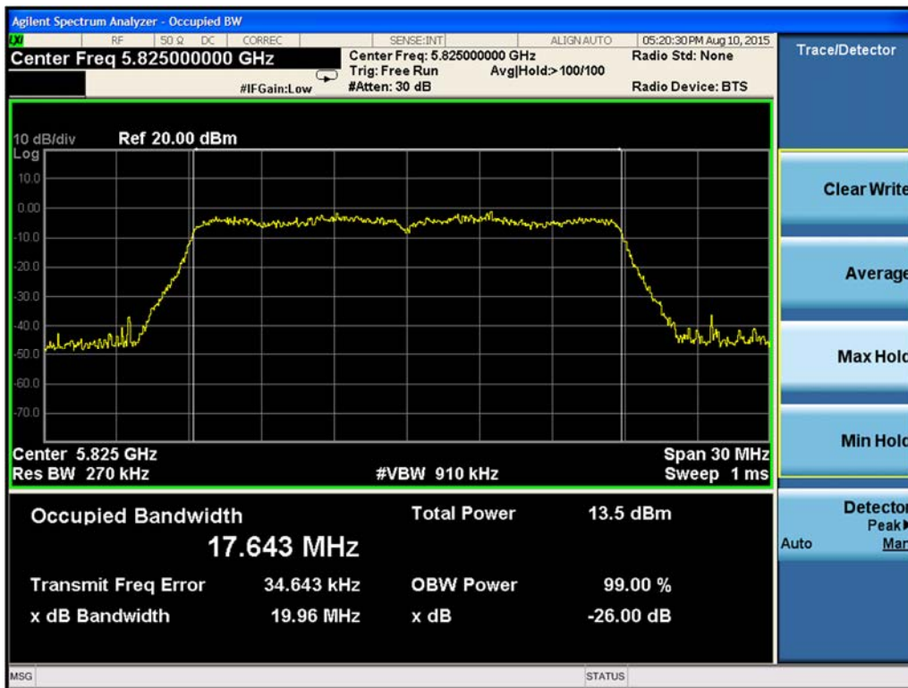
Figure 9-195. 99% Occupied Bandwidth Chain A 802.11ac VHT20 (Ch. 165)
