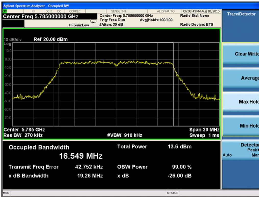
Figure 9-155. 99% Occupied Bandwidth Chain B 802.11a (Ch. 157)
