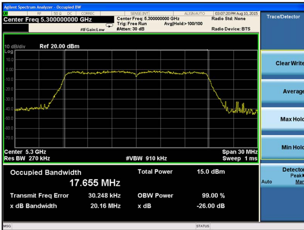
Figure 9-161. 99% Occupied Bandwidth Chain A 802.11n HT20 (Ch. 60)
