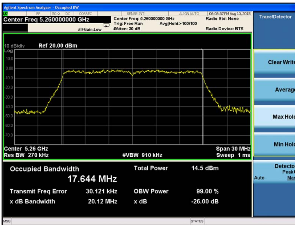
Figure 9-173. 99% Occupied Bandwidth Chain B 802.11n HT20 (Ch. 52)
