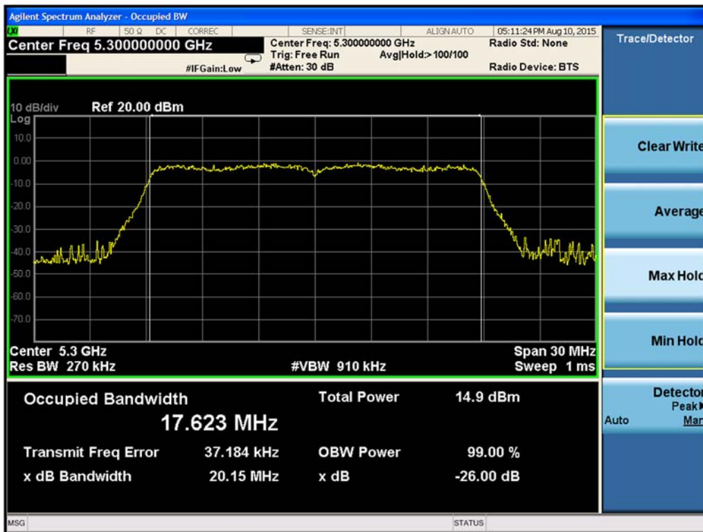
Figure 9-187. 99% Occupied Bandwidth Chain A 802.11ac VHT20 (Ch. 60)
