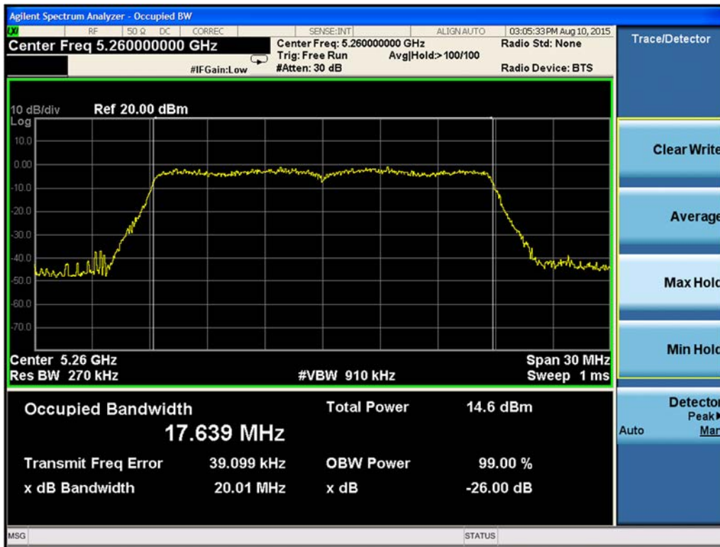
Figure 9-160. 99% Occupied Bandwidth Chain A 802.11n HT20 (Ch. 52)
