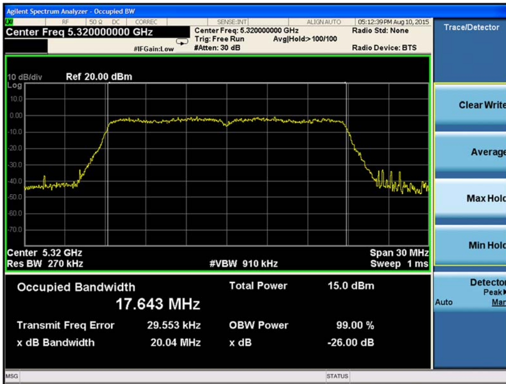
Figure 9-188. 99% Occupied Bandwidth Chain A 802.11ac VHT20 (Ch. 64)
