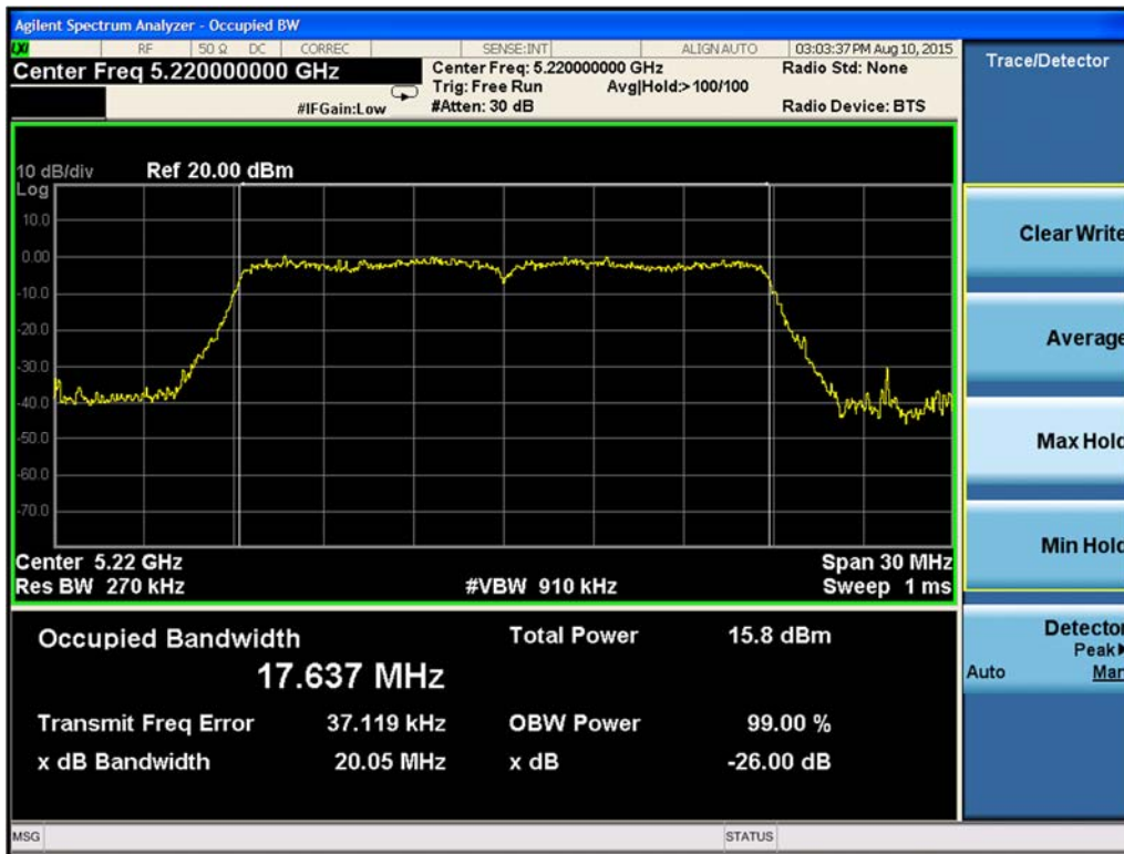
Figure 9-158. 99% Occupied Bandwidth Chain A 802.11n HT20 (Ch. 44)
