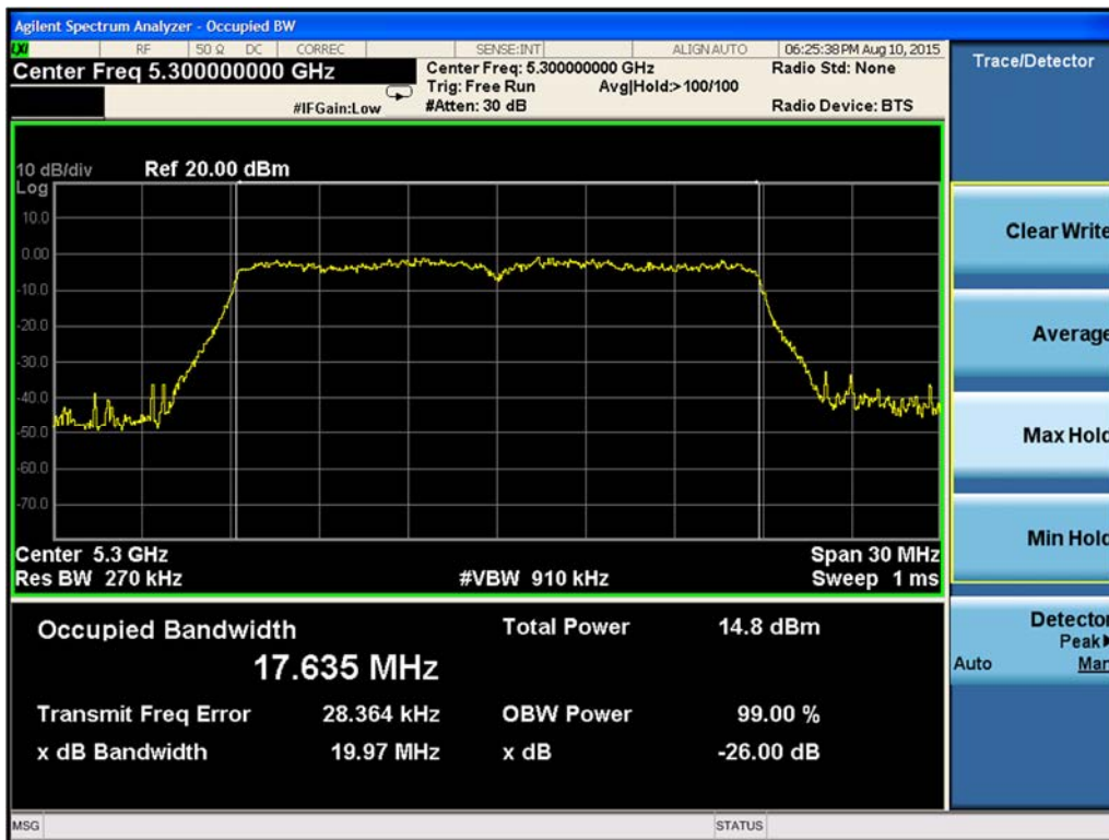
Figure 9-200. 99% Occupied Bandwidth Chain B 802.11ac VHT20 (Ch. 60)
