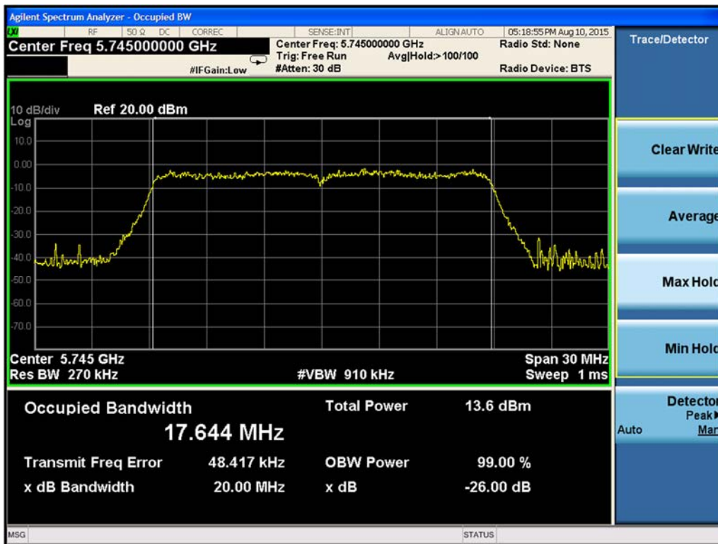
Figure 9-193. 99% Occupied Bandwidth Chain A 802.11ac VHT20 (Ch. 149)
