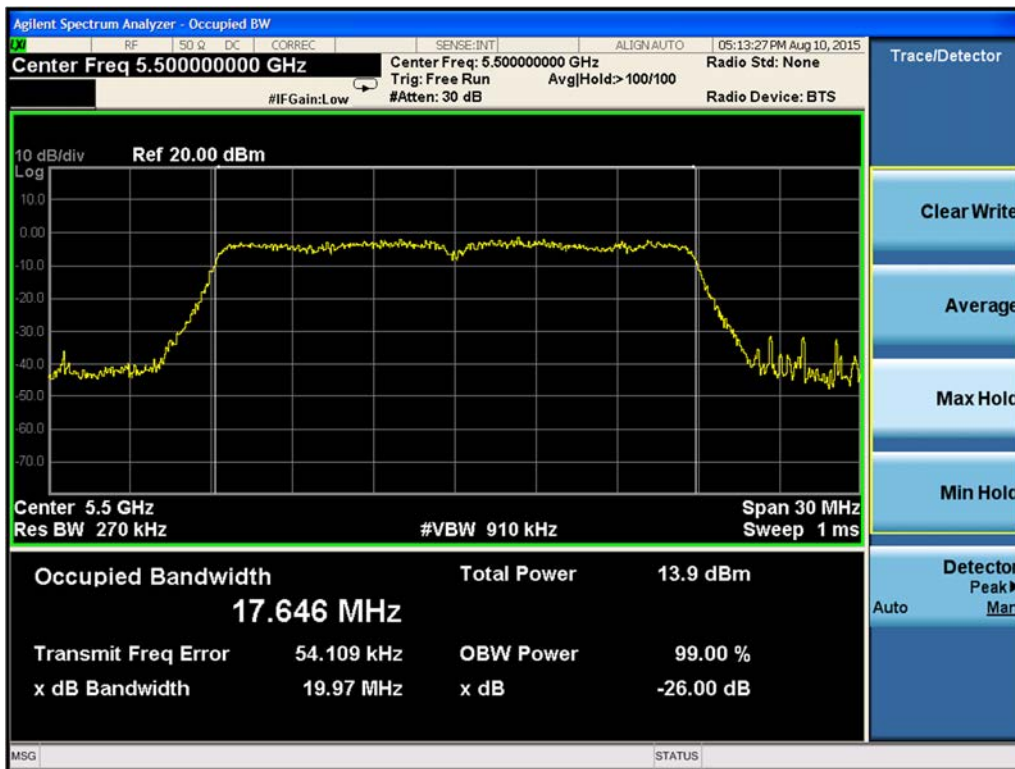
Figure 9-189. 99% Occupied Bandwidth Chain A 802.11ac VHT20 (Ch. 100)
