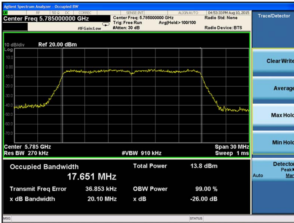
Figure 9-168. 99% Occupied Bandwidth Chain A 802.11n HT20 (Ch. 157)
