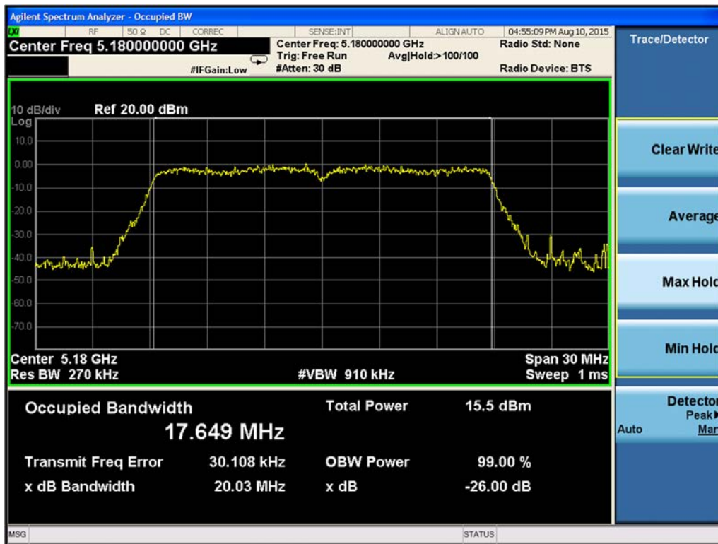
Figure 9-183. 99% Occupied Bandwidth Chain A 802.11ac VHT20 (Ch. 36)
