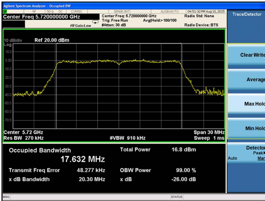
Figure 9-166. 99% Occupied Bandwidth Chain A 802.11n HT20 (Ch. 144)
