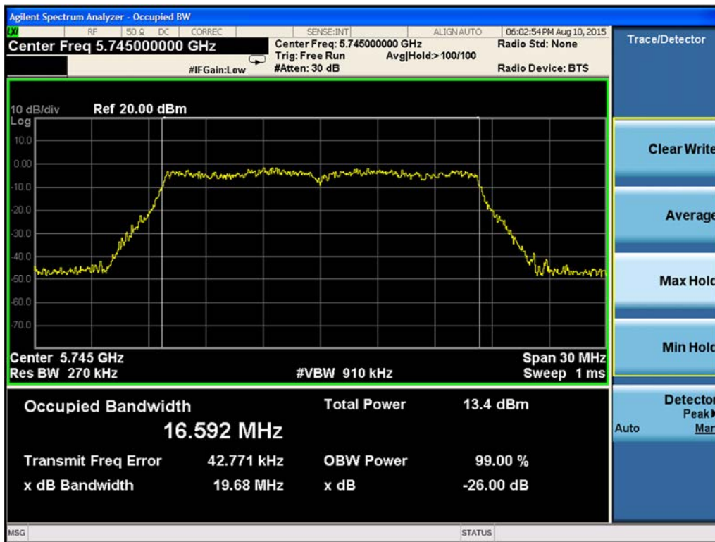
Figure 9-154. 99% Occupied Bandwidth Chain B 802.11a (Ch. 149)
