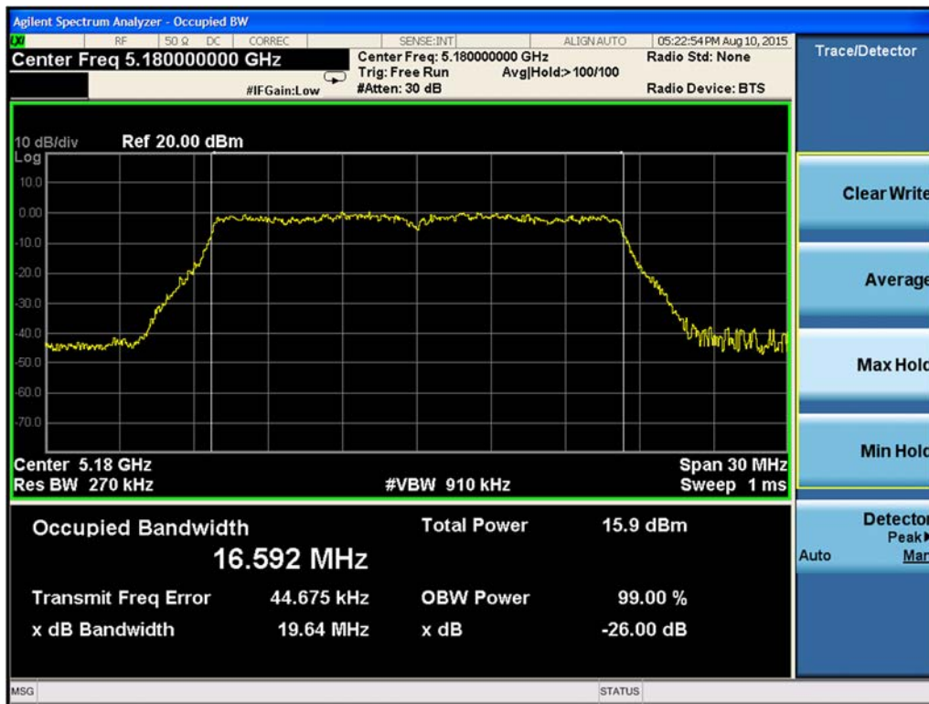
Figure 9-144. 99% Occupied Bandwidth Chain B 802.11a (Ch. 36)
