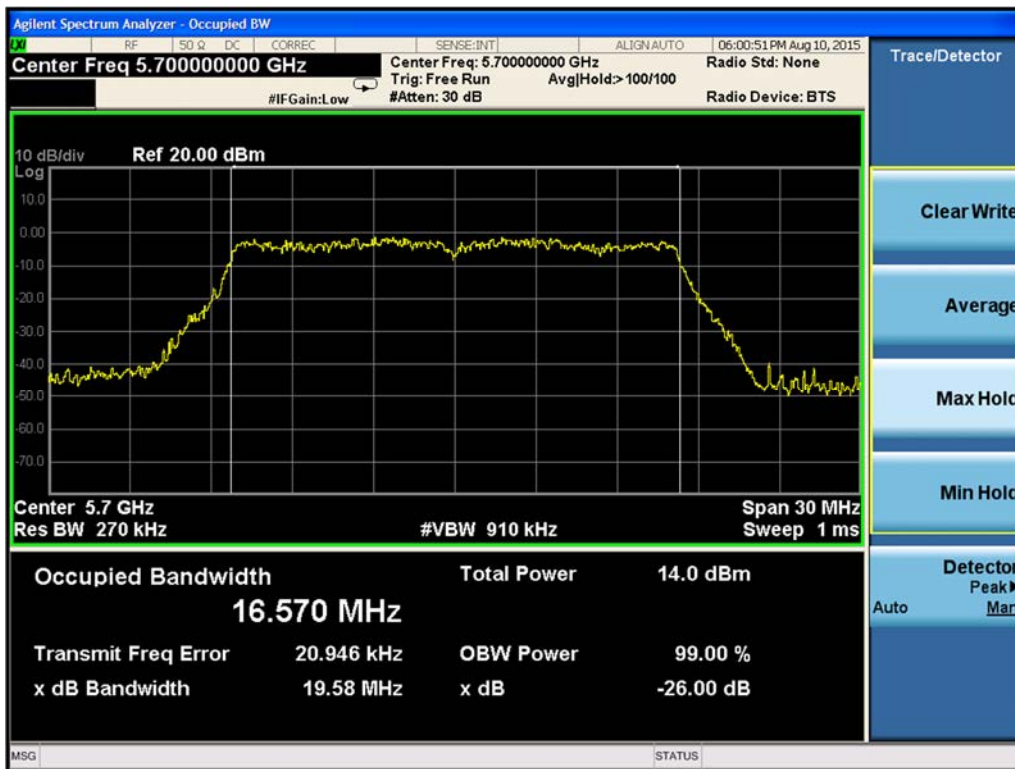
Figure 9-152. 99% Occupied Bandwidth Chain B 802.11a (Ch. 140)
