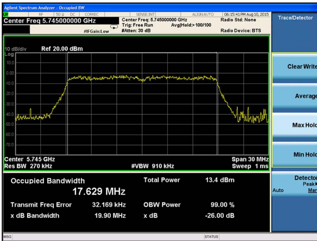
Figure 9-180. 99% Occupied Bandwidth Chain B 802.11n HT20 (Ch. 149)
