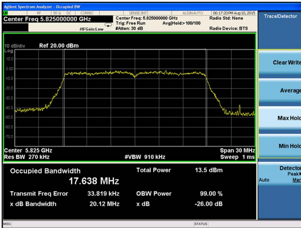
Figure 9-182. 99% Occupied Bandwidth Chain B 802.11n HT20 (Ch. 165)
