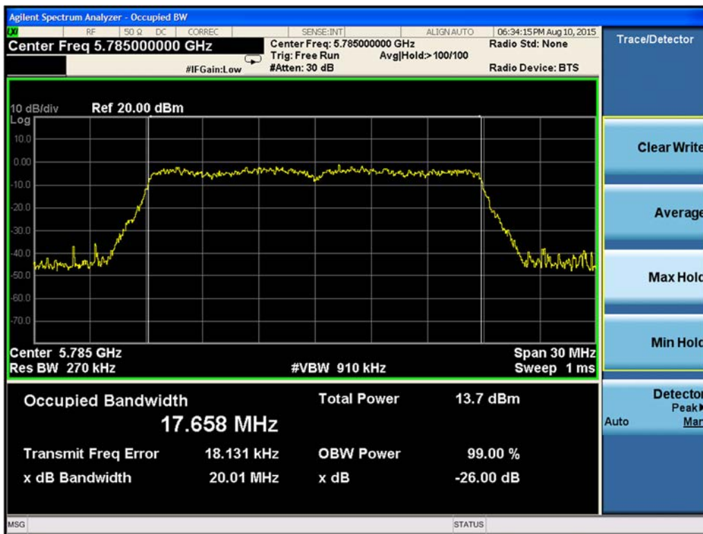
Figure 9-207. 99% Occupied Bandwidth Chain B 802.11ac VHT20 (Ch. 157)
