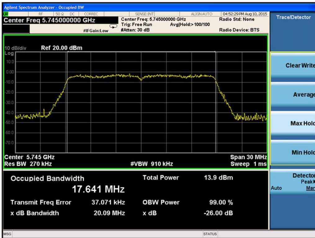
Figure 9-167. 99% Occupied Bandwidth Chain A 802.11n HT20 (Ch. 149)
