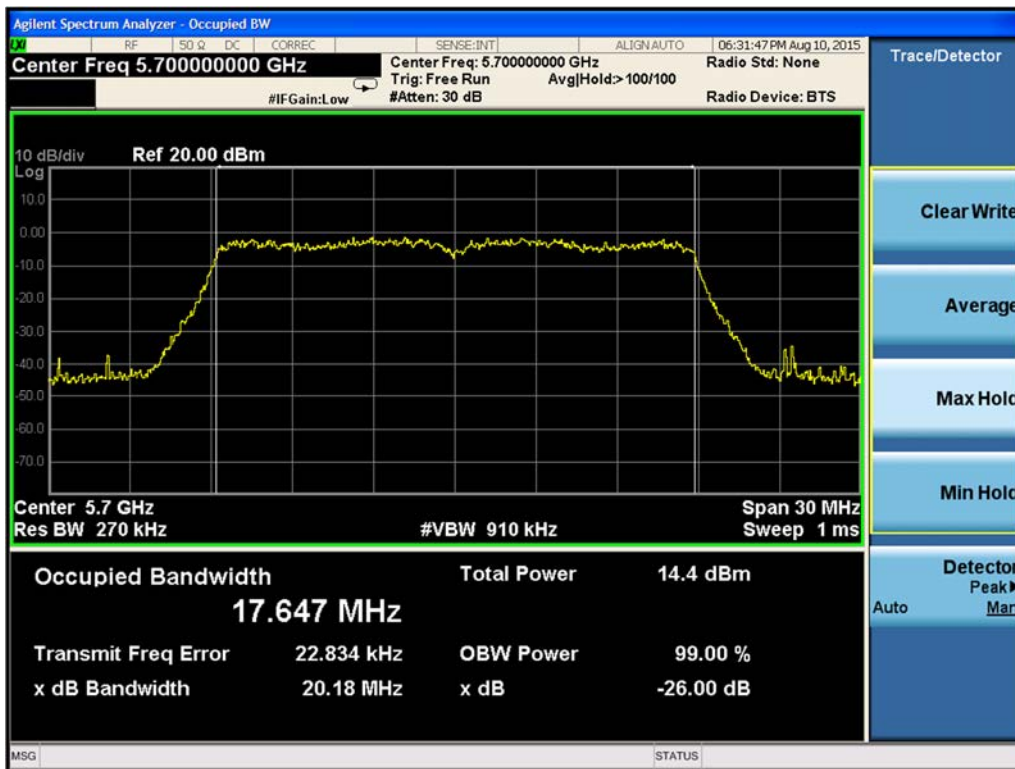
Figure 9-204. 99% Occupied Bandwidth Chain B 802.11ac VHT20 (Ch. 140)
