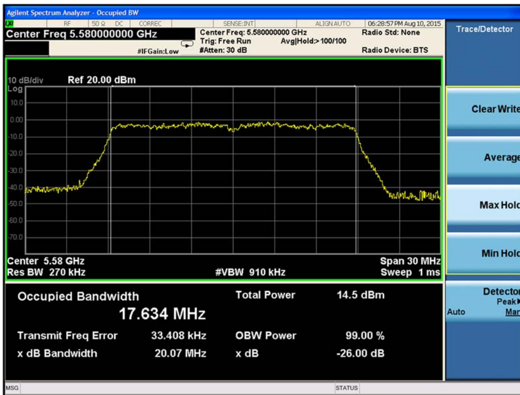
Figure 9-203. 99% Occupied Bandwidth Chain B 802.11ac VHT20 (Ch. 116)
