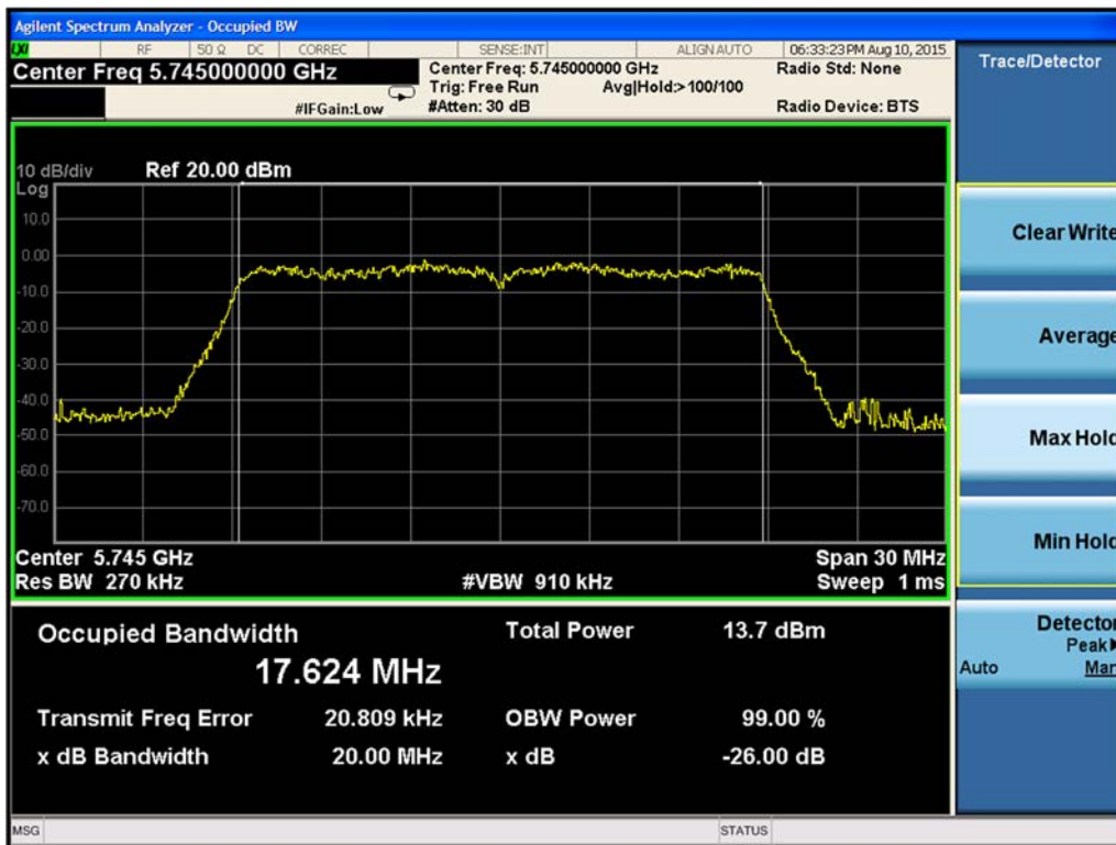
Figure 9-206. 99% Occupied Bandwidth Chain B 802.11ac VHT20 (Ch. 149)
