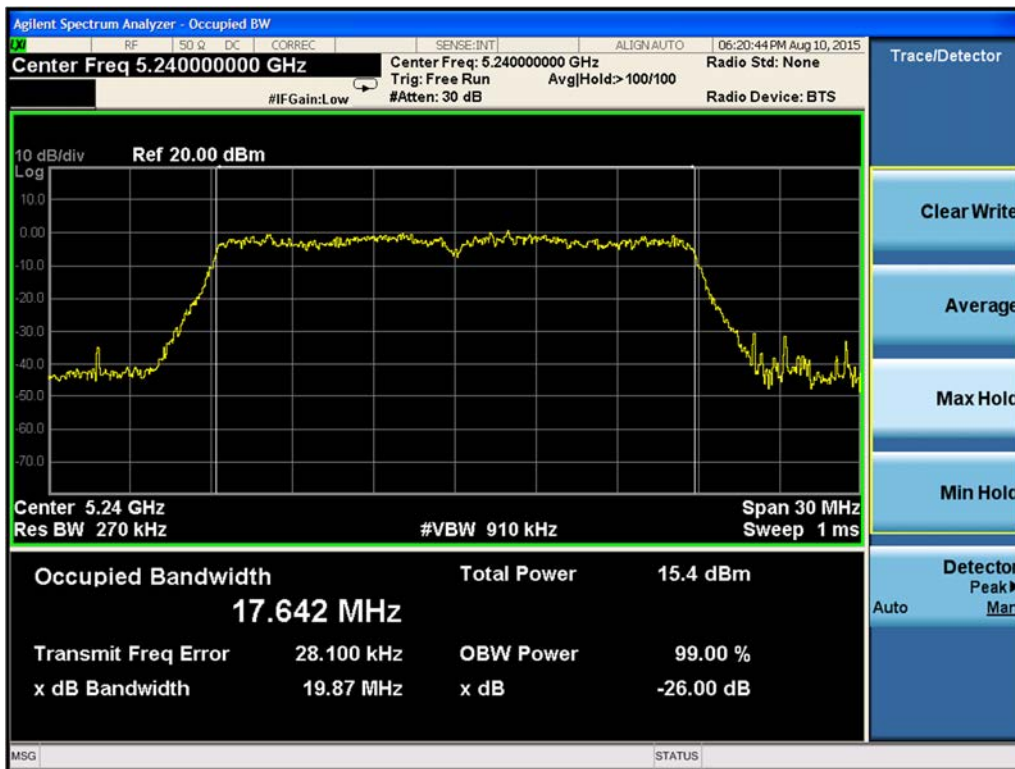
Figure 9-198. 99% Occupied Bandwidth Chain B 802.11ac VHT20 (Ch. 48)
