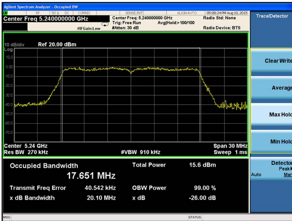
Figure 9-185. 99% Occupied Bandwidth Chain A 802.11ac VHT20 (Ch. 48)
