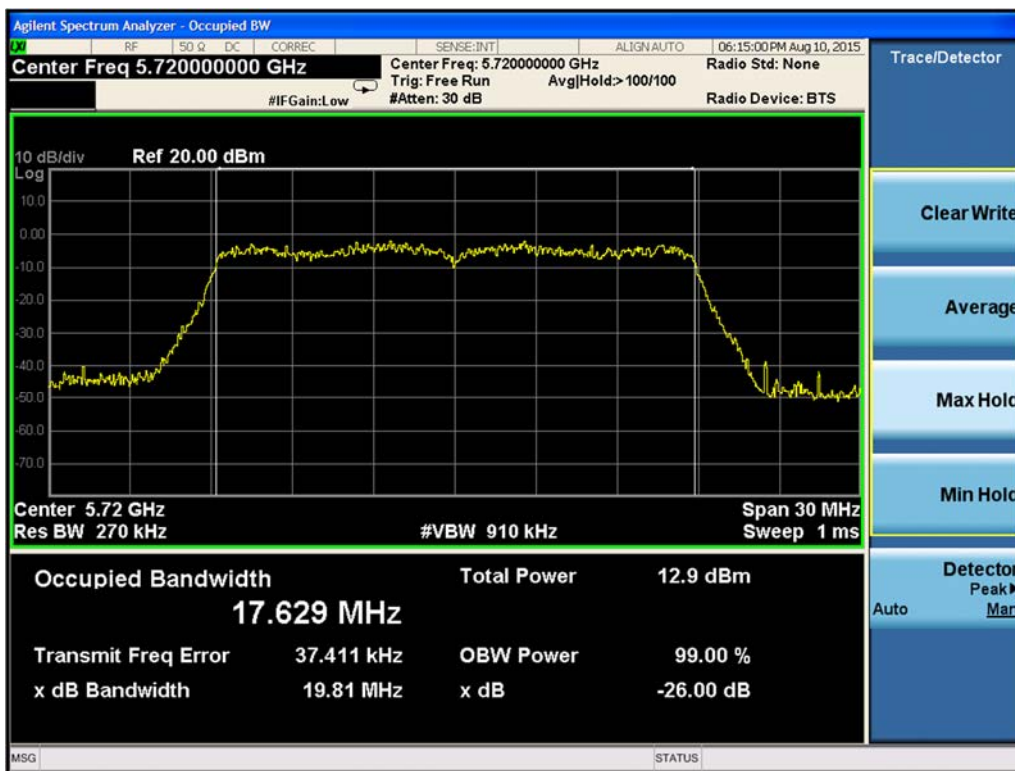
Figure 9-179. 99% Occupied Bandwidth Chain B 802.11n HT20 (Ch. 144)
