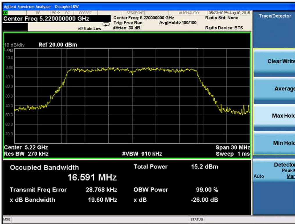
Figure 9-145. 99% Occupied Bandwidth Chain B 802.11a (Ch. 44)
