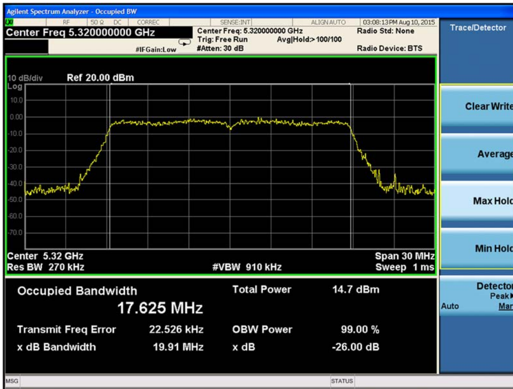
Figure 9-162. 99% Occupied Bandwidth Chain A 802.11n HT20 (Ch. 64)
