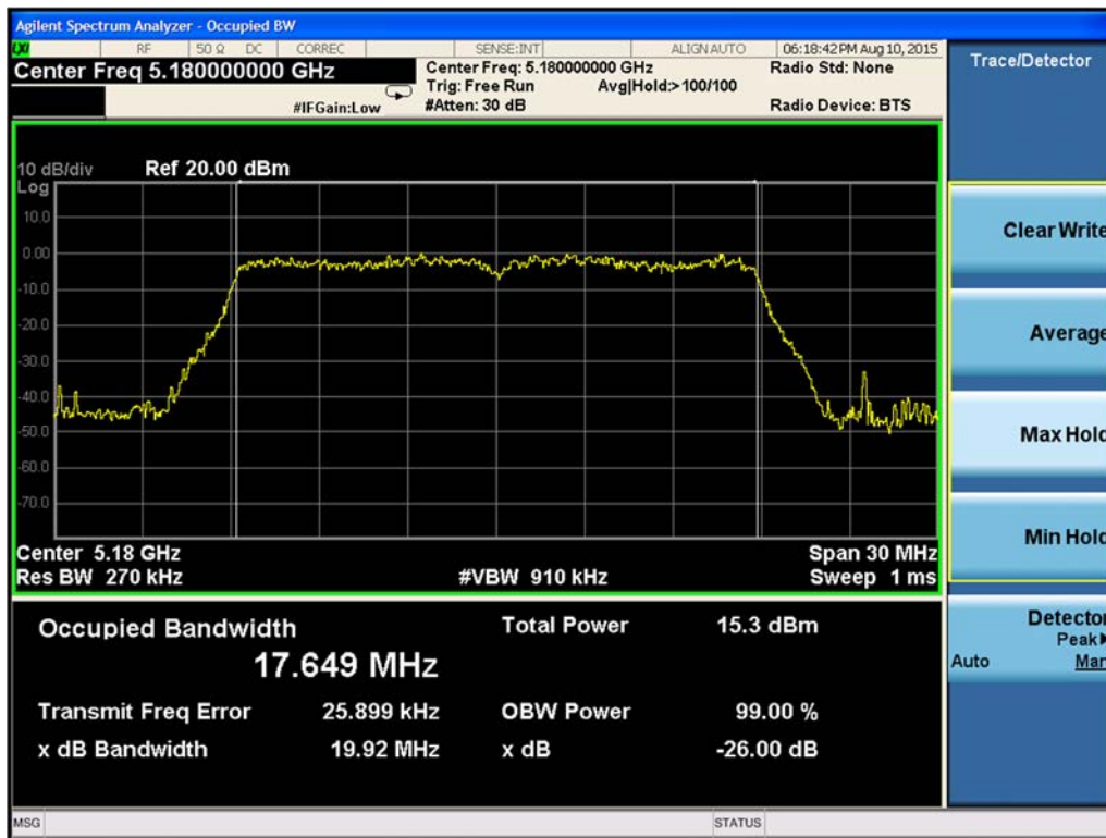
Figure 9-196. 99% Occupied Bandwidth Chain B 802.11ac VHT20 (Ch. 36)
