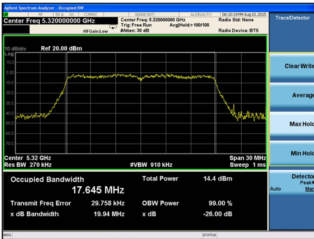
Figure 9-175. 99% Occupied Bandwidth Chain B 802.11n HT20 (Ch. 64)
