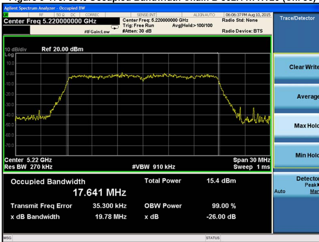
Figure 9-171. 99% Occupied Bandwidth Chain B 802.11n HT20 (Ch. 44)
