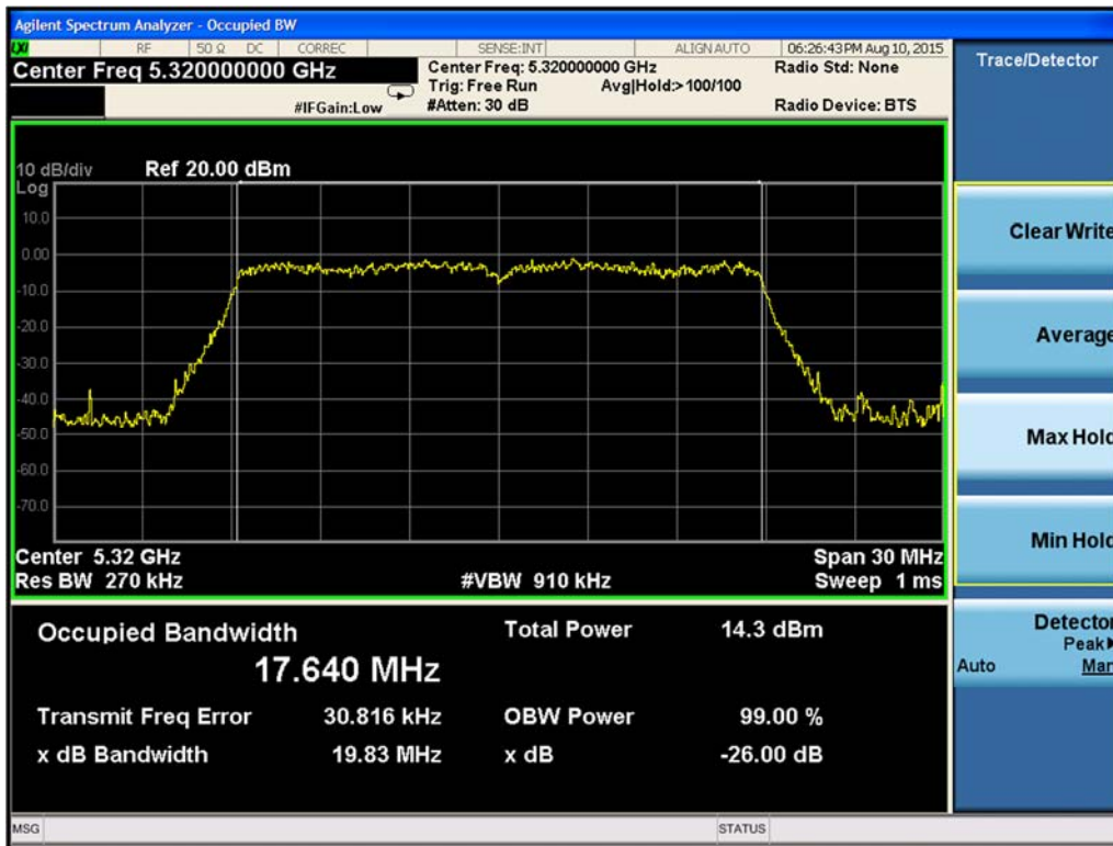
Figure 9-201. 99% Occupied Bandwidth Chain B 802.11ac VHT20 (Ch. 64)
