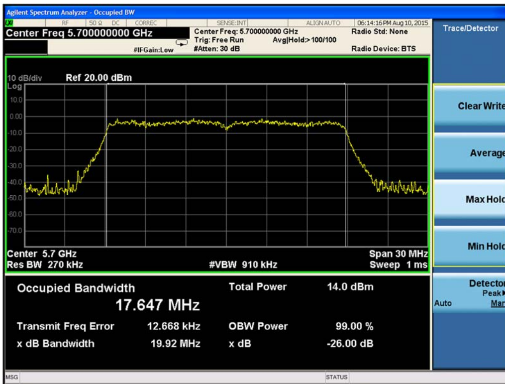
Figure 9-178. 99% Occupied Bandwidth Chain B 802.11n HT20 (Ch. 140)
