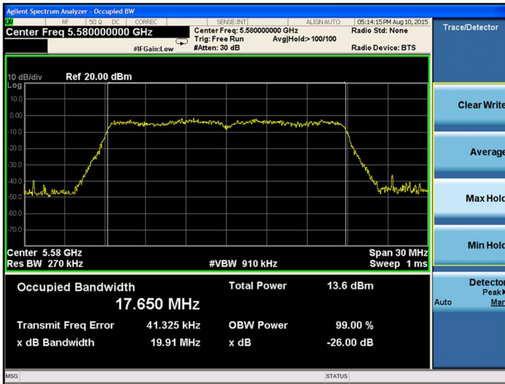
Figure 9-190. 99% Occupied Bandwidth Chain A 802.11ac VHT20 (Ch. 116)
