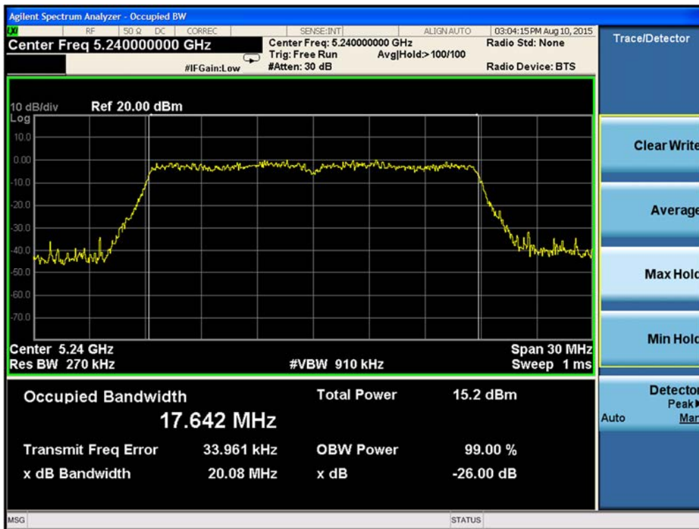
Figure 9-159. 99% Occupied Bandwidth Chain A 802.11n HT20 (Ch. 48)
