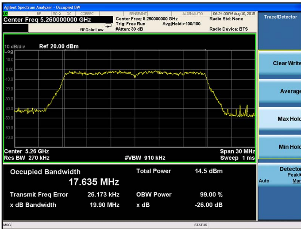
Figure 9-199. 99% Occupied Bandwidth Chain B 802.11ac VHT20 (Ch. 52)
