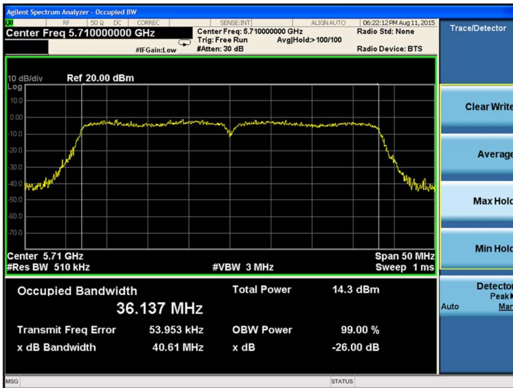
Figure 9-217. 99% Occupied Bandwidth Chain A 802.11n HT40 (Ch. 142)
