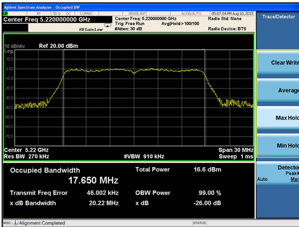
Figure 9-184. 99% Occupied Bandwidth Chain A 802.11ac VHT20 (Ch. 44)
