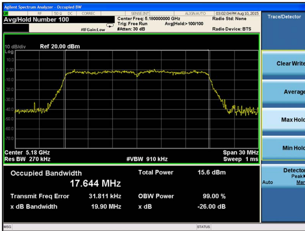
Figure 9-157. 99% Occupied Bandwidth Chain A 802.11n HT20 (Ch. 36)
