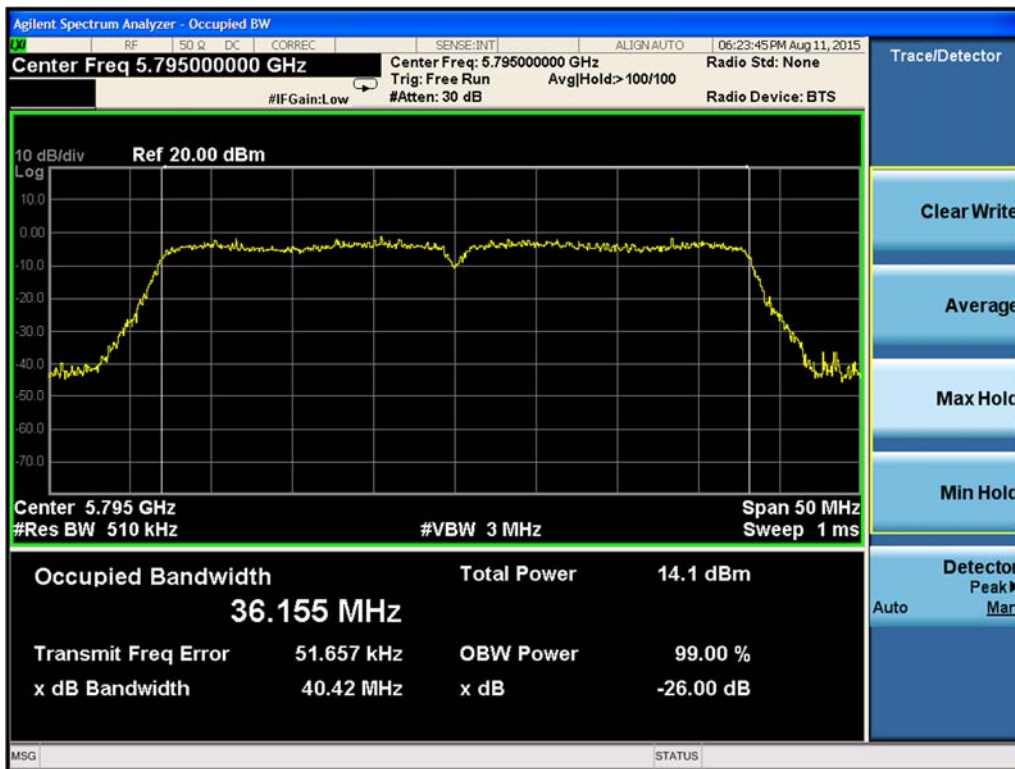
Figure 9-219. 99% Occupied Bandwidth Chain A 802.11n HT40 (Ch. 159)
