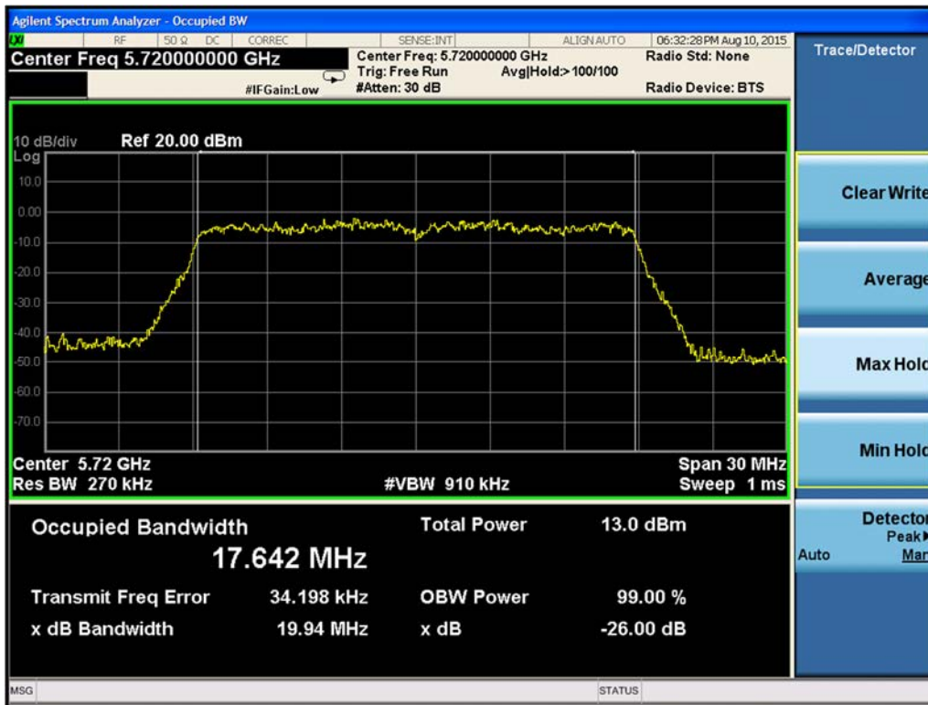
Figure 9-205. 99% Occupied Bandwidth Chain B 802.11ac VHT20 (Ch. 144)
