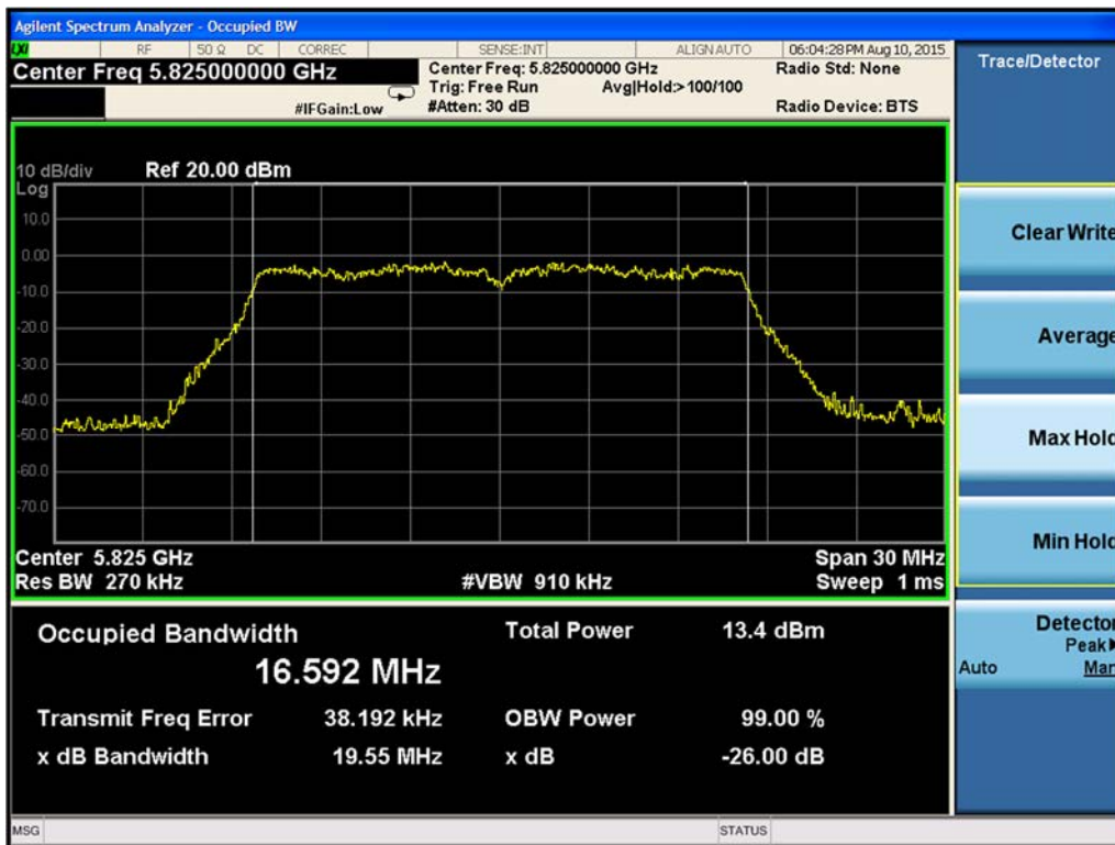
Figure 9-156. 99% Occupied Bandwidth Chain B 802.11a (Ch. 165)
