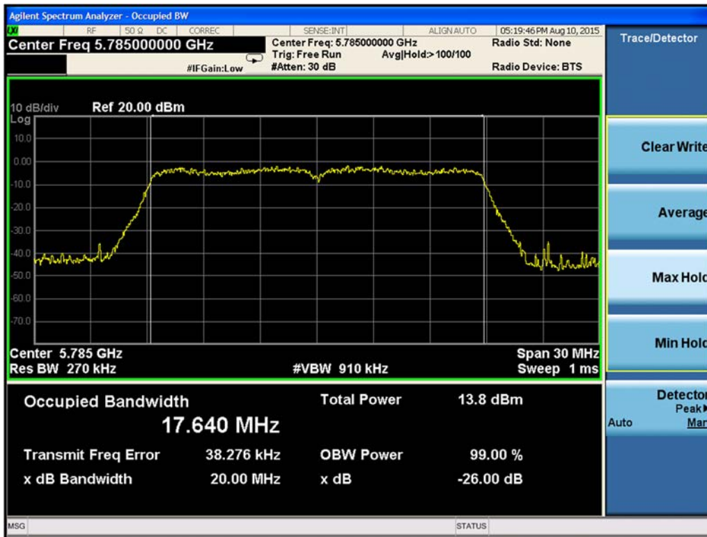
Figure 9-194. 99% Occupied Bandwidth Chain A 802.11ac VHT20 (Ch. 157)
