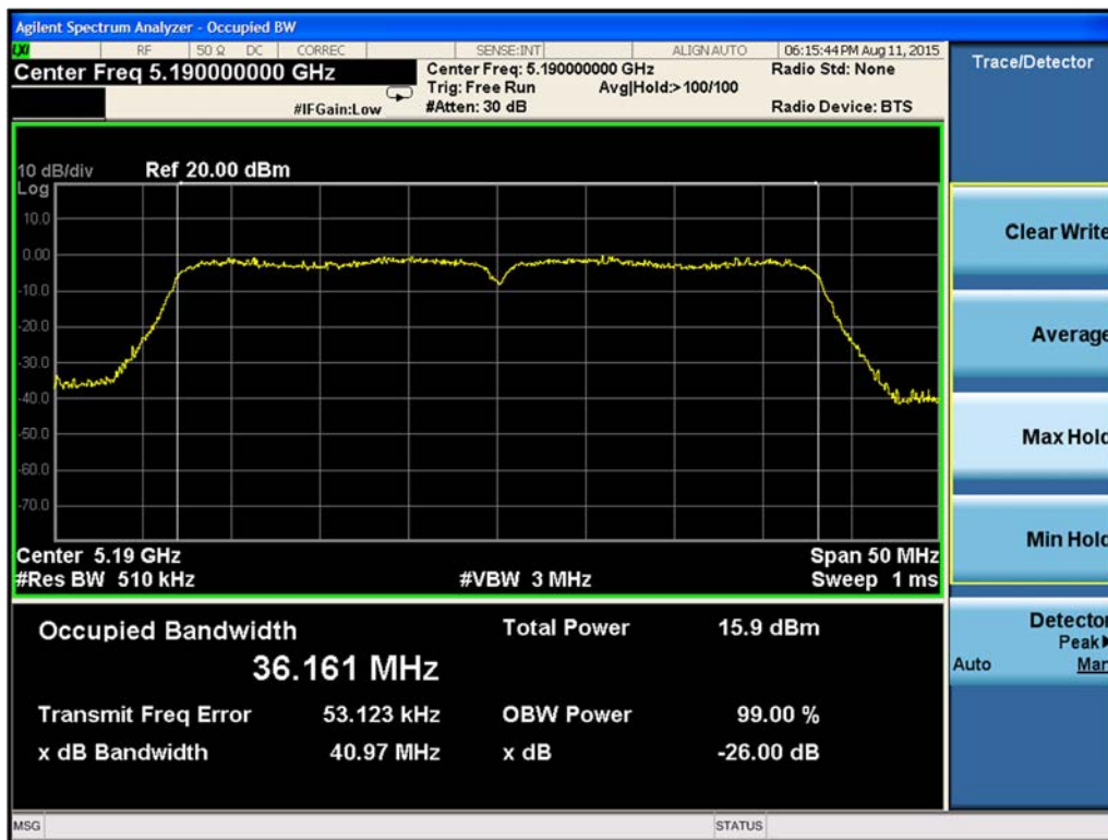
Figure 9-209. 99% Occupied Bandwidth Chain A 802.11n HT40 (Ch. 38)
