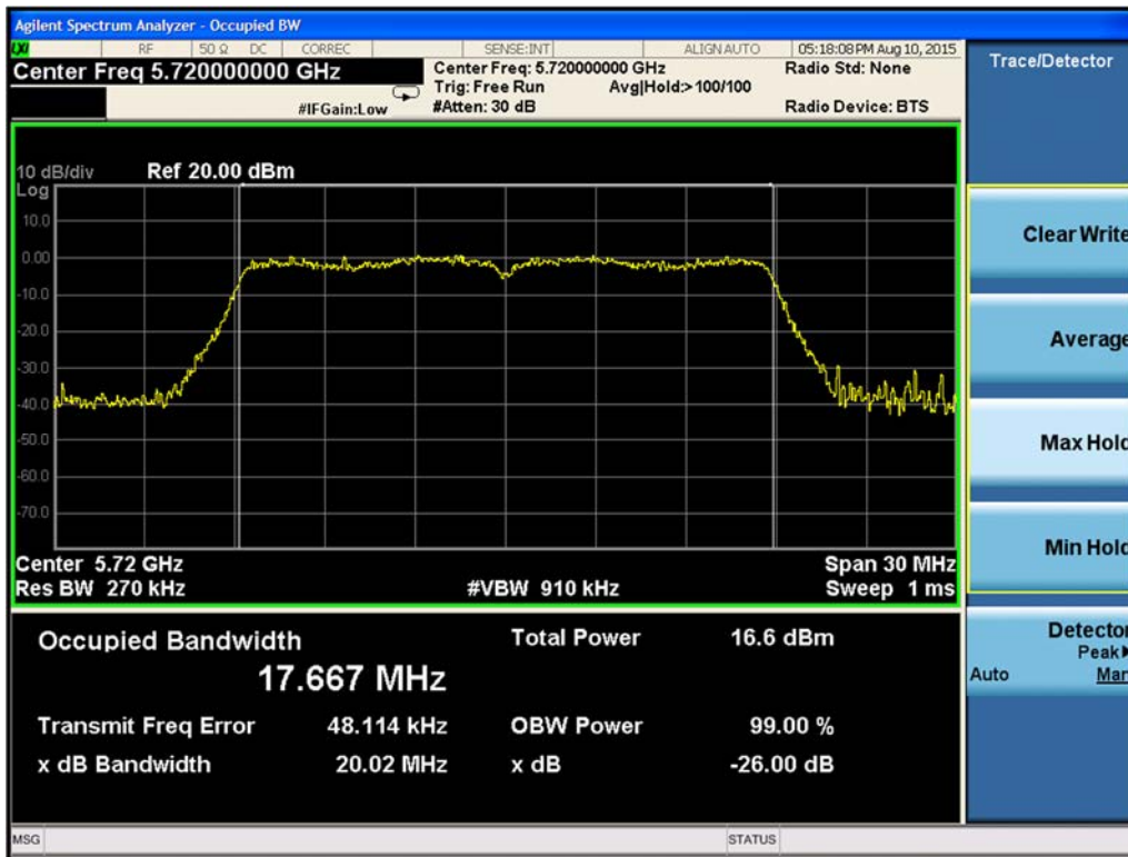
Figure 9-192. 99% Occupied Bandwidth Chain A 802.11ac VHT20 (Ch. 144)
