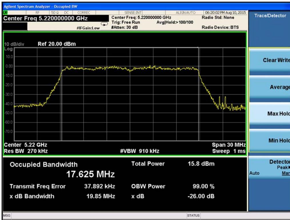
Figure 9-197. 99% Occupied Bandwidth Chain B 802.11ac VHT20 (Ch. 44)
