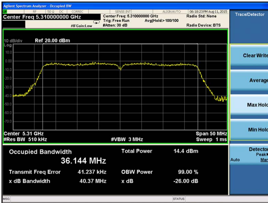
Figure 9-212. 99% Occupied Bandwidth Chain A 802.11n HT40 (Ch. 62)
