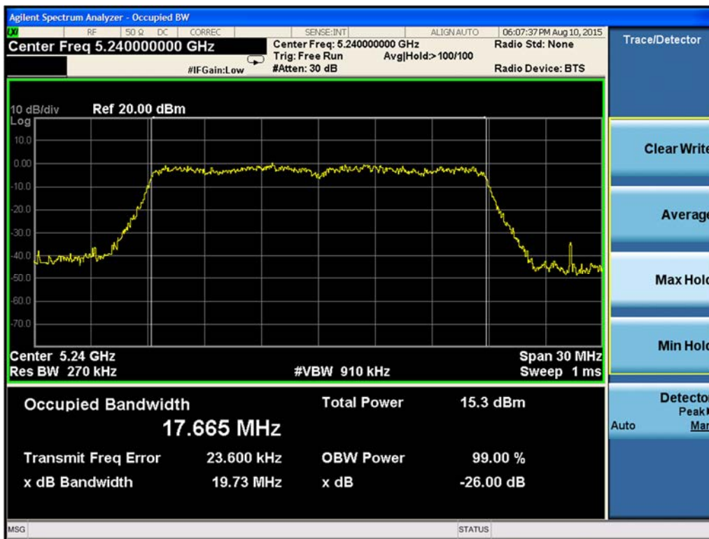
Figure 9-172. 99% Occupied Bandwidth Chain B 802.11n HT20 (Ch. 48)
