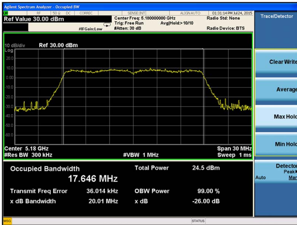
Figure 9-53. 26-dB Emission Bandwidth Chain A 802.11ac VHT20 (Ch. 36)
