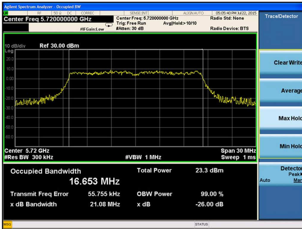
Figure 9-23. 26-dB Emission Bandwidth Chain B 802.11a (Ch. 144)
