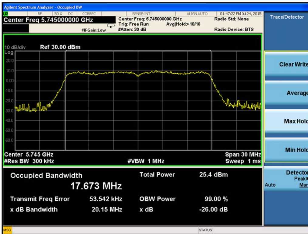
Figure 9-63. 26-dB Emission Bandwidth Chain A 802.11ac VHT20 (Ch. 149)
