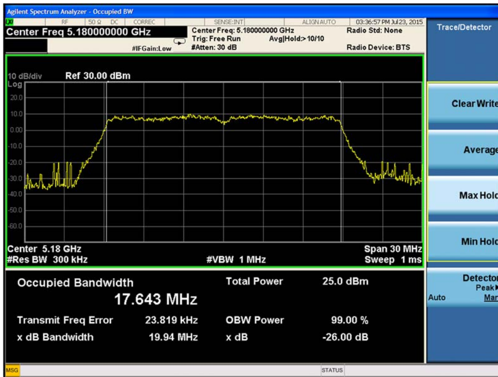
Figure 9-40. 26-dB Emission Bandwidth Chain B 802.11n HT20 (Ch. 36)
