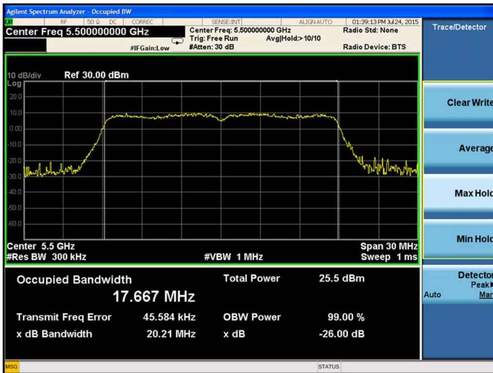
Figure 9-59. 26-dB Emission Bandwidth Chain A 802.11ac VHT20 (Ch. 100)
