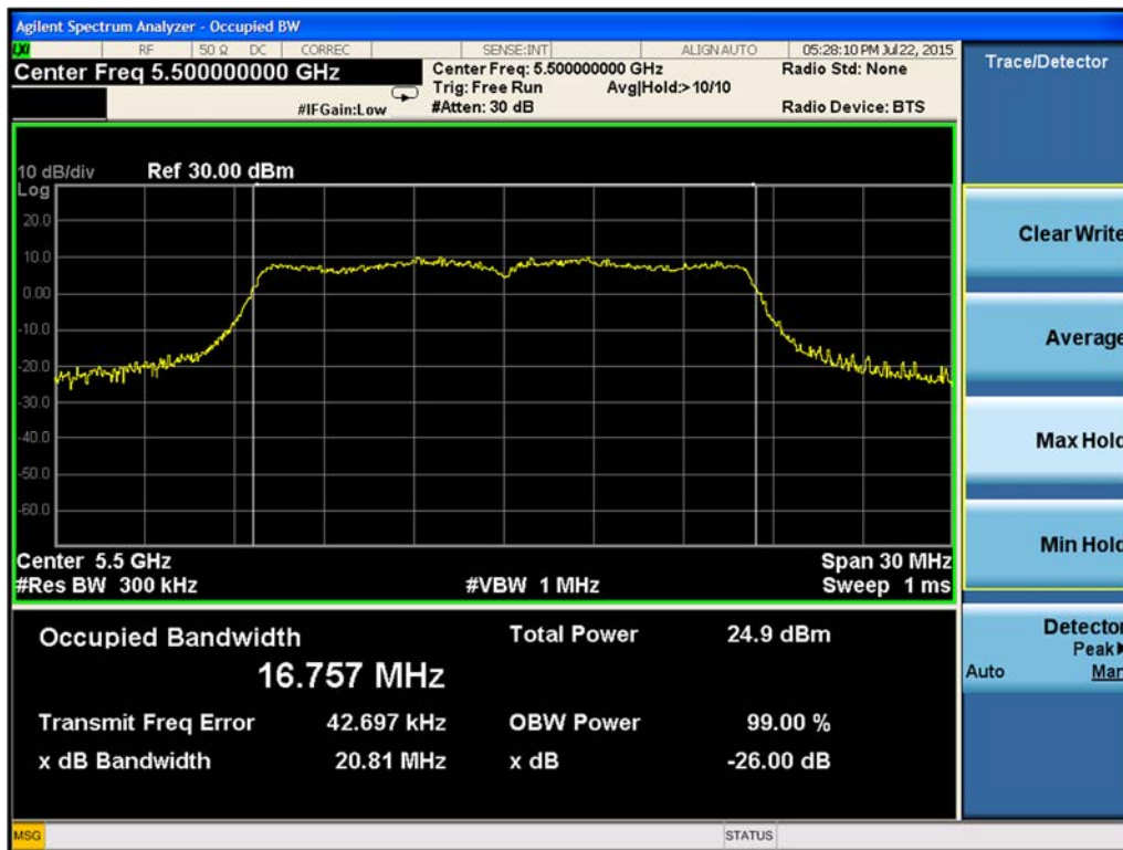
Figure 9-7 . 26-dB Emission Bandwidth Chain A 802.11a (Ch. 100)
