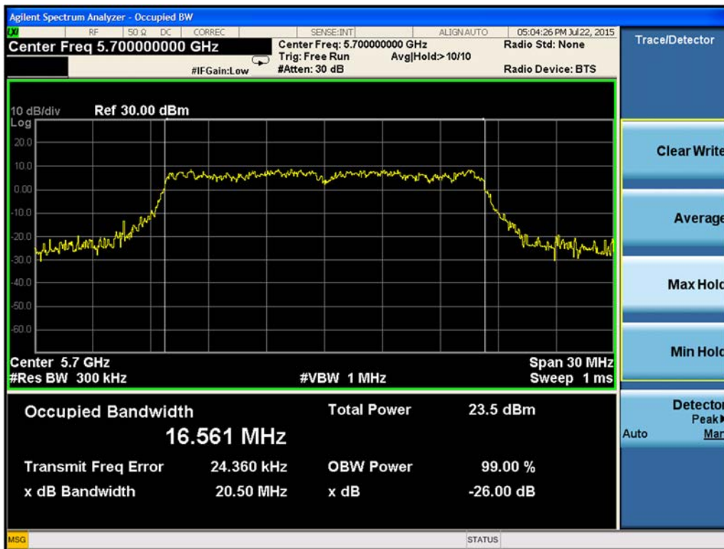
Figure 9-22. 26-dB Emission Bandwidth Chain B 802.11a (Ch. 140)
