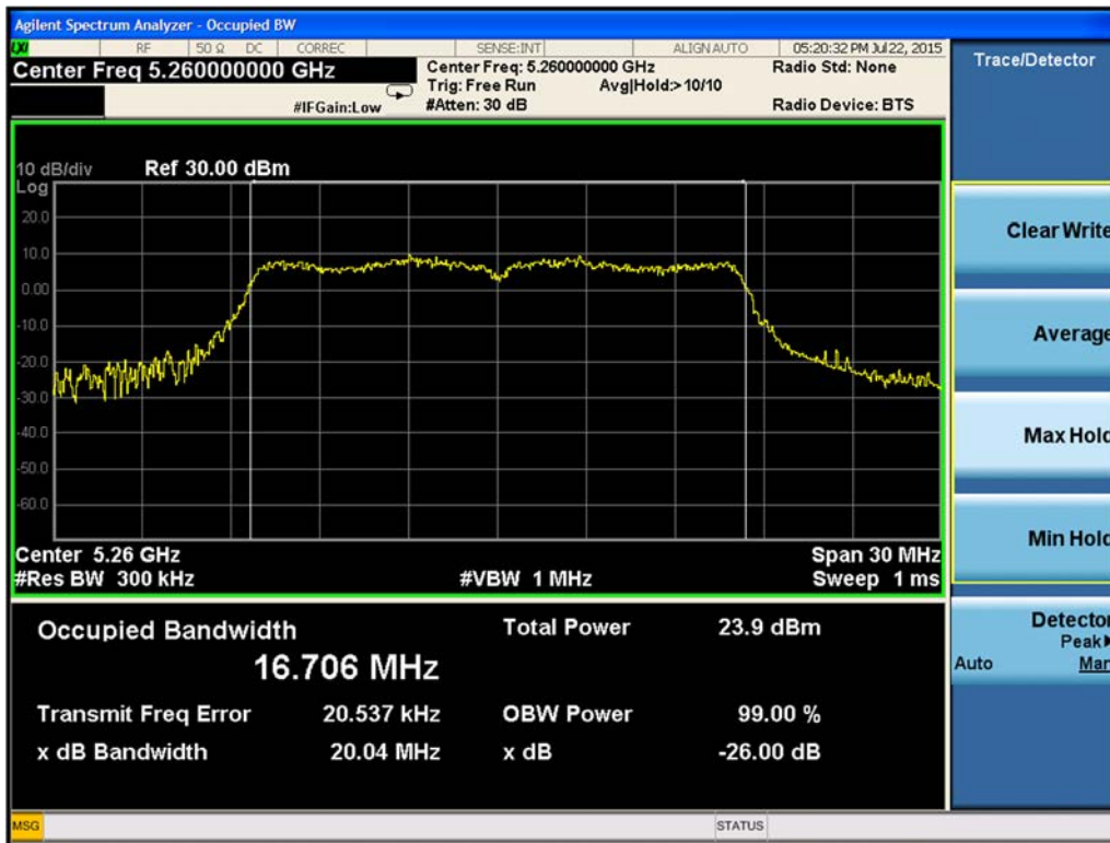
Figure 9-4. 26-dB Emission Bandwidth Chain A 802.11a (Ch. 52)
