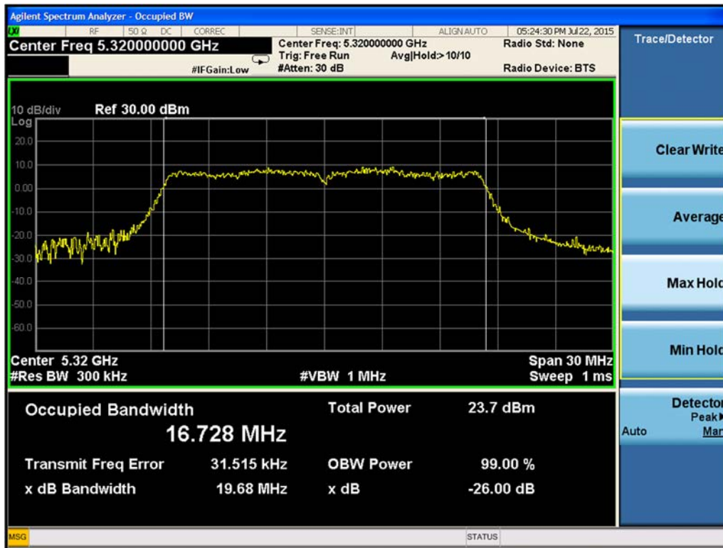
Figure 9-6. 26-dB Emission Bandwidth Chain A 802.11a (Ch. 64)
