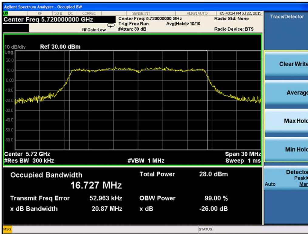
Figure 9-10. 26-dB Emission Bandwidth Chain A 802.11a (Ch. 144)
