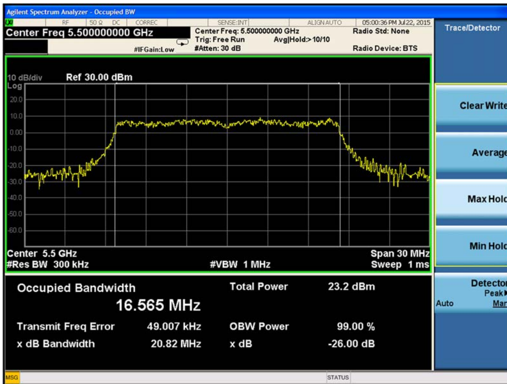
Figure 9-20. 26-dB Emission Bandwidth Chain B 802.11a (Ch. 100)
