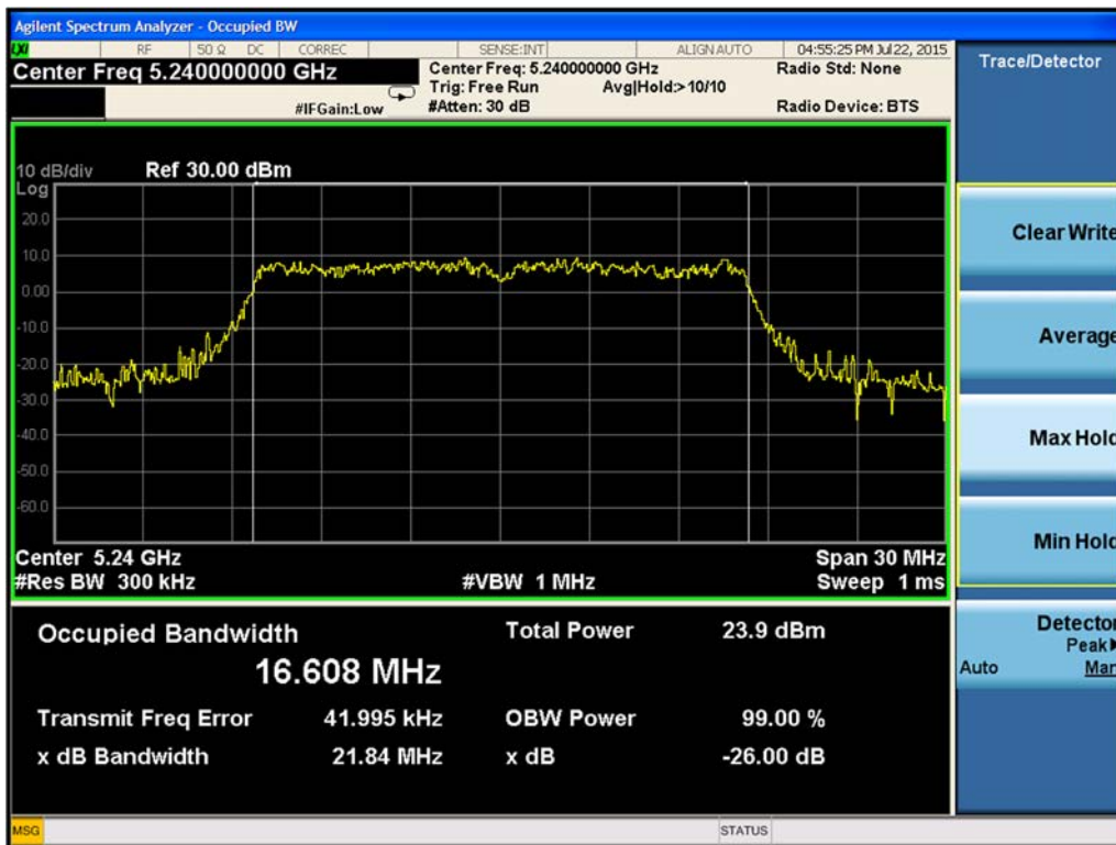
Figure 9-16. 26-dB Emission Bandwidth Chain B 802.11a (Ch. 48)
