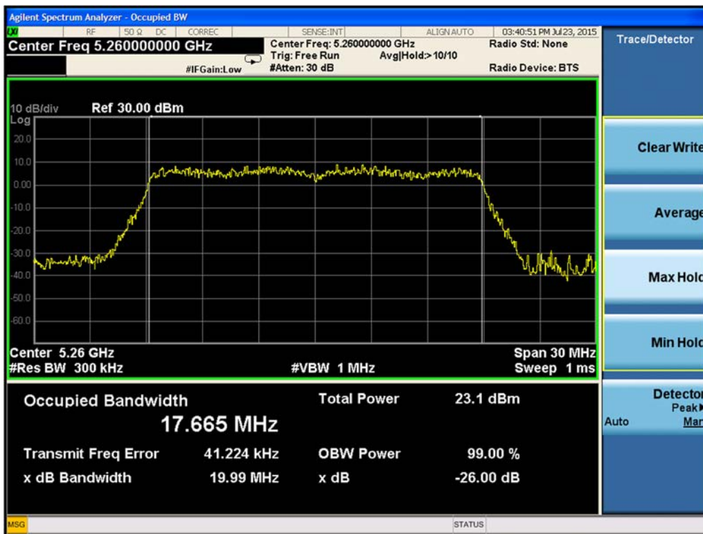
Figure 9-43. 26-dB Emission Bandwidth Chain B 802.11n HT20 (Ch. 52)
