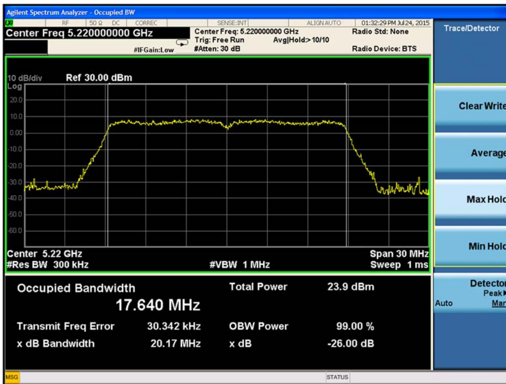
Figure 9-54. 26-dB Emission Bandwidth Chain A 802.11ac VHT20 (Ch. 44)
