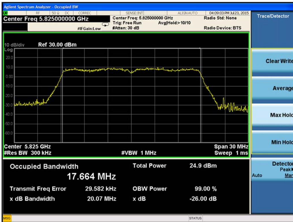
Figure 9-39. 26-dB Emission Bandwidth Chain A 802.11n HT20 (Ch. 165)
