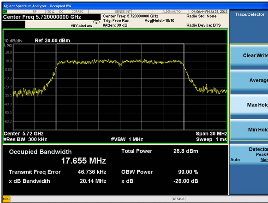
Figure 9-36. 26-dB Emission Bandwidth Chain A 802.11n HT20 (Ch. 144)
