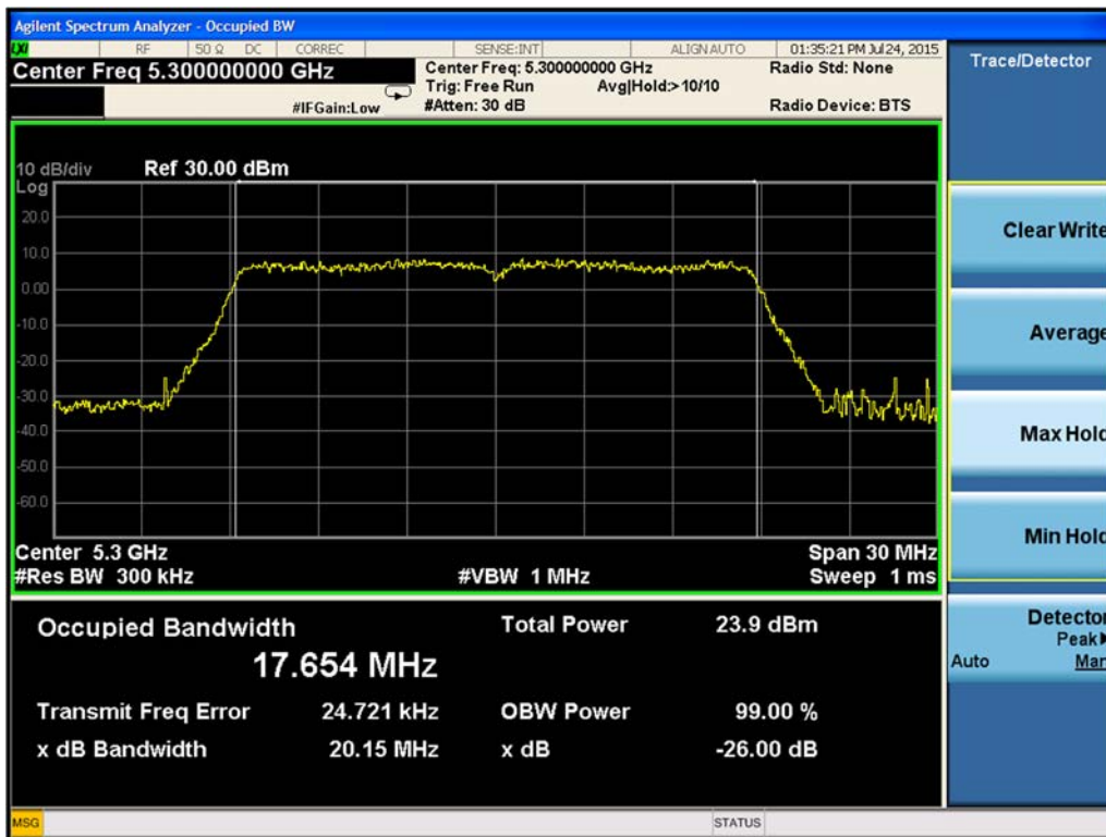
Figure 9-57. 26-dB Emission Bandwidth Chain A 802.11ac VHT20 (Ch. 60)
