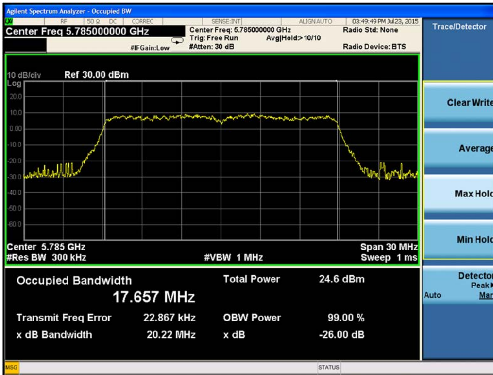
Figure 9-51. 26-dB Emission Bandwidth Chain B 802.11n HT20 (Ch. 157)
