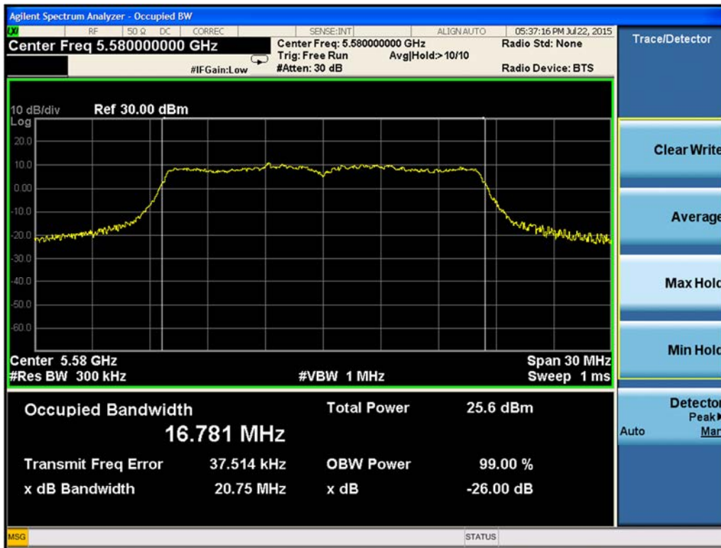
Figure 9-8. 26-dB Emission Bandwidth Chain A 802.11a (Ch. 116)
