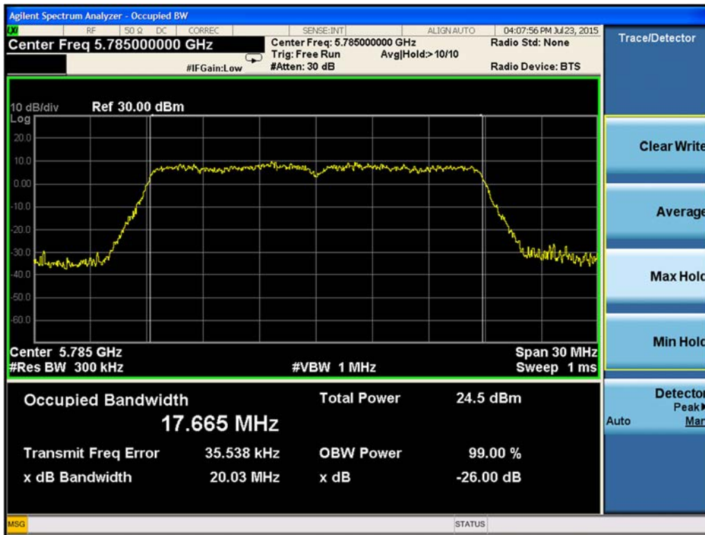
Figure 9-38. 26-dB Emission Bandwidth Chain A 802.11n HT20 (Ch. 157)
