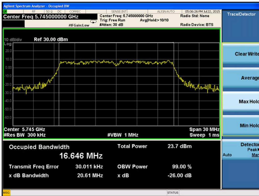
Figure 9-24. 26-dB Emission Bandwidth Chain B 802.11a (Ch. 149)
