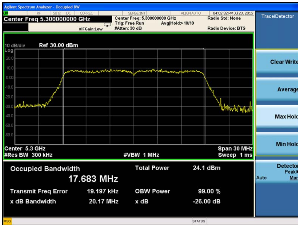
Figure 9-31. 26-dB Emission Bandwidth Chain A 802.11n HT20 (Ch. 60)
