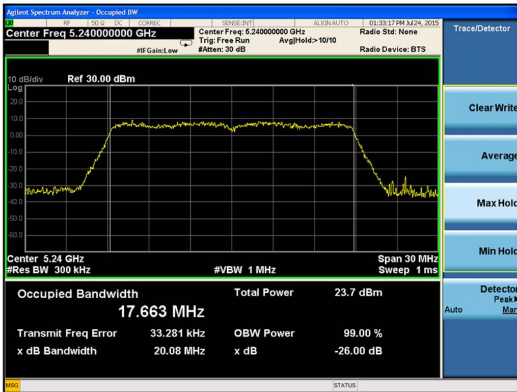
Figure 9-55. 26-dB Emission Bandwidth Chain A 802.11ac VHT20 (Ch. 48)
