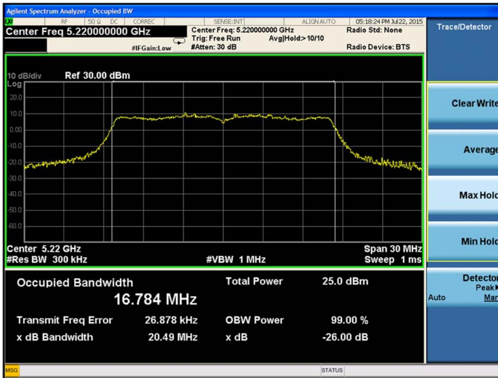
Figure 9-2. 26-dB Emission Bandwidth Chain A 802.11a (Ch. 44)
