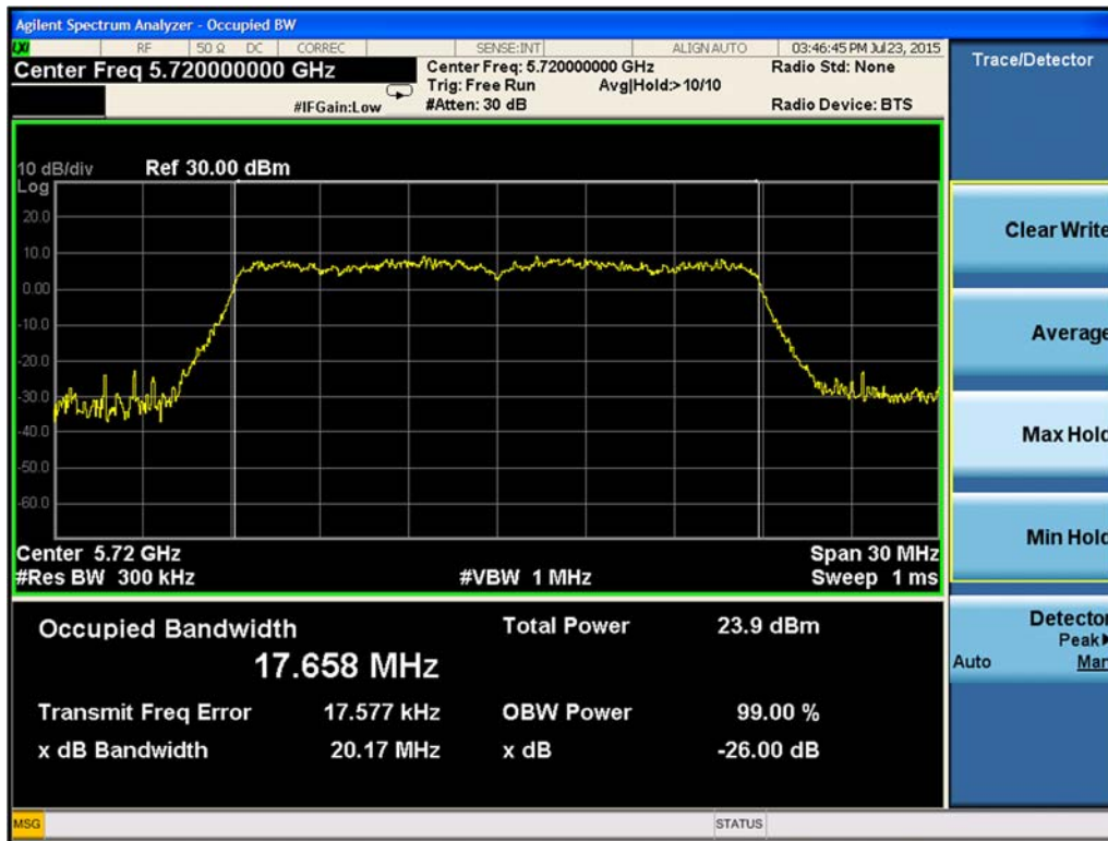
Figure 9-49. 26-dB Emission Bandwidth Chain B 802.11n HT20 (Ch. 144)
