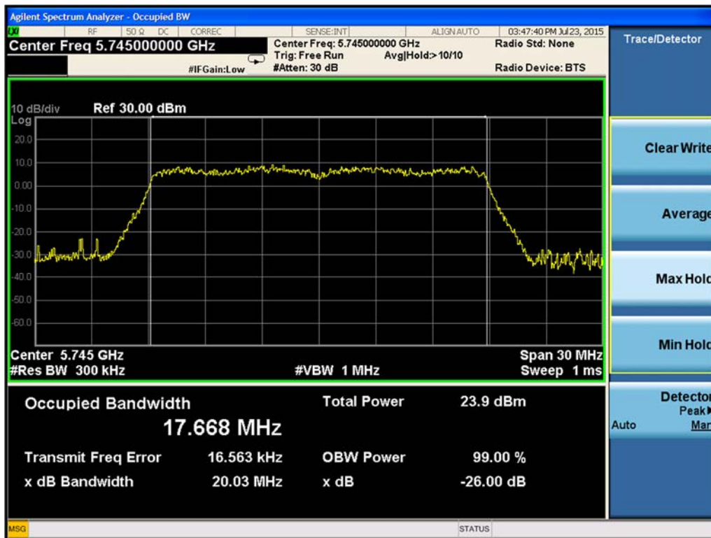
Figure 9-50. 26-dB Emission Bandwidth Chain B 802.11n HT20 (Ch. 149)
