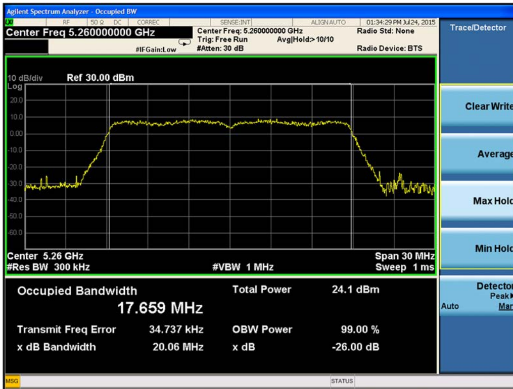
Figure 9-56. 26-dB Emission Bandwidth Chain A 802.11ac VHT20 (Ch. 52)
