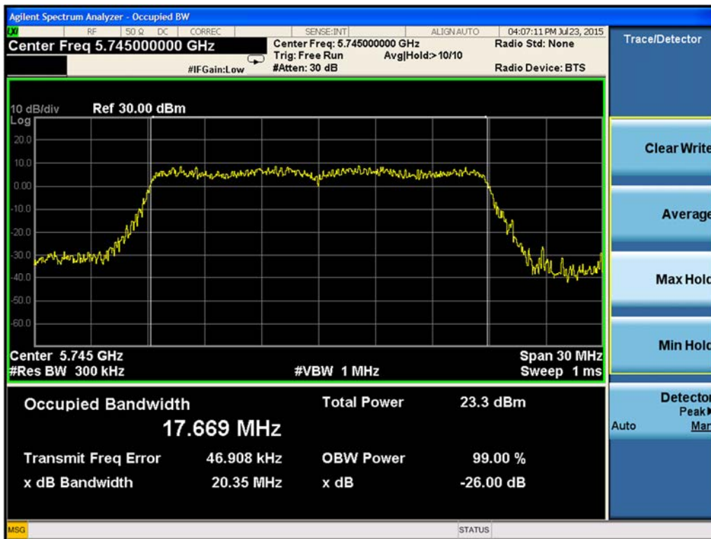
Figure 9-37. 26-dB Emission Bandwidth Chain A 802.11n HT20 (Ch. 149)
