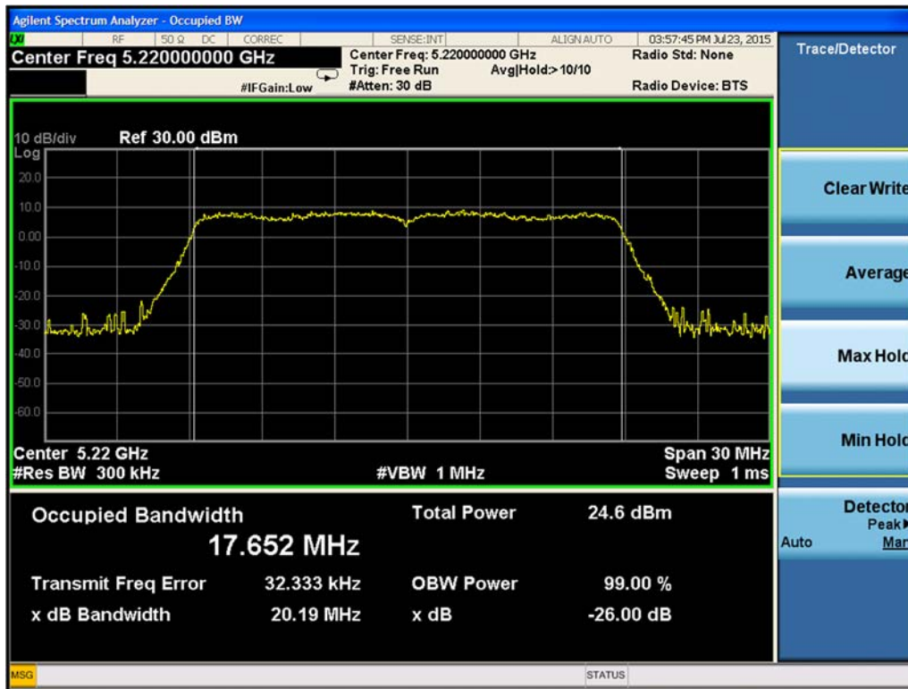
Figure 9-28. 26-dB Emission Bandwidth Chain A 802.11n HT20 (Ch. 44)
