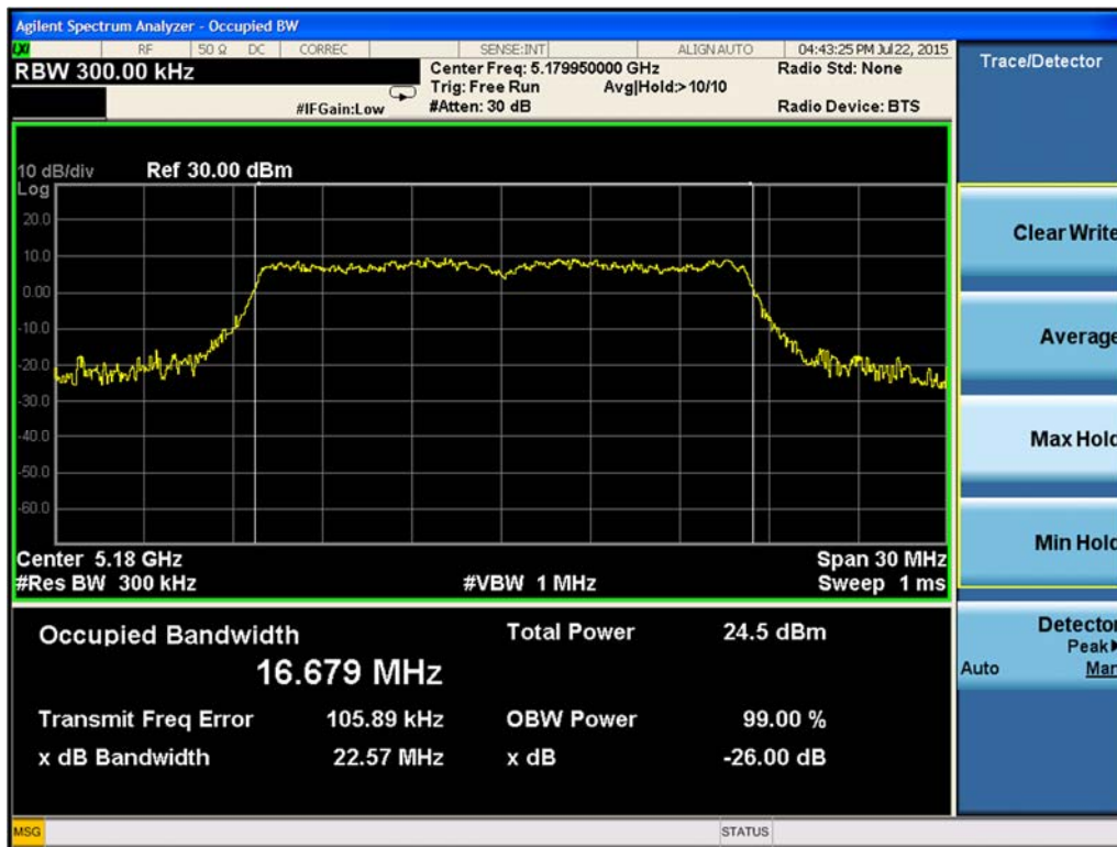
Figure 9-14. 26-dB Emission Bandwidth Chain B 802.11a (Ch. 36)
