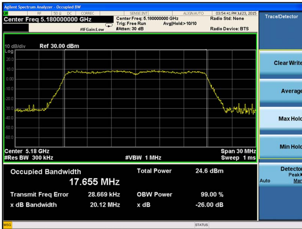
Figure 9-27. 26-dB Emission Bandwidth Chain A 802.11n HT20 (Ch. 36)
