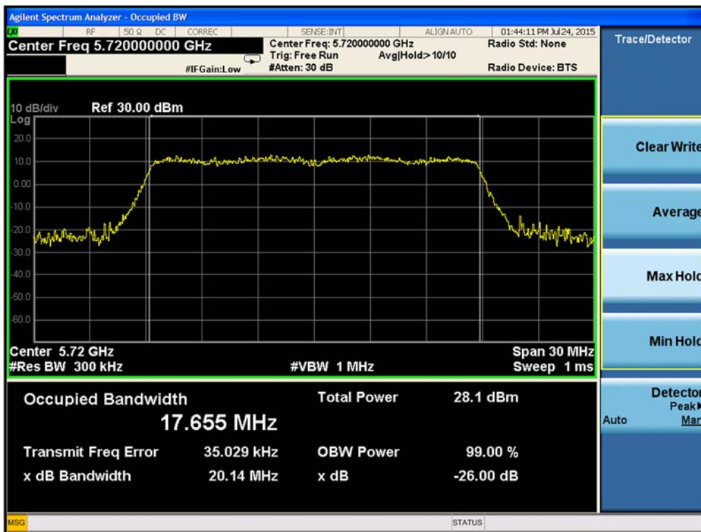
Figure 9-62. 26-dB Emission Bandwidth Chain A 802.11ac VHT20 (Ch. 144)
