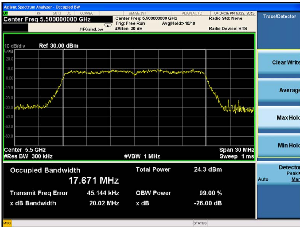
Figure 9-33. 26-dB Emission Bandwidth Chain A 802.11n HT20 (Ch. 100)
