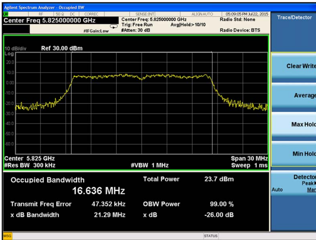
Figure 9-26. 26-dB Emission Bandwidth Chain B 802.11a (Ch. 165)
