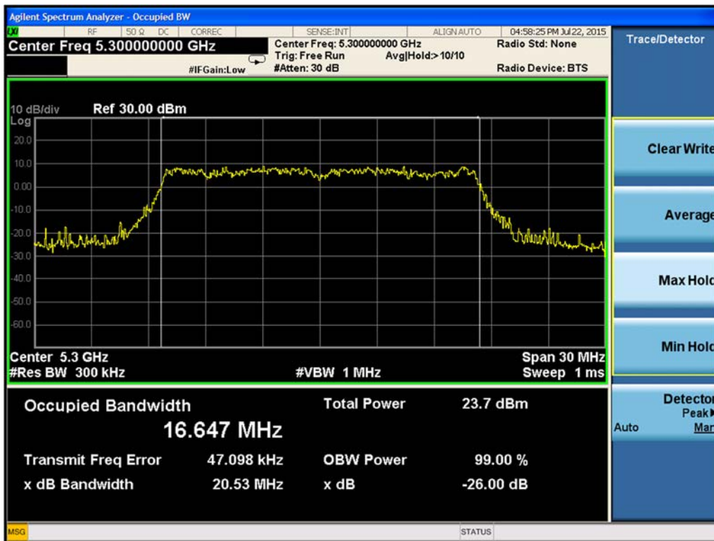
Figure 9-18. 26-dB Emission Bandwidth Chain B 802.11a (Ch. 60)
