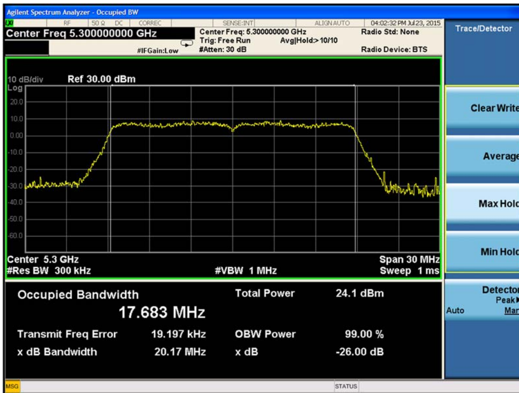
Figure 9-44. 26-dB Emission Bandwidth Chain B 802.11n HT20 (Ch. 60)
