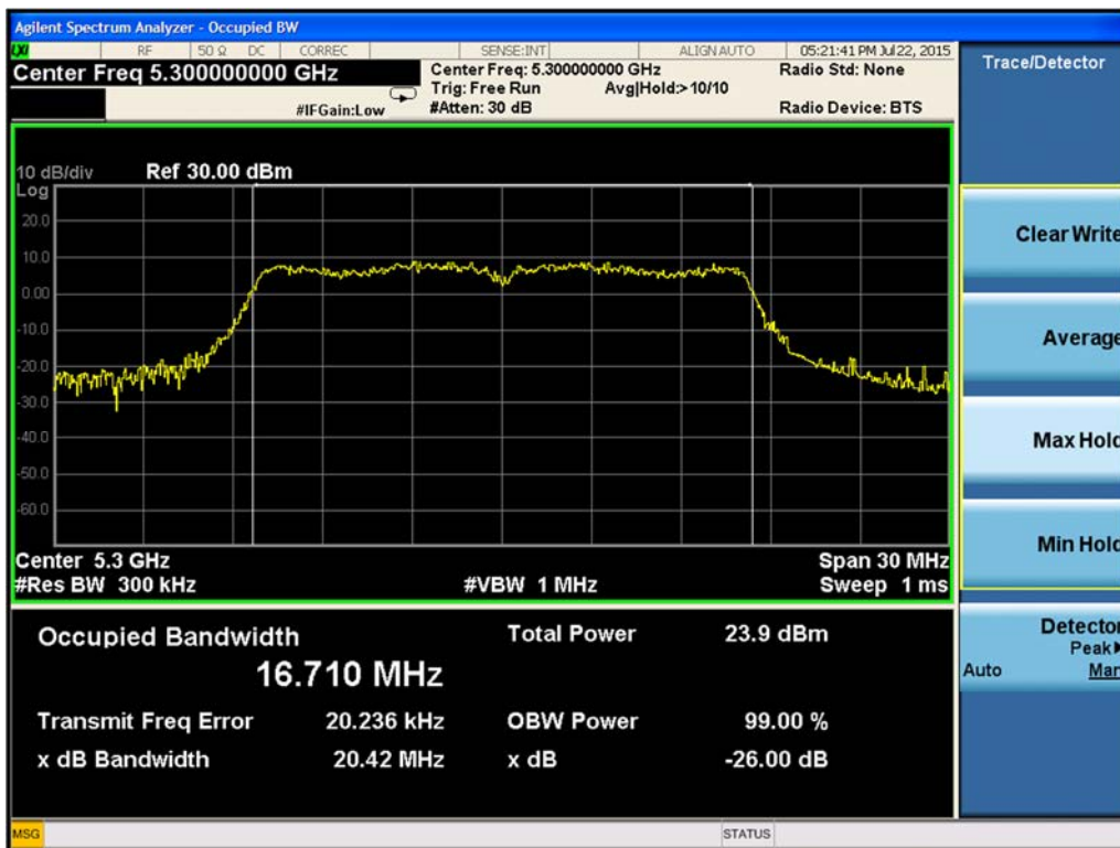
Figure 9-5. 26-dB Emission Bandwidth Chain A 802.11a (Ch. 60)
