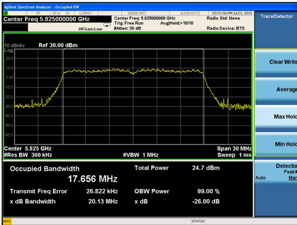
Figure 9-52. 26-dB Emission Bandwidth Chain B 802.11n HT20 (Ch. 165)
