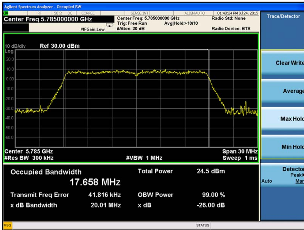
Figure 9-64. 26-dB Emission Bandwidth Chain A 802.11ac VHT20 (Ch. 157)
