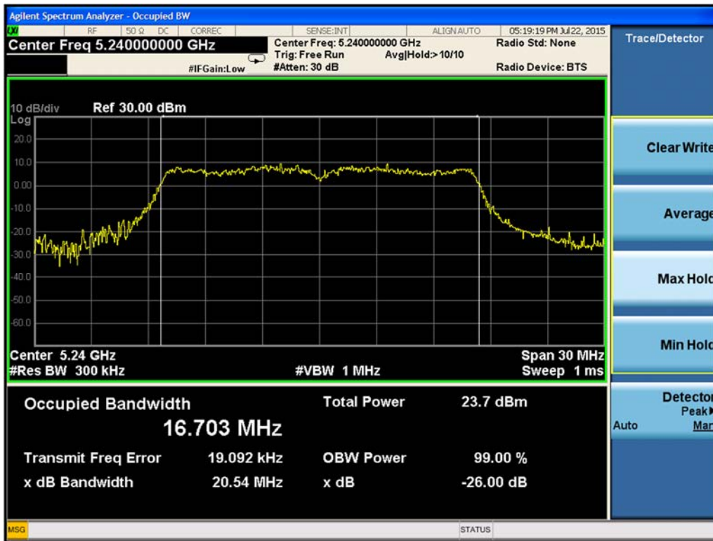
Figure 9-3 26-dB Emission Bandwidth Chain A 802.11a (Ch. 48)
