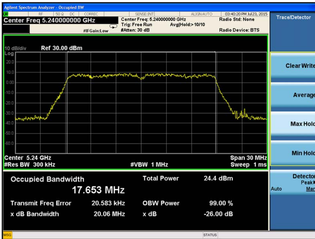
Figure 9-42. 26-dB Emission Bandwidth Chain B 802.11n HT20 (Ch. 48)
