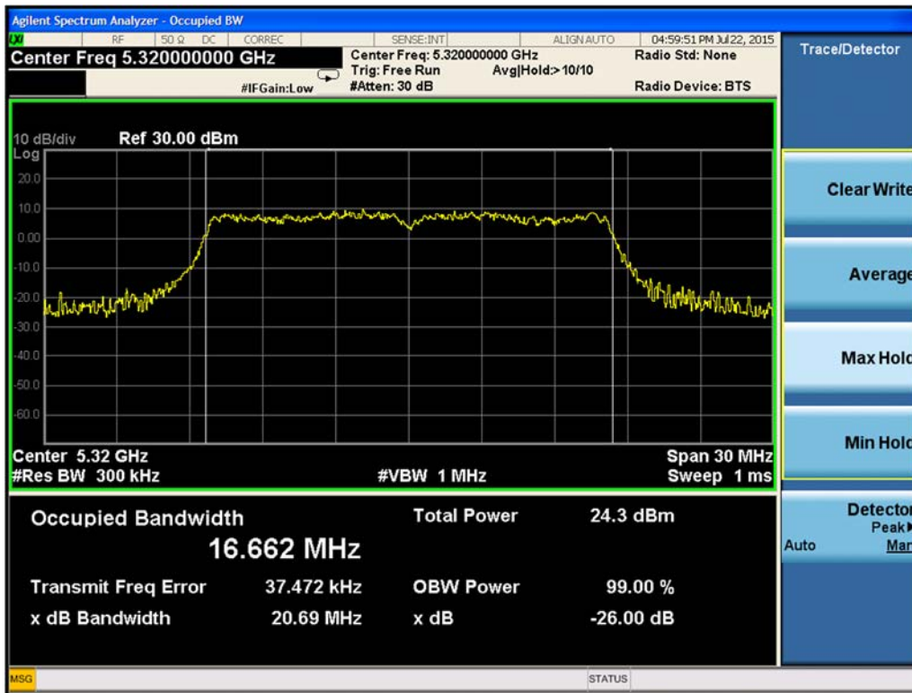
Figure 9-19. 26-dB Emission Bandwidth Chain B 802.11a (Ch. 64)
