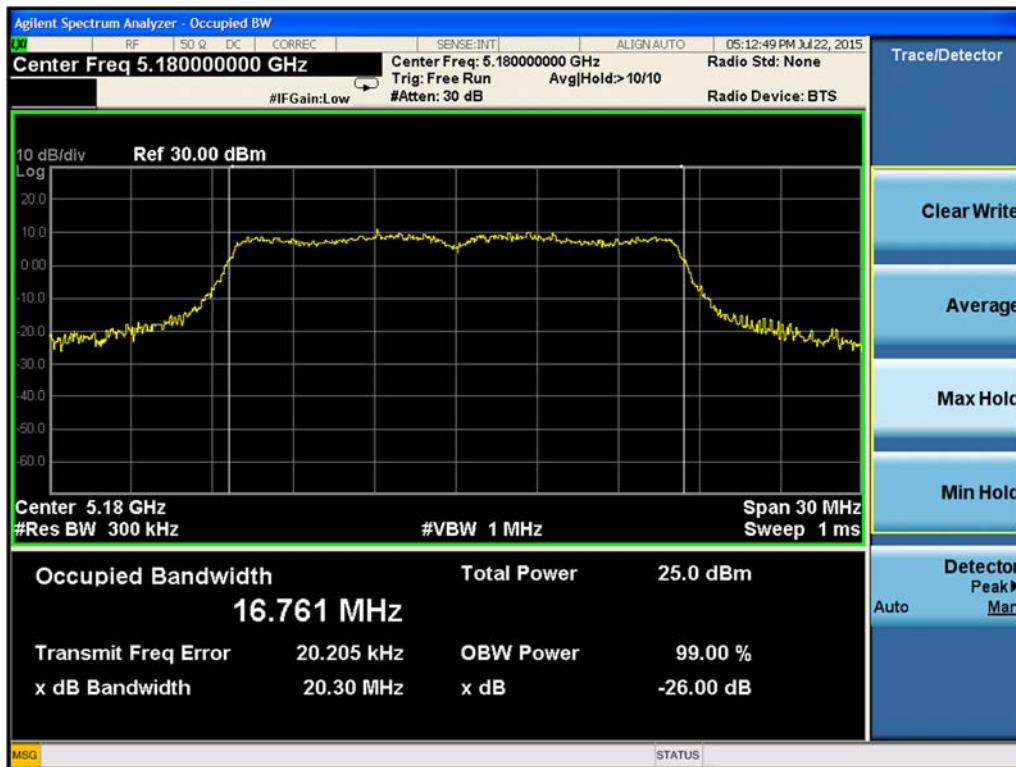
Figure 9-1. 26-dB Emission Bandwidth Chain A 802.11a (Ch. 36)
