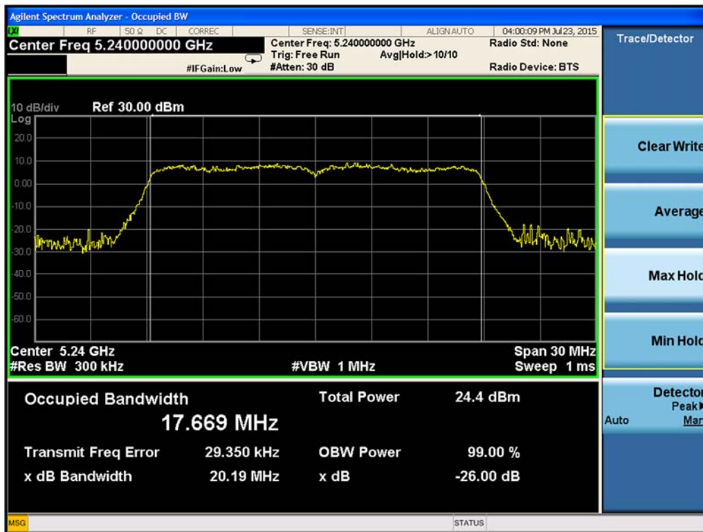
Figure 9-29. 26-dB Emission Bandwidth Chain A 802.11n HT20 (Ch. 48)
