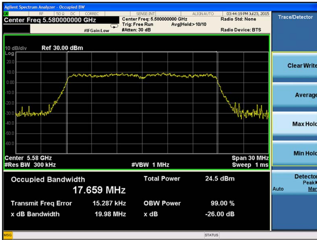
Figure 9-47. 26-dB Emission Bandwidth Chain B 802.11n HT20 (Ch. 116)
