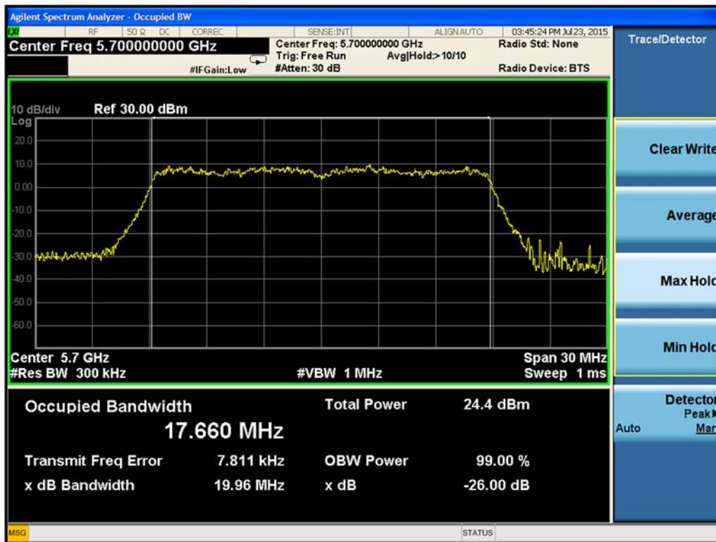
Figure 9-48. 26-dB Emission Bandwidth Chain B 802.11n HT20 (Ch. 140)
