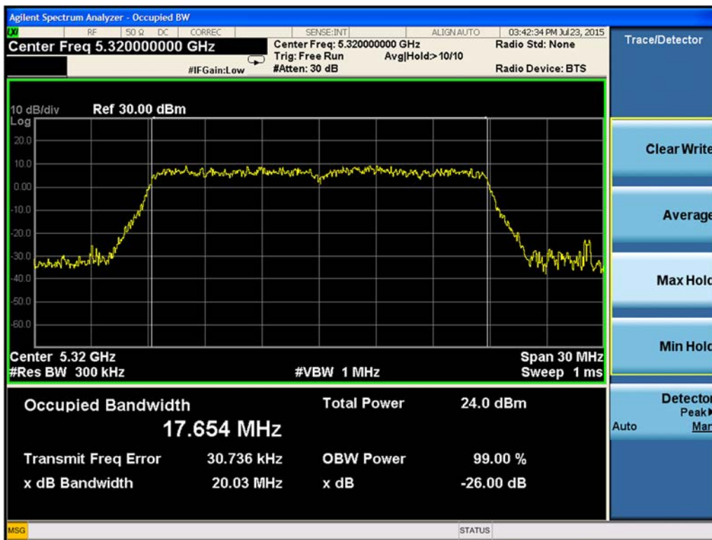
Figure 9-45. 26-dB Emission Bandwidth Chain B 802.11n HT20 (Ch. 64)
