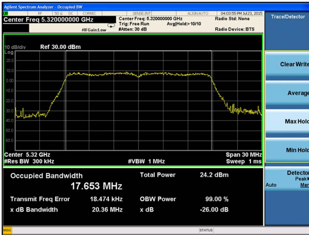
Figure 9-32. 26-dB Emission Bandwidth Chain A 802.11n HT20 (Ch. 64)
