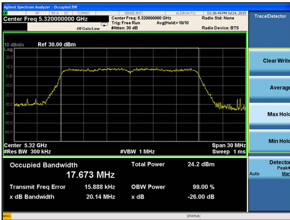
Figure 9-58. 26-dB Emission Bandwidth Chain A 802.11ac VHT20 (Ch. 64)
