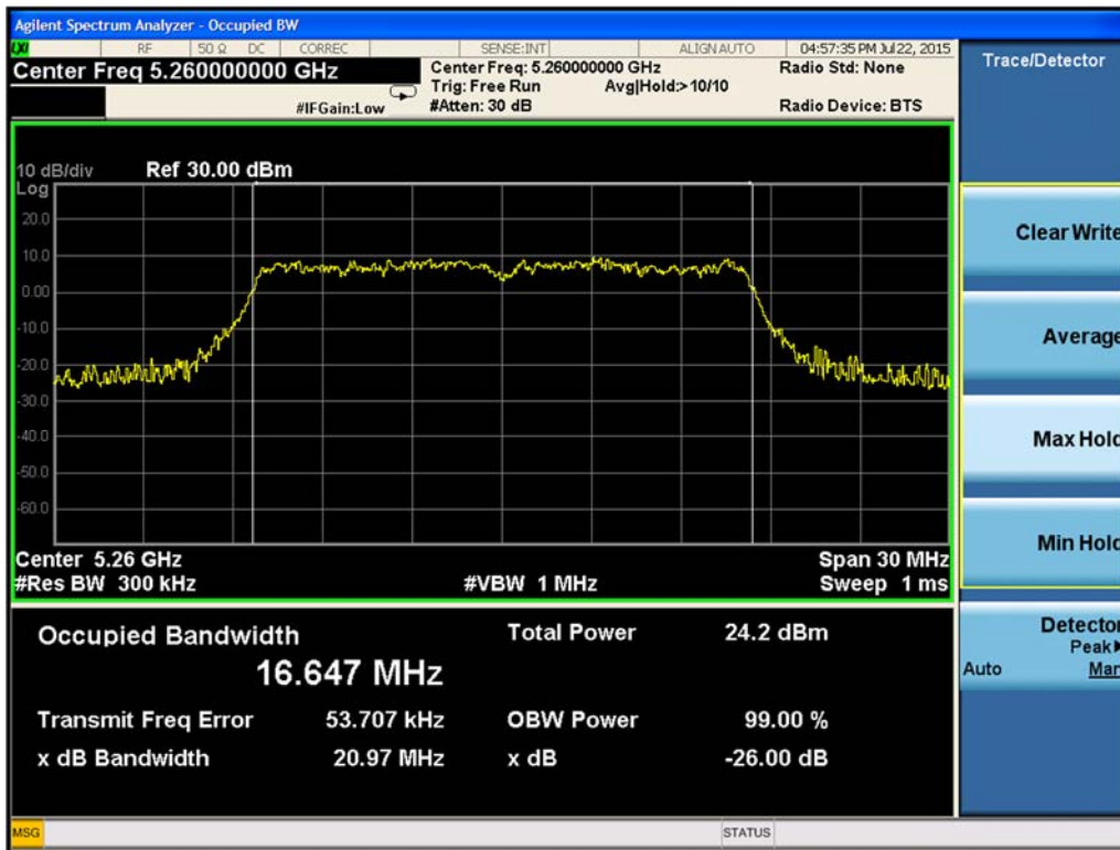
Figure 9-17. 26-dB Emission Bandwidth Chain B 802.11a (Ch. 52)
