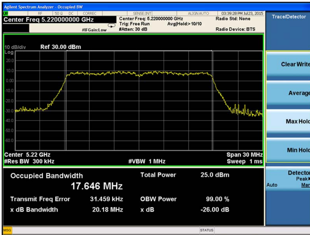
Figure 9-41. 26-dB Emission Bandwidth Chain B 802.11n HT20 (Ch. 44)
