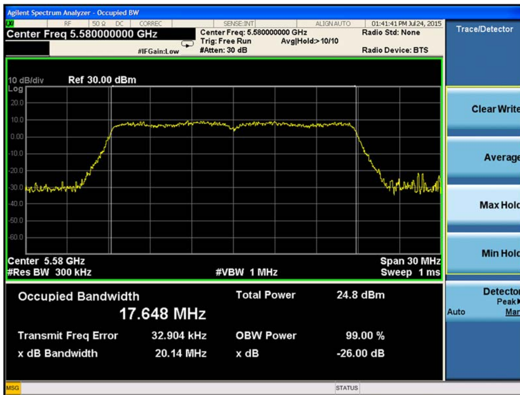
Figure 9-60. 26-dB Emission Bandwidth Chain A 802.11ac VHT20 (Ch. 116)
