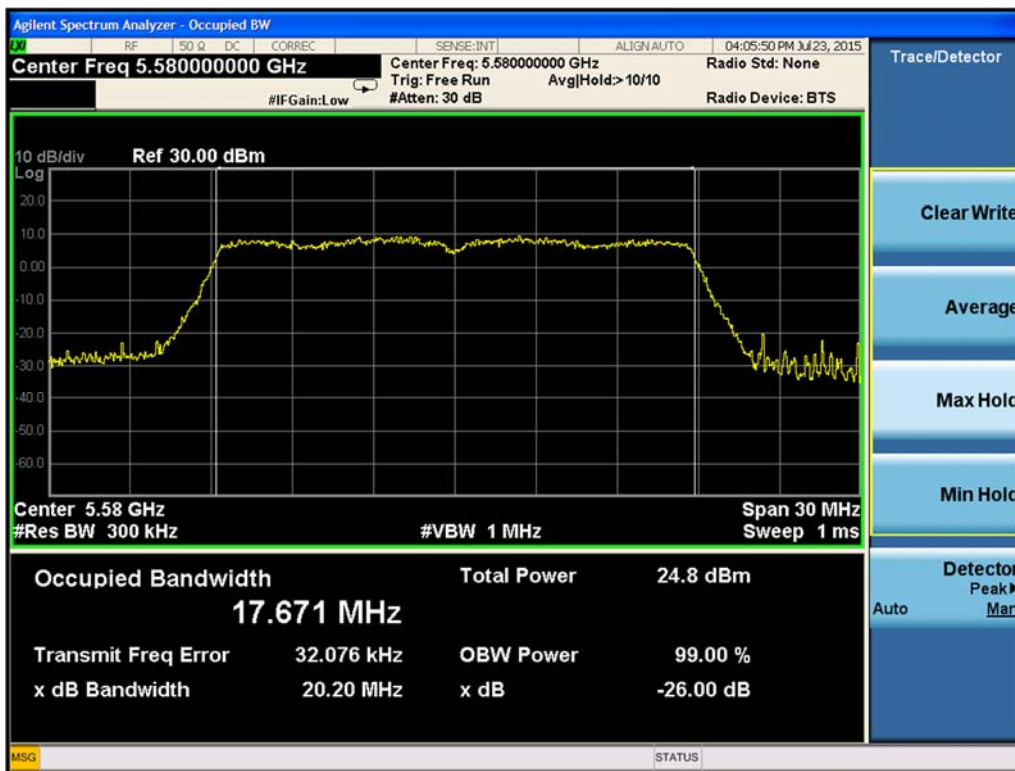
Figure 9-34. 26-dB Emission Bandwidth Chain A 802.11n HT20 (Ch. 116)
