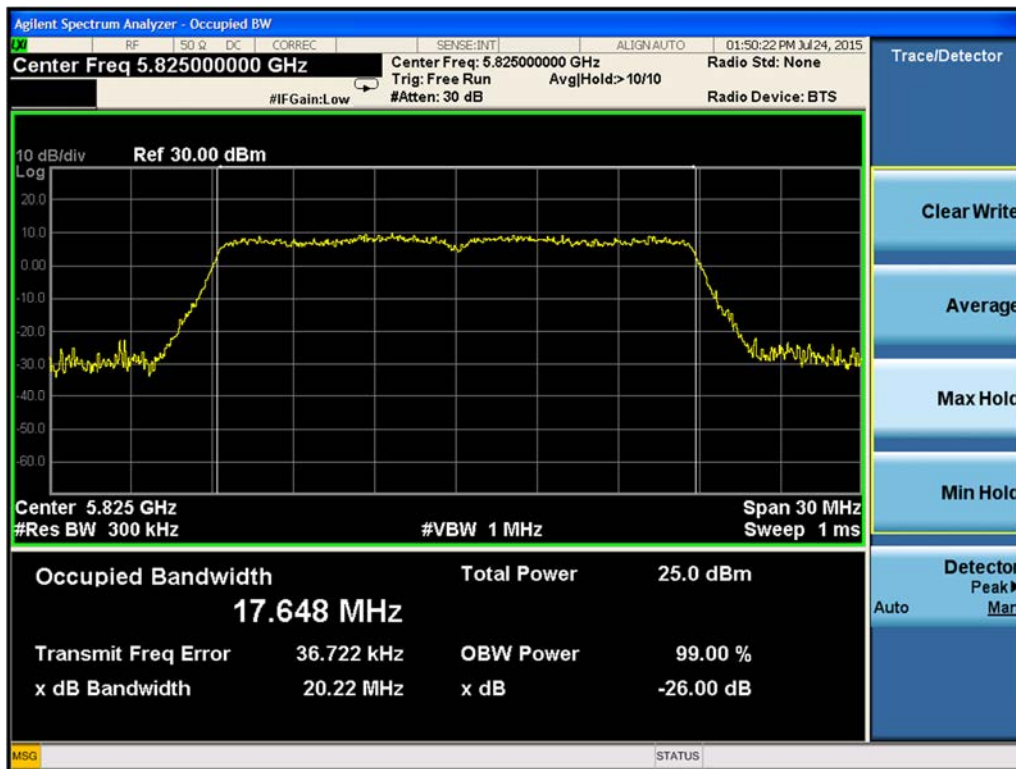
Figure 9-65. 26-dB Emission Bandwidth Chain A 802.11ac VHT20 (Ch. 165)
