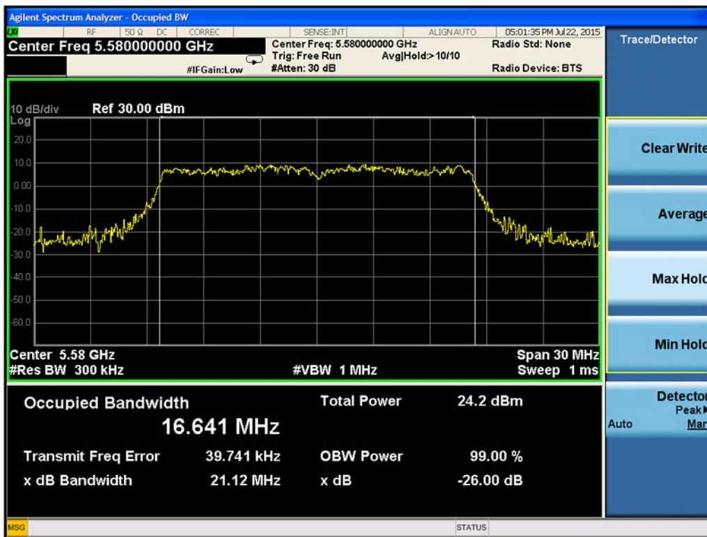
Figure 9-21. 26-dB Emission Bandwidth Chain B 802.11a (Ch. 116)
