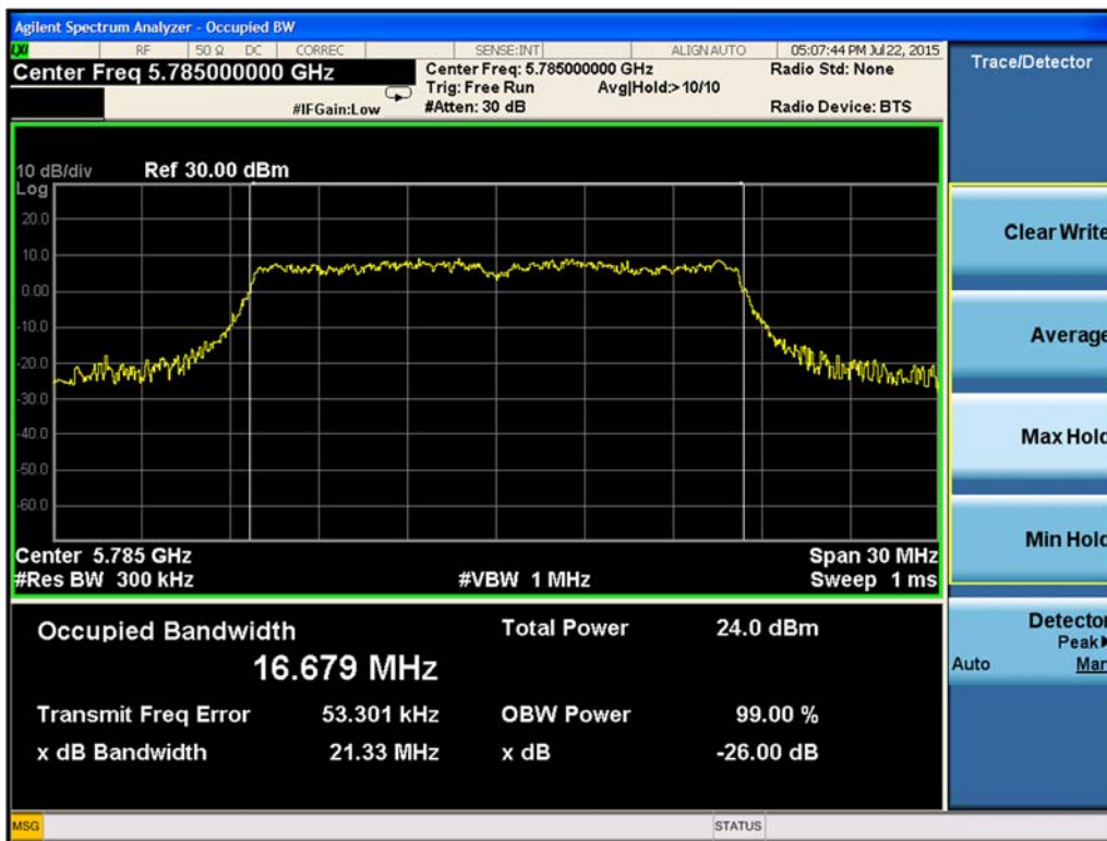
Figure 9-25. 26-dB Emission Bandwidth Chain B 802.11a (Ch. 157)
