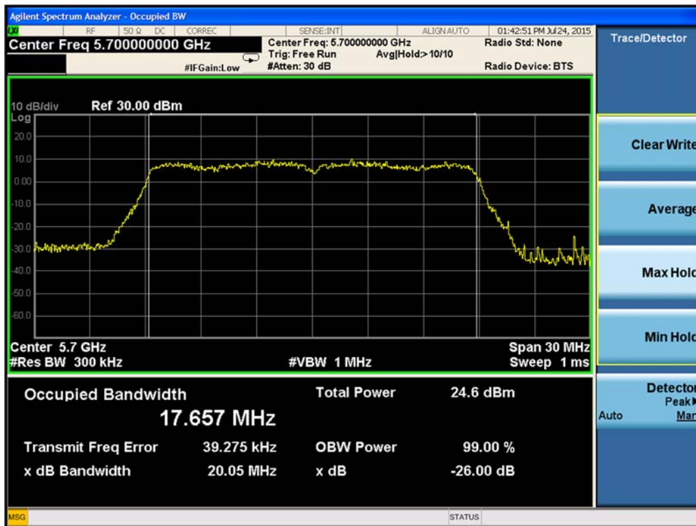
Figure 9-61. 26-dB Emission Bandwidth Chain A 802.11ac VHT20 (Ch. 140)
