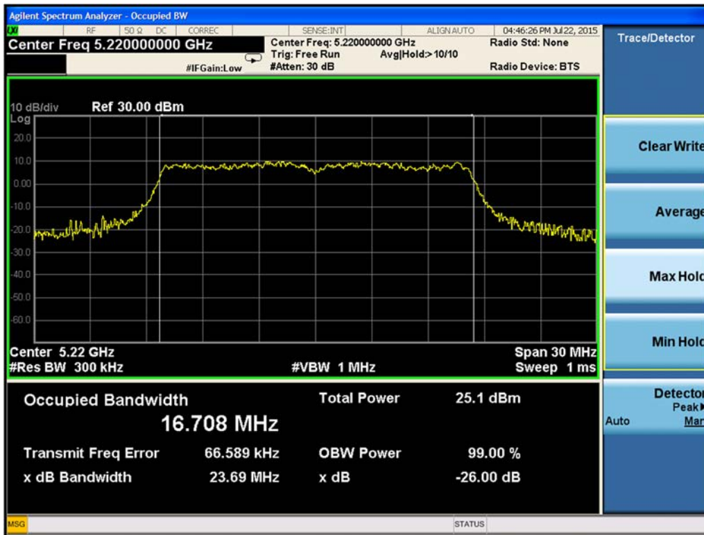
Figure 9-15. 26-dB Emission Bandwidth Chain B 802.11a (Ch. 44)
