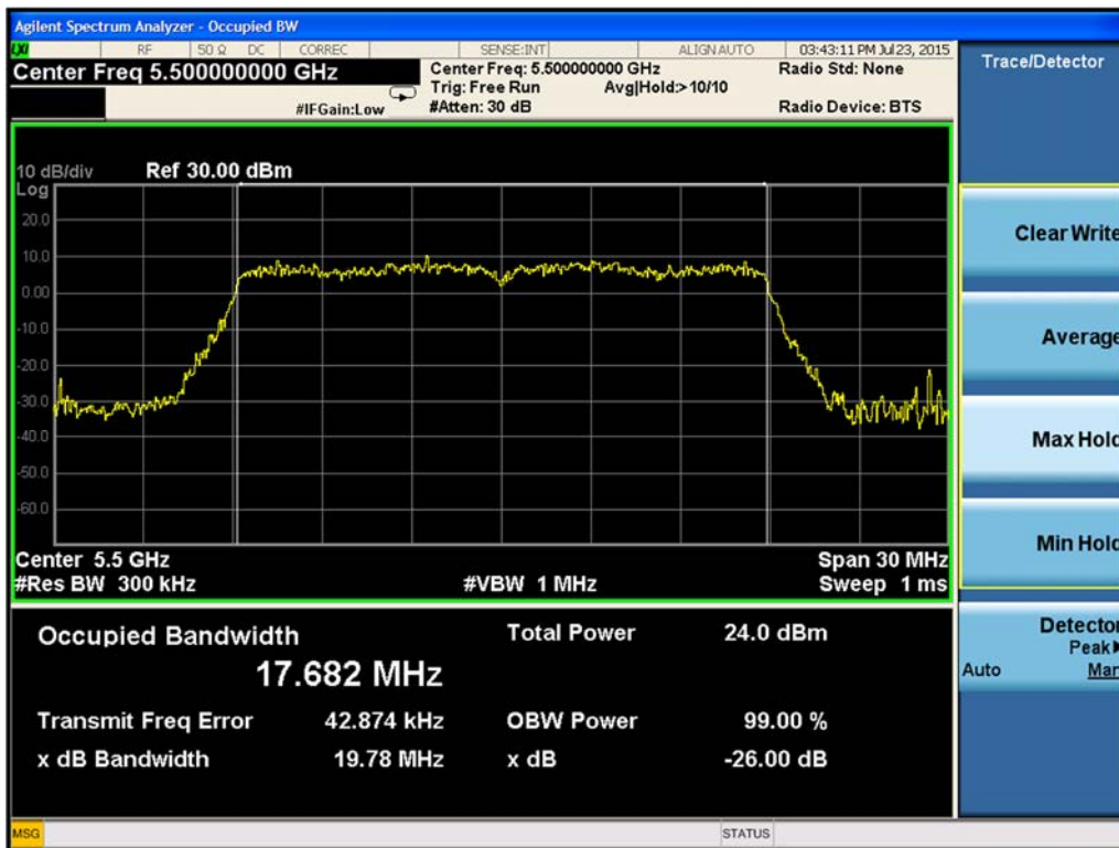
Figure 9-46. 26-dB Emission Bandwidth Chain B 802.11n HT20 (Ch. 100)
