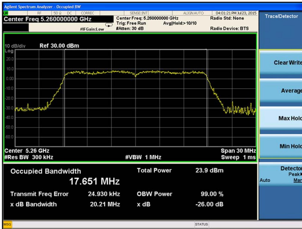
Figure 9-30. 26-dB Emission Bandwidth Chain A 802.11n HT20 (Ch. 52)
