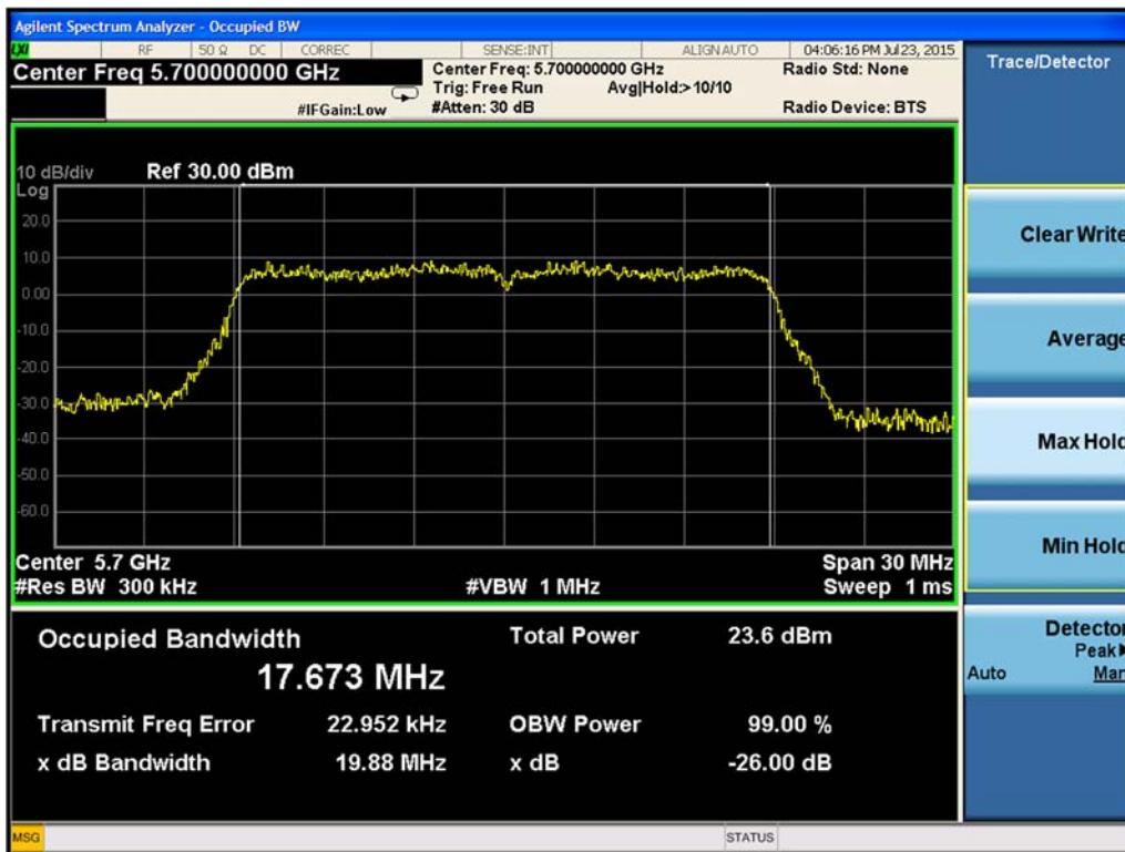
Figure 9-35. 26-dB Emission Bandwidth Chain A 802.11n HT20 (Ch. 140)
