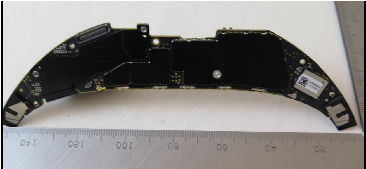
Radio Board – Top with antennae, Removed shield
