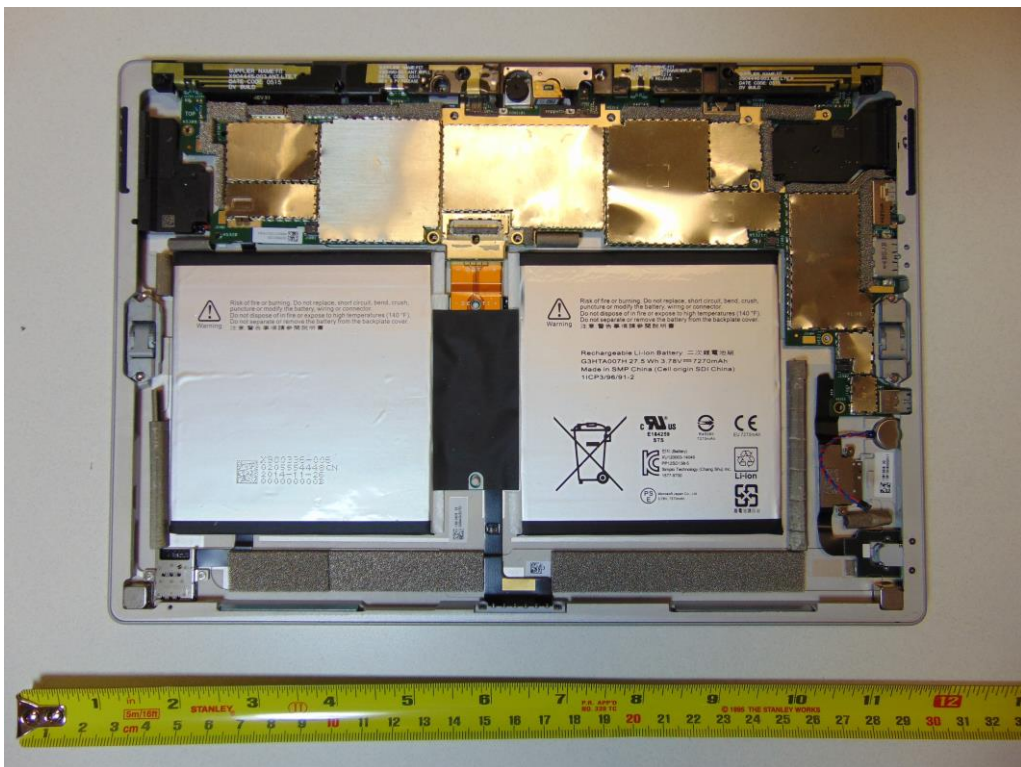
Figure 2 Antenna/Motherboard/Battery
