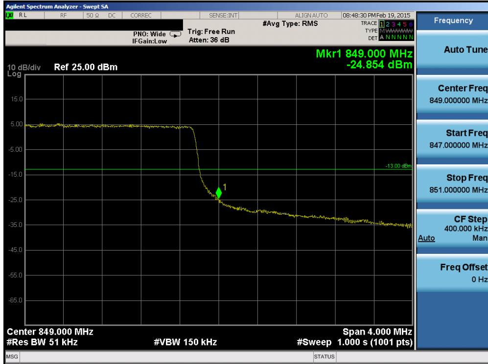
Plot 6-112. Upper Band Edge Plot (Band 5 – 5.0MHz QPSK – RB Size 25)
