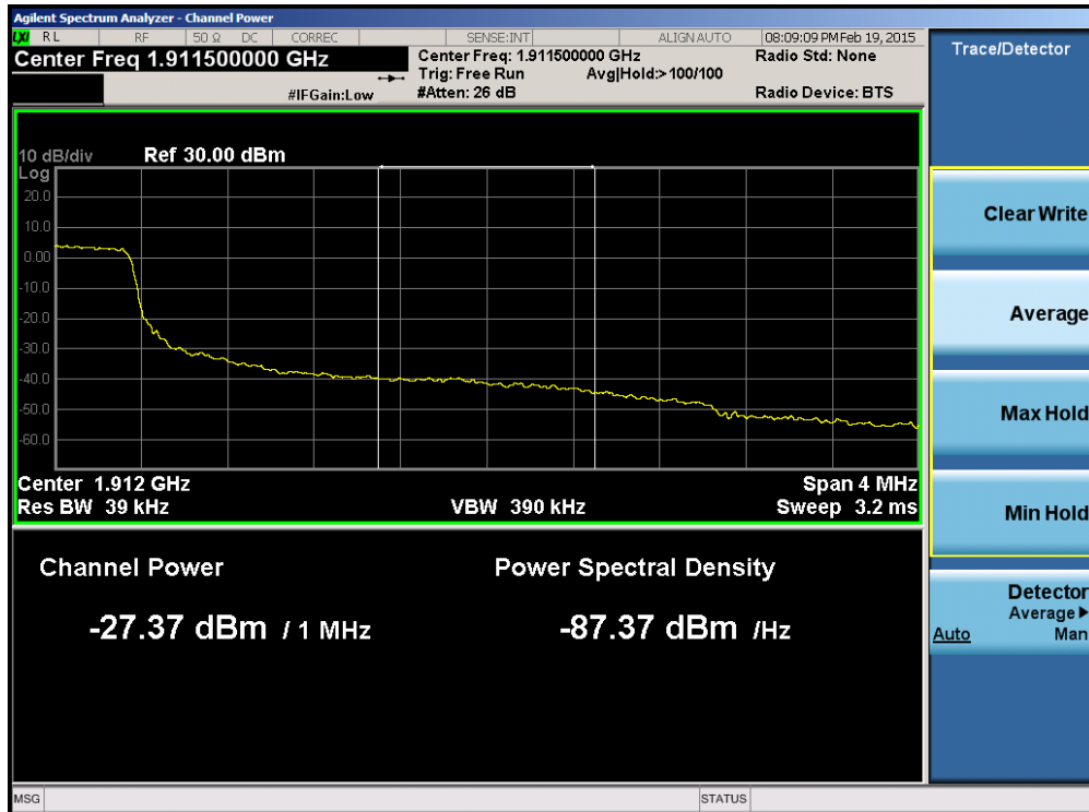
Plot 6-147. Upper Extended Band Edge Plot (Band 2 – 3.0MHz QPSK – RB Size 15)
