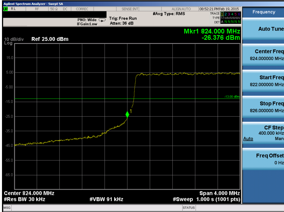
Plot 6-106. Lower Band Edge Plot (Band 5 – 3.0MHz QPSK – RB Size 15)
