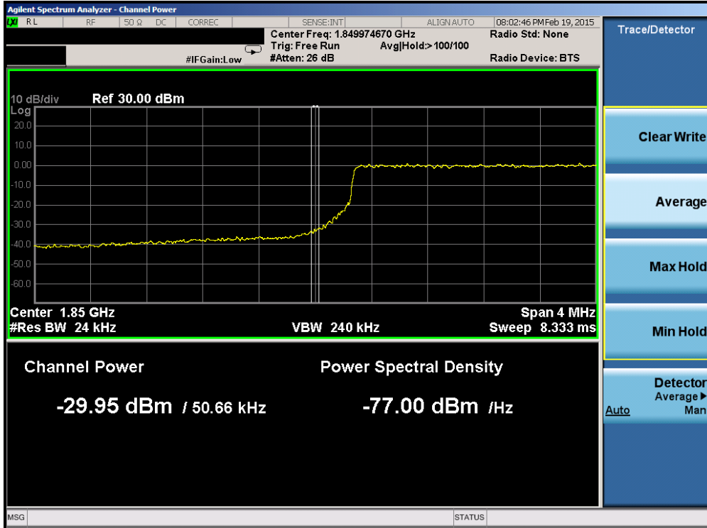
Plot 6-148. Lower Band Edge Plot (Band 2 – 5.0MHz QPSK – RB Size 25)
