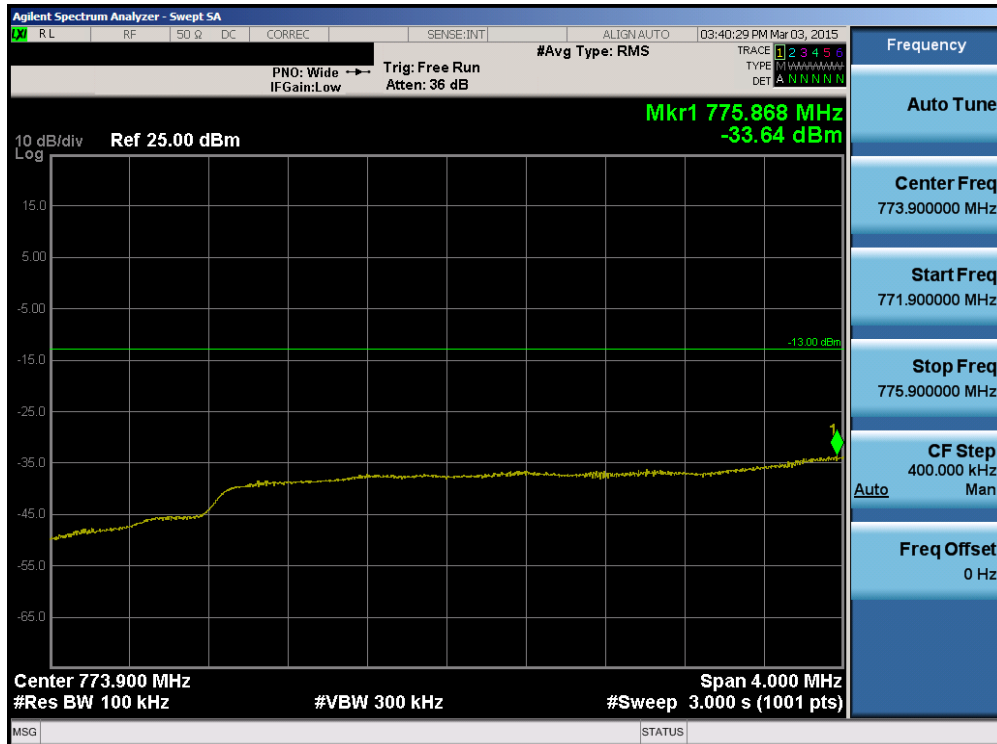
Plot 6-93. Lower Extended Band Edge Plot (Band 13 – 5.0MHz QPSK – RB Size 25)
