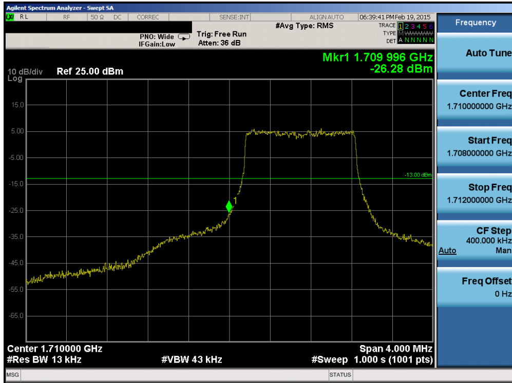
Plot 6-116. Lower Band Edge Plot (Band 4 – 1.4MHz QPSK – RB Size 6)
