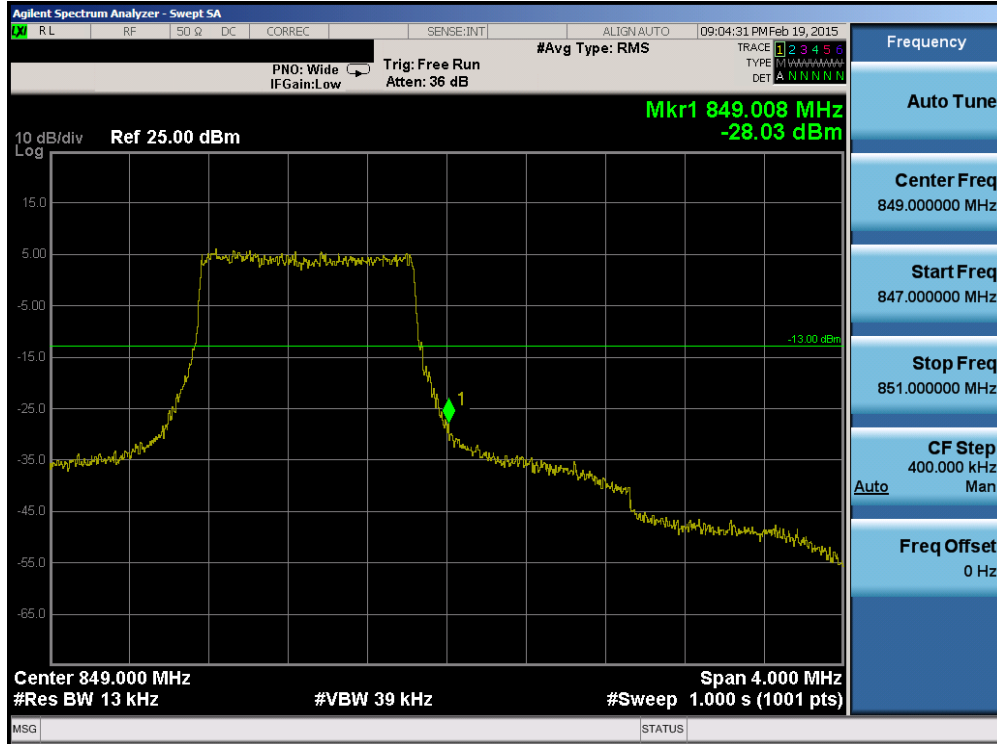
Plot 6-104. Upper Band Edge Plot (Band 5 – 1.4MHz QPSK – RB Size 6)
