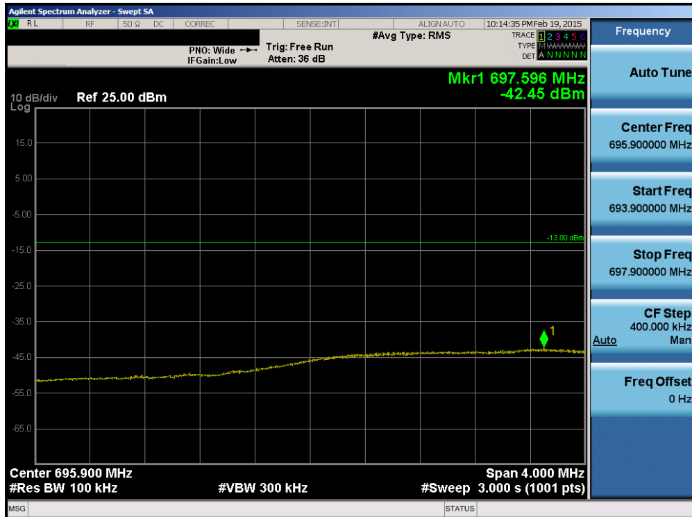
Plot 6-87. Lower Extended Band Edge Plot (Band 17 – 5.0MHz QPSK – RB Size 25)
