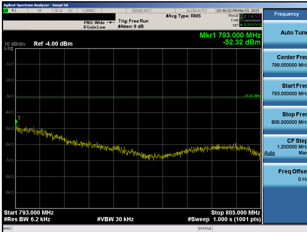
Plot 6-101. Upper Emission Mask Plot (Band 13 – 10.0MHz QPSK – RB Size 50)
