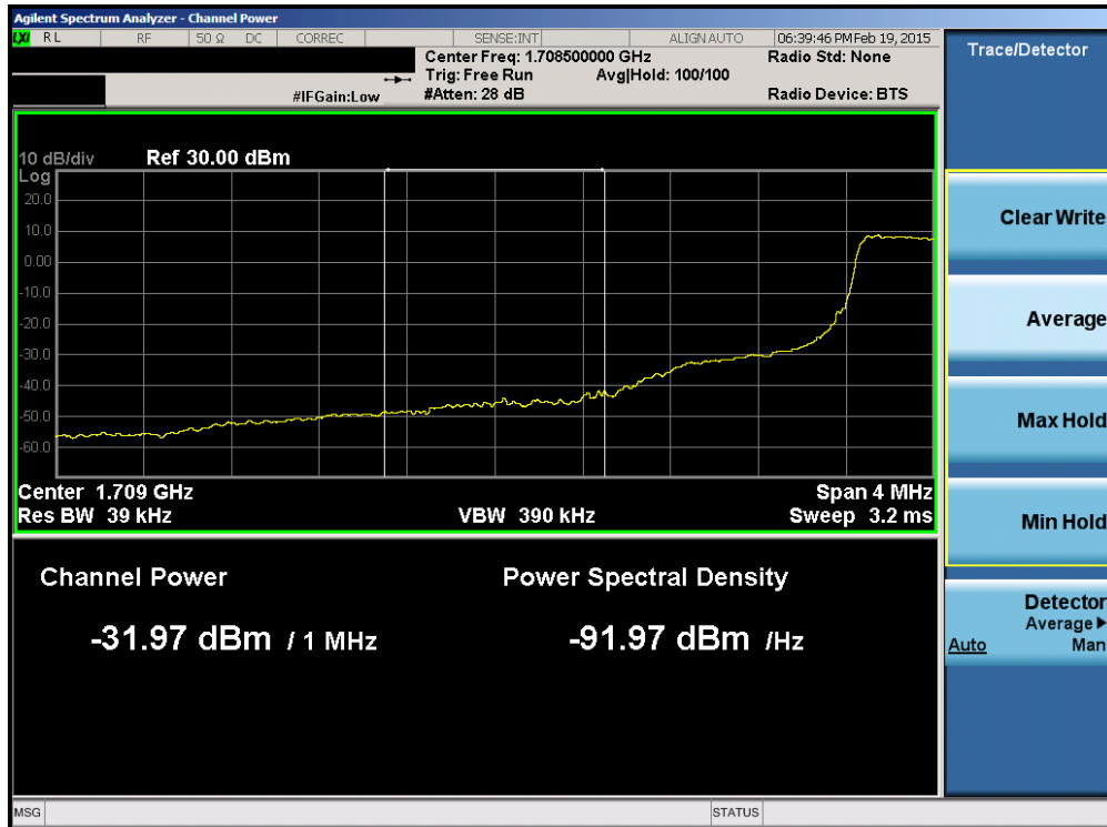
Plot 6-117. Lower Extended Band Edge Plot (Band 4 – 1.4MHz QPSK – RB Size 6)
