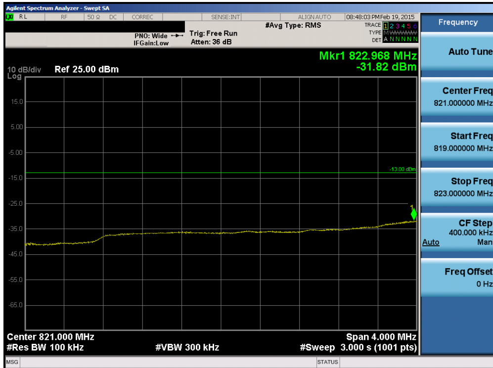
Plot 6-111. Lower Extended Band Edge Plot (Band 5 – 5.0MHz QPSK – RB Size 25)
