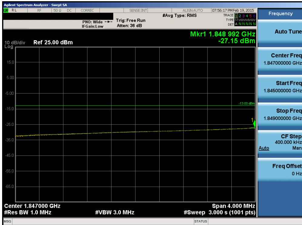
Plot 6-161. Lower Extended Band Edge Plot (Band 2 – 20.0MHz QPSK – RB Size 100)
