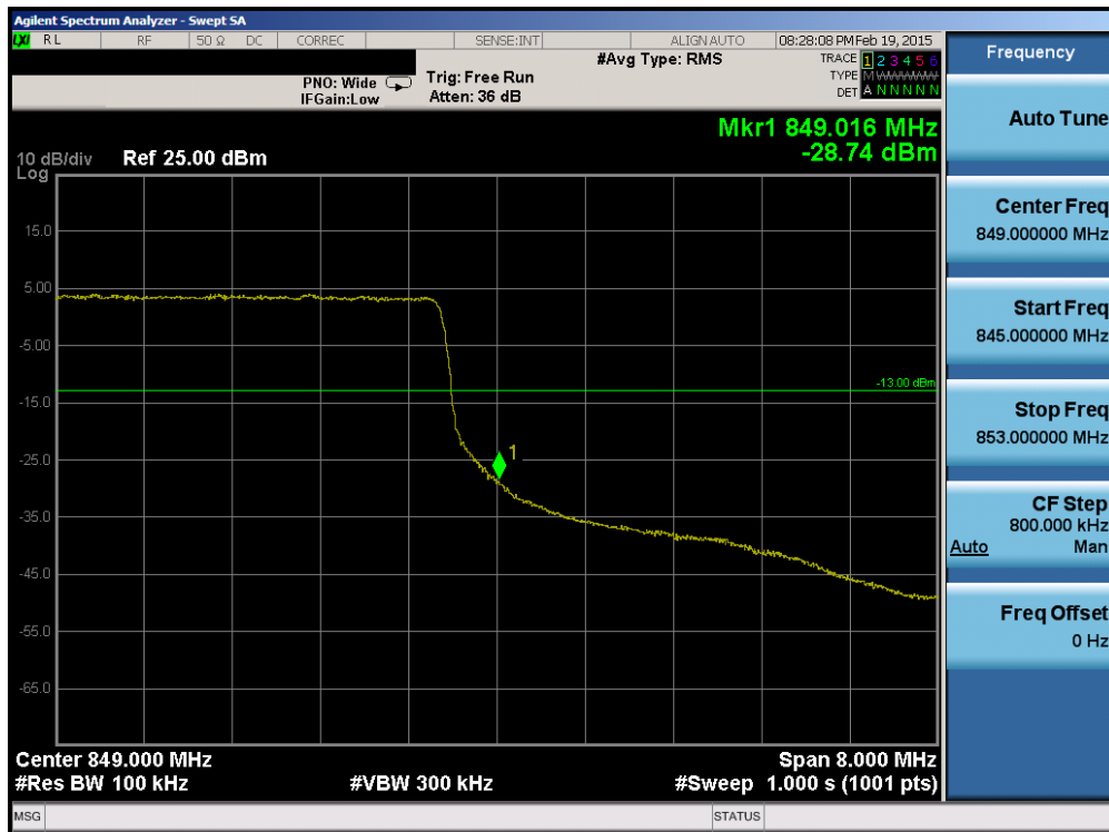
Plot 6-115. Upper Band Edge Plot (Band 5 – 10.0MHz QPSK – RB Size 50)
