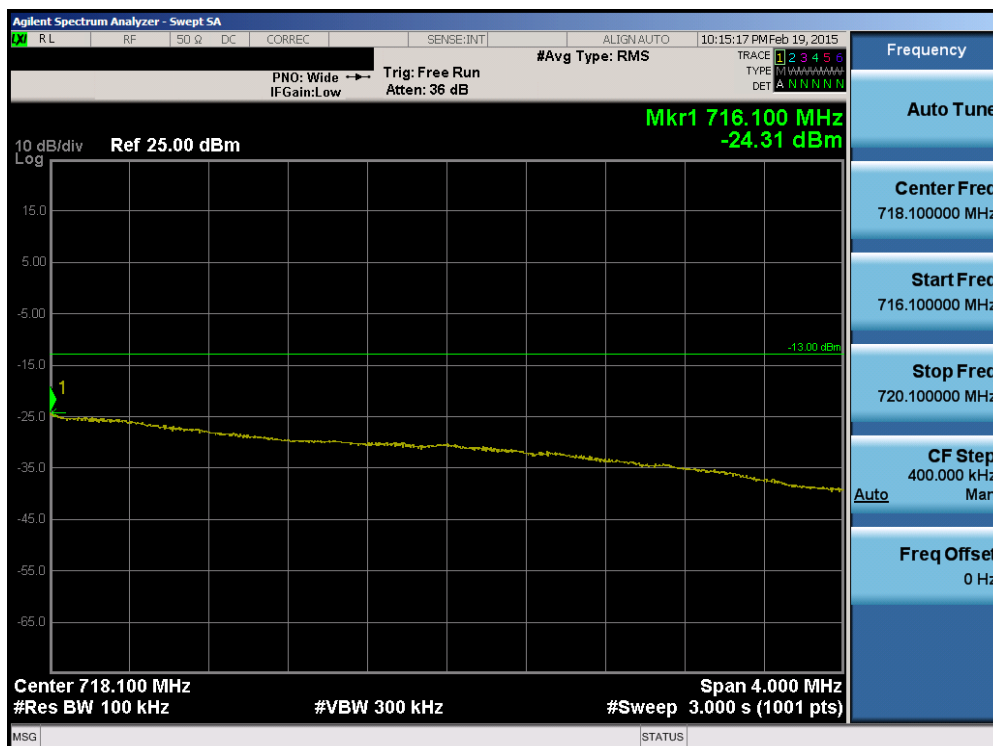
Plot 6-89. Upper Extended Band Edge Plot (Band 17 – 5.0MHz QPSK – RB Size 25)
