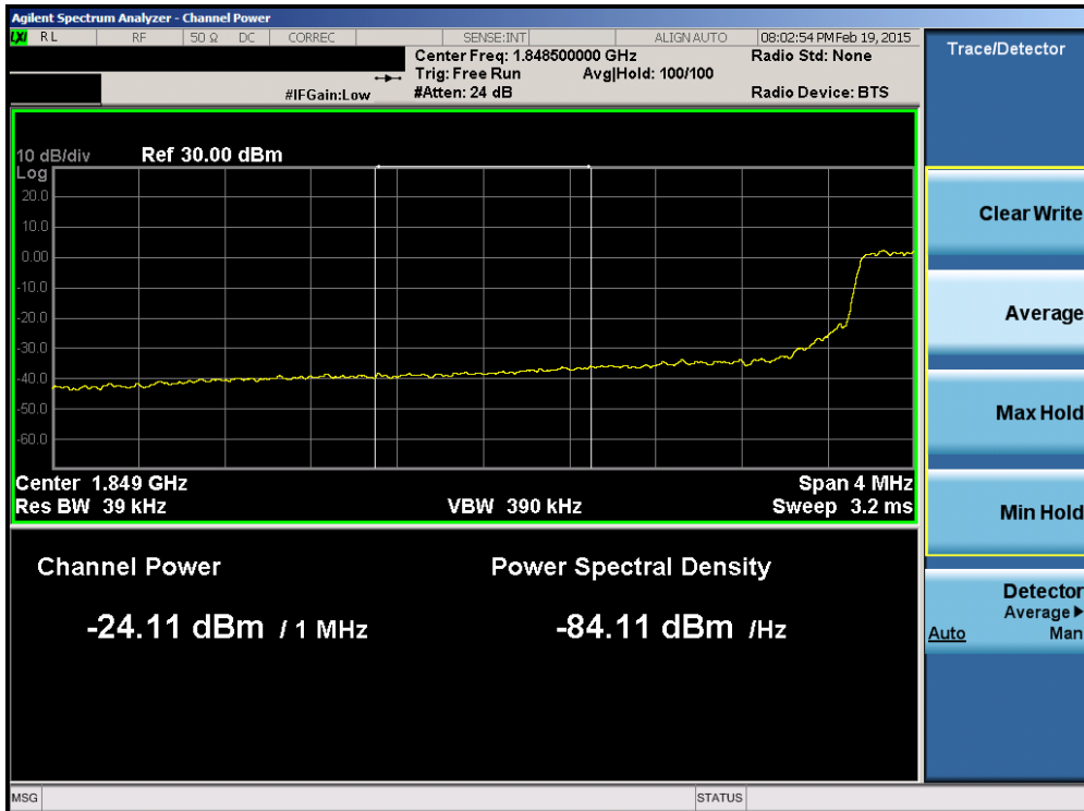
Plot 6-149. Lower Extended Band Edge Plot (Band 2 – 5.0MHz QPSK – RB Size 25)
