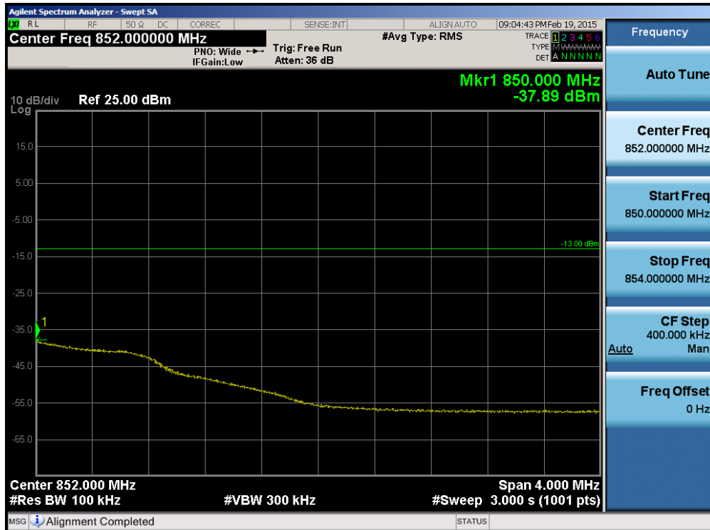
Plot 6-105. Upper Extended Band Edge Plot (Band 5 – 1.4MHz QPSK – RB Size 6)
