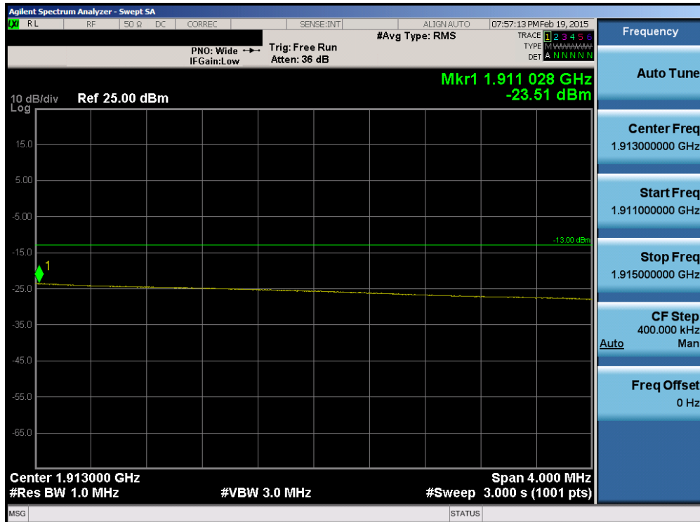
Plot 6-163. Upper Extended Band Edge Plot (Band 2 – 20.0MHz QPSK – RB Size 100)
