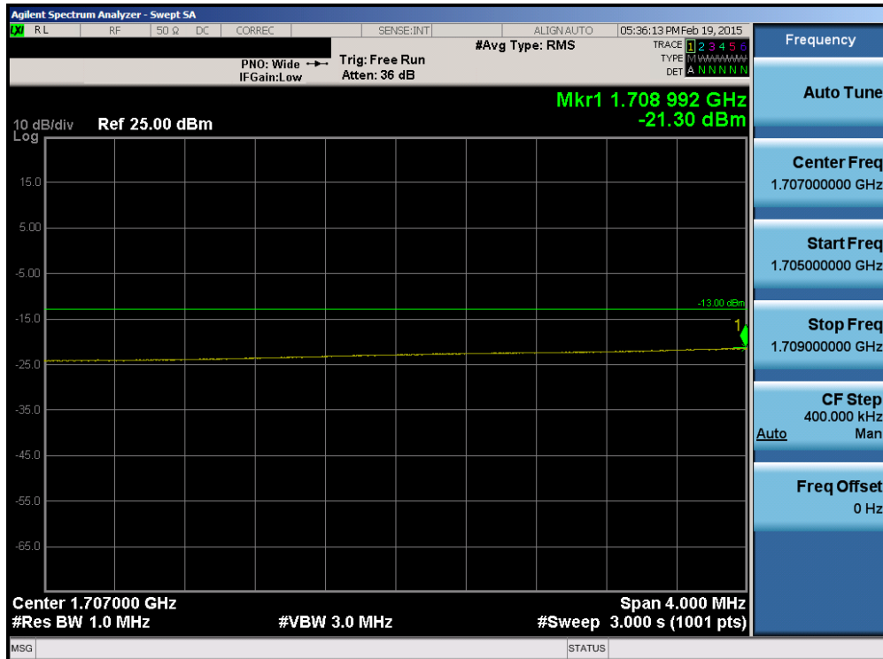
Plot 6-137. Lower Extended Band Edge Plot (Band 4 – 20.0MHz QPSK – RB Size 100)
