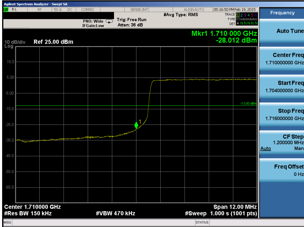
Plot 6-132. Lower Band Edge Plot (Band 4 – 15.0MHz QPSK – RB Size 75)
