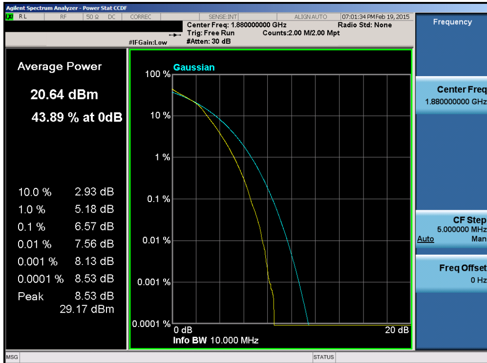
Plot 6-171. PAR Plot (Band 2 – 10.0MHz 16-QAM – RB Size 50)
