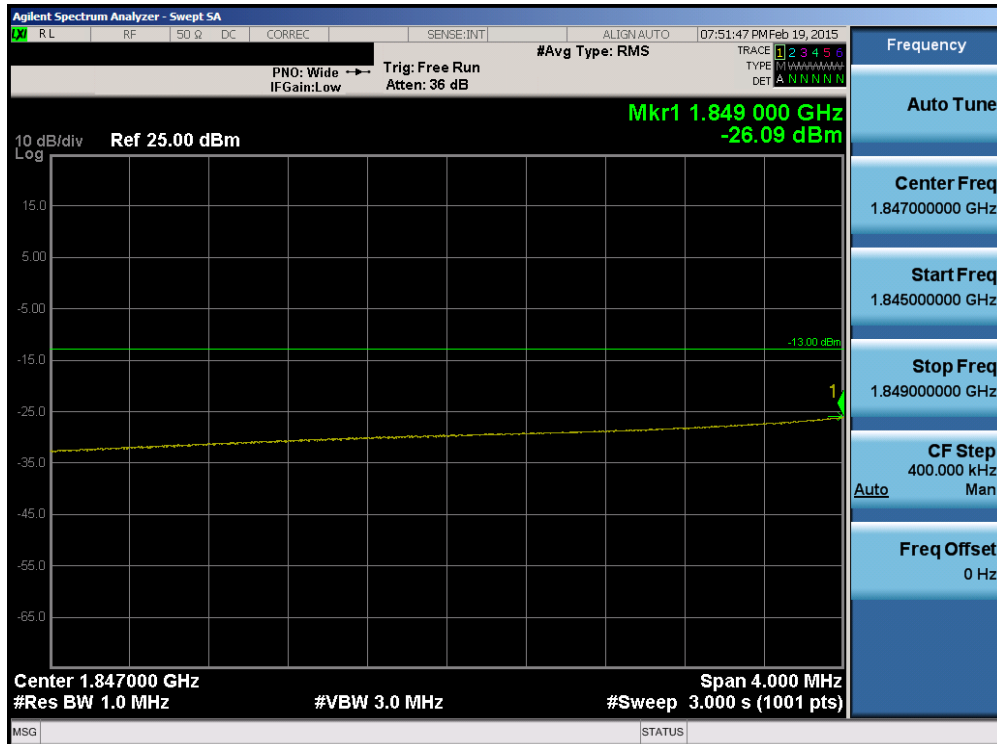
Plot 6-157. Lower Extended Band Edge Plot (Band 2 – 15.0MHz QPSK – RB Size 75)
