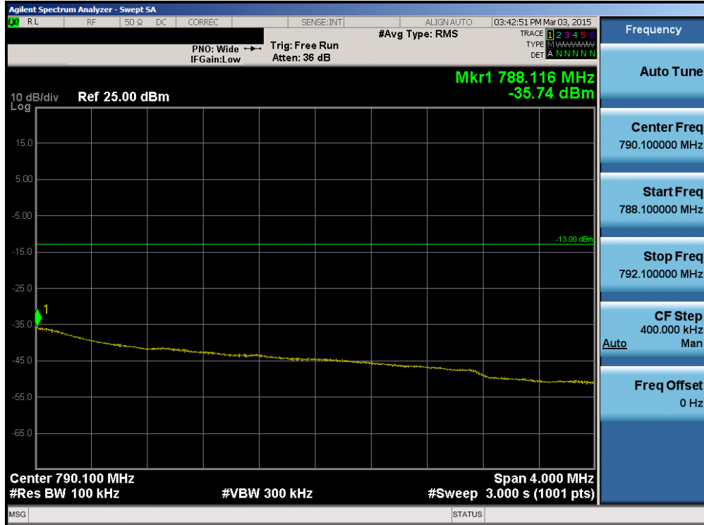
Plot 6-96. Upper Extended Band Edge Plot (Band 13 – 5.0MHz QPSK – RB Size 25)
