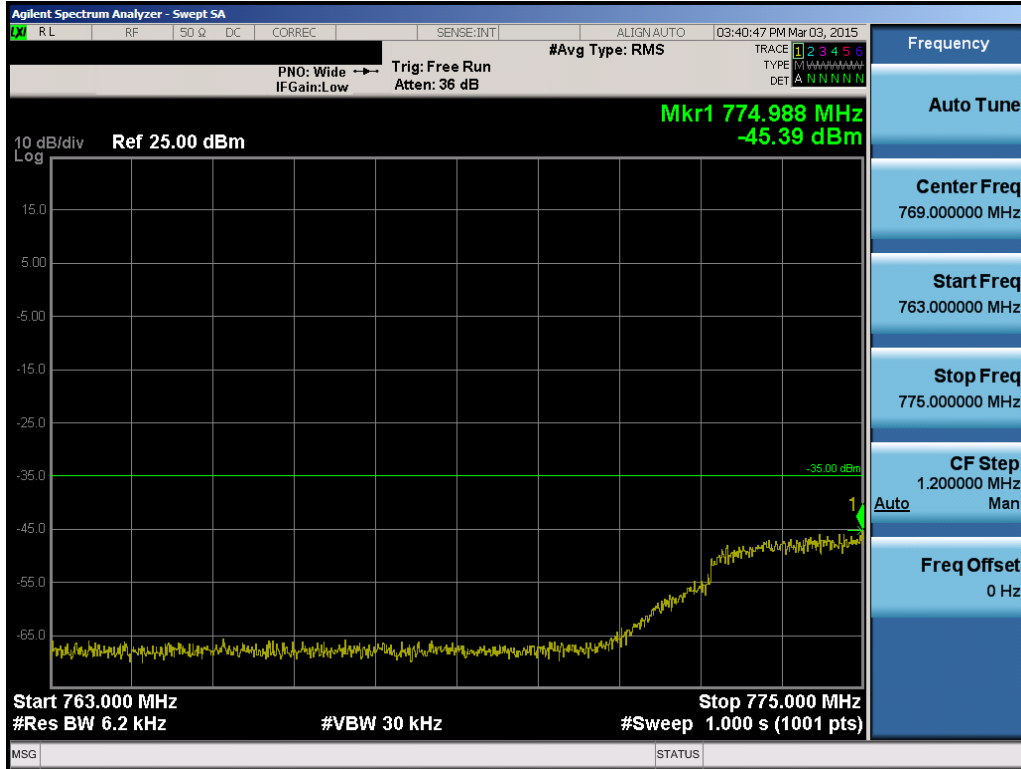
Plot 6-94. Lower Emission Mask Plot (Band 13 – 5.0MHz QPSK – RB Size 25)
