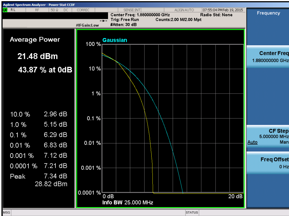
Plot 6-175. PAR Plot (Band 2 – 20.0MHz 16-QAM – RB Size 100)
