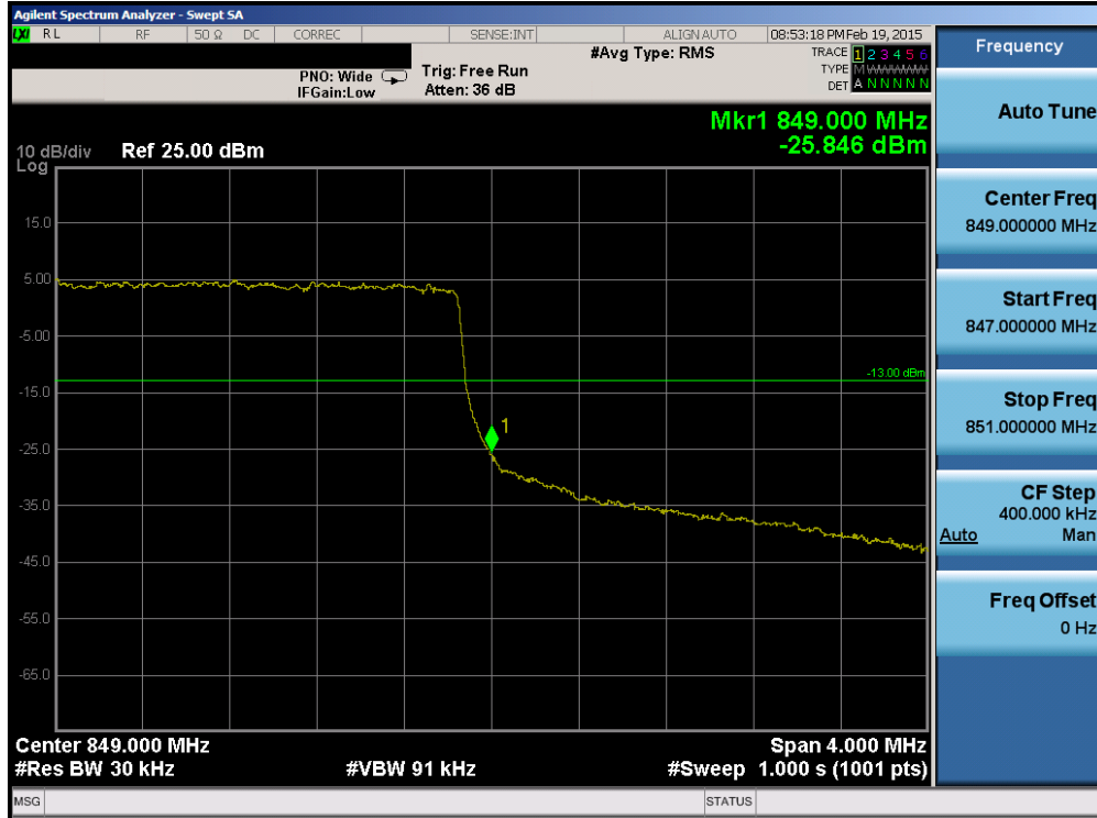
Plot 6-108. Upper Band Edge Plot (Band 5 – 3.0MHz QPSK – RB Size 15)
