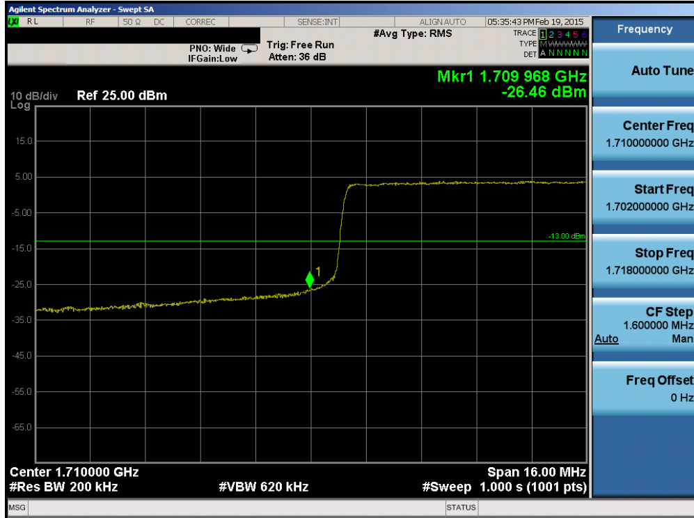
Plot 6-136. Lower Band Edge Plot (Band 4 – 20.0MHz QPSK – RB Size 100)
