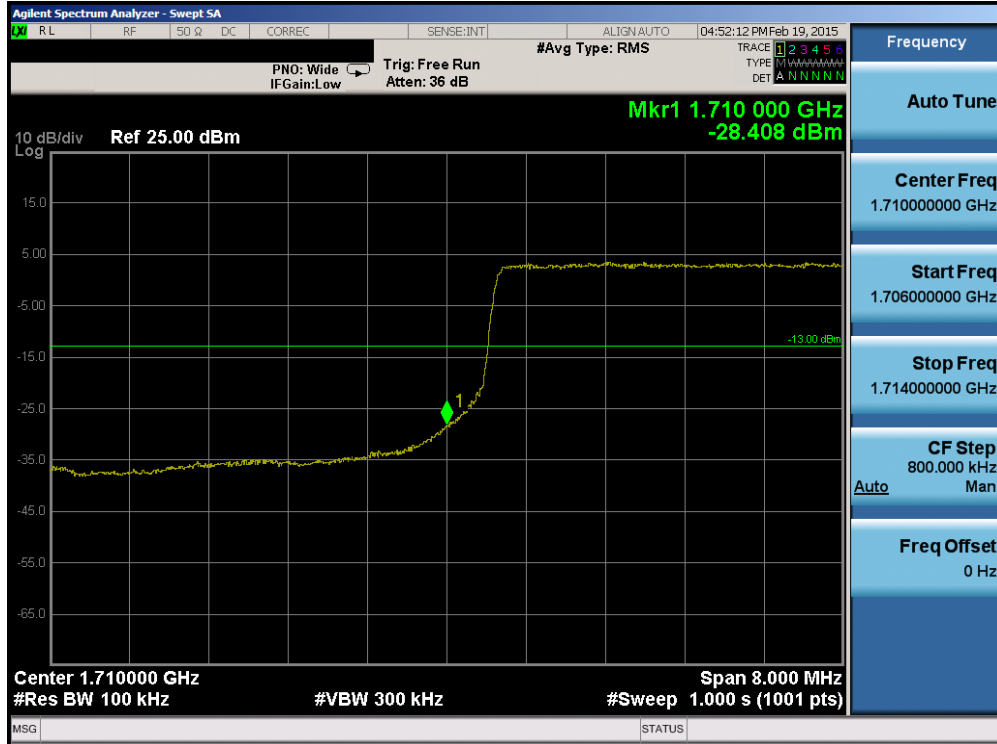
Plot 6-128. Lower Band Edge Plot (Band 4 – 10.0MHz QPSK – RB Size 50)
