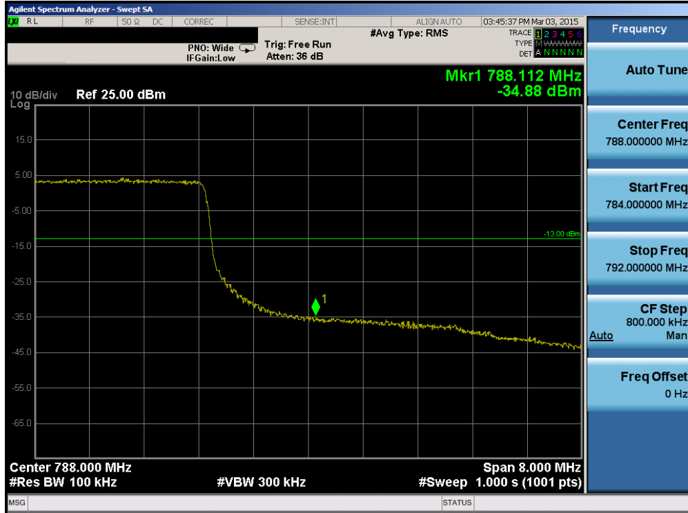
Plot 6-100. Upper Band Edge Plot (Band 13 – 10.0MHz QPSK – RB Size 50)
