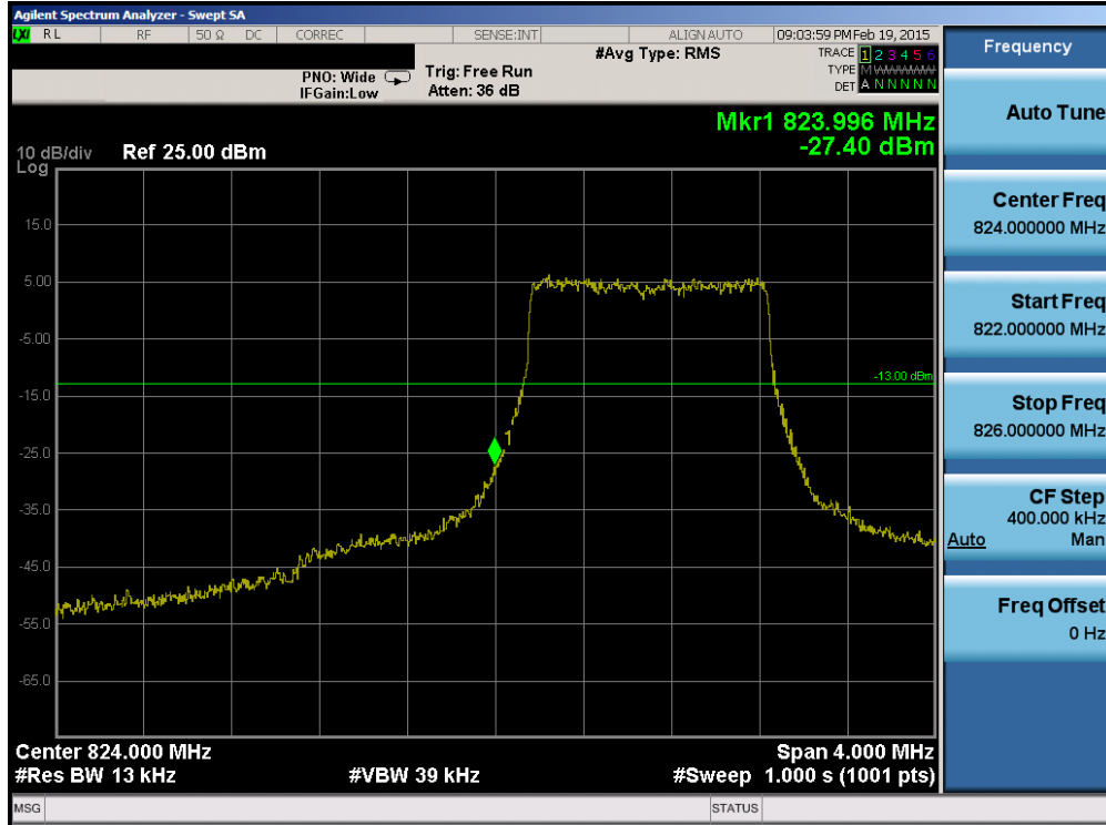
Plot 6-102. Lower Band Edge Plot (Band 5 – 1.4MHz QPSK – RB Size 6)
