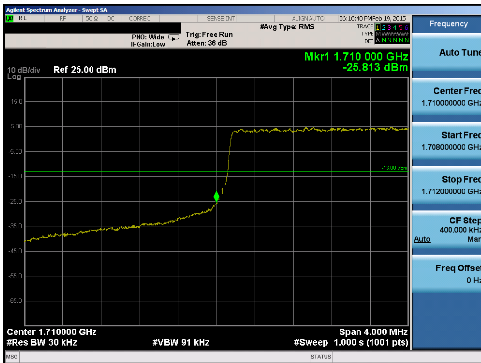
Plot 6-120. Lower Band Edge Plot (Band 4 – 3.0MHz QPSK – RB Size 15)
