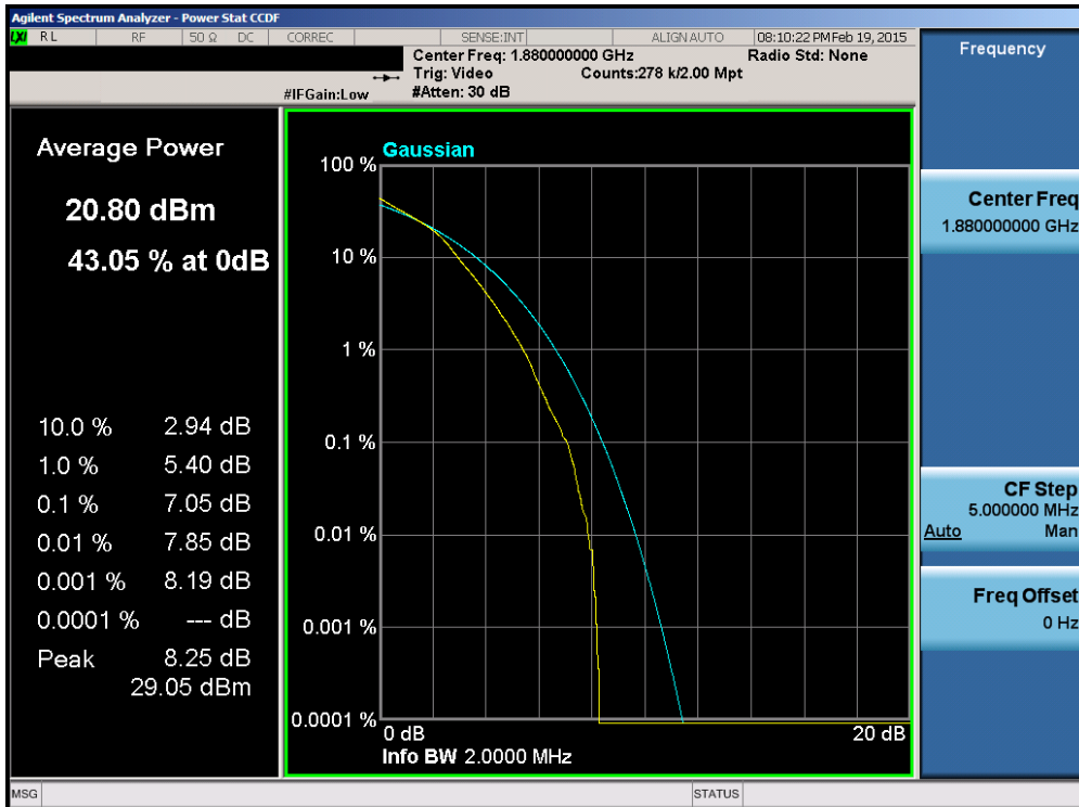
Plot 6-165. PAR Plot (Band 2 – 1.4MHz 16-QAM – RB Size 6)
