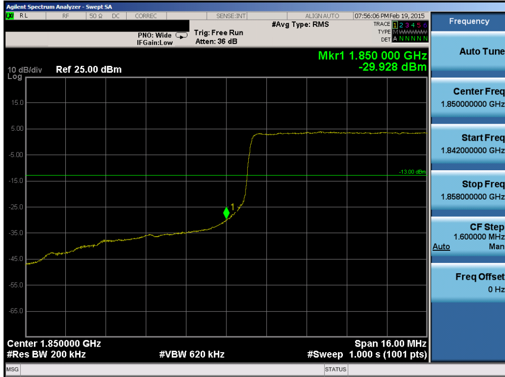
Plot 6-160. Lower Band Edge Plot (Band 2 – 20.0MHz QPSK – RB Size 100)
