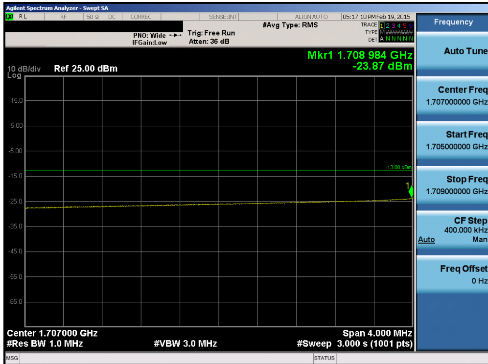
Plot 6-133. Lower Extended Band Edge Plot (Band 4 – 15.0MHz QPSK – RB Size 75)
