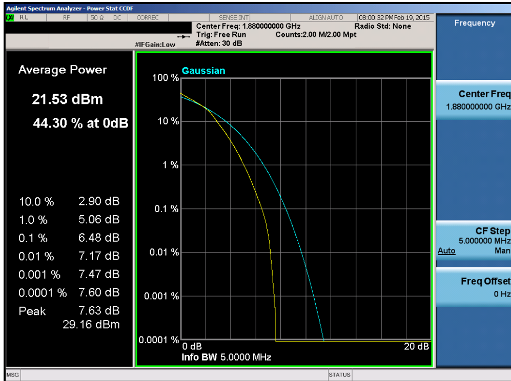
Plot 6-169. PAR Plot (Band 2 – 5.0MHz 16-QAM – RB Size 25)
