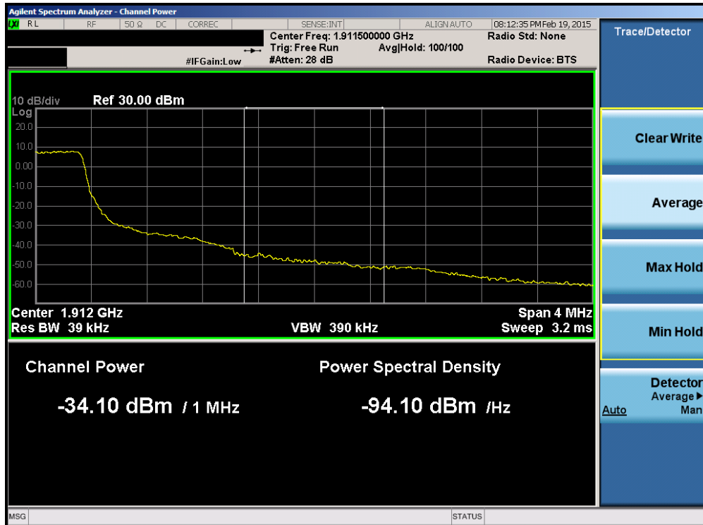
Plot 6-143. Upper Extended Band Edge Plot (Band 2 – 1.4MHz QPSK – RB Size 6)
