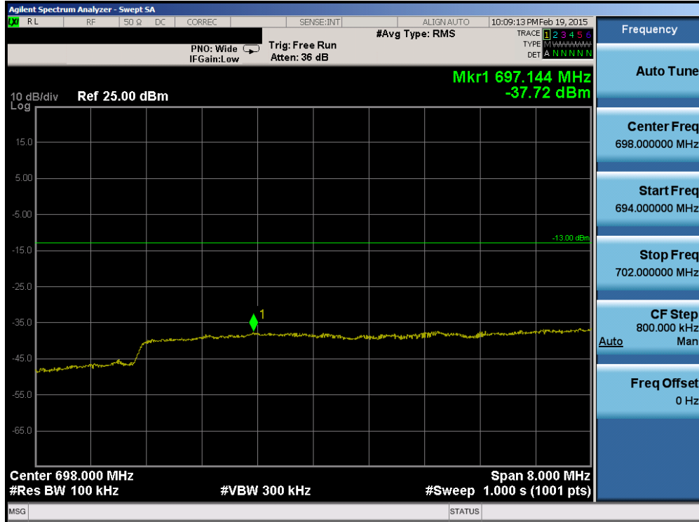
Plot 6-90. Lower Band Edge Plot (Band 17 – 10.0MHz QPSK – RB Size 50)
