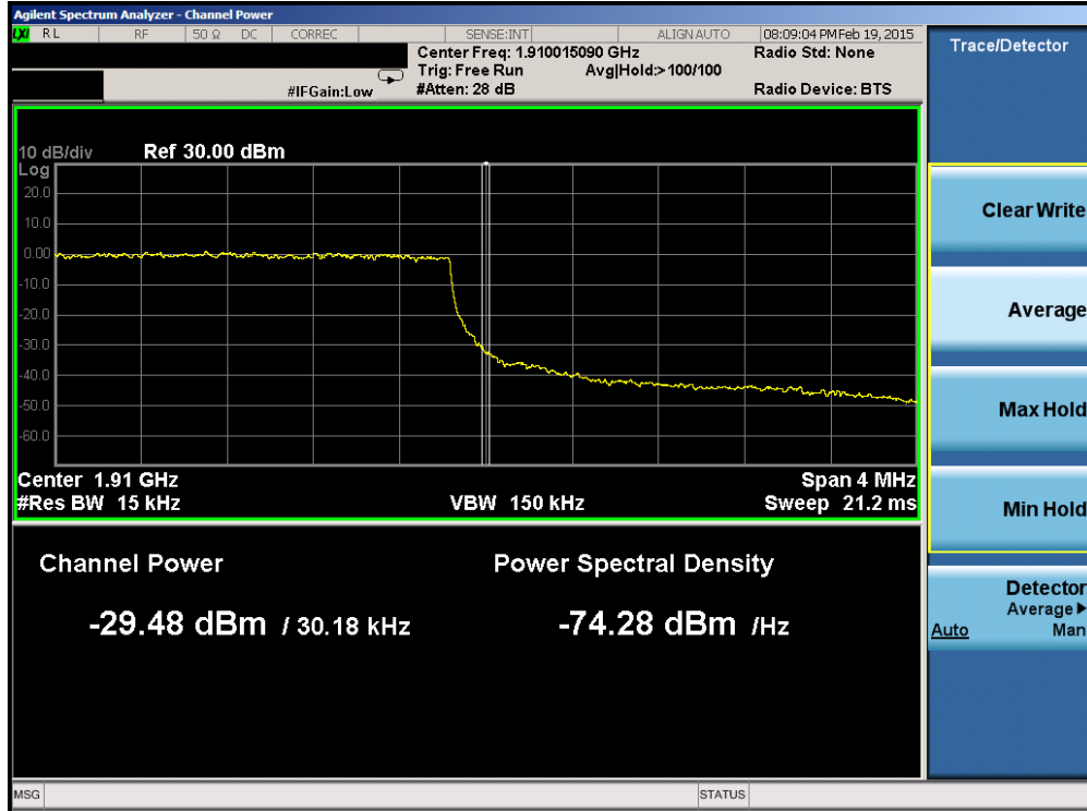
Plot 6-146. Upper Band Edge Plot (Band 2 – 3.0MHz QPSK – RB Size 15)
