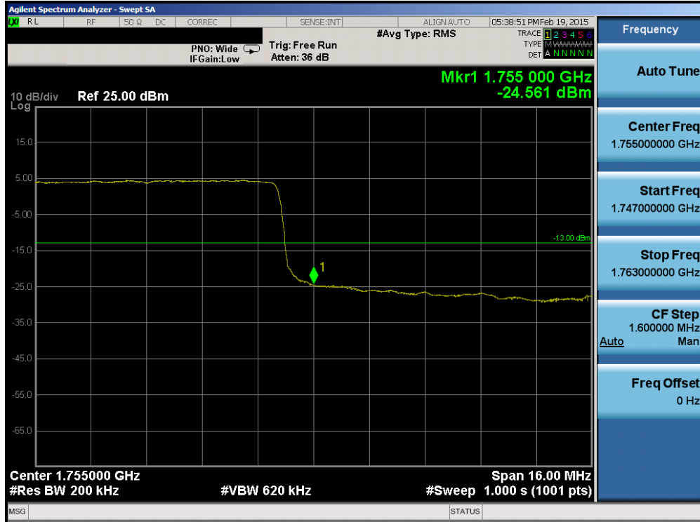
Plot 6-138. Upper Band Edge Plot (Band 4 – 20.0MHz QPSK – RB Size 100)
