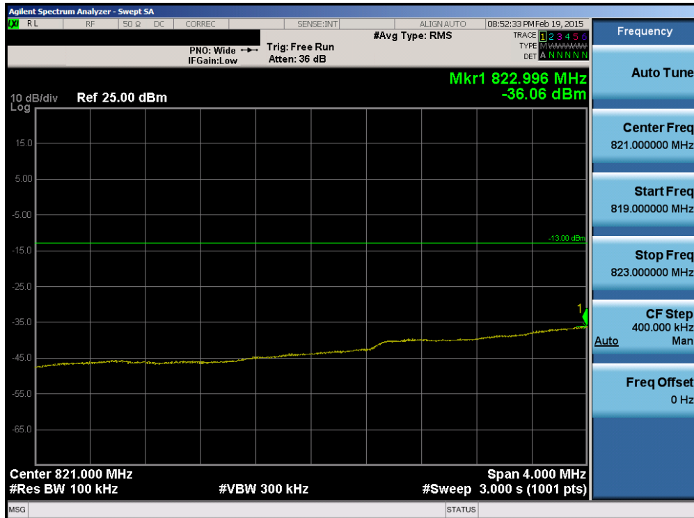
Plot 6-107. Lower Extended Band Edge Plot (Band 5 – 3.0MHz QPSK – RB Size 15)
