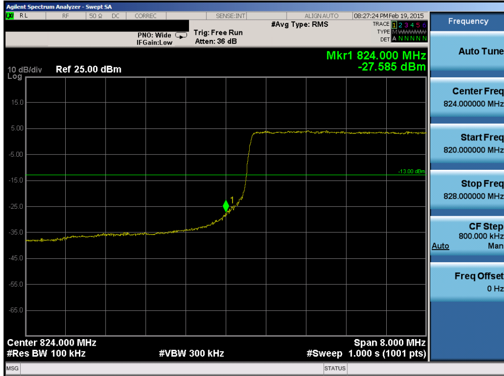
Plot 6-114. Lower Band Edge Plot (Band 5 – 10.0MHz QPSK – RB Size 50)
