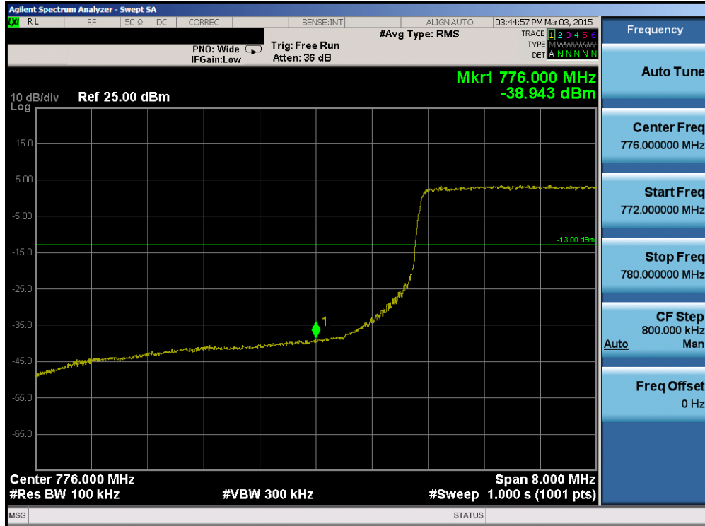
Plot 6-98. Lower Band Edge Plot (Band 13 – 10.0MHz QPSK – RB Size 50)
