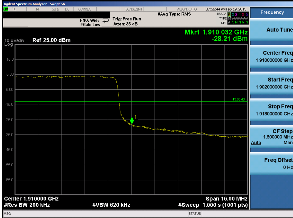
Plot 6-162. Upper Band Edge Plot (Band 2 – 20.0MHz QPSK – RB Size 100)
