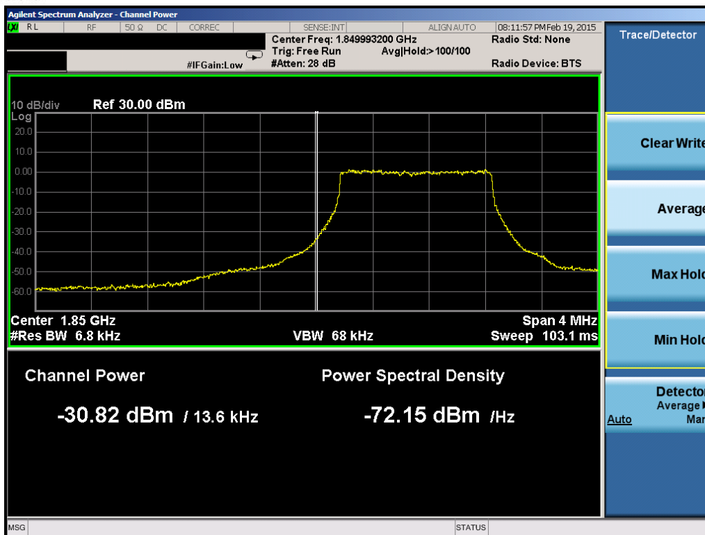
Plot 6-140. Lower Band Edge Plot (Band 2 – 1.4MHz QPSK – RB Size 6)
