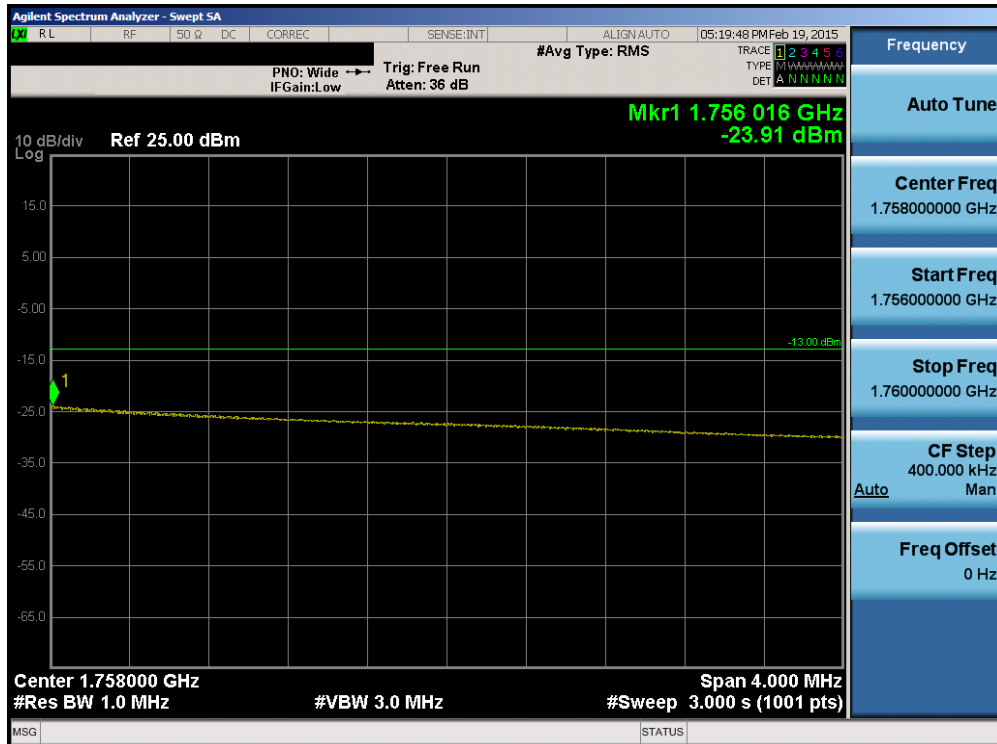
Plot 6-135. Upper Extended Band Edge Plot (Band 4 – 15.0MHz QPSK – RB Size 75)
