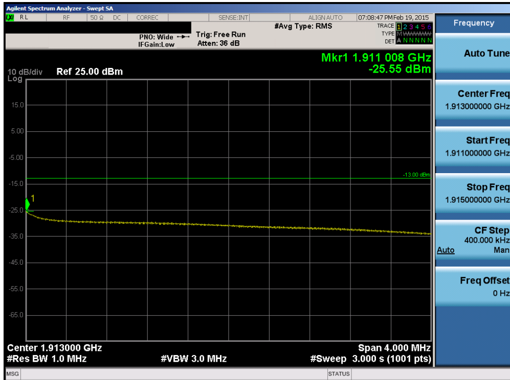
Plot 6-155. Upper Extended Band Edge Plot (Band 2 – 10.0MHz QPSK – RB Size 50)
