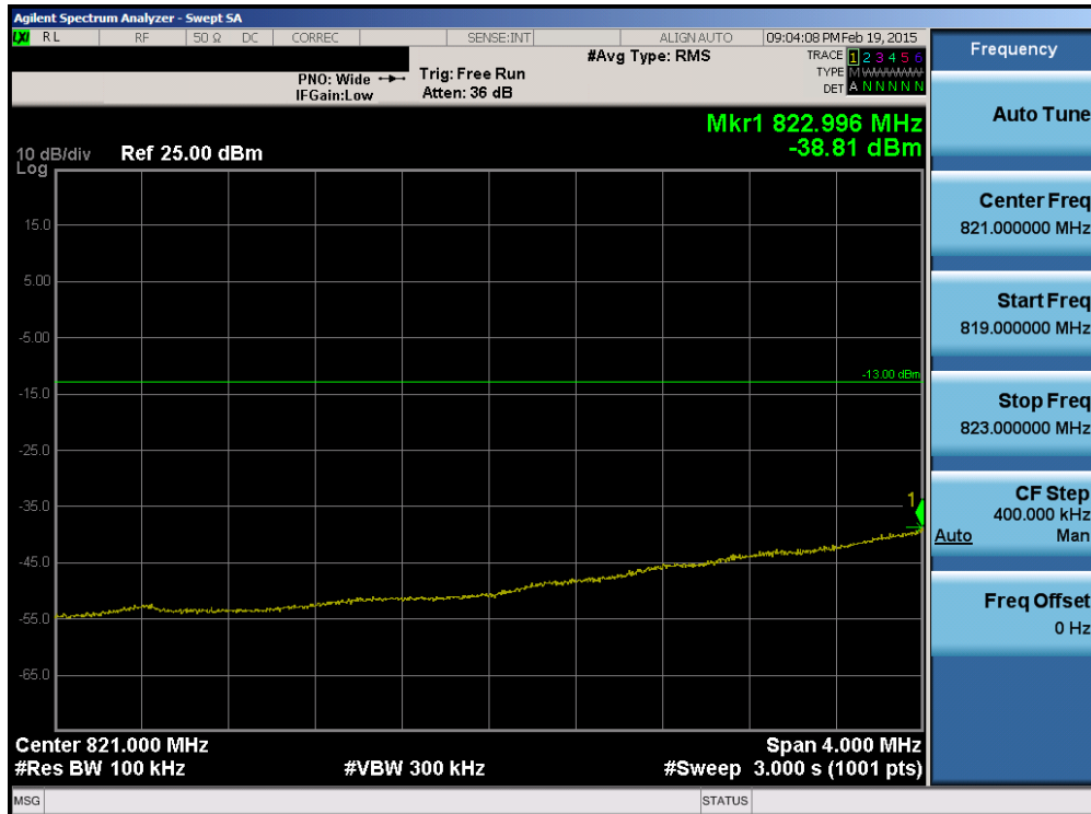
Plot 6-103. Lower Extended Band Edge Plot (Band 5 – 1.4MHz QPSK – RB Size 6)
