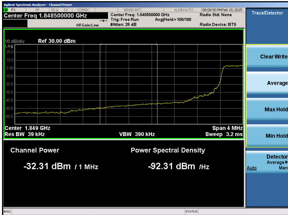
Plot 6-145. Lower Extended Band Edge Plot (Band 2 – 3.0MHz QPSK – RB Size 15)
