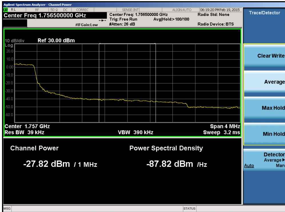
Plot 6-123. Upper Extended Band Edge Plot (Band 4 – 3.0MHz QPSK – RB Size 15)
