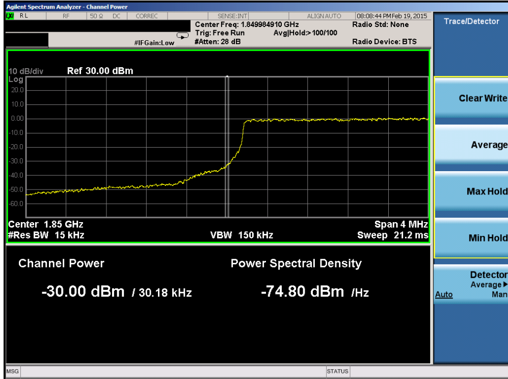
Plot 6-144. Lower Band Edge Plot (Band 2 – 3.0MHz QPSK – RB Size 15)
