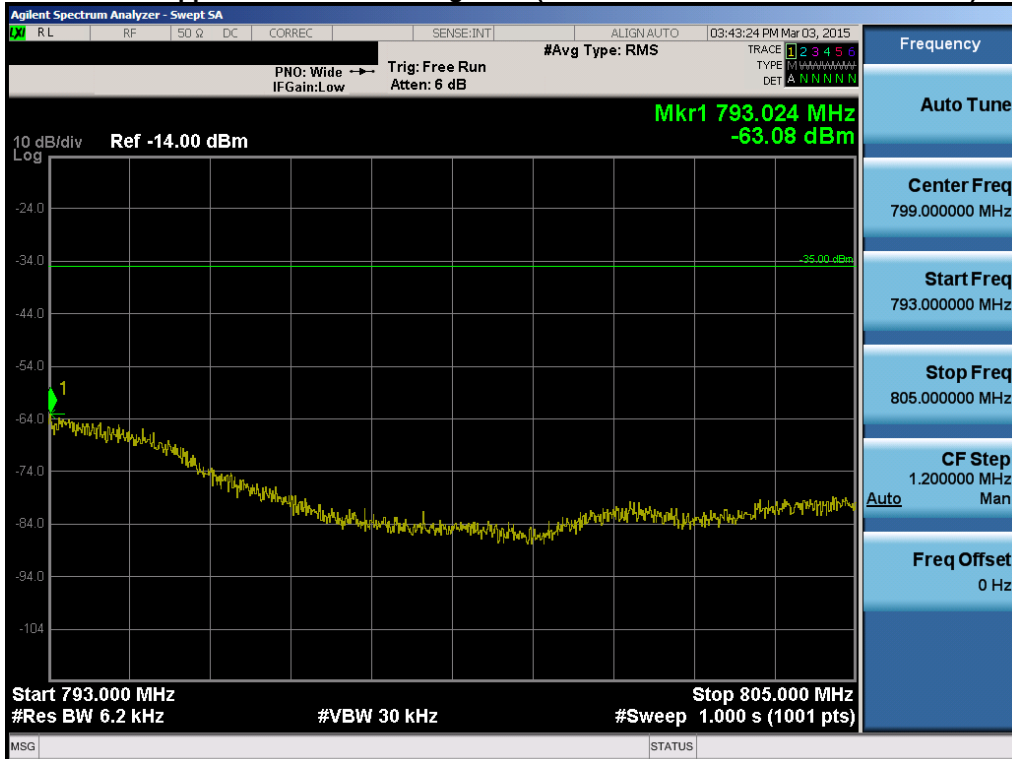
Plot 6-97. Upper Emission Mask Plot (Band 13 – 5.0MHz QPSK – RB Size 25)
