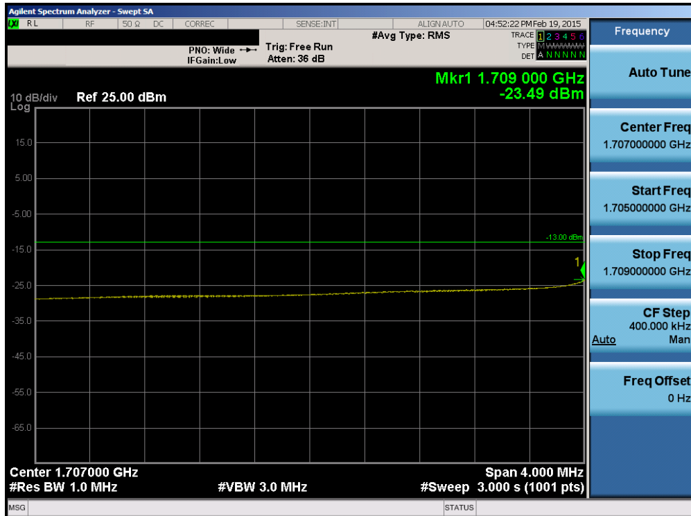
Plot 6-129. Lower Extended Band Edge Plot (Band 4 – 10.0MHz QPSK – RB Size 50)
