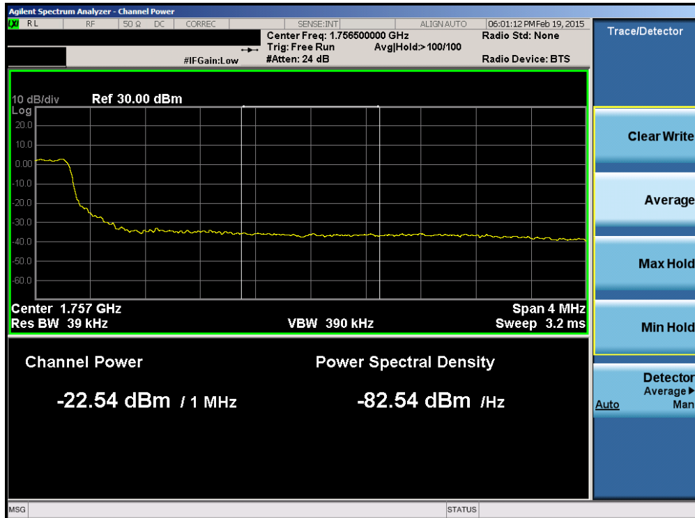
Plot 6-127. Upper Extended Band Edge Plot (Band 4 – 5.0MHz QPSK – RB Size 25)
