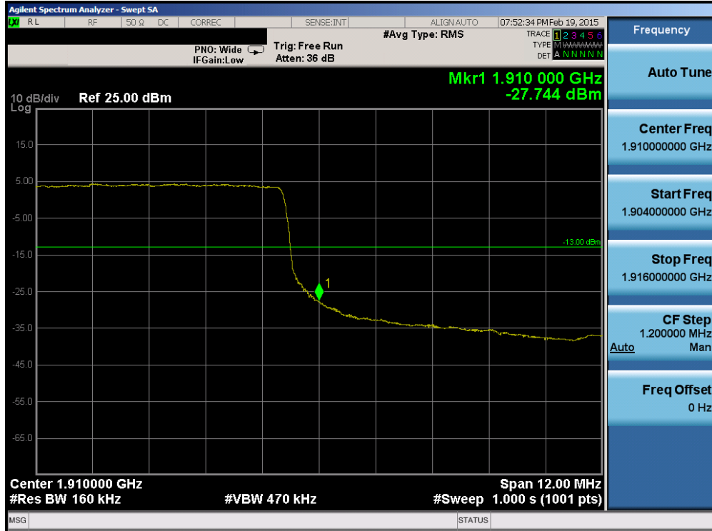
Plot 6-158. Upper Band Edge Plot (Band 2 – 15.0MHz QPSK – RB Size 75)
