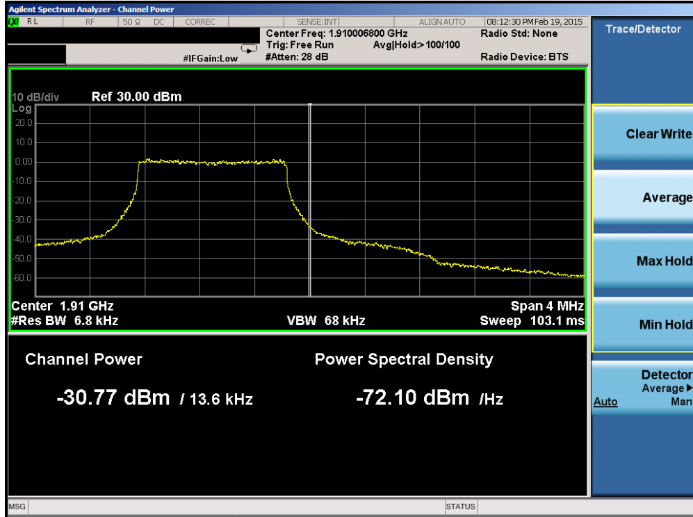
Plot 6-142. Upper Band Edge Plot (Band 2 – 1.4MHz QPSK – RB Size 6)
