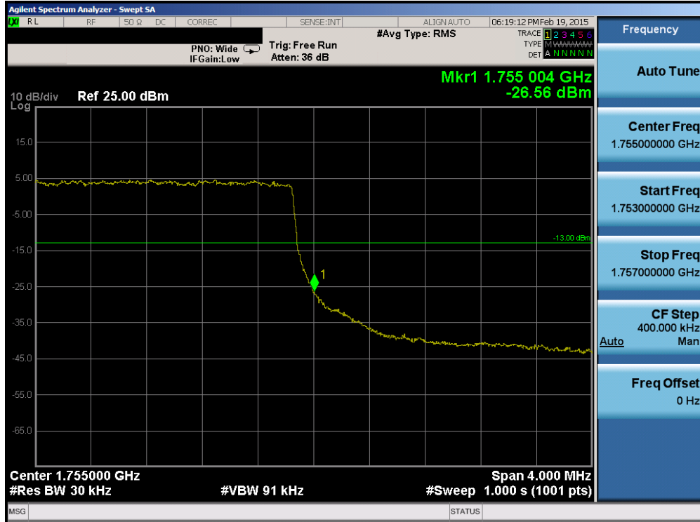
Plot 6-122. Upper Band Edge Plot (Band 4 – 3.0MHz QPSK – RB Size 15)
