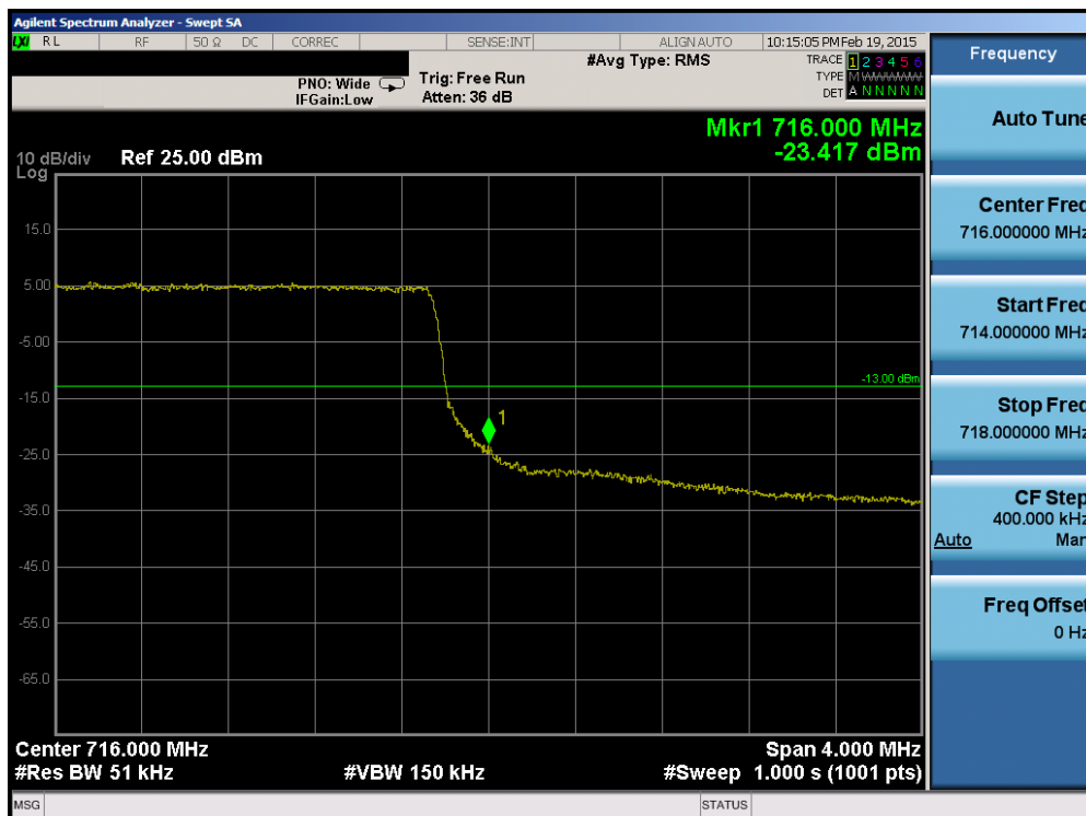
Plot 6-88. Upper Band Edge Plot (Band 17 – 5.0MHz QPSK – RB Size 25)
