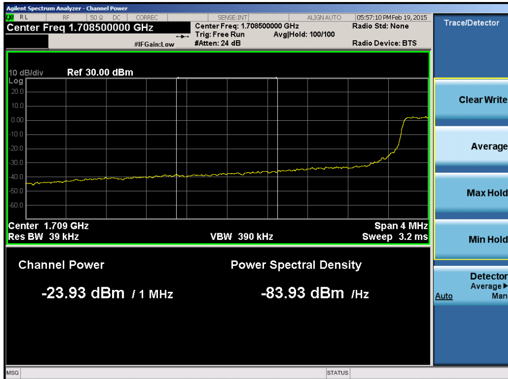
Plot 6-125. Lower Extended Band Edge Plot (Band 4 – 5.0MHz QPSK – RB Size 25)
