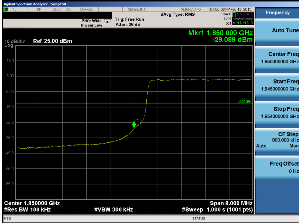
Plot 6-152. Lower Band Edge Plot (Band 2 – 10.0MHz QPSK – RB Size 50)
