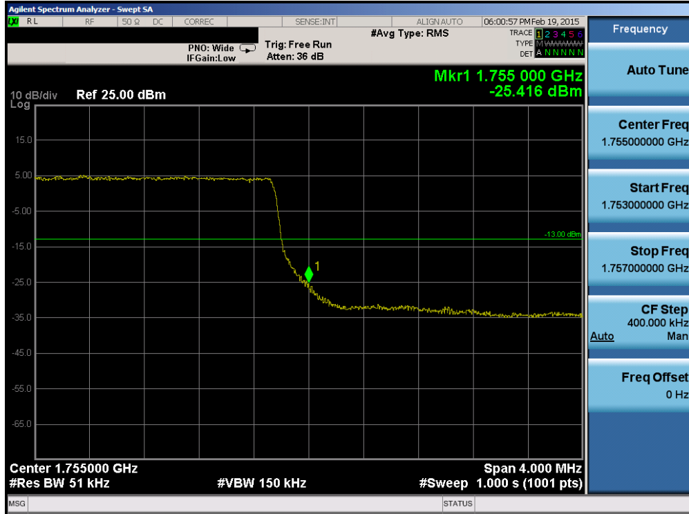
Plot 6-126. Upper Band Edge Plot (Band 4 – 5.0MHz QPSK – RB Size 25)
