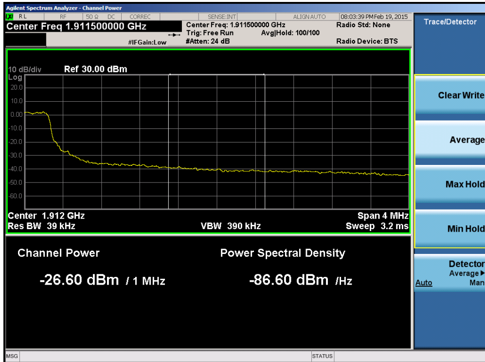
Plot 6-151. Upper Extended Band Edge Plot (Band 2 – 5.0MHz QPSK – RB Size 25)
