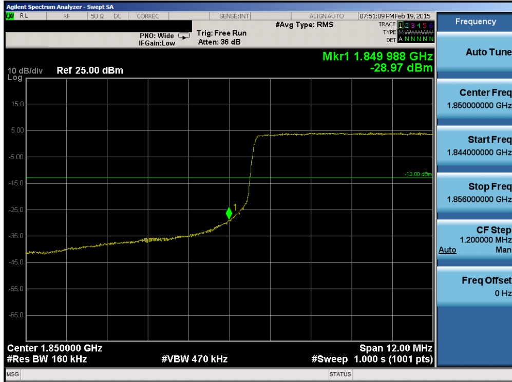
Plot 6-156. Lower Band Edge Plot (Band 2 – 15.0MHz QPSK – RB Size 75)
