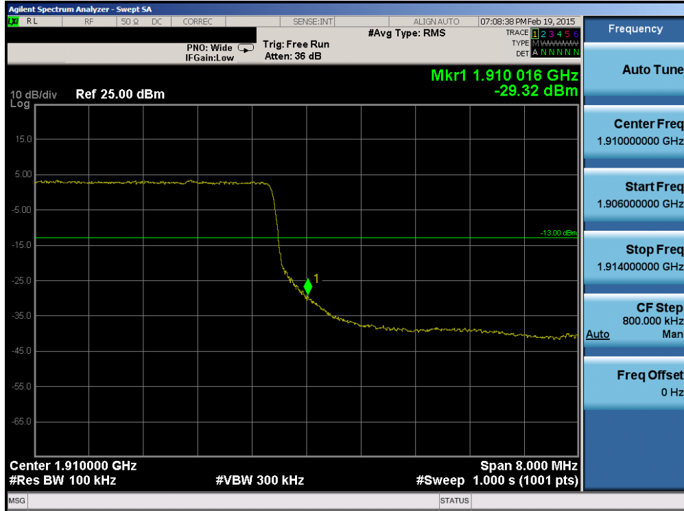
Plot 6-154. Upper Band Edge Plot (Band 2 – 10.0MHz QPSK – RB Size 50)
