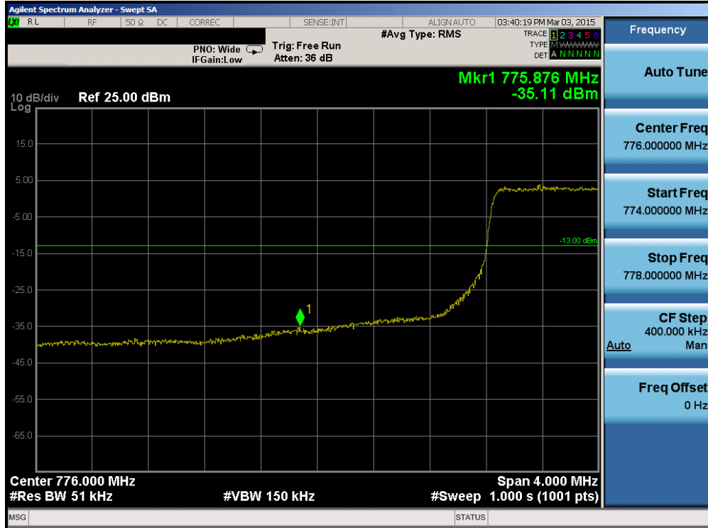
Plot 6-92. Lower Band Edge Plot (Band 13 – 5.0MHz QPSK – RB Size 25)
