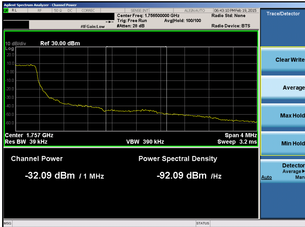
Plot 6-119. Upper Extended Band Edge Plot (Band 4 – 1.4MHz QPSK – RB Size 6)
