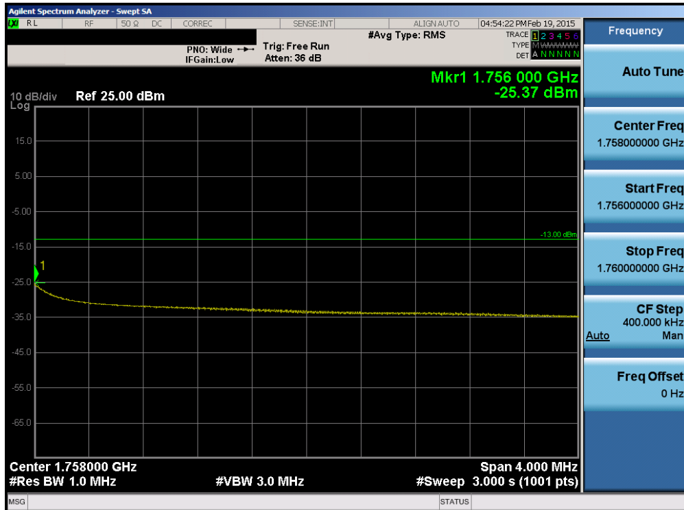
Plot 6-131. Upper Extended Band Edge Plot (Band 4 – 10.0MHz QPSK – RB Size 50)
