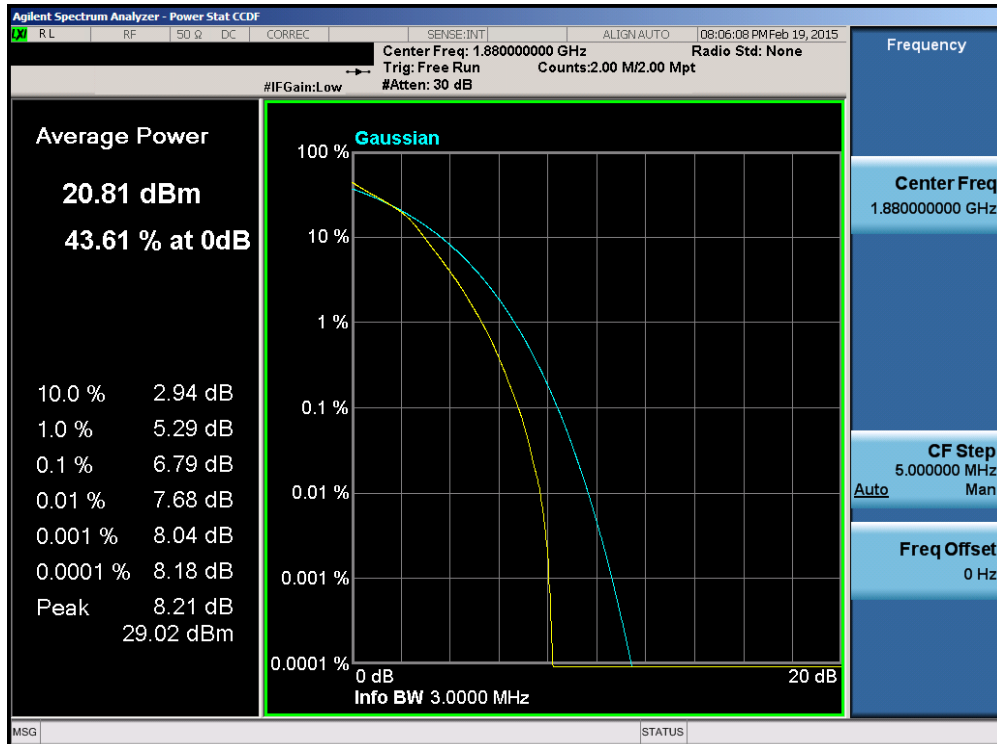
Plot 6-167. PAR Plot (Band 2 – 3.0MHz 16-QAM – RB Size 15)
