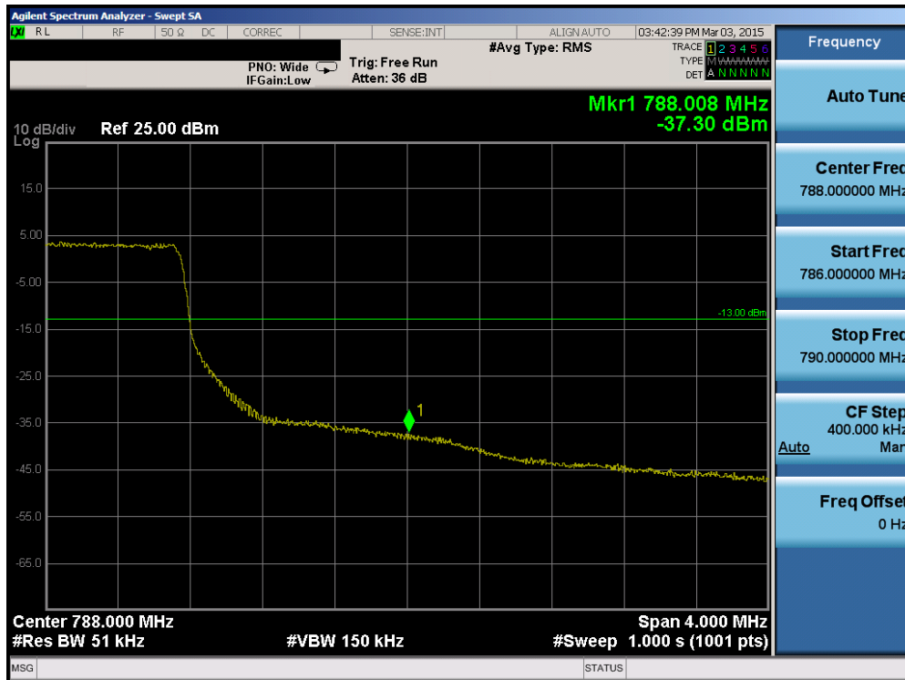
Plot 6-95. Upper Band Edge Plot (Band 13 – 5.0MHz QPSK – RB Size 25)
