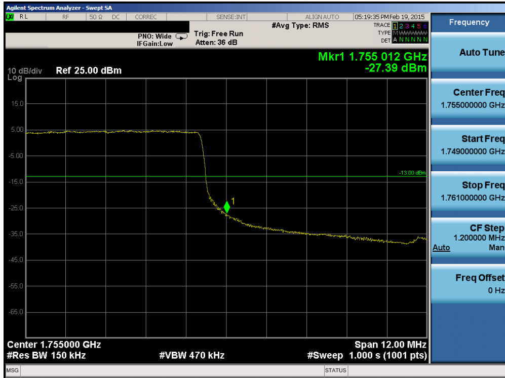
Plot 6-134. Upper Band Edge Plot (Band 4 – 15.0MHz QPSK – RB Size 75)
