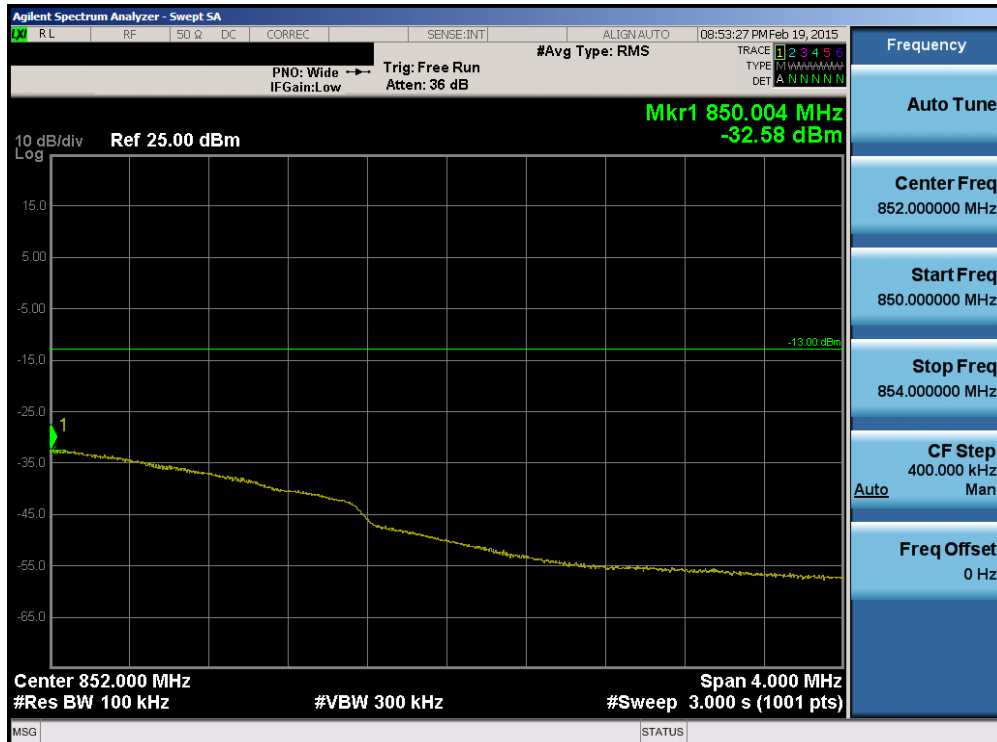
Plot 6-109. Upper Extended Band Edge Plot (Band 5 – Band 5 – 3.0MHz QPSK – RB Size 15)
