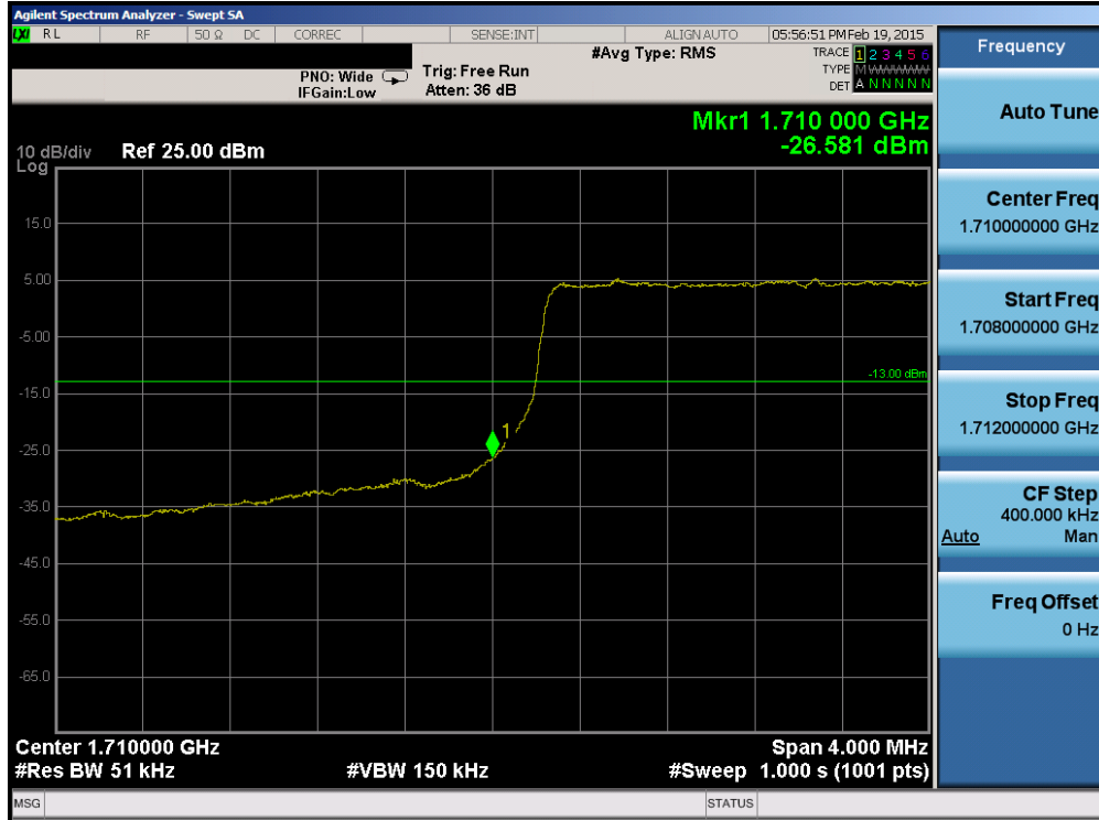
Plot 6-124. Lower Band Edge Plot (Band 4 – 5.0MHz QPSK – RB Size 25)
