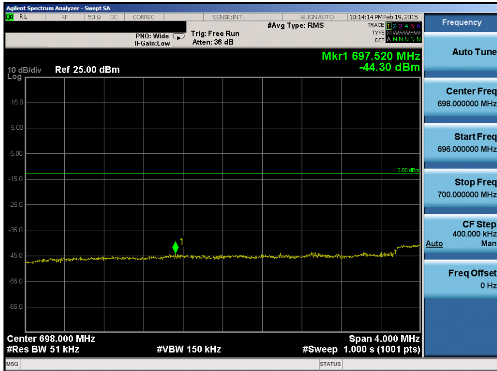
Plot 6-86. Lower Band Edge Plot (Band 17 – 5.0MHz QPSK – RB Size 25)
