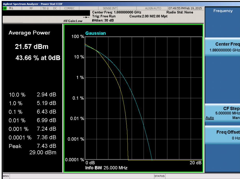
Plot 6-173. PAR Plot (Band 2 – 15.0MHz 16-QAM – RB Size 75)
