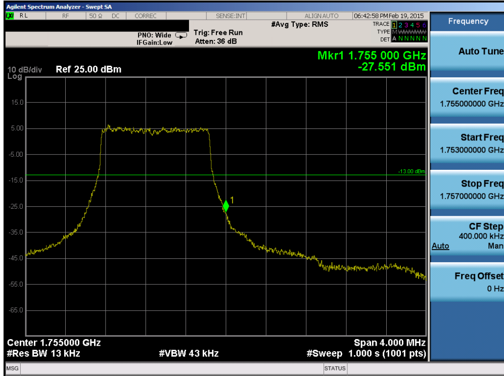
Plot 6-118. Upper Band Edge Plot (Band 4 – 1.4MHz QPSK – RB Size 6)
