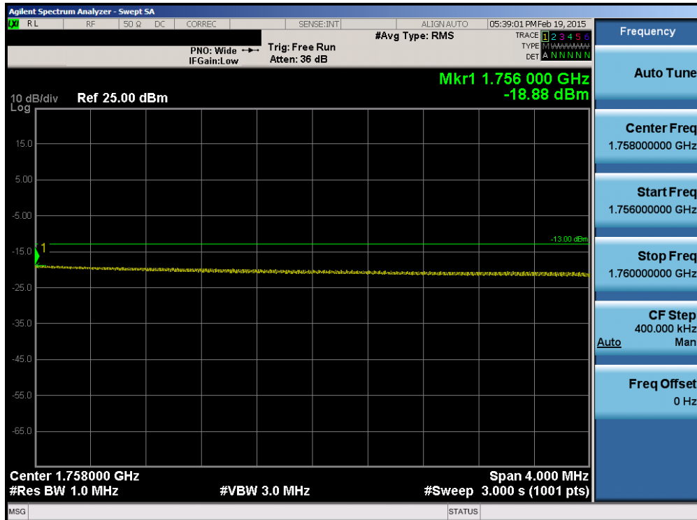
Plot 6-139. Upper Extended Band Edge Plot (Band 4 – 20.0MHz QPSK – RB Size 100)
