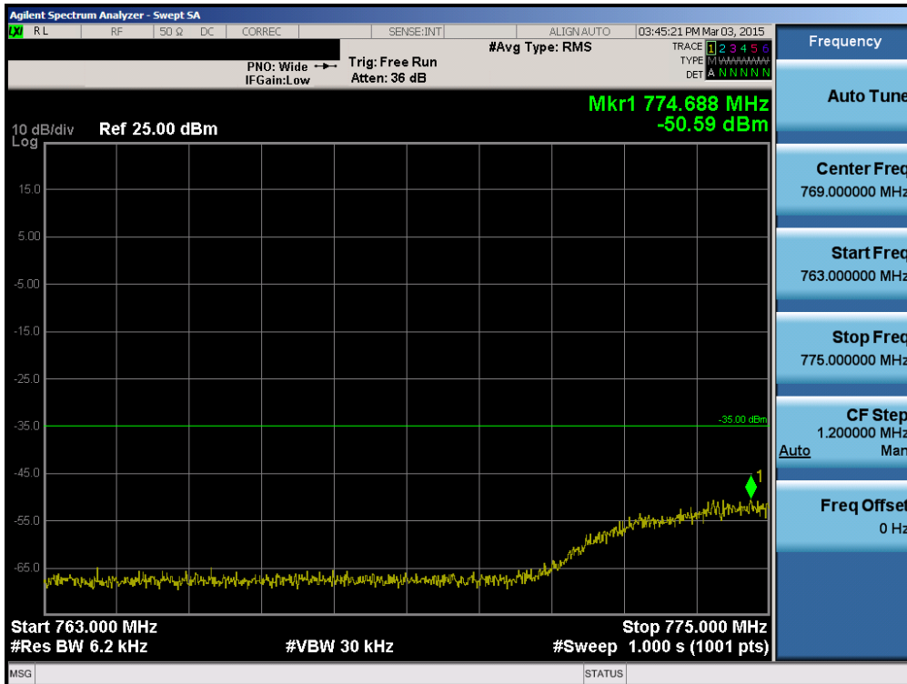
Plot 6-99. Lower Emission Mask Plot (Band 13 – 10.0MHz QPSK – RB Size 50)
