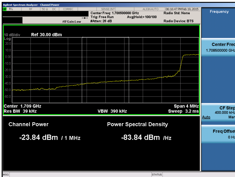
Plot 6-121. Lower Extended Band Edge Plot (Band 4 – 3.0MHz QPSK – RB Size 15)
