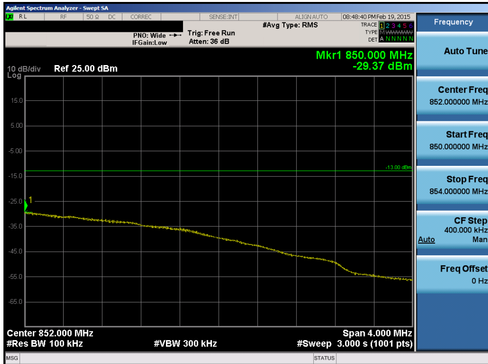
Plot 6-113. Upper Extended Band Edge Plot (Band 5 – 5.0MHz QPSK – RB Size 25)
