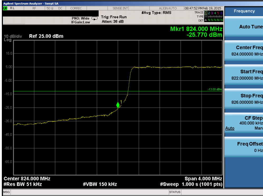
Plot 6-110. Lower Band Edge Plot (Band 5 – 5.0MHz QPSK – RB Size 25)
