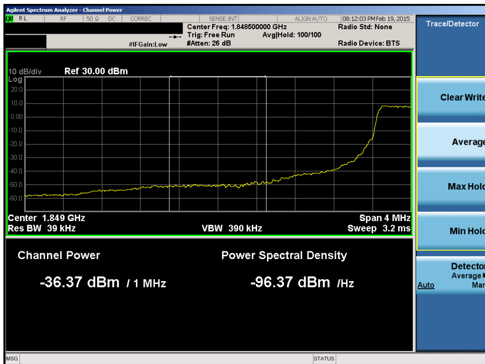
Plot 6-141. Lower Extended Band Edge Plot (Band 2 – 1.4MHz QPSK – RB Size 6)
