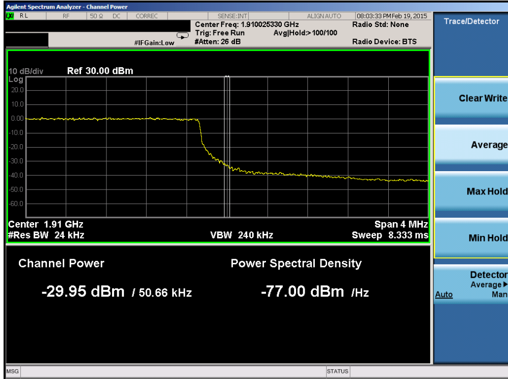
Plot 6-150. Upper Band Edge Plot (Band 2 – 5.0MHz QPSK – RB Size 25)
