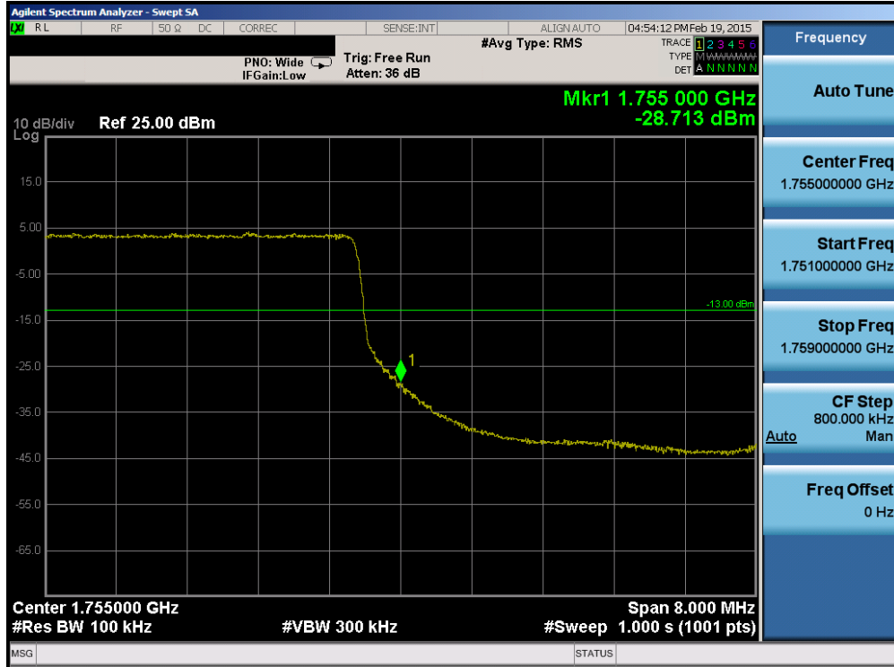
Plot 6-130. Upper Band Edge Plot (Band 4 – 10.0MHz QPSK – RB Size 50)
