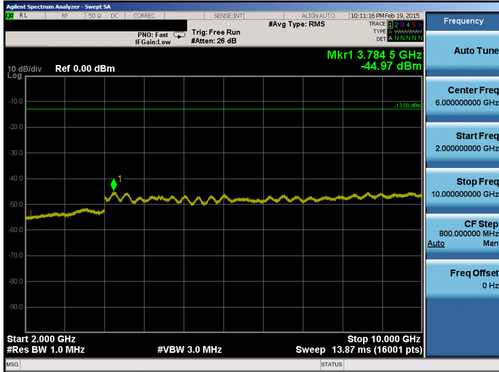
Plot 6-49. Conducted Spurious Plot (Band 17 – 10.0MHz QPSK – RB Size 1, RB Offset 0 – High Channel)
