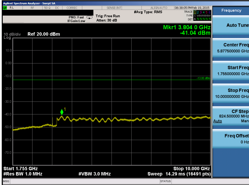
Plot 6-69. Conducted Spurious Plot (Band 4 – 1.4MHz QPSK – RB Size 1, RB Offset 0 – Low Channel)
