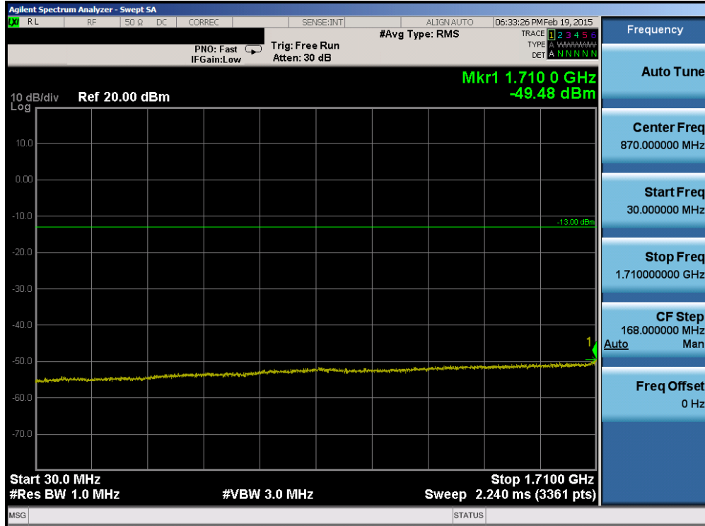
Plot 6-71. Conducted Spurious Plot (Band 4 – 1.4MHz QPSK – RB Size 1, RB Offset 0 – Mid Channel)
