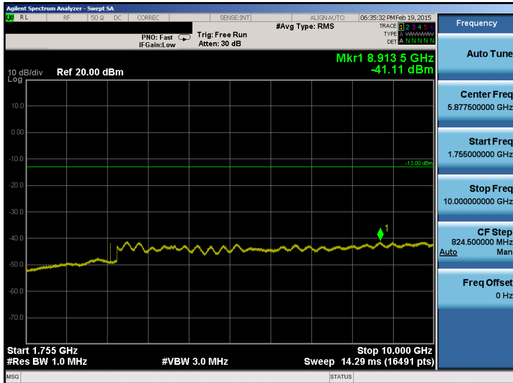
Plot 6-72. Conducted Spurious Plot (Band 4 – 1.4MHz QPSK – RB Size 1, RB Offset 0 – Mid Channel)
