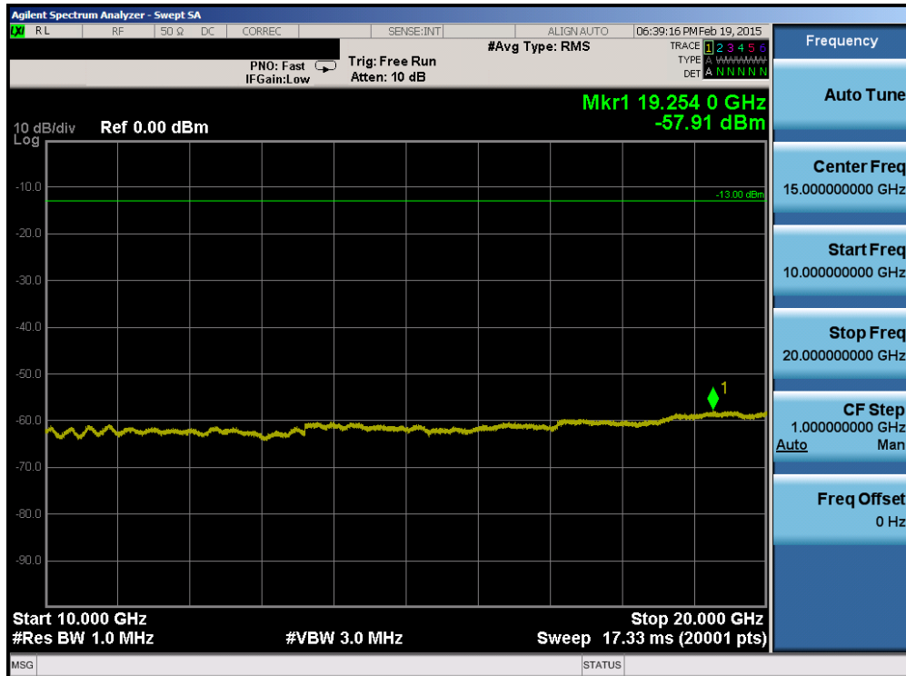
Plot 6-70. Conducted Spurious Plot (Band 4 – 1.4MHz QPSK – RB Size 1, RB Offset 0 – Low Channel)
