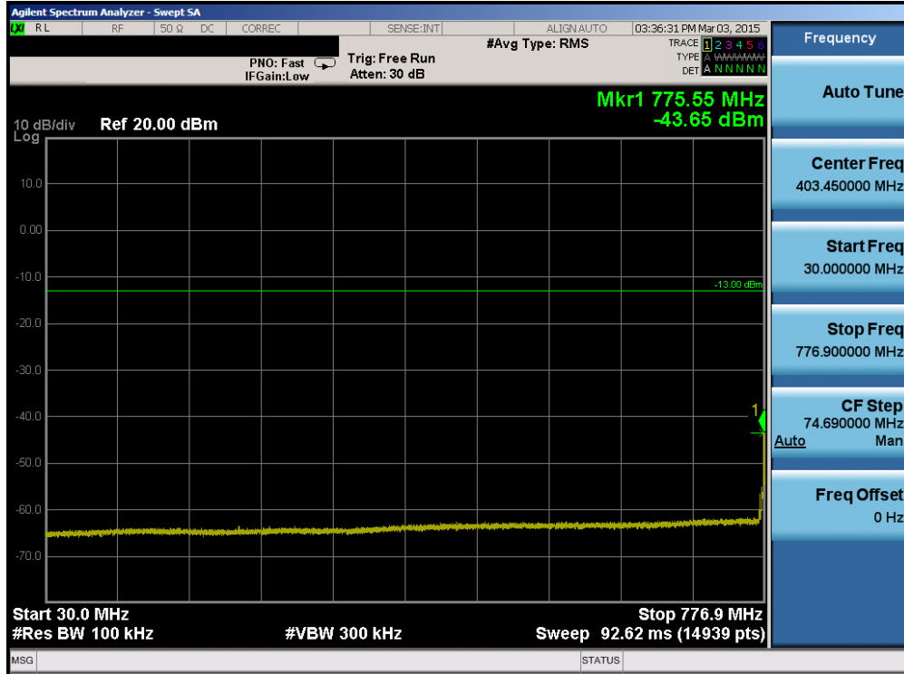
Plot 6-53. Conducted Spurious Plot (Band 13 – 5.0MHz QPSK – RB Size 1, RB Offset 0 – Mid Channel)
