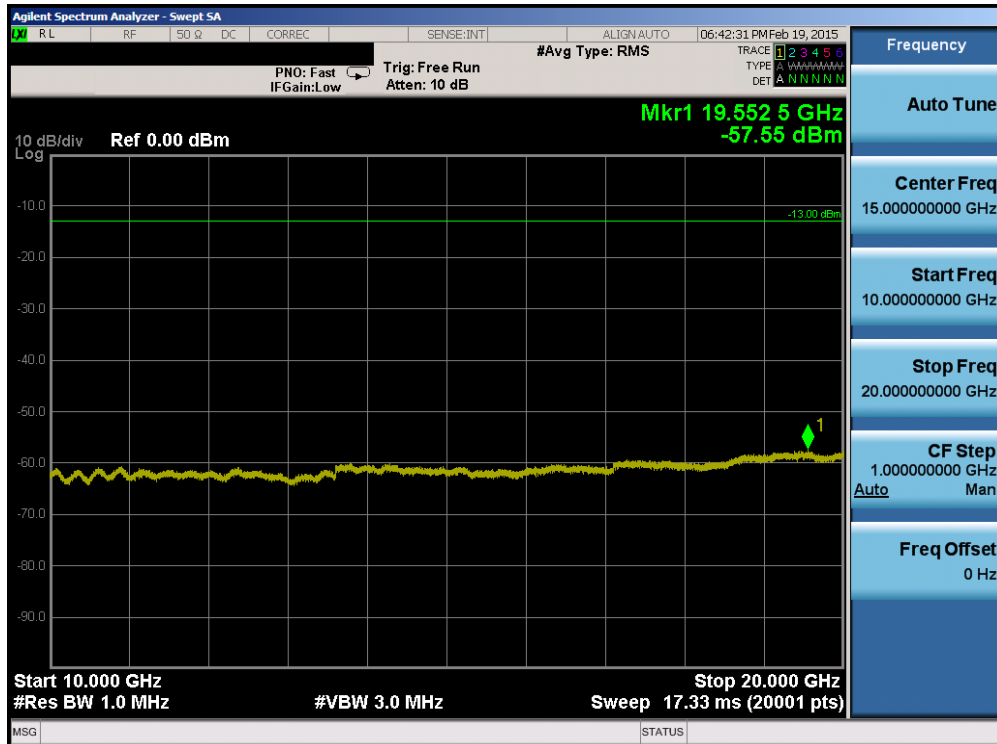
Plot 6-76. Conducted Spurious Plot (Band 4 – 1.4MHz QPSK – RB Size 1, RB Offset 0 – High Channel)
