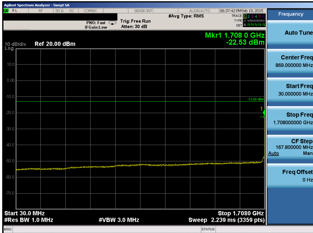
Plot 6-68. Conducted Spurious Plot (Band 4 – 1.4MHz QPSK – RB Size 1, RB Offset 0 – Low Channel)
