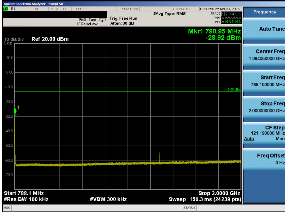
Plot 6-57. Conducted Spurious Plot (Band 13 – 5.0MHz QPSK – RB Size 1, RB Offset 0 – High Channel)
