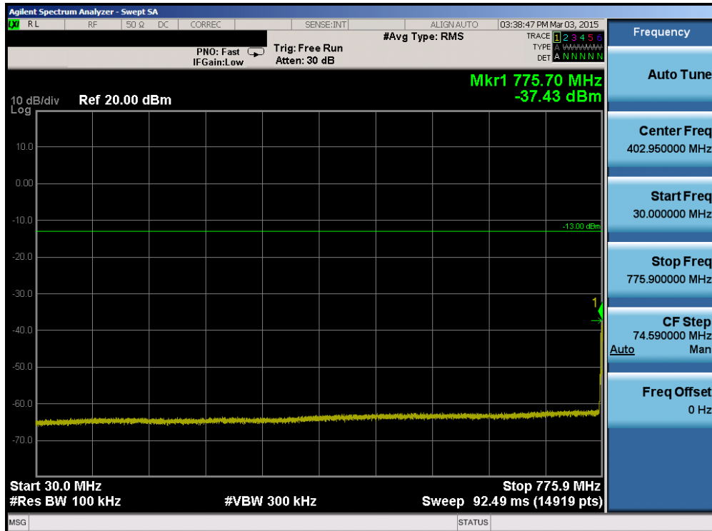
Plot 6-50. Conducted Spurious Plot (Band 13 – 5.0MHz QPSK – RB Size 1, RB Offset 0 – Low Channel)
