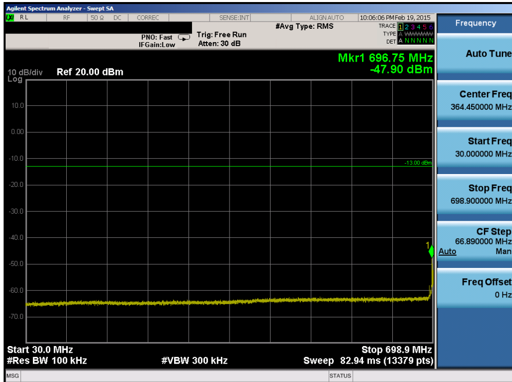
Plot 6-44. Conducted Spurious Plot (Band 17 – 10.0MHz QPSK – RB Size 1, RB Offset 0 – Mid Channel)
