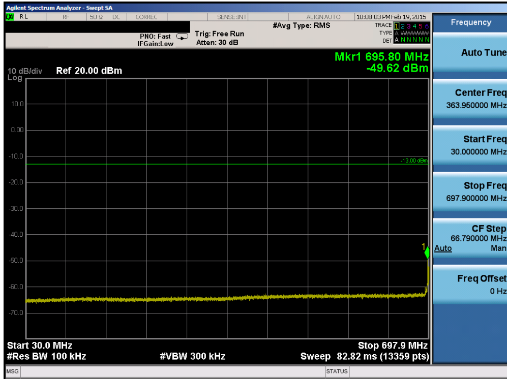
Plot 6-41. Conducted Spurious Plot (Band 17 – 10.0MHz QPSK – RB Size 1, RB Offset 0– Low Channel)
