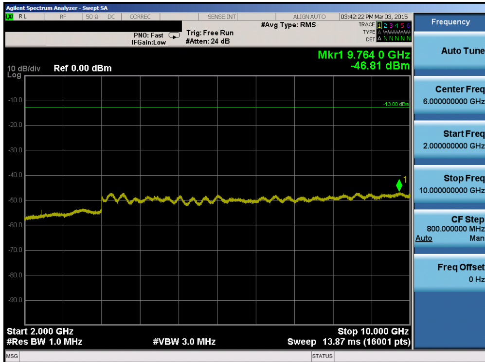
Plot 6-58. Conducted Spurious Plot (Band 13 – 5.0MHz QPSK – RB Size 1, RB Offset 0 – High Channel)
