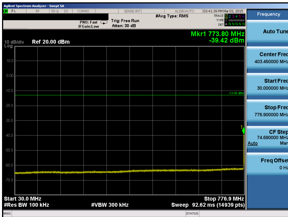
Plot 6-56. Conducted Spurious Plot (Band 13 – 5.0MHz QPSK – RB Size 1, RB Offset 0 – High Channel)
