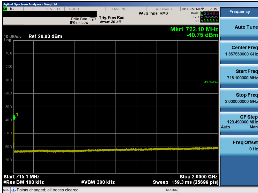
Plot 6-42. Conducted Spurious Plot (Band 17 – 10.0MHz QPSK – RB Size 1, RB Offset 0 – Low Channel)
