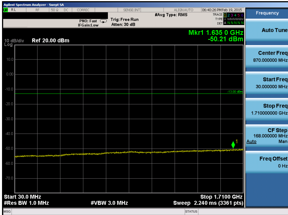
Plot 6-74. Conducted Spurious Plot (Band 4 – 1.4MHz QPSK – RB Size 1, RB Offset 0 – High Channel)
