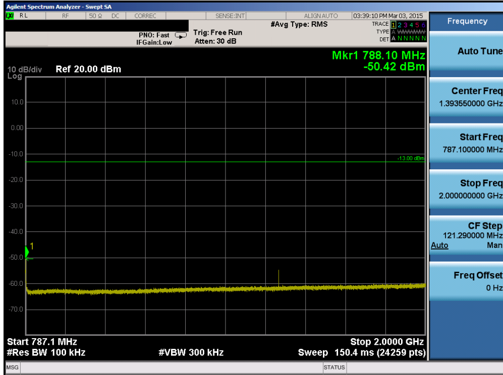
Plot 6-51. Conducted Spurious Plot (Band 13 – 5.0MHz QPSK – RB Size 1, RB Offset 0 – Low Channel)
