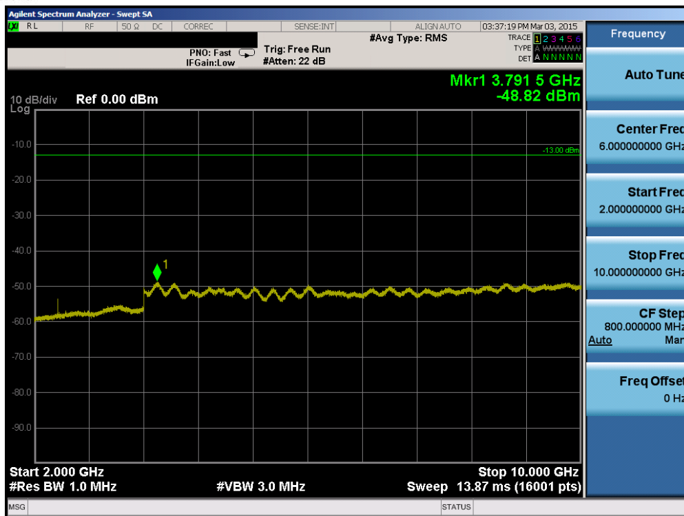
Plot 6-55. Conducted Spurious Plot (Band 13 – 5.0MHz QPSK – RB Size 1, RB Offset 0 – Mid Channel)
