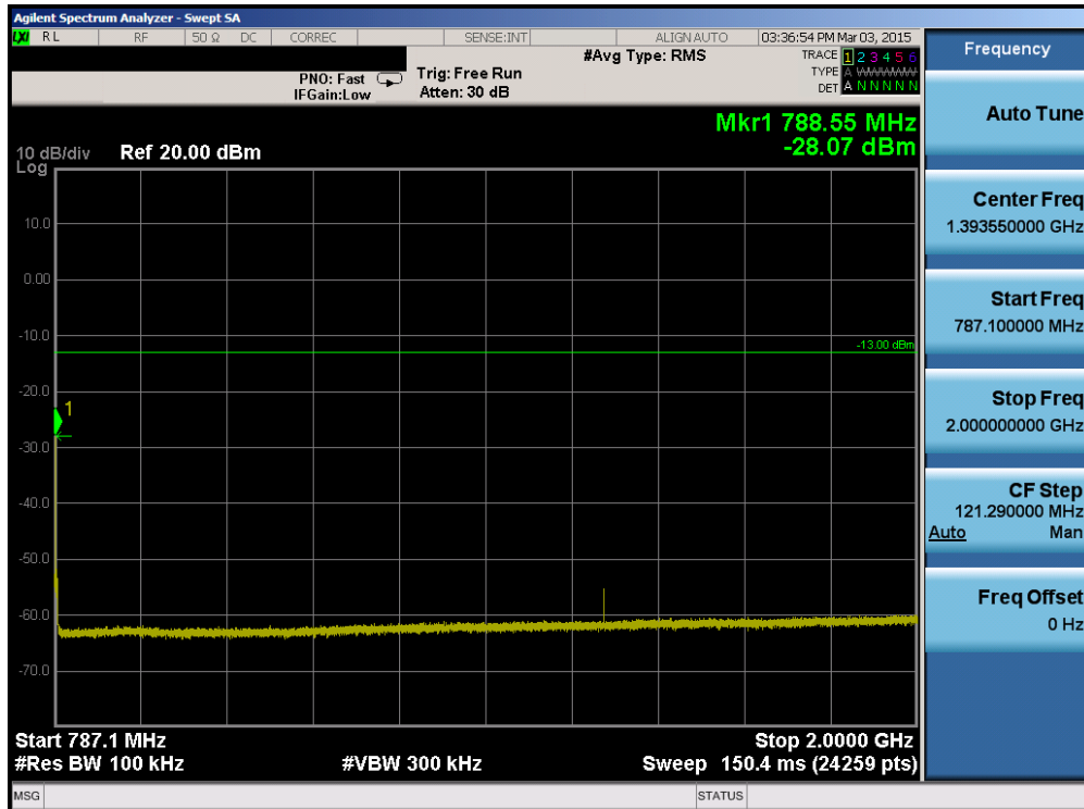
Plot 6-54. Conducted Spurious Plot (Band 13 – 5.0MHz QPSK – RB Size 1, RB Offset 0 – Mid Channel)
