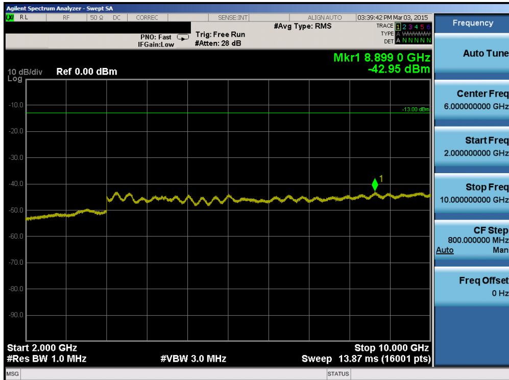
Plot 6-52. Conducted Spurious Plot (Band 13 – 5.0MHz QPSK – RB Size 1, RB Offset 0 – Low Channel)
