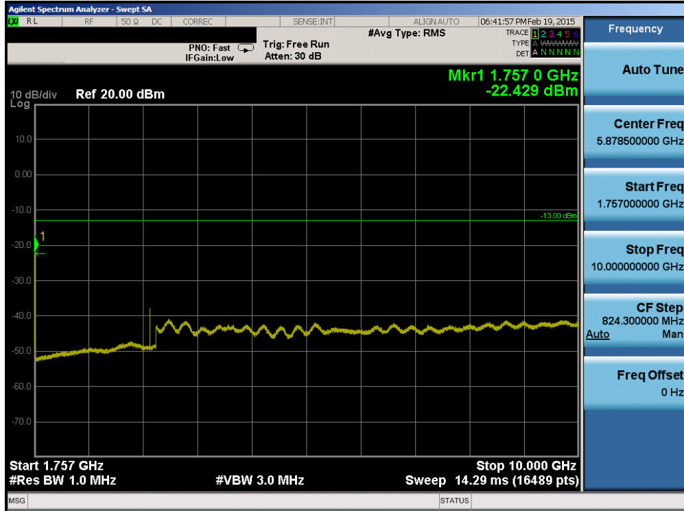
Plot 6-75. Conducted Spurious Plot (Band 4 – 1.4MHz QPSK – RB Size 1, RB Offset 0 – High Channel)
