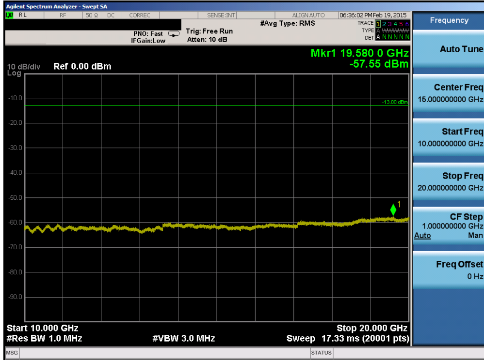
Plot 6-73. Conducted Spurious Plot (Band 4 – 1.4MHz QPSK – RB Size 1, RB Offset 0 – Mid Channel)
