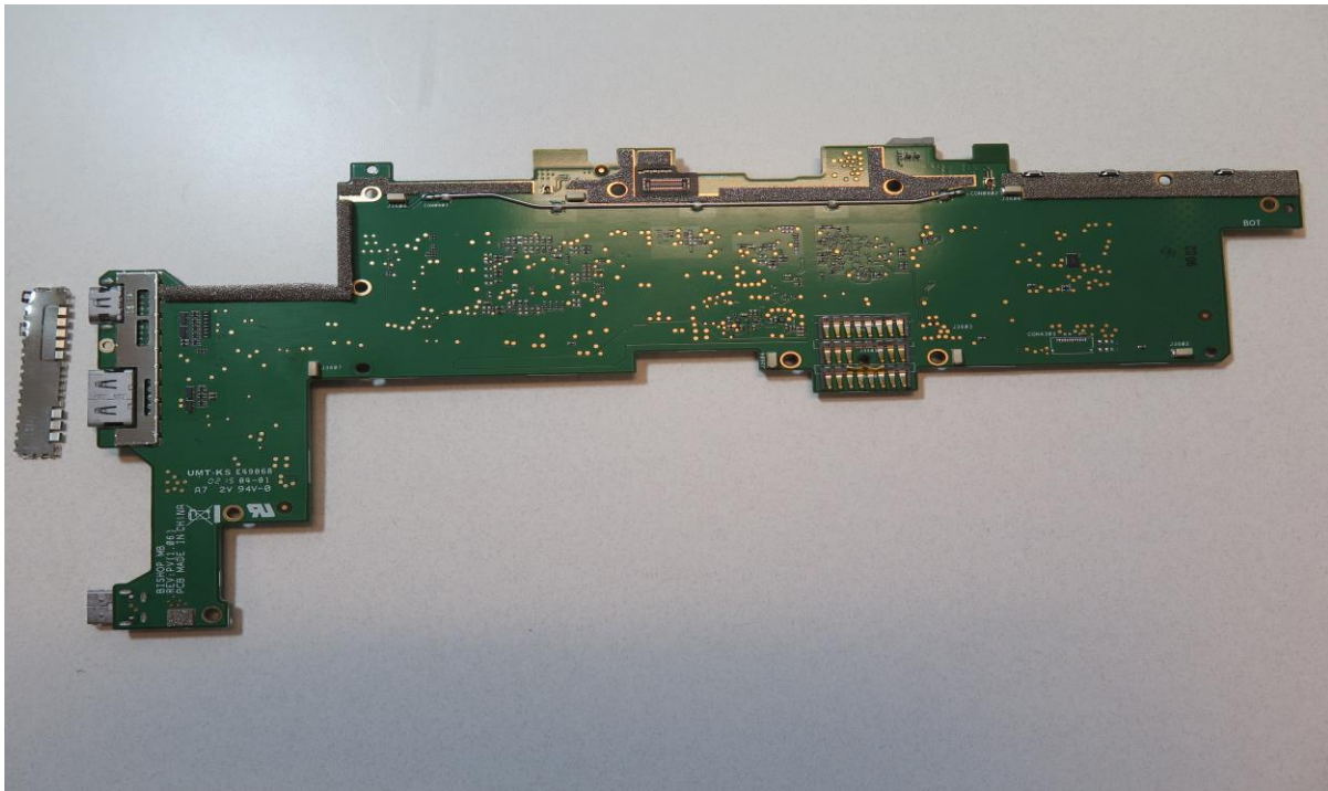
Motherboard bottom side with shield can removed
