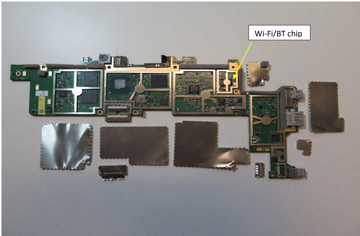
Motherboard top side with shield cans removed
