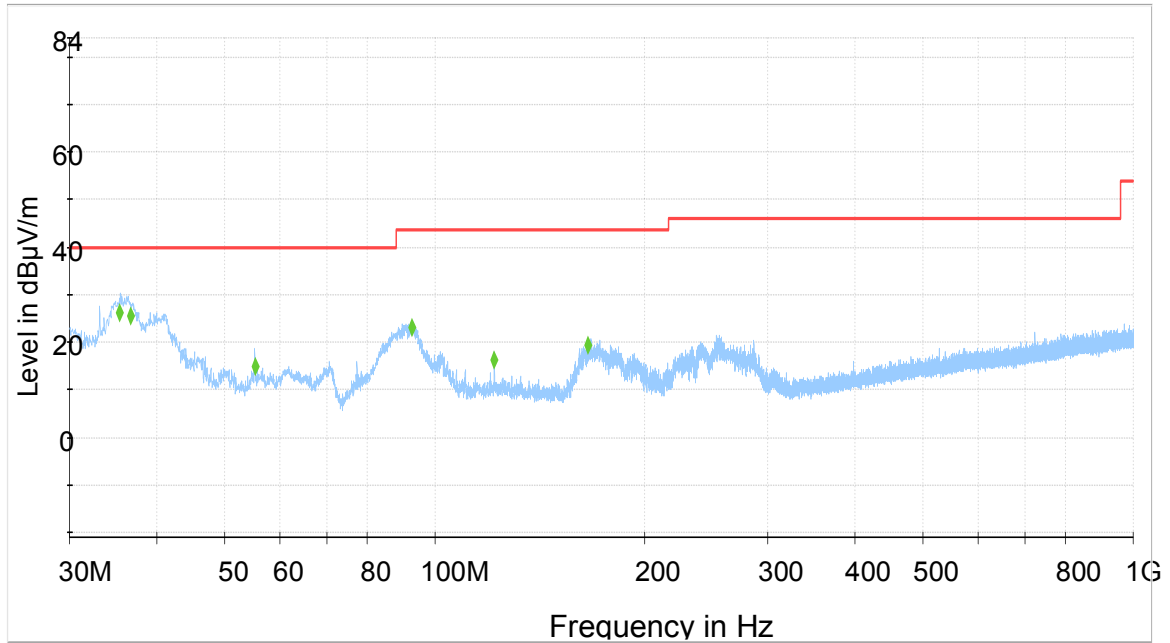
Plot 9-18. Radiated Spurious Emissions (Ch. 39) (30MHz - 1GHz)
