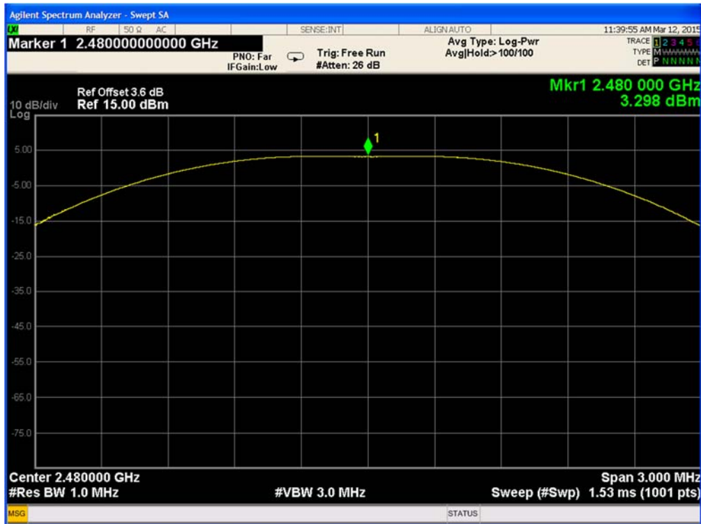
Plot 9-9. Peak Power (Ch. 39)
