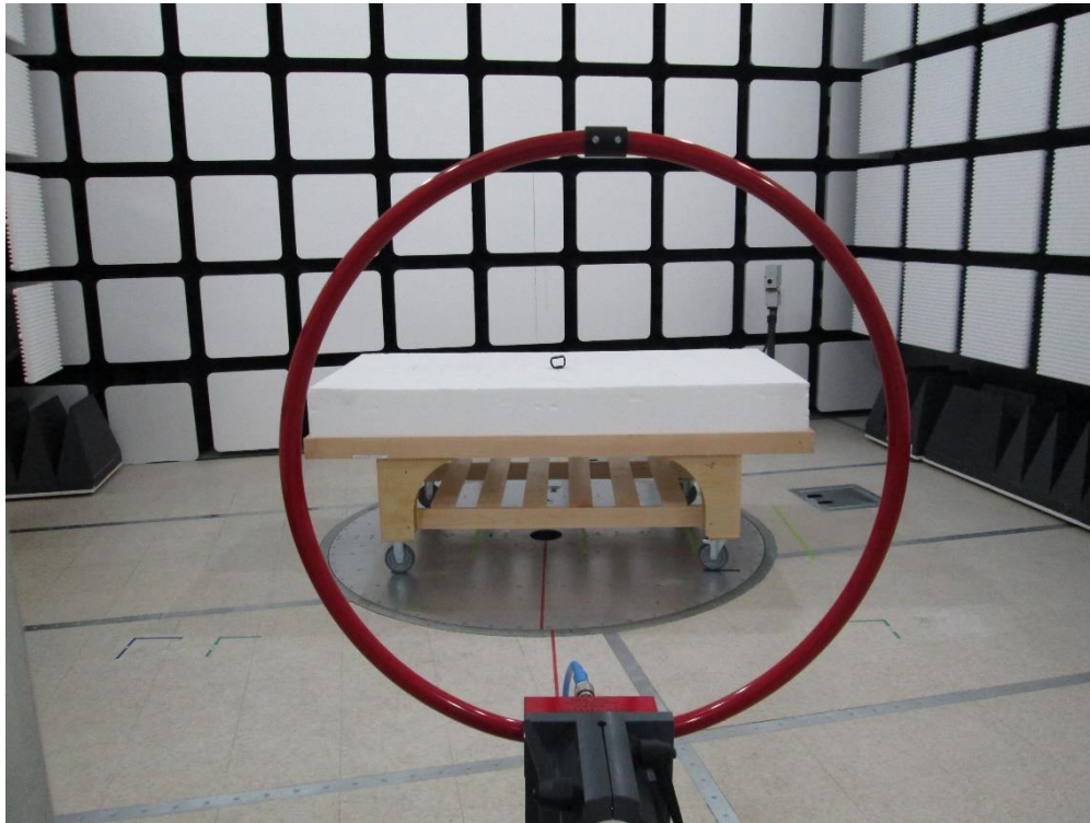
Fig.3 Radiated Emissions Test Setup (Below 30MHz)
