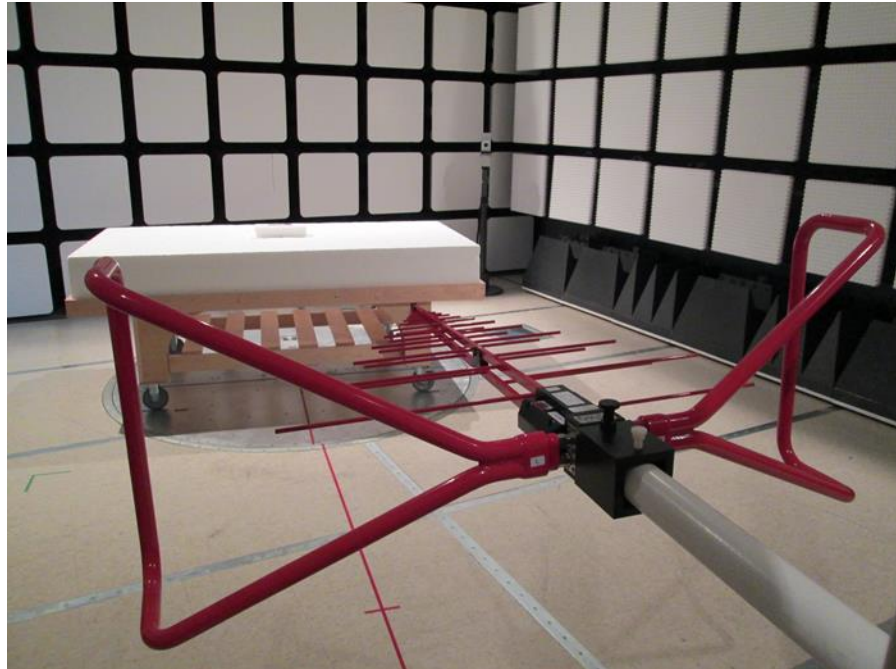
Fig.2 Radiated Emissions Test Setup (30MHz – 1GHz)
