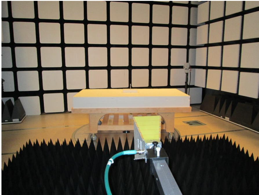
Fig.3 Radiated Emissions Test Setup (1-18GHz)
