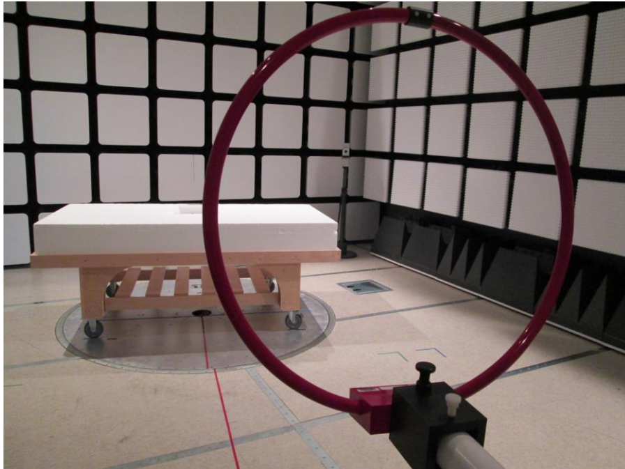
Fig.1 Radiated Emissions Test Setup (Below 30MHz)
