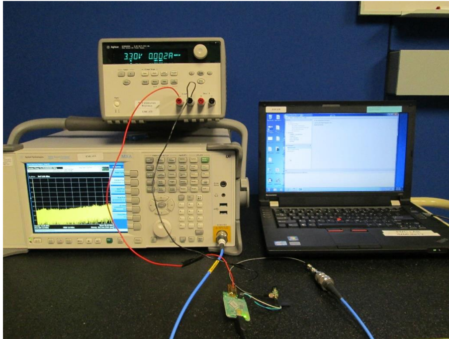
Fig.7 Antenna port Conducted Measurements Test Setup
