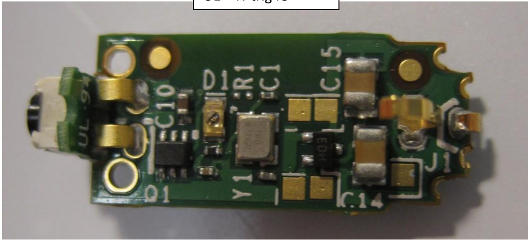
Rear portion – back side
