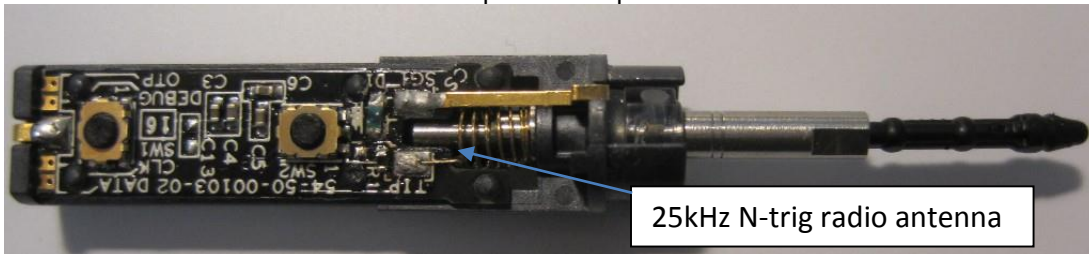
Front portion – top side
