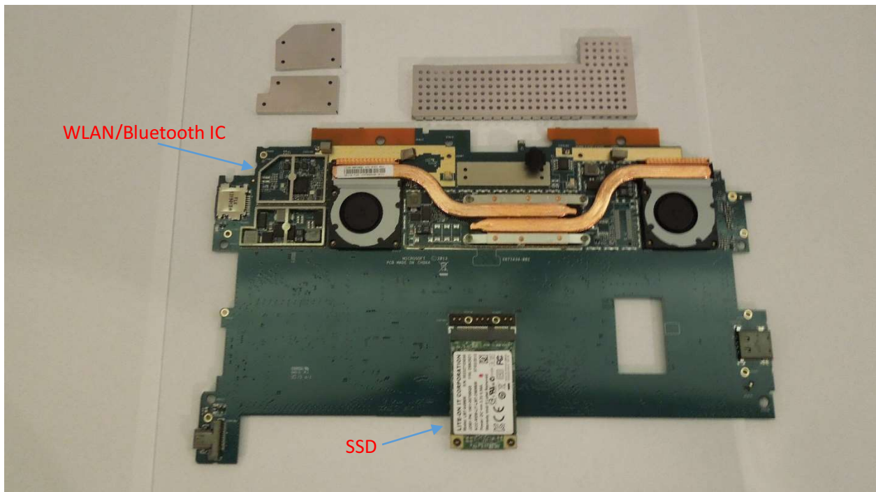
Motherboard Processor Side, with shields removed
