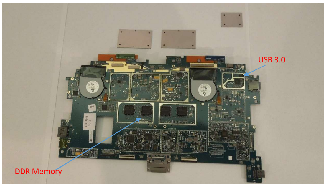
Motherboard Component Side, with shields removed
