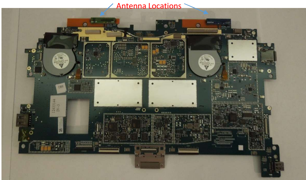
Motherboard Component Side, with shields attached
