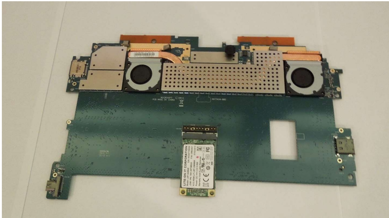
Motherboard Processor Side, with shields attached
