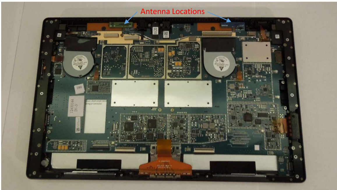
Top, with display removed
