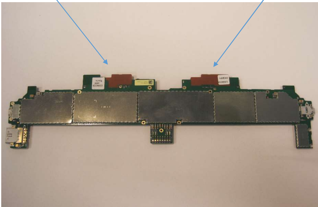
Bottom side of Wi-MIMO Antenna location
