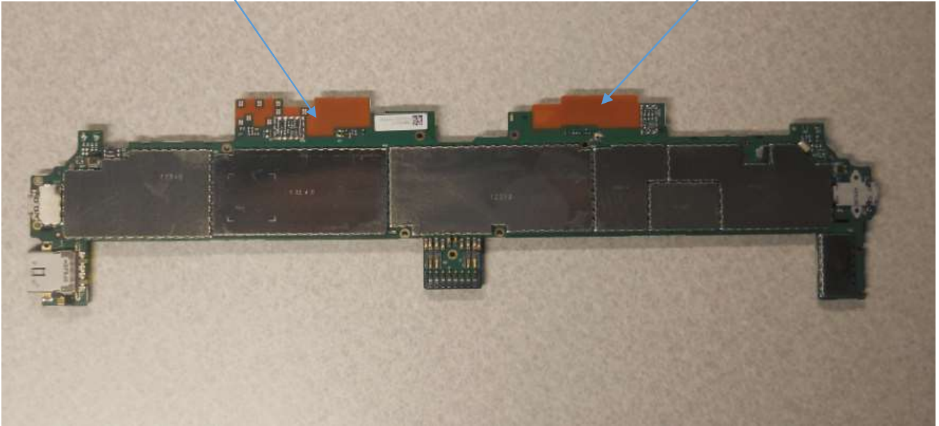
Bottom side of Wi-MIMO Antenna location
