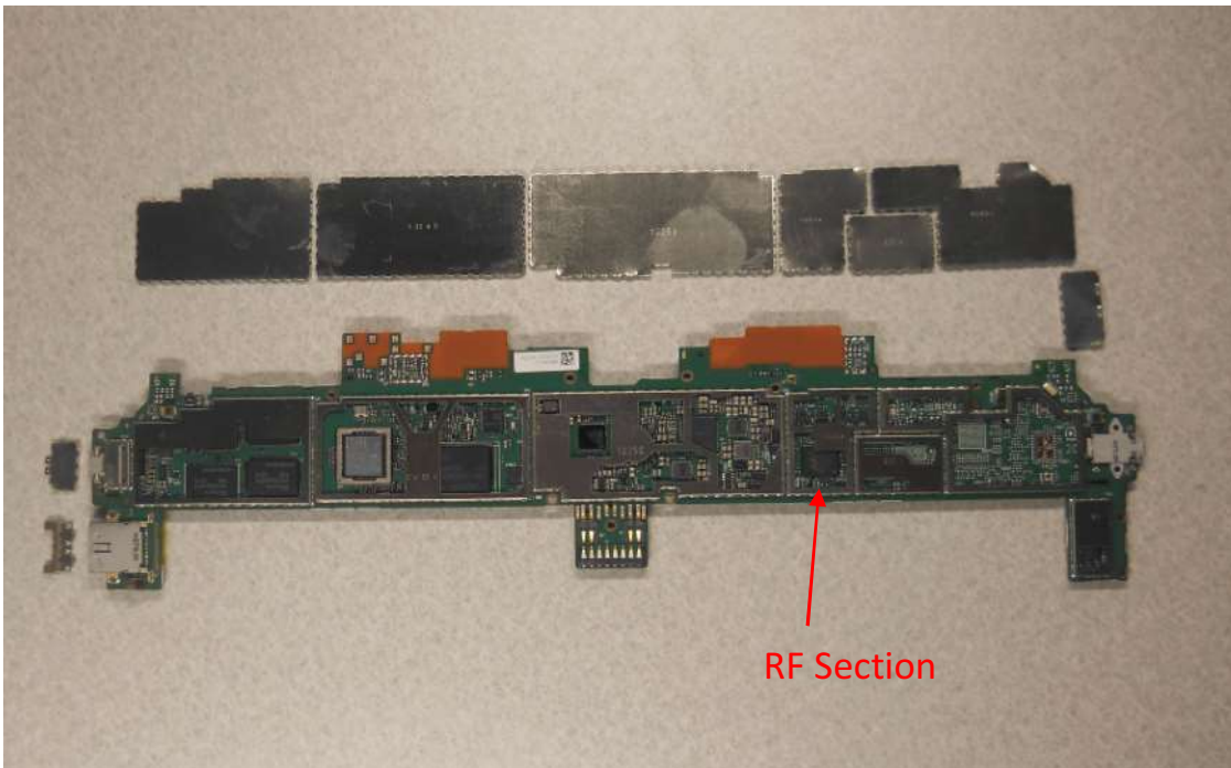
Bottom side of motherboard with shield cans removed.
