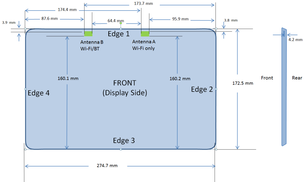
Antenna Locations
