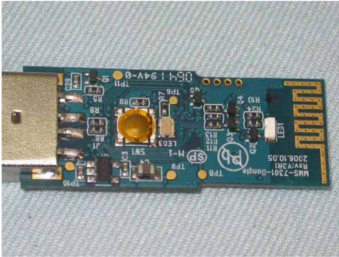
Antenna Type : PCB Antenna , Antenna Gain : 2.77dBi
