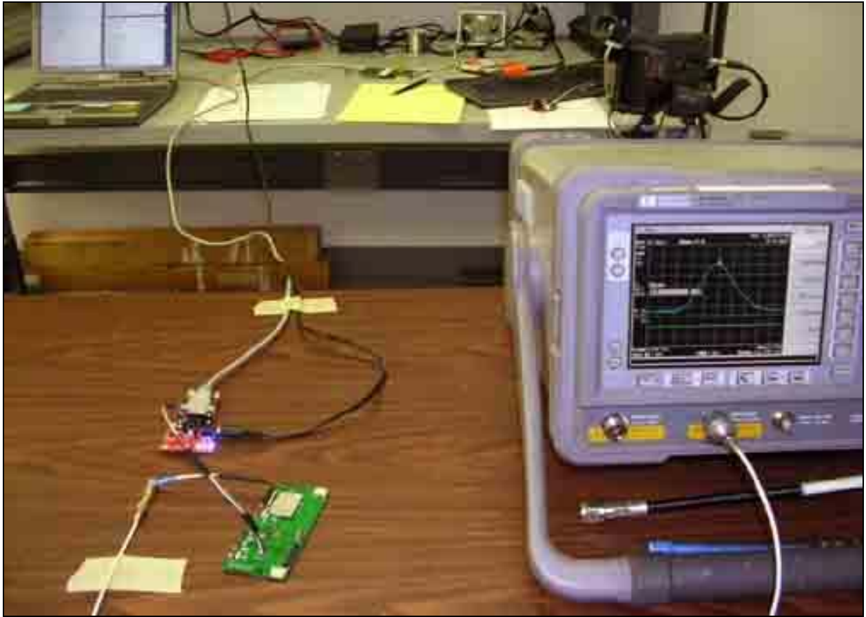
PHOTOGRAPH SHOWING DIRECT CONNECT TESTING
