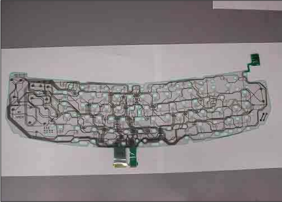
Membrane 136027 Rev A SST-1 Top
