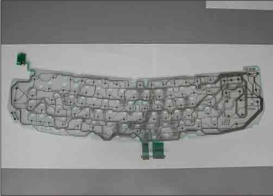
Membrane 136027 Rev A SST-1 Bottom
