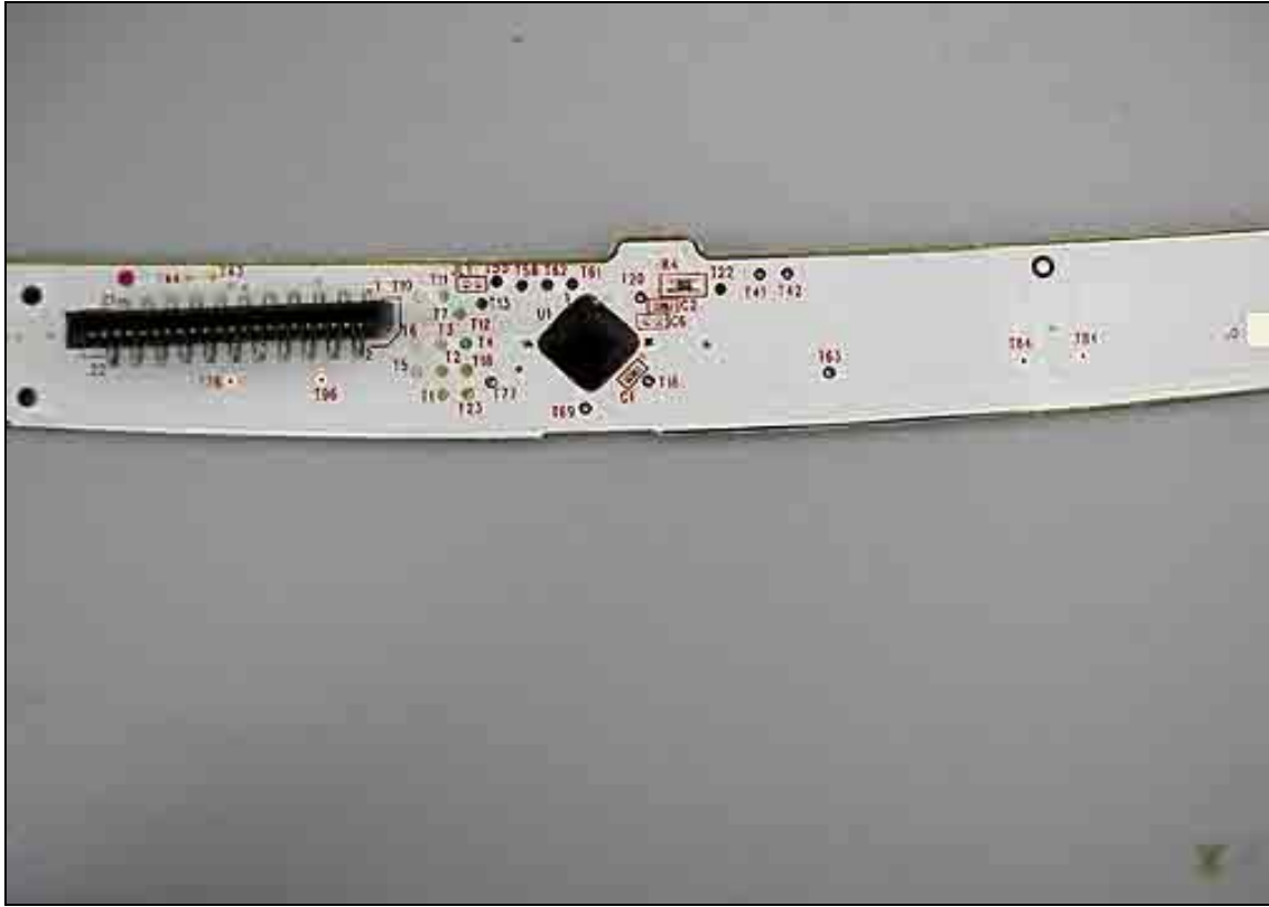
PCB 920-709-05 Rev 1 Top Side Center
