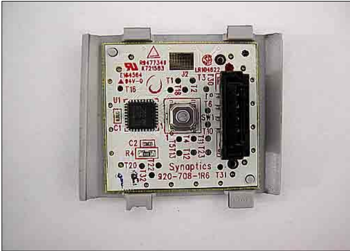
PCB 920-708-1RS T31 Top
