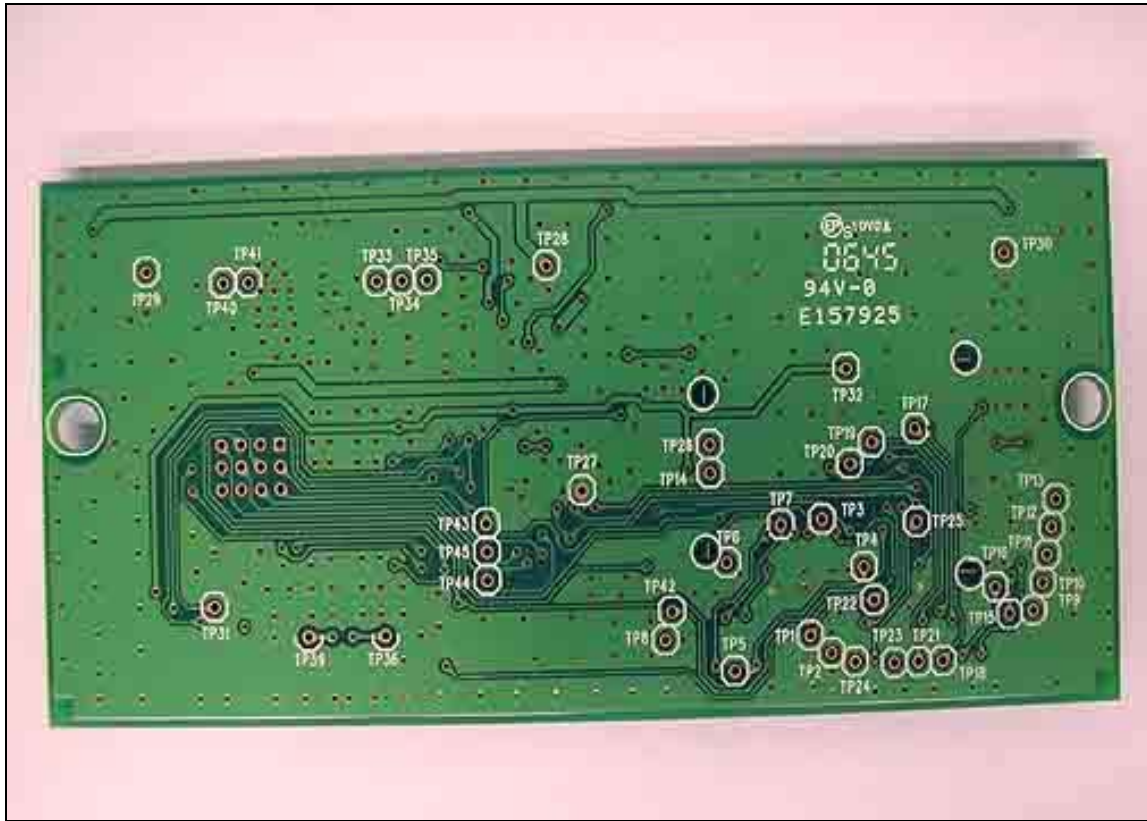
Main PCB 136552L Rev 06 Bottom
