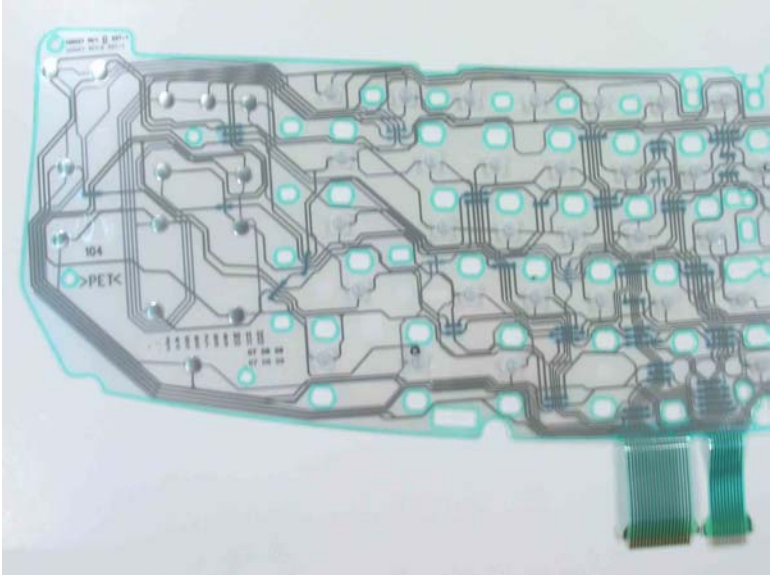
Membrane 136027 Rev B Top Left
