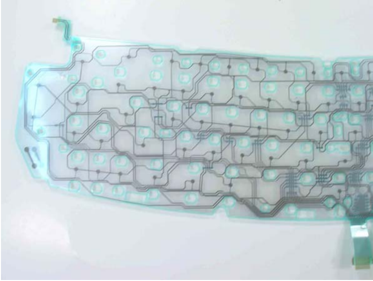
Membrane 136027 Rev B Bottom Left
