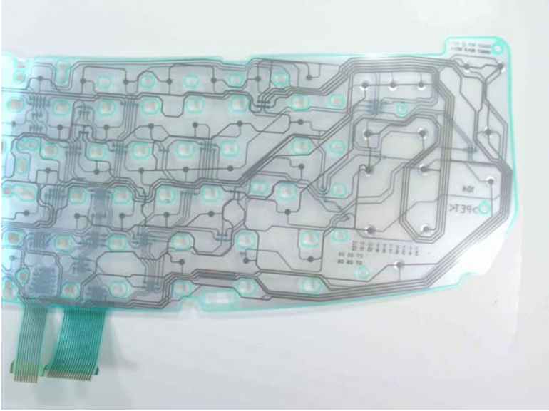
Membrane 136027 Rev B Bottom Right
