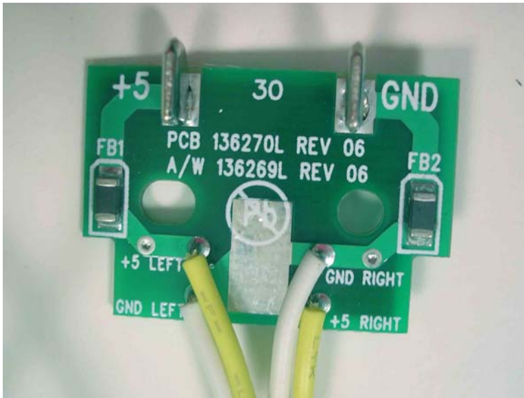
PCB 136270L Top 1
