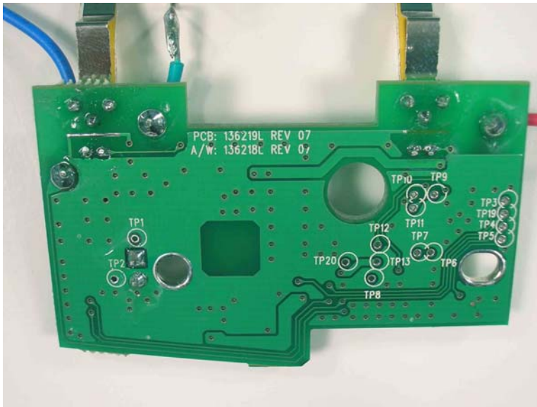
PCB 136219L Bottom
