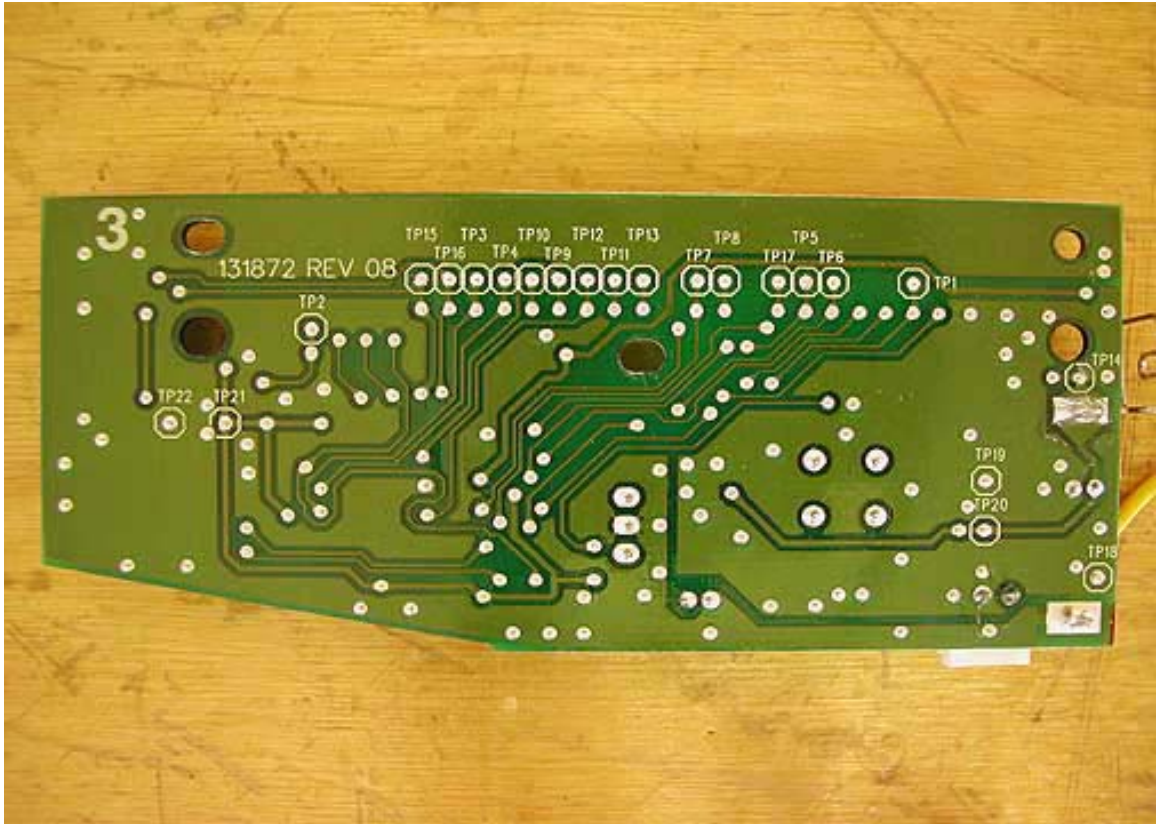
PCB Solder Side
