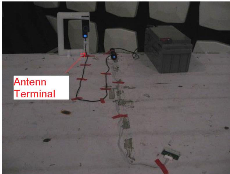
Y axis test setup photograph
