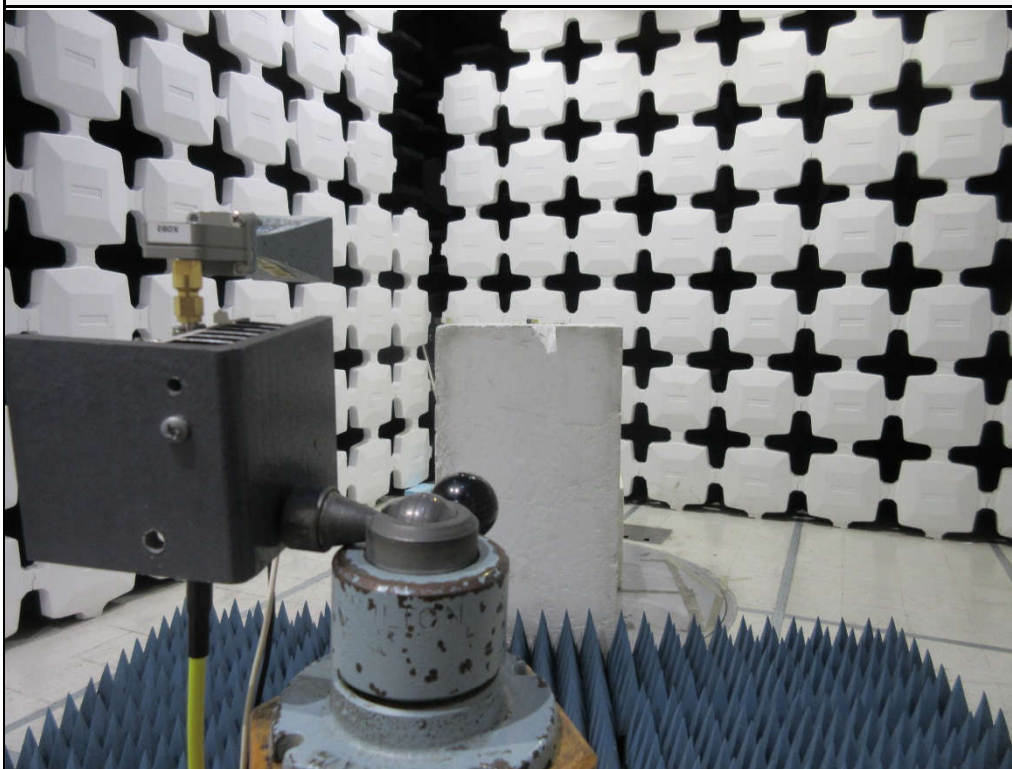
Test Setup for Spurious Radiated Emissions, 18 – 25GHz – Antenna Polarization Vertical
