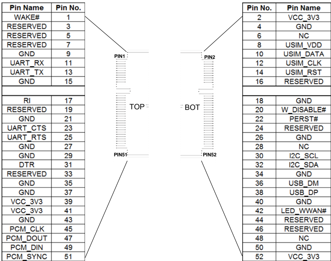
Figure 2: Pin Assignment
