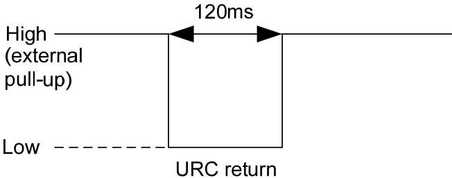
Figure 12: WAKE# Behavior
