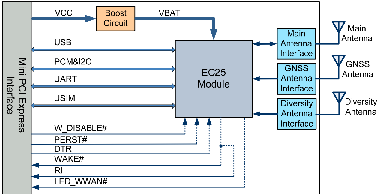
Figure 1: Functional Diagram
